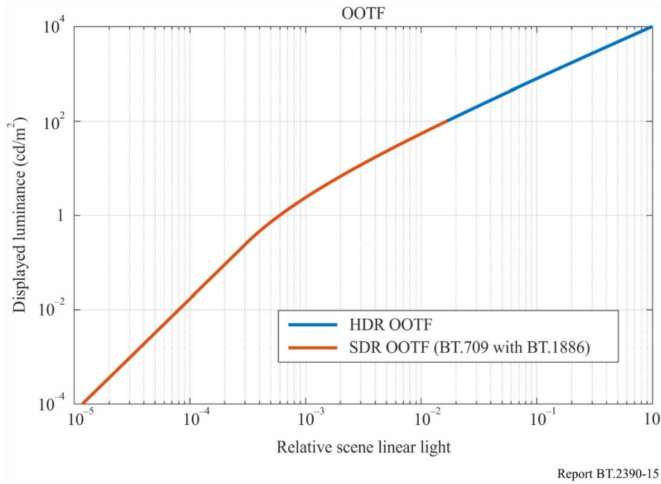
FIGURE 15 PQ and SDR OOTF
