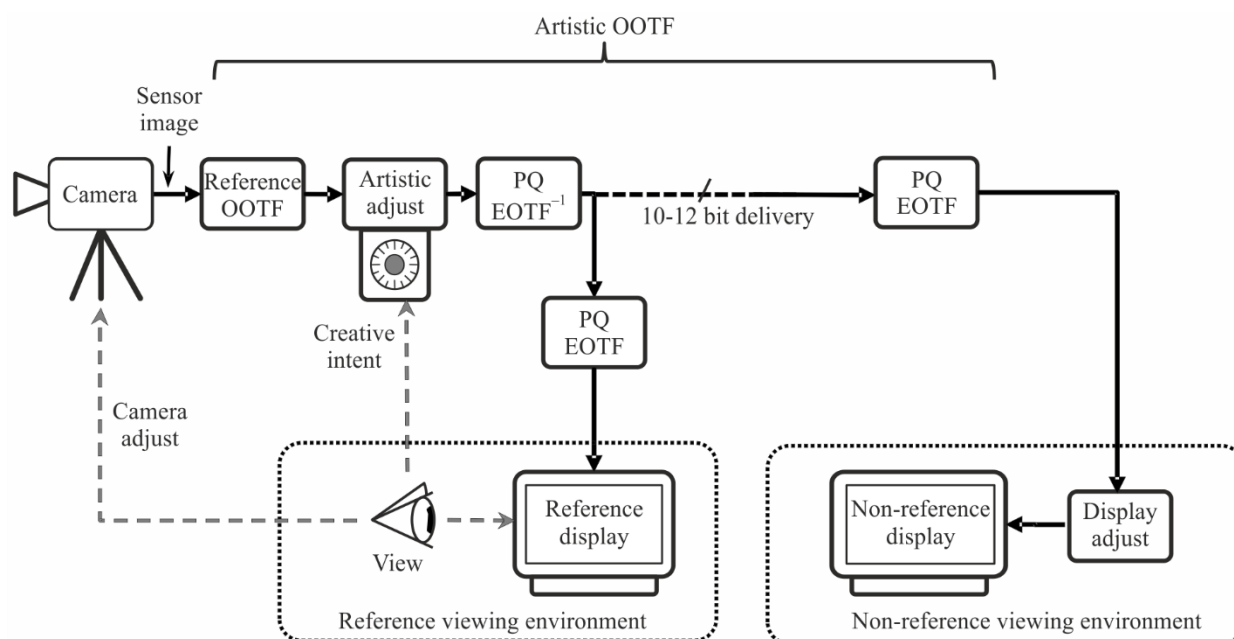
FIGURE 12 PQ HDR-TV system with 10-bit or 12-bit integer values
