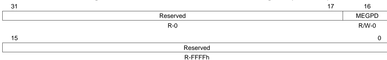
Figure 9-1. Power-Down Controller Command Register (PDCCMD)
