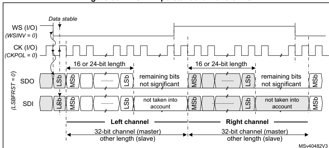
Figure 601. I2S Philips standard waveforms
