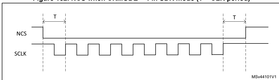
Figure 152. NCS when CKMODE = 1 in SDR mode ( T = \text{CLK period} )
