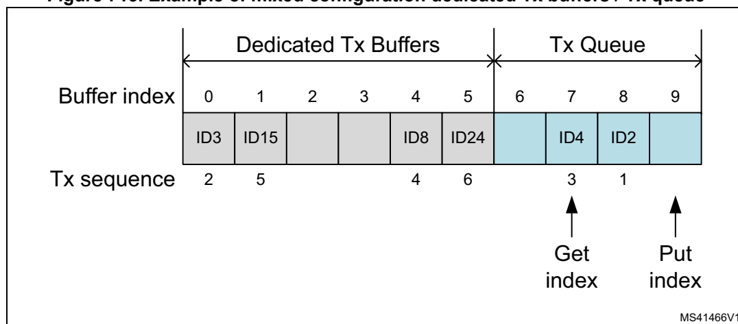
Figure 713. Example of mixed configuration dedicated Tx buffers / Tx queue
