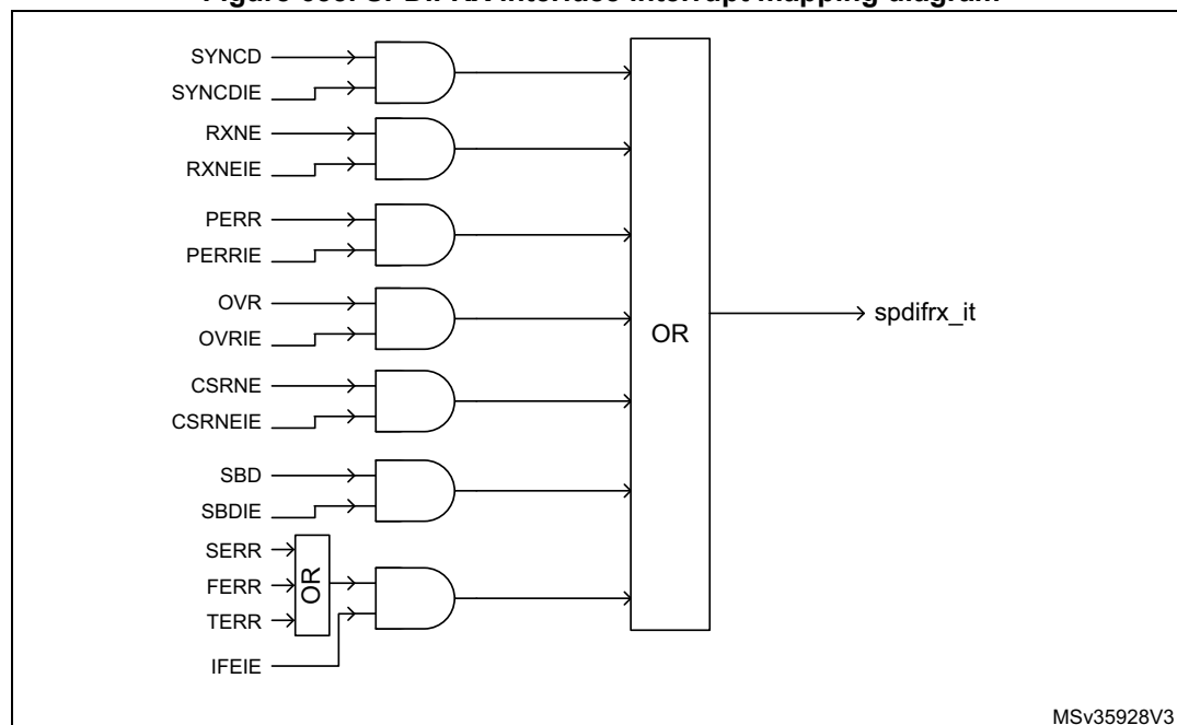
Figure 655. SPDIFRX interface interrupt mapping diagram
