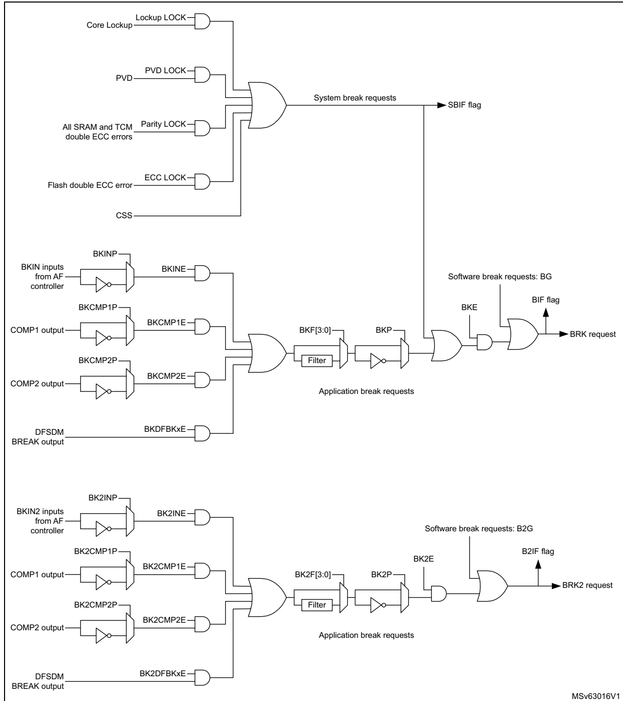
Figure 360. Break and Break2 circuitry overview
