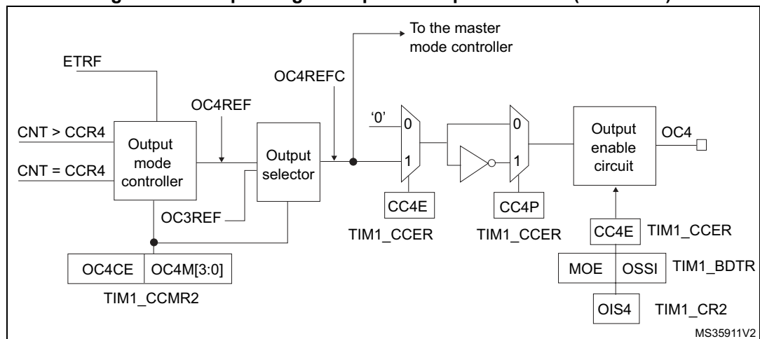
Figure 348. Output stage of capture/compare channel (channel 4)
