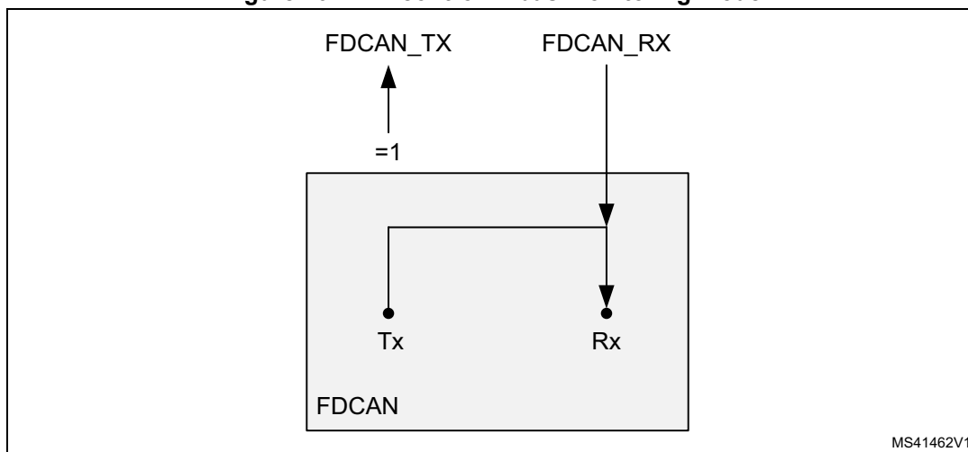
Figure 707. Pin control in bus monitoring mode
