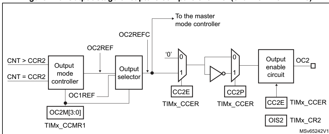
Figure 470. Output stage of capture/compare channel (channel 2 for TIM15)
