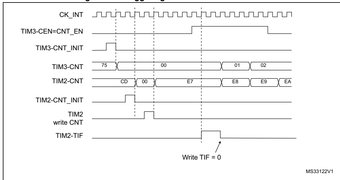
Figure 425. Triggering TIM2 with Enable of TIM3
