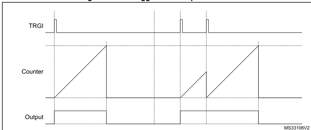
Figure 368. Retriggerable one pulse mode
