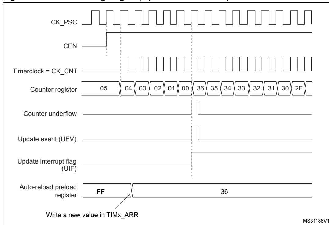
Figure 330. Counter timing diagram, update event when repetition counter is not used
