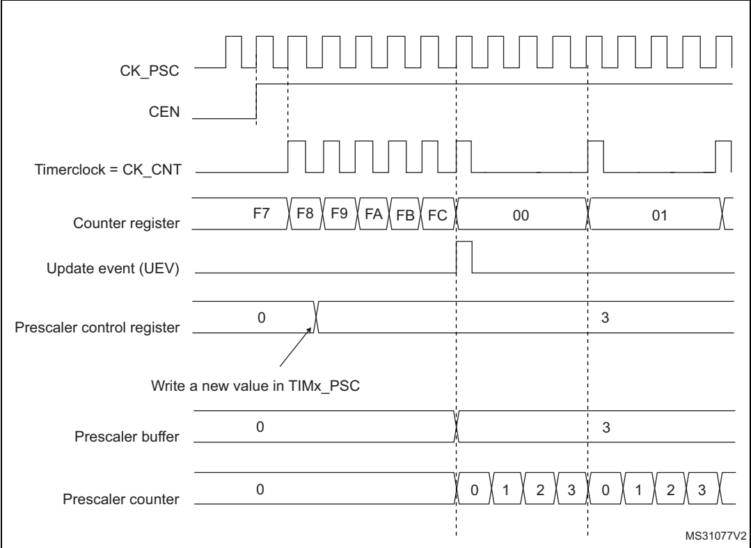
Figure 456. Counter timing diagram with prescaler division change from 1 to 4
