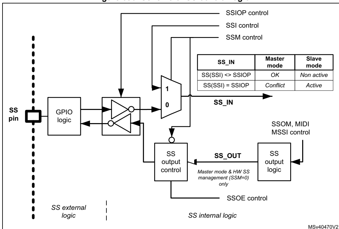
Figure 590. Scheme of SS control logic
