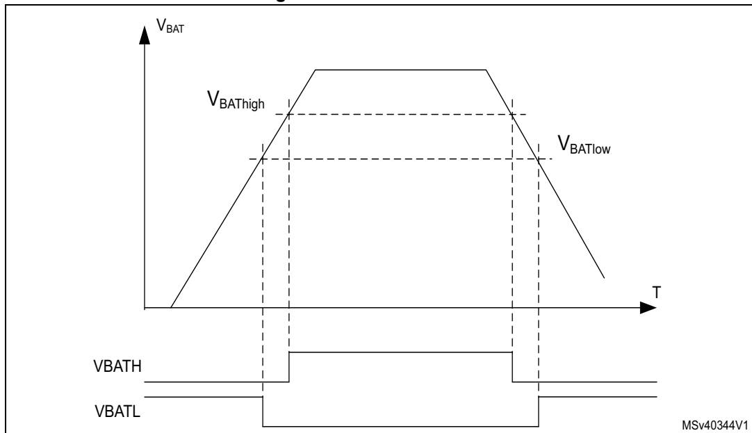
Figure 31. VBAT thresholds
