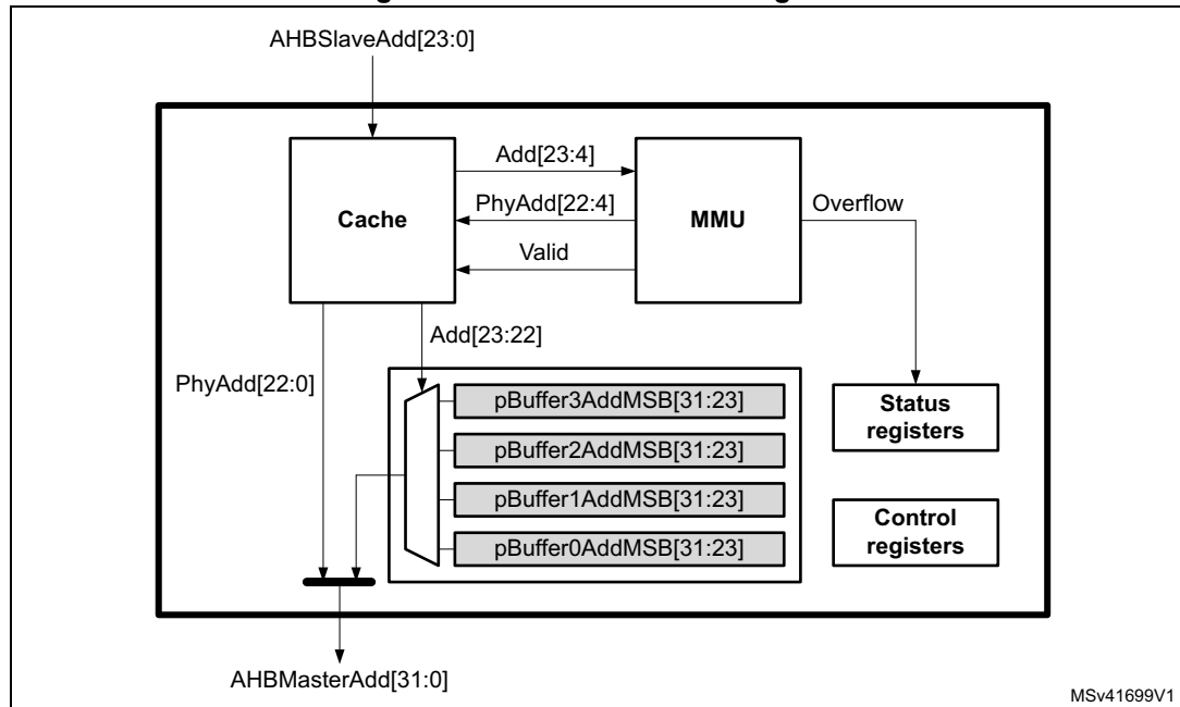
Figure 101. GFXMMU block diagram
