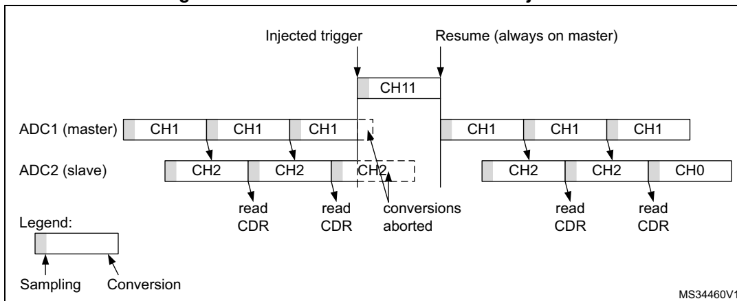
Figure 213. Interleaved conversion with injection
