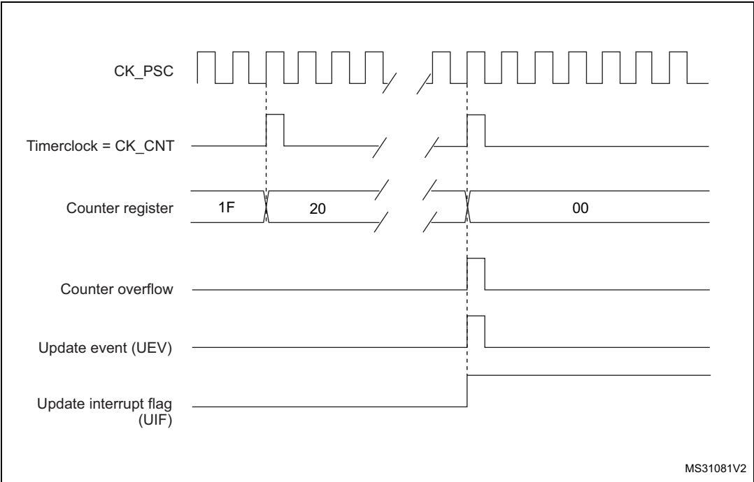
Figure 384. Counter timing diagram, Update event when ARPE=0 (TIMx_ARR not preloaded)
