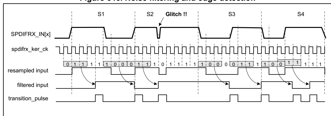
Figure 646. Noise filtering and edge detection
