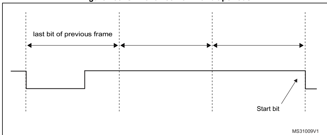
Figure 758. SFT of three nominal bit periods
