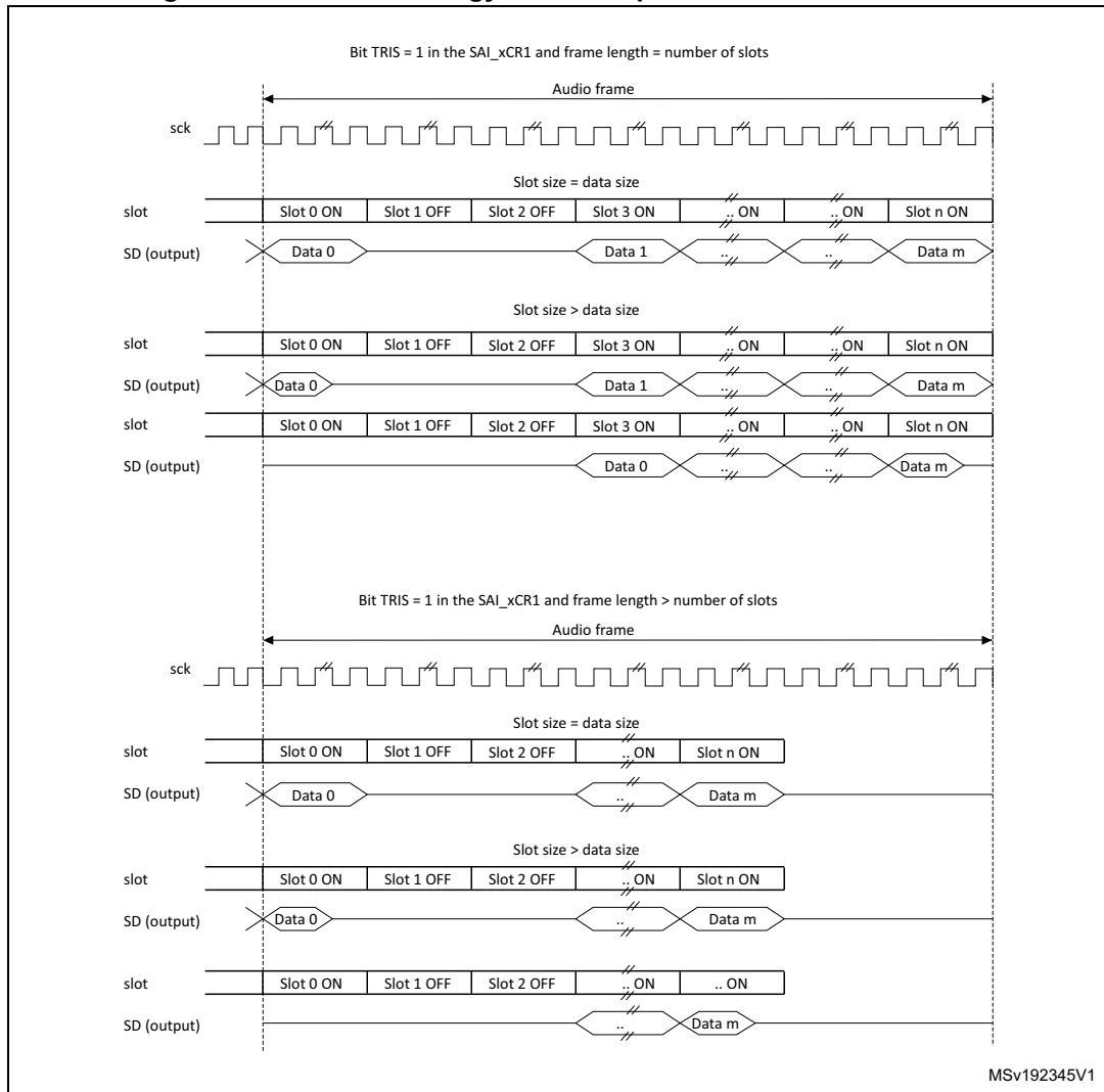
Figure 636. Tristate strategy on SD output line on an inactive slot
