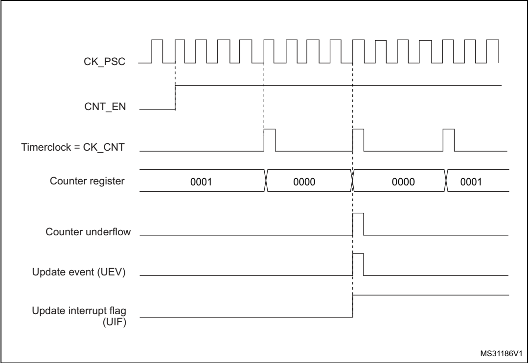
Figure 328. Counter timing diagram, internal clock divided by 4
