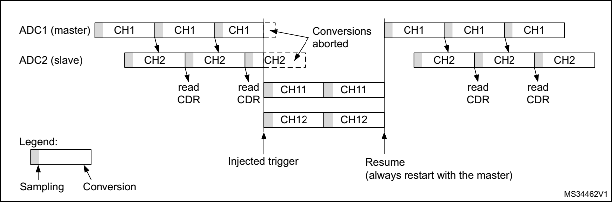
Figure 220. Two Interleaved channels (CH1, CH2) with injected sequence CH11, CH12 - case 2: Slave interrupted first
