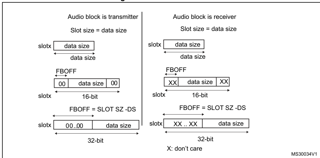
Figure 623. First bit offset
