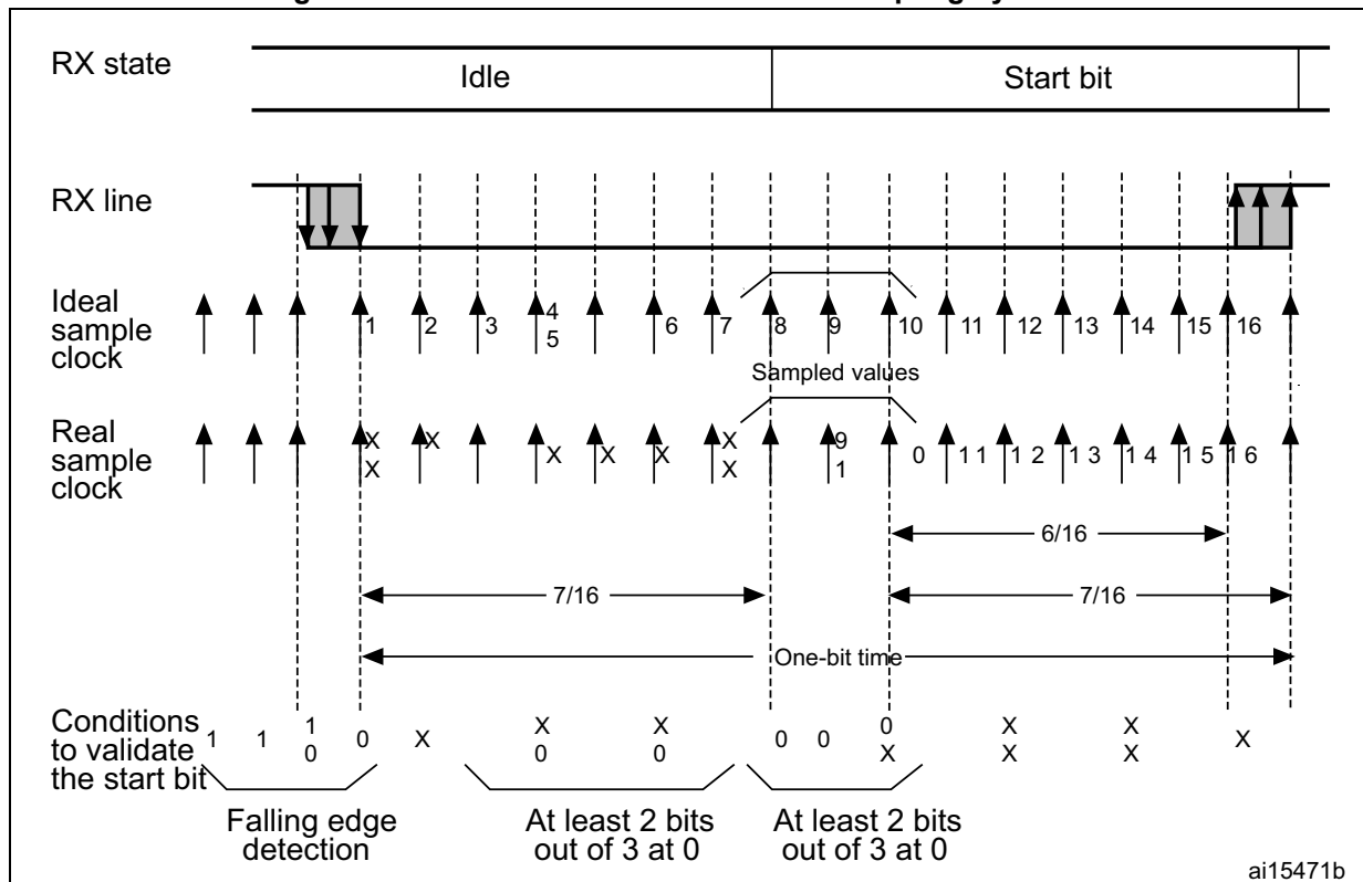
Figure 546. Start bit detection when oversampling by 16 or 8
