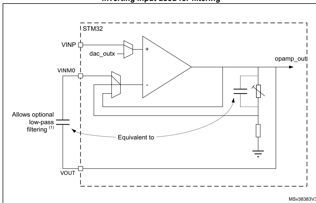
Figure 248. PGA mode, internal gain setting (x2/x4/x8/x16), inverting input used for filtering
