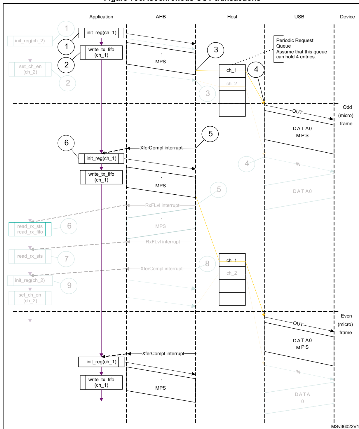
Figure 736. Isochronous OUT transactions
