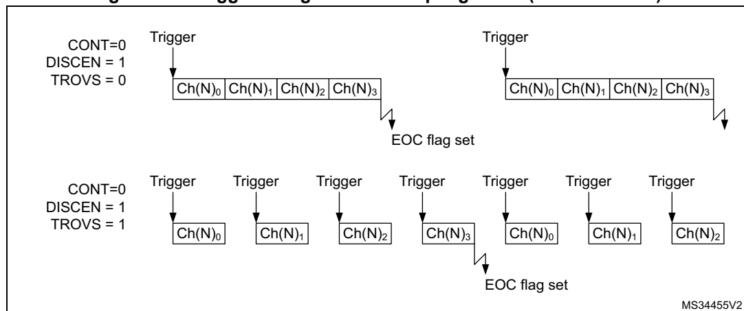
Figure 203. Triggered regular oversampling mode (TROVS bit = 1)
