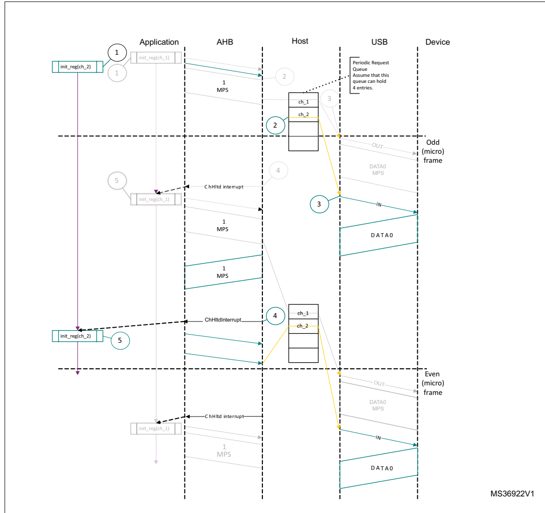
Figure 743. Normal isochronous IN transactions - DMA mode
