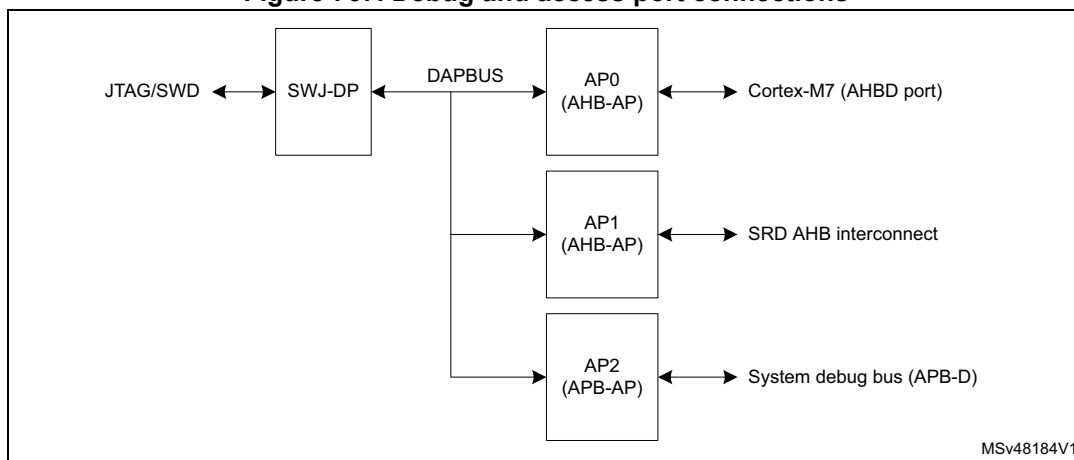
Figure 767. Debug and access port connections
