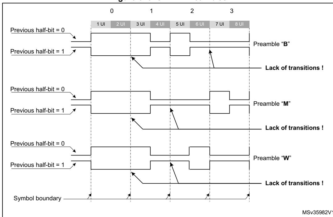
Figure 643. S/PDIF Preambles
