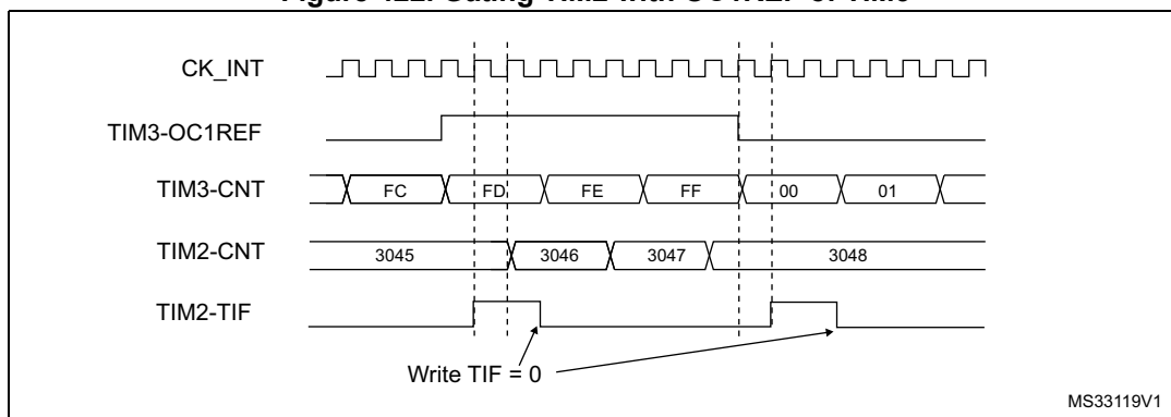
Figure 422. Gating TIM2 with OC1REF of TIM3
