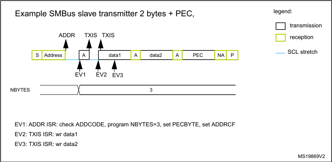
Figure 536. Transfer bus diagrams for SMBus slave transmitter (SBC = 1)
