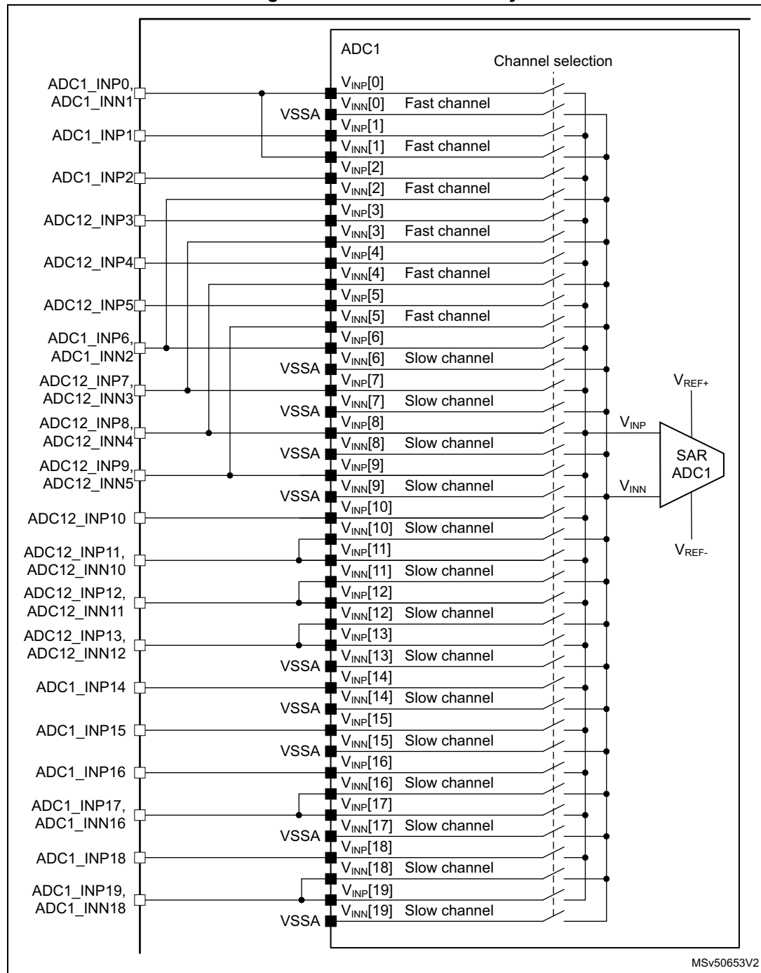
Figure 159. ADC1 connectivity
