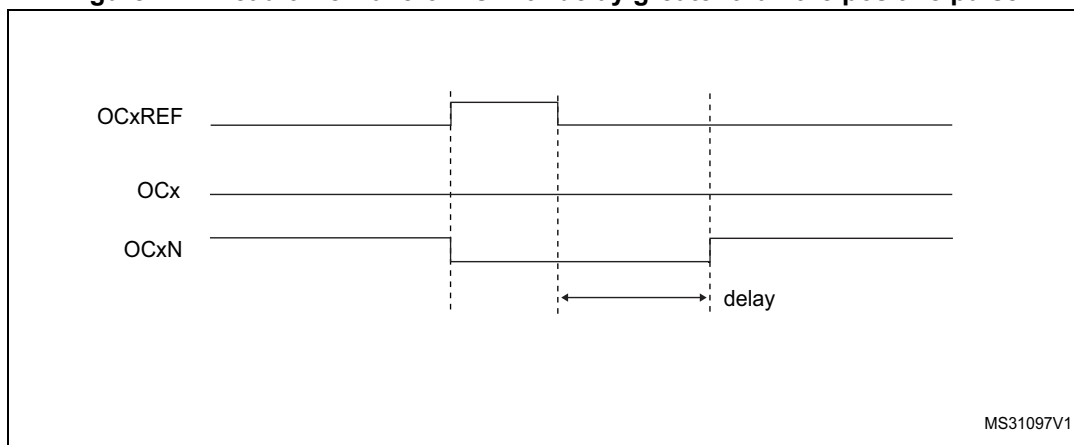
Figure 477. Dead-time waveforms with delay greater than the positive pulse.
