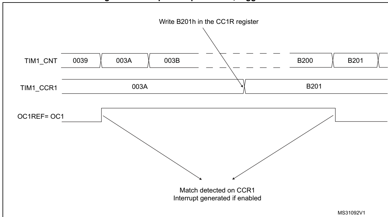
Figure 472. Output compare mode, toggle on OC1
