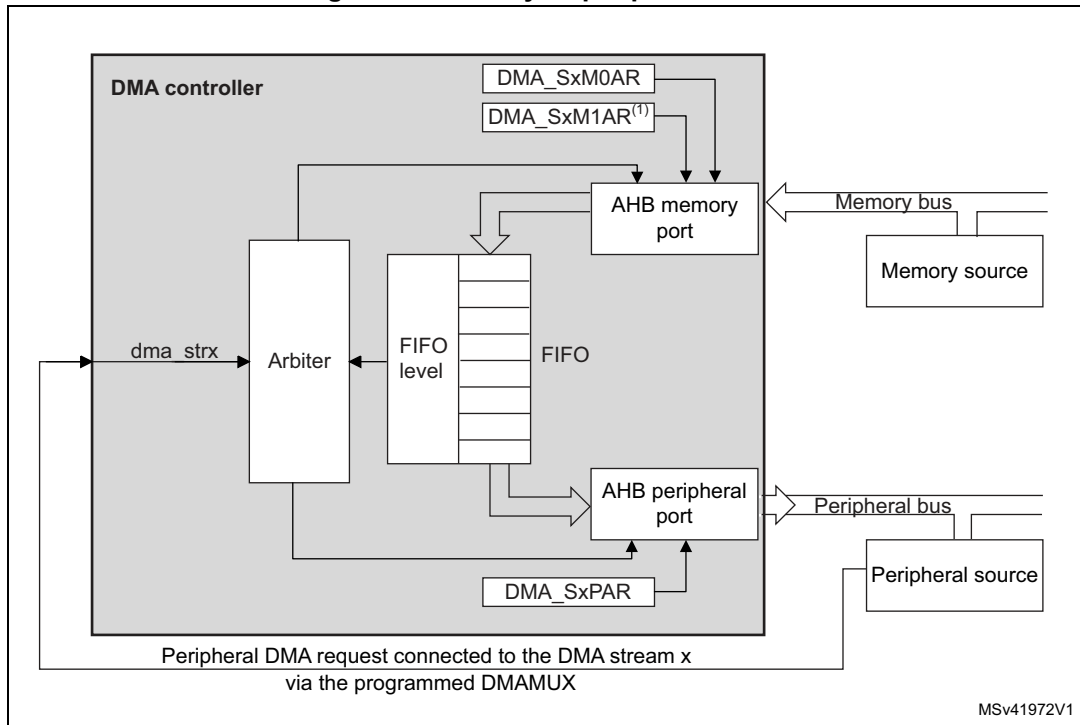
Figure 85. Memory-to-peripheral mode
