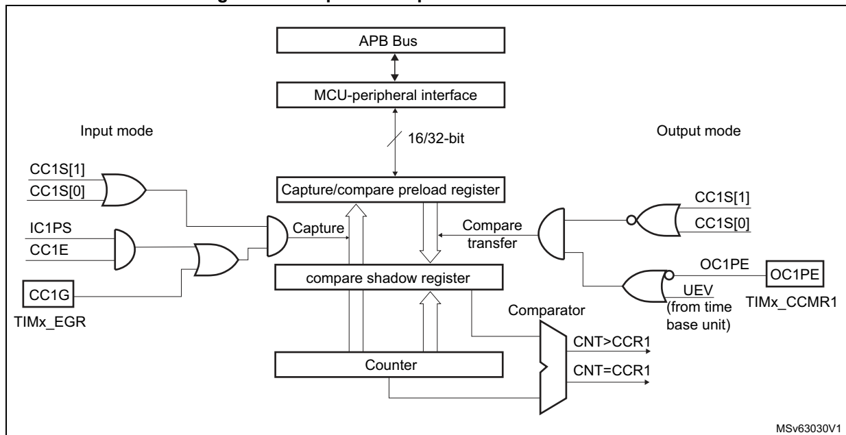
Figure 403. Capture/Compare channel 1 main circuit
