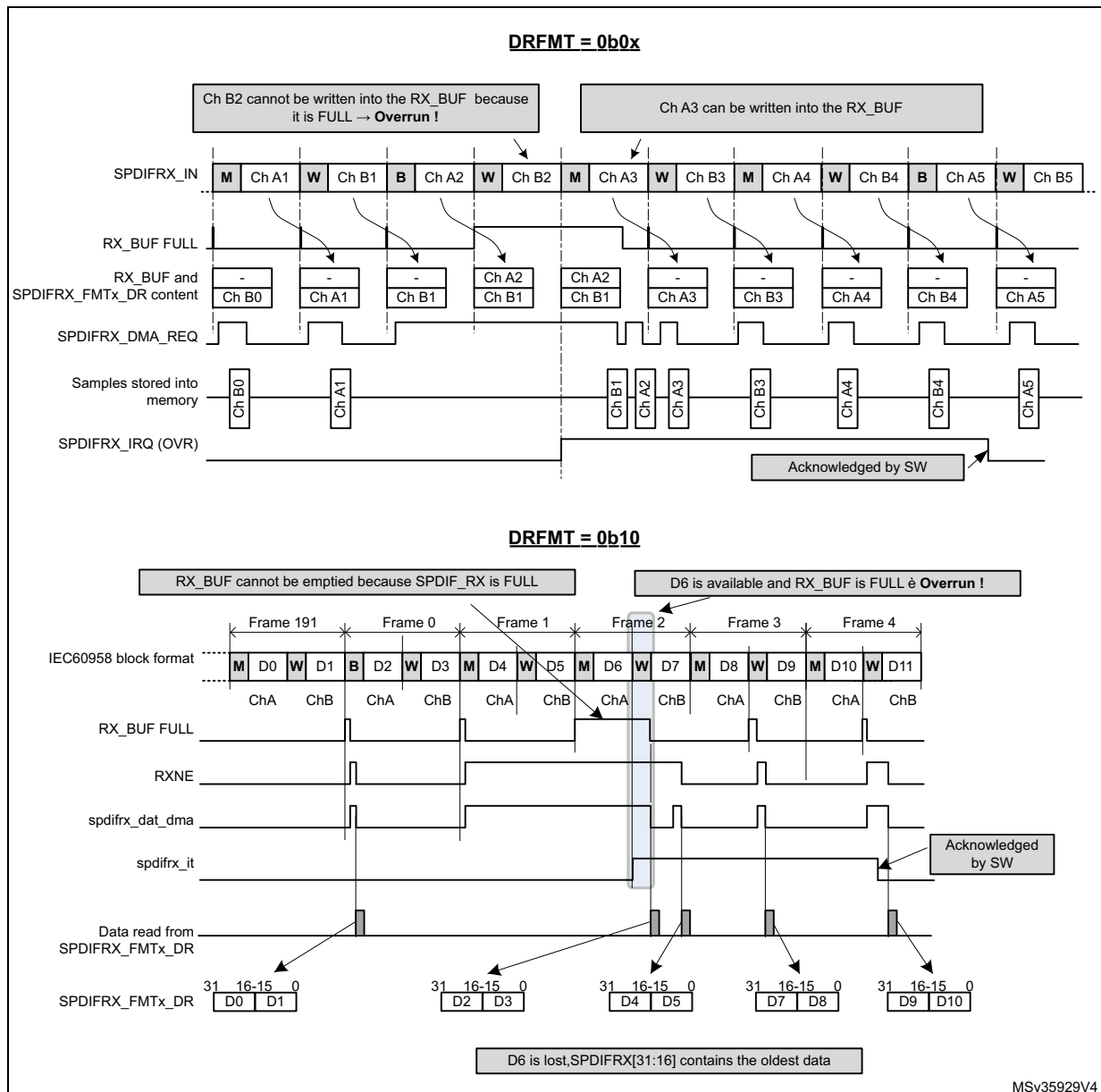
Figure 653. S/PDIF overrun error when RXSTEO = 0
