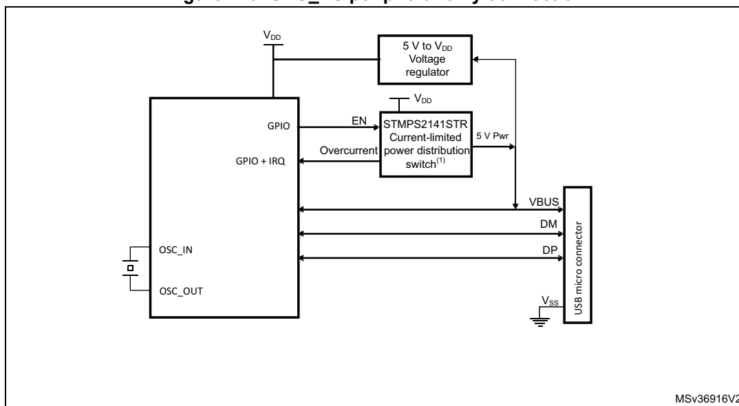
Figure 723. OTG_HS peripheral-only connection
