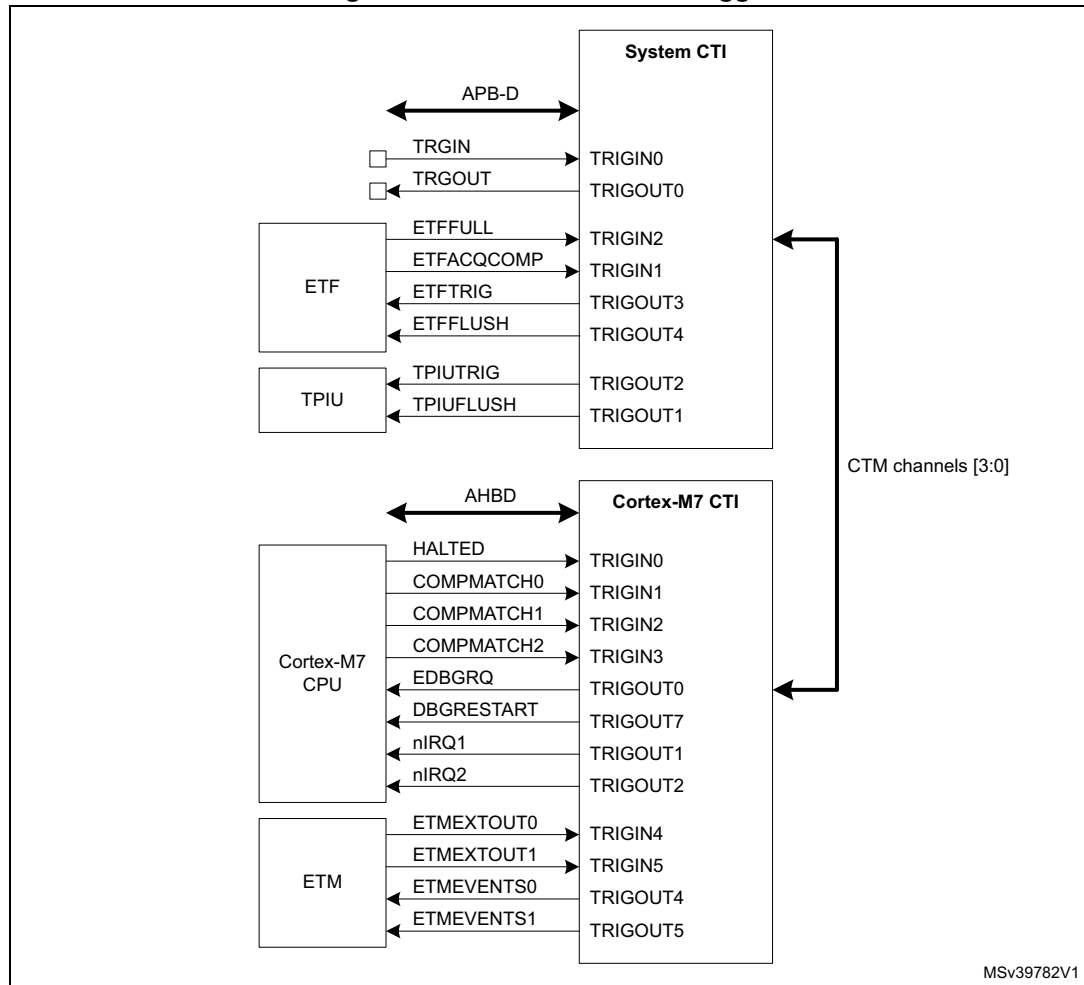
Figure 769. Embedded cross trigger
