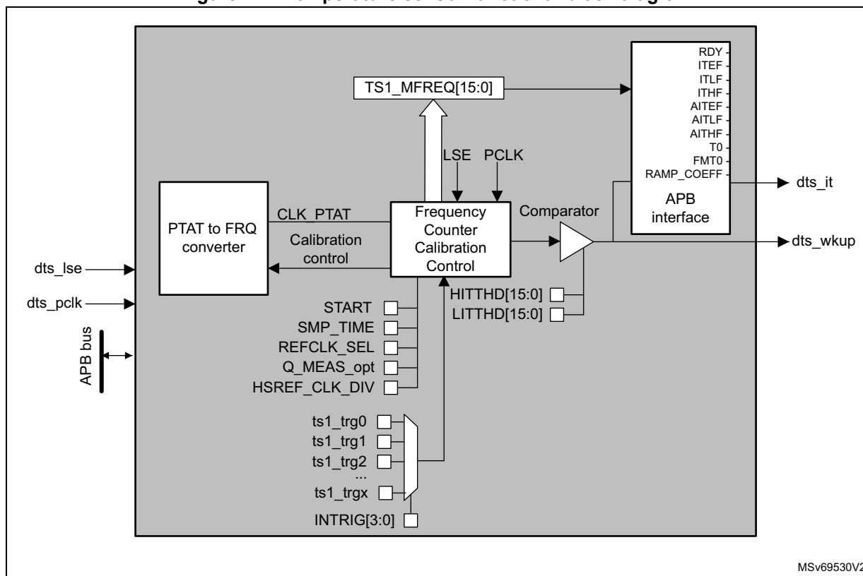
Figure 227. Temperature sensor functional block diagram
