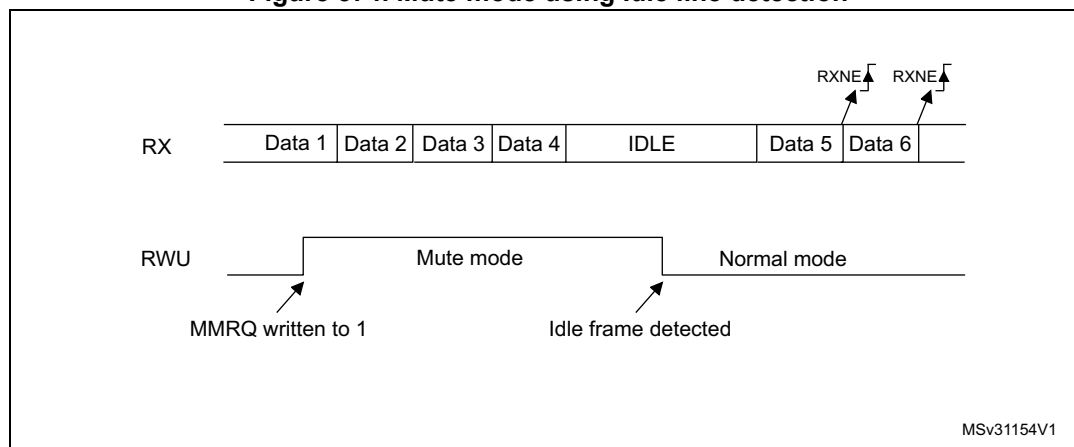
Figure 574. Mute mode using Idle line detection
