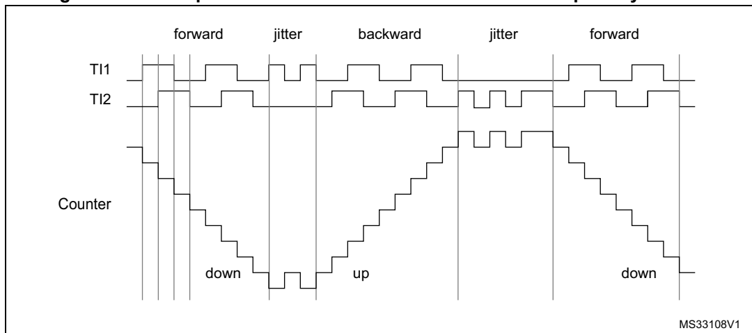
Figure 415. Example of encoder interface mode with TI1FP1 polarity inverted
