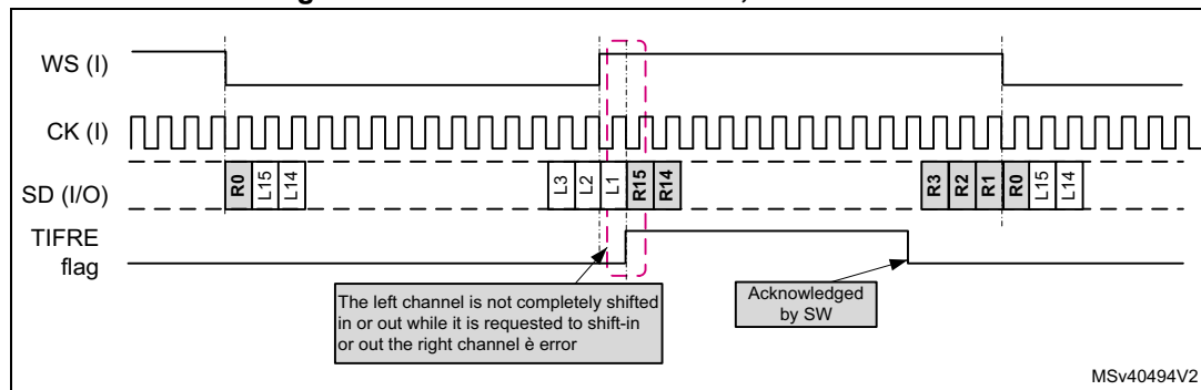
Figure 616. Frame error detection, with FIXCH=0
