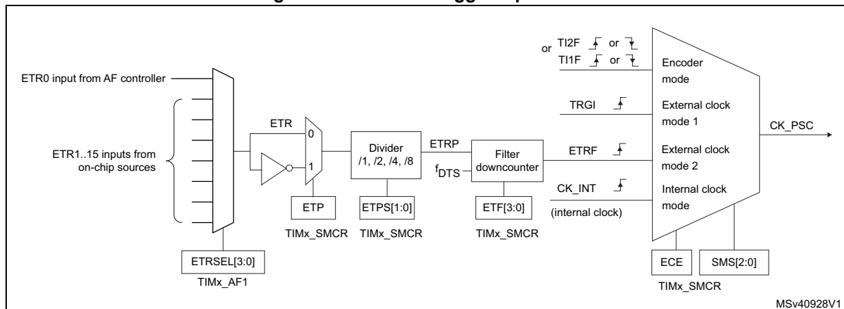
Figure 400. External trigger input block
