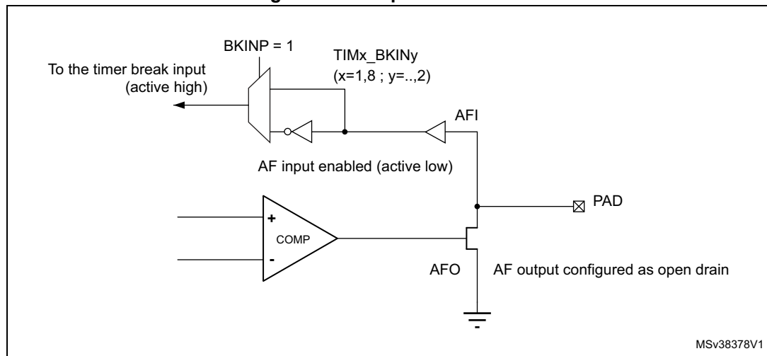
Figure 243. Output redirection
