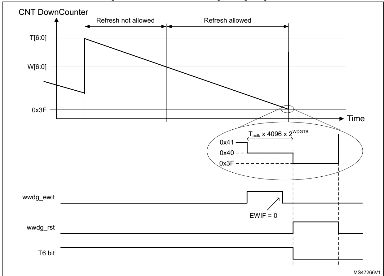
Figure 507. Window watchdog timing diagram
