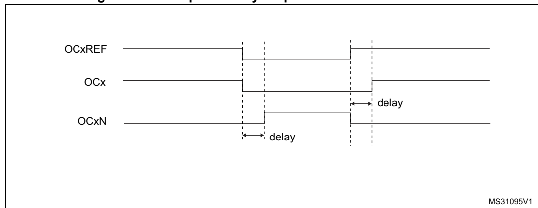
Figure 357. Complementary output with dead-time insertion
