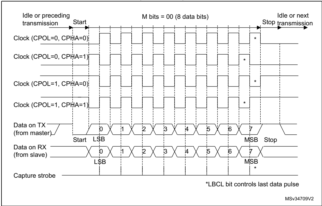
Figure 555. USART data clock timing diagram in synchronous master mode (M bits = 00)
