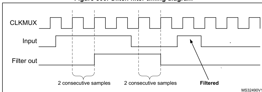
Figure 500. Glitch filter timing diagram
