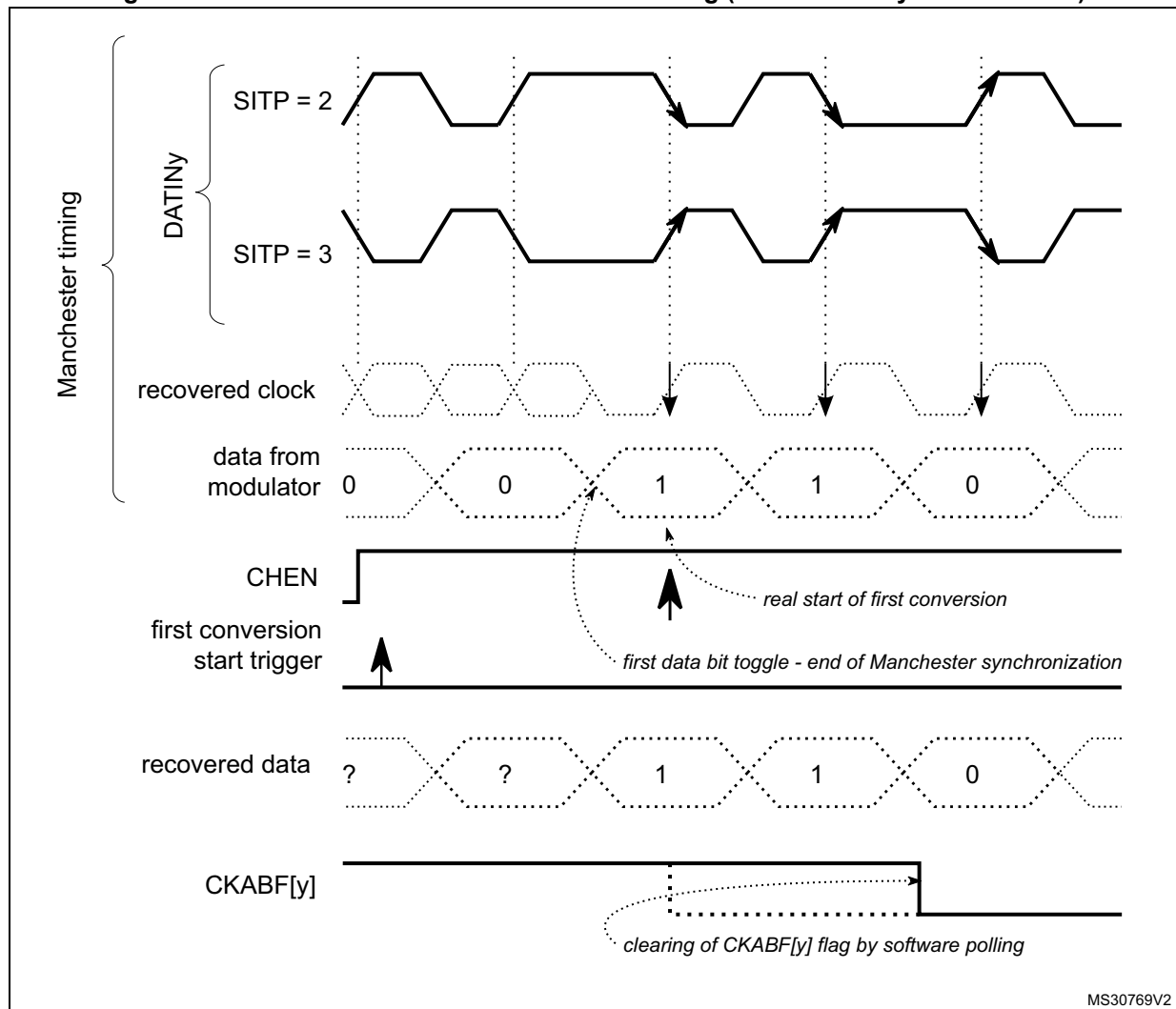
Figure 258. First conversion for Manchester coding (Manchester synchronization)
