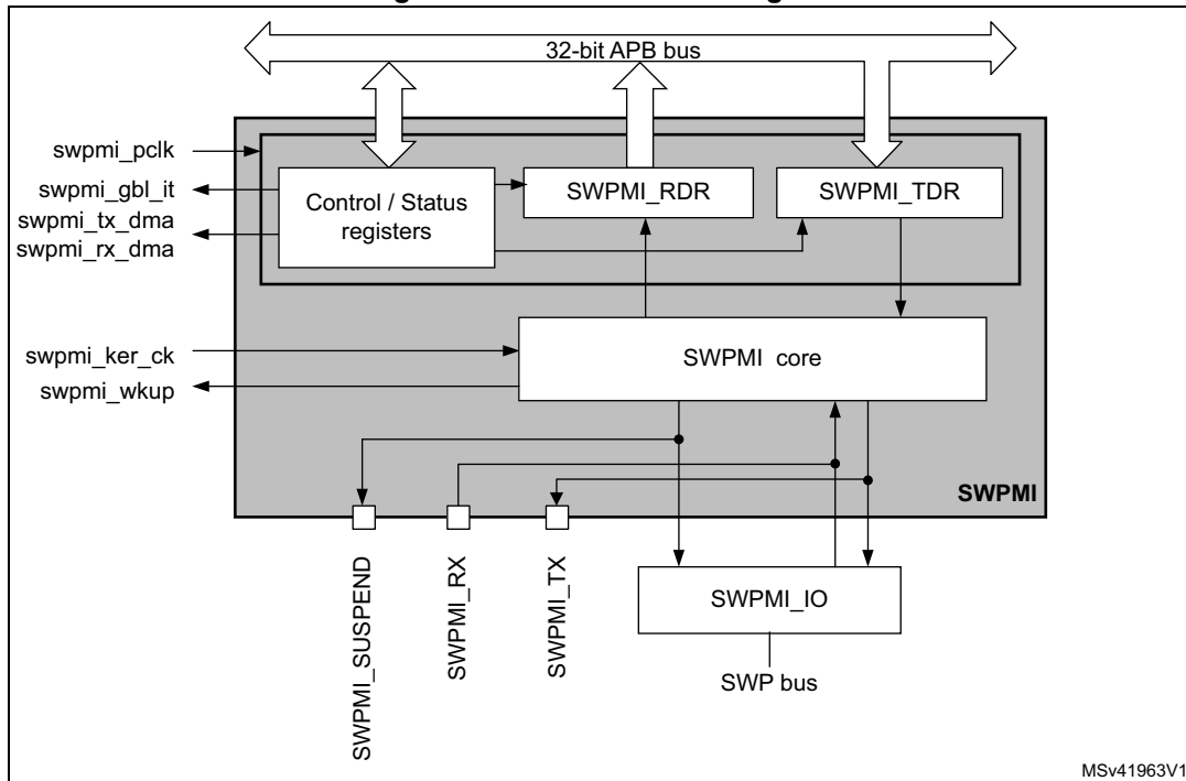
Figure 658. SWPMI block diagram
