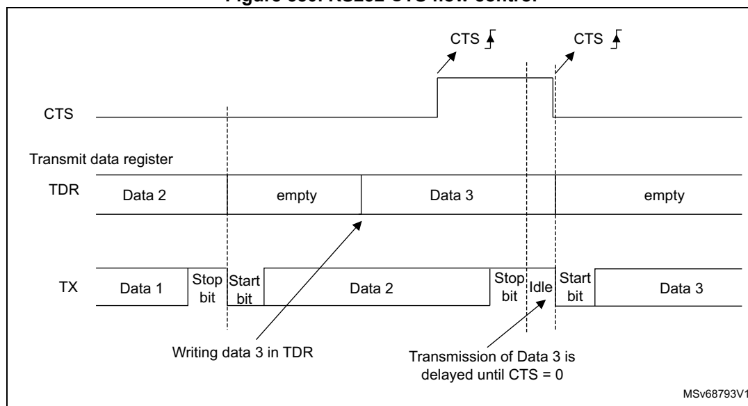
Figure 580. RS232 CTS flow control
