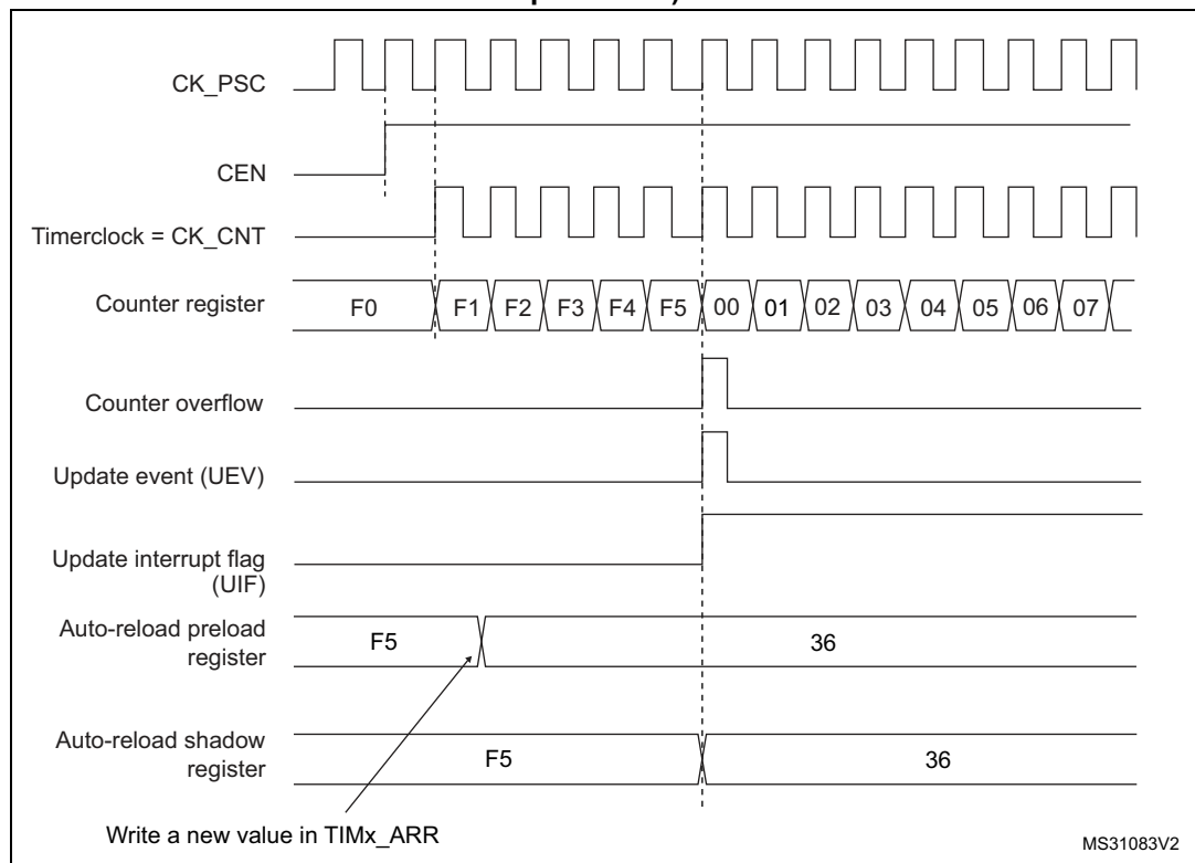
Figure 385. Counter timing diagram, Update event when ARPE=1 (TIMx_ARR preloaded)
