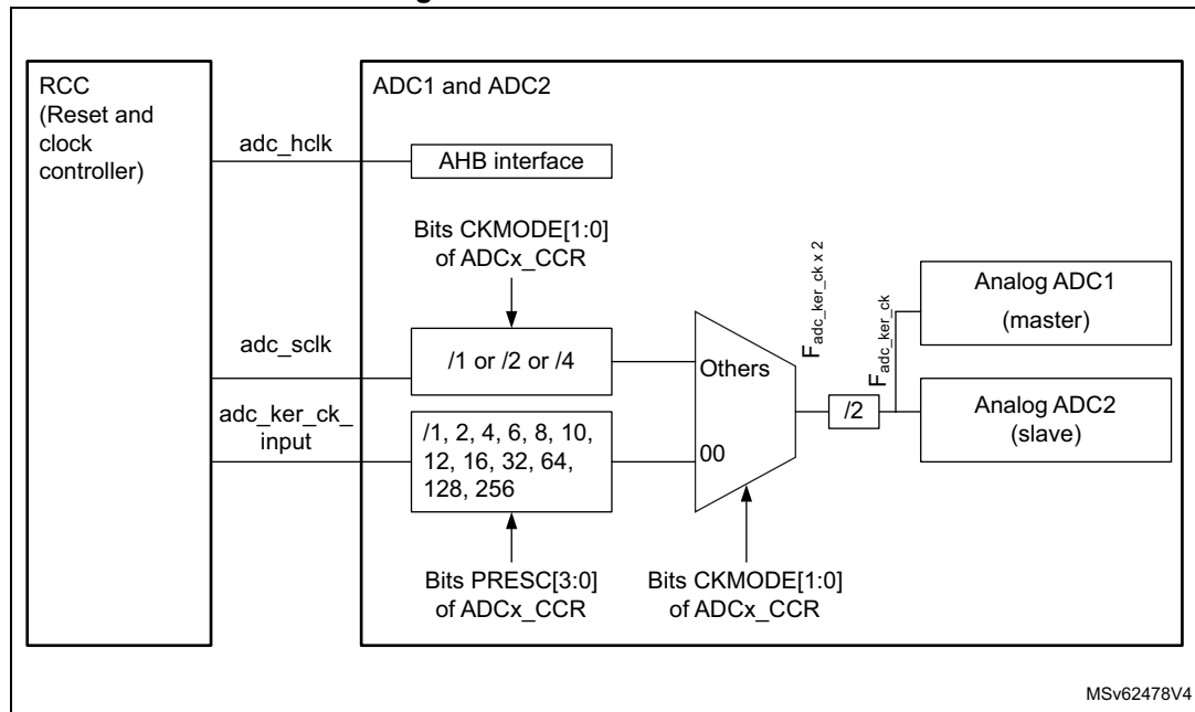
Figure 158. ADC Clock scheme
