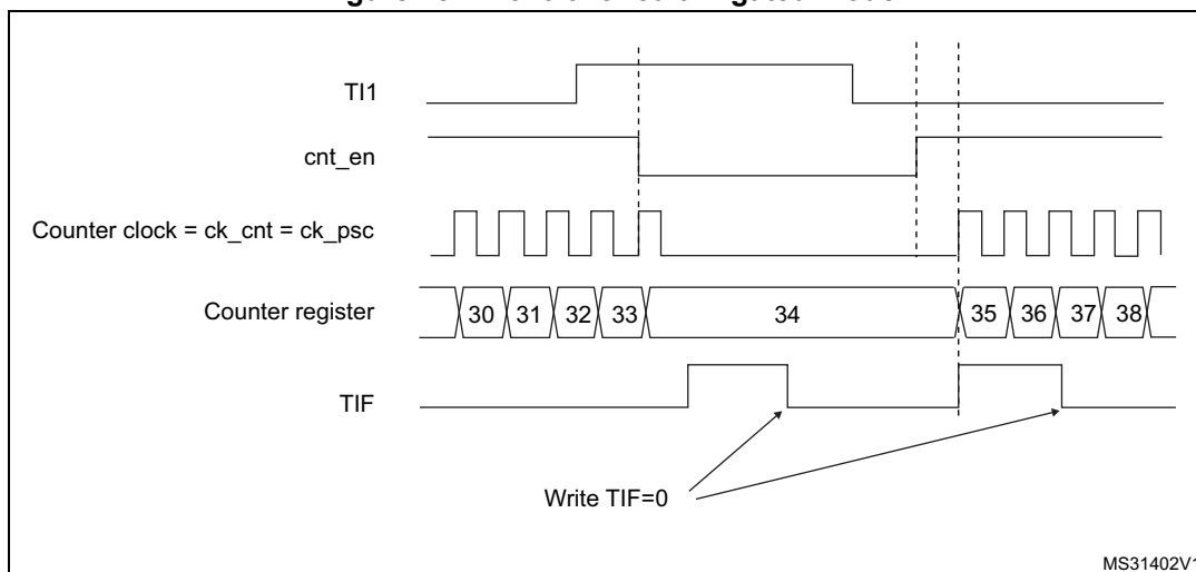
Figure 451. Control circuit in gated mode
