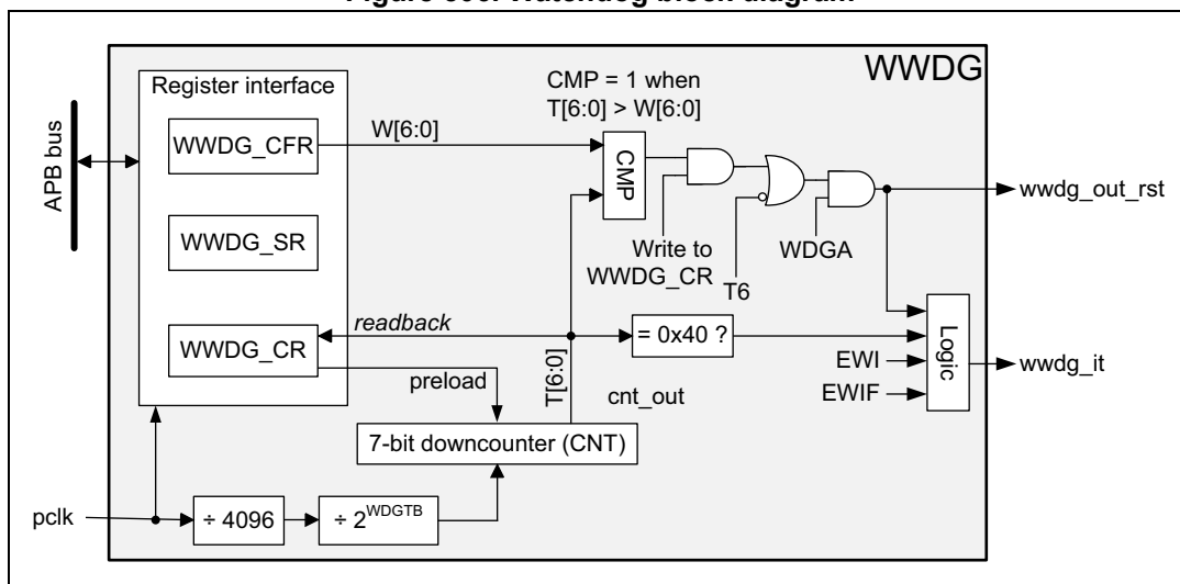
Figure 506. Watchdog block diagram
