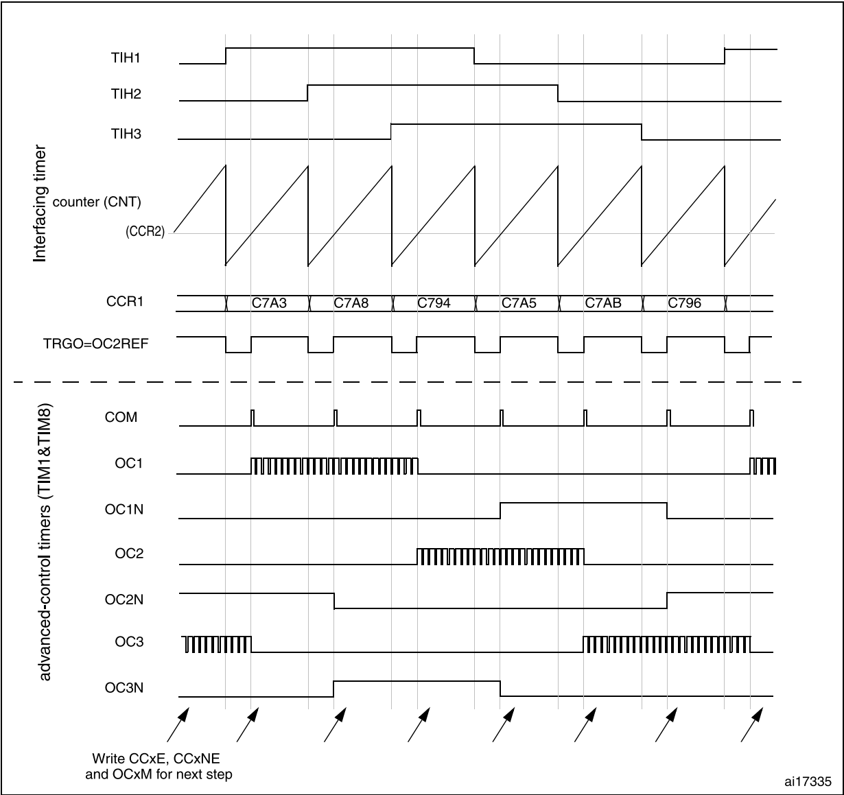
Figure 372. Example of Hall sensor interface
