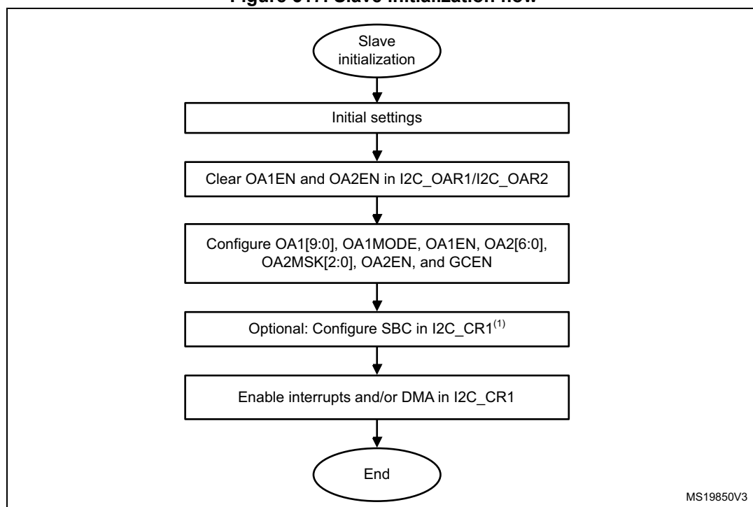
Figure 517. Slave initialization flow
