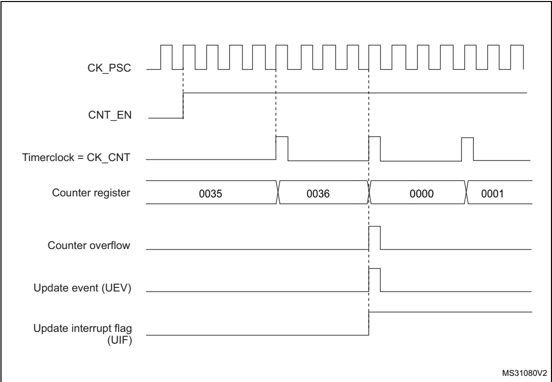
Figure 493. Counter timing diagram, internal clock divided by 4
