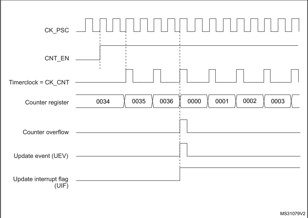
Figure 321. Counter timing diagram, internal clock divided by 2
