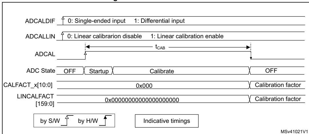
Figure 161. ADC calibration
