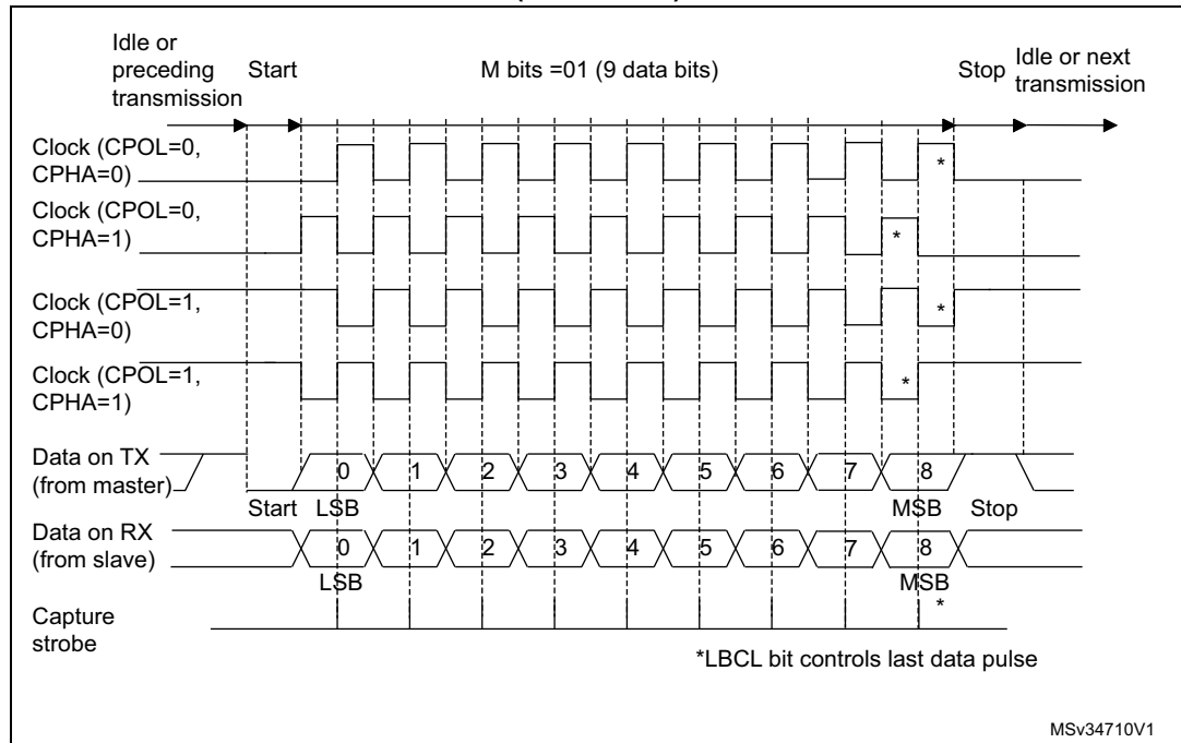
Figure 556. USART data clock timing diagram in synchronous master mode (M bits = 01)
