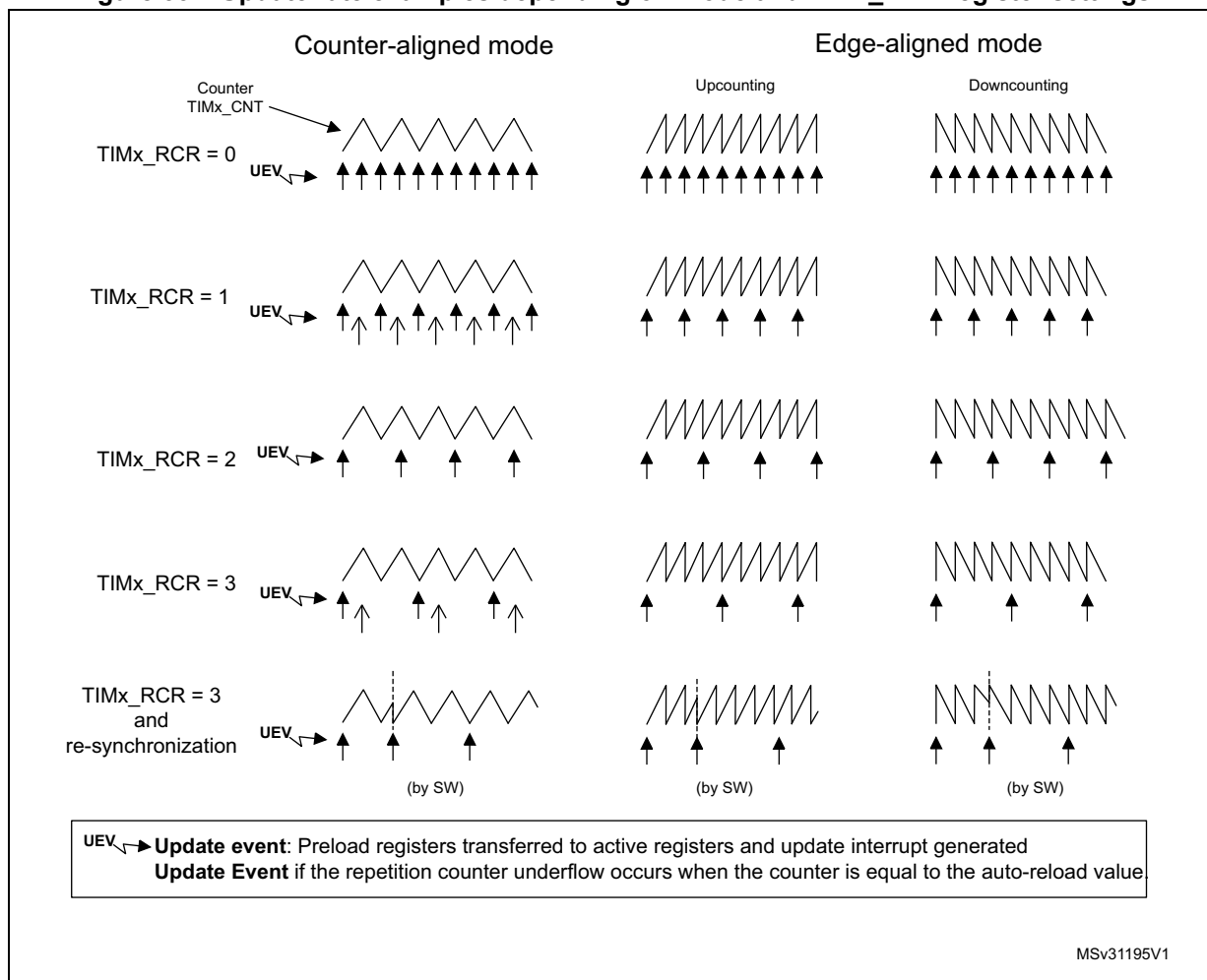
Figure 337. Update rate examples depending on mode and TIMx_RCR register settings
