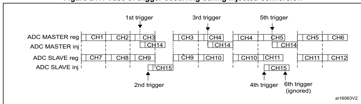
Figure 217. Case of trigger occurring during injected conversion
