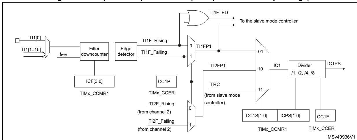
Figure 467. Capture/compare channel (example: channel 1 input stage)
