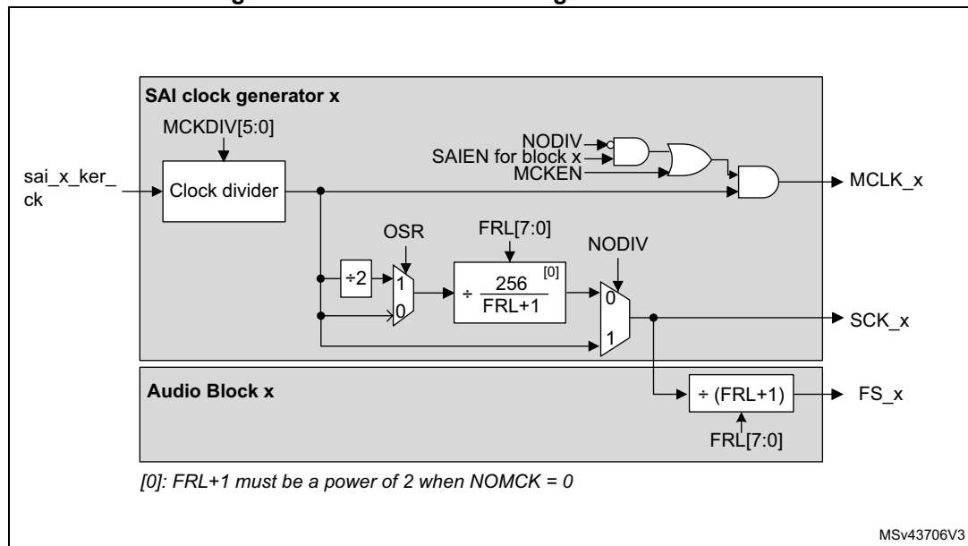
Figure 624. Audio block clock generator overview
