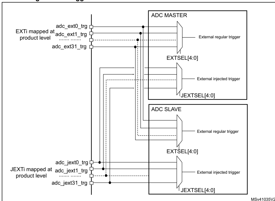
Figure 168. Triggers are shared between ADC master and ADC slave
