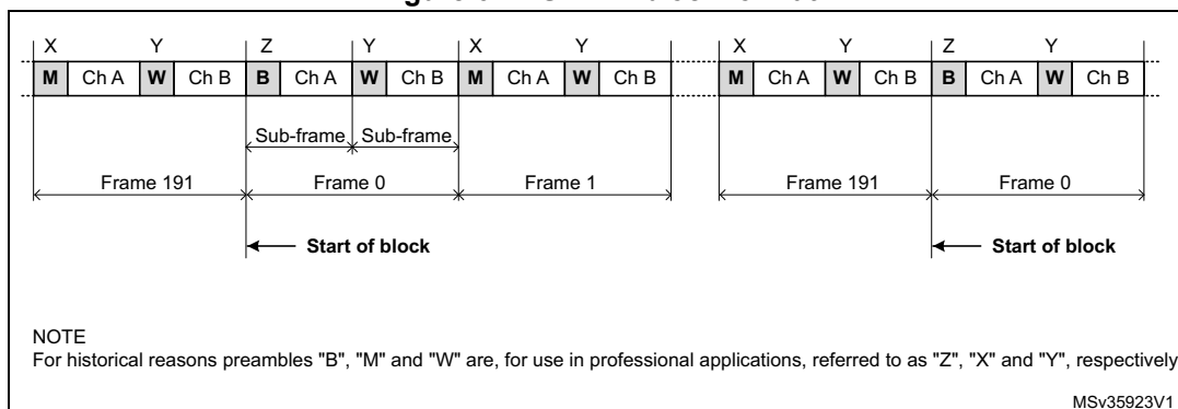
Figure 642. S/PDIF block format
