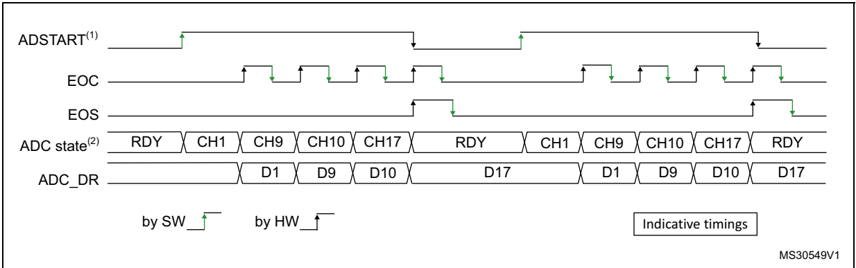
Figure 182. Single conversions of a sequence, software trigger
