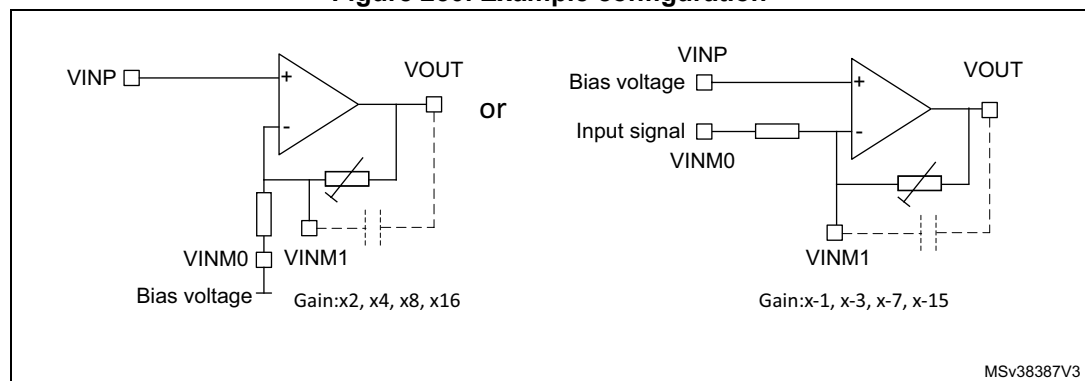
Figure 250. Example configuration
