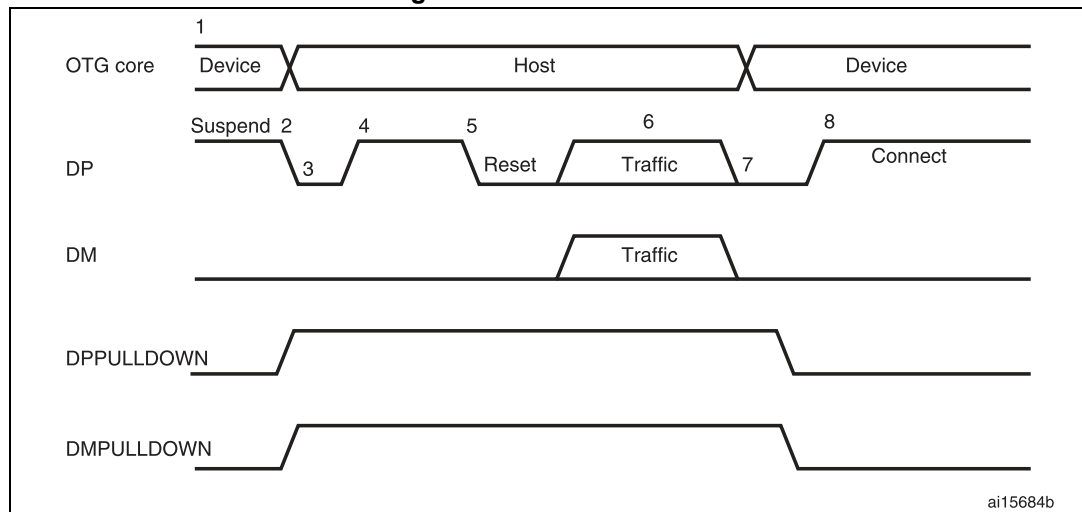
Figure 751. B-device HNP
