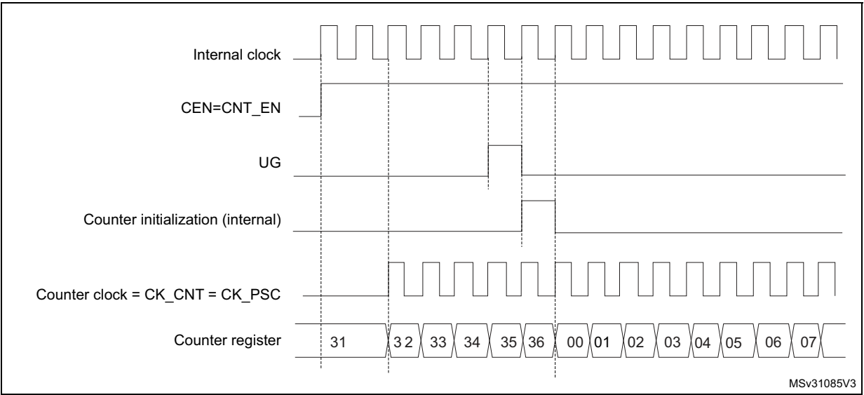
Figure 437. Control circuit in normal mode, internal clock divided by 1
