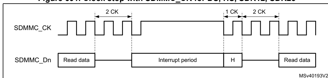
Figure 691. Clock stop with SDMMC_CK for DS, HS, SDR12, SDR25
