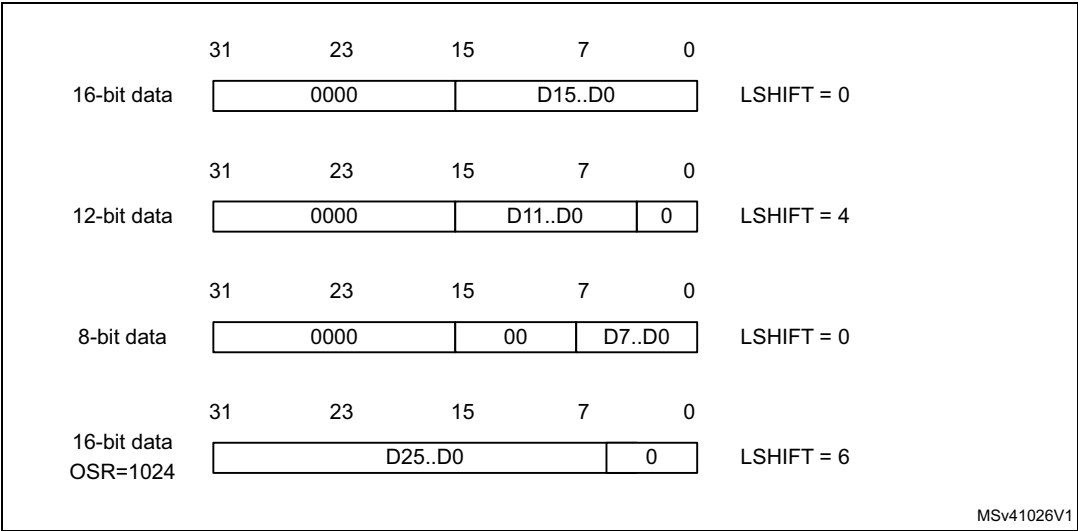
Figure 188. Left alignment (offset disabled, unsigned value)
