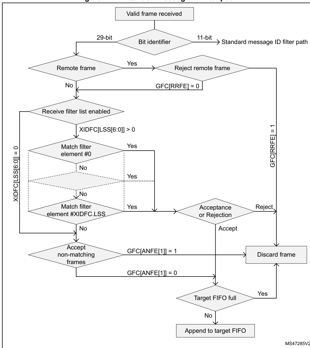
Figure 711. Extended message ID filter path
