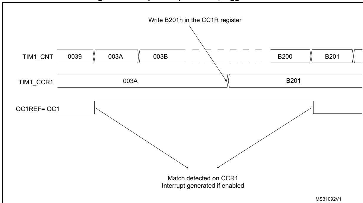
Figure 406. Output compare mode, toggle on OC1
