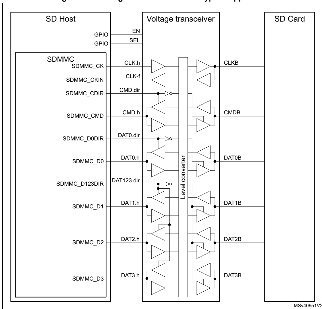
Figure 703. Voltage switch transceiver typical application
