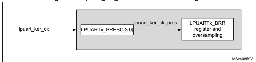
Figure 573. lpuart_ker_ck clock divider block diagram
