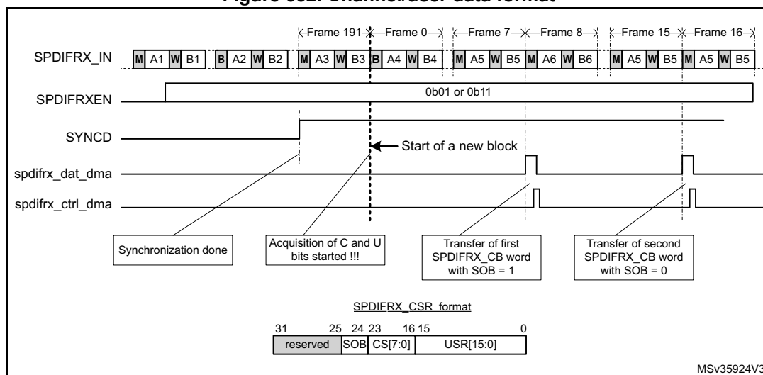
Figure 652. Channel/user data format
