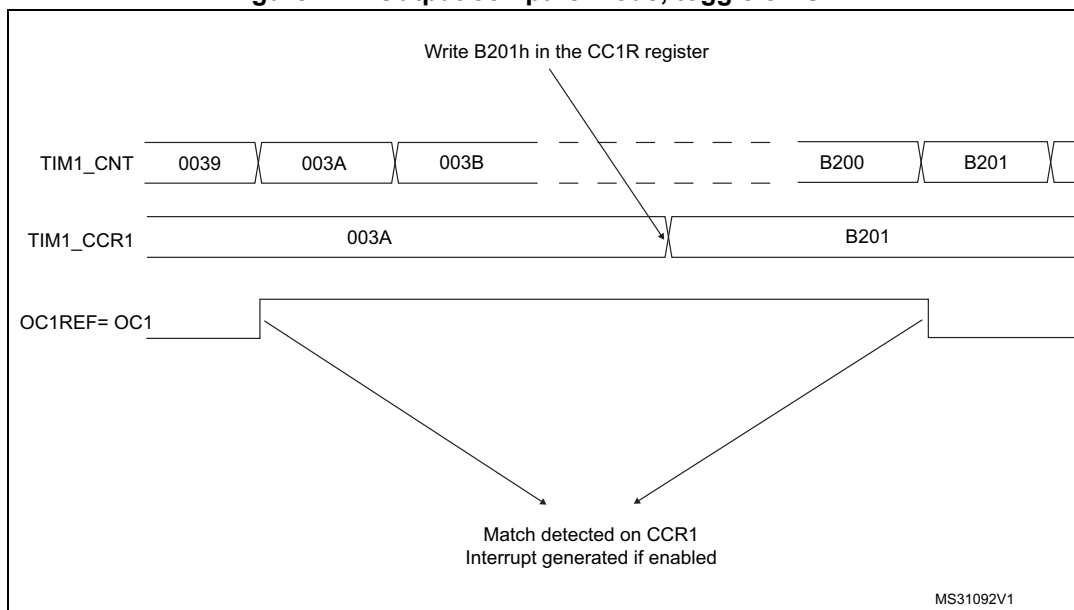
Figure 444. Output compare mode, toggle on OC1.
