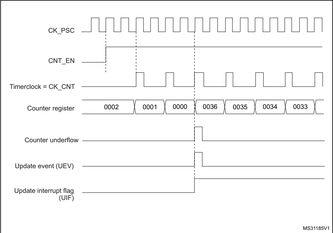
Figure 327. Counter timing diagram, internal clock divided by 2
