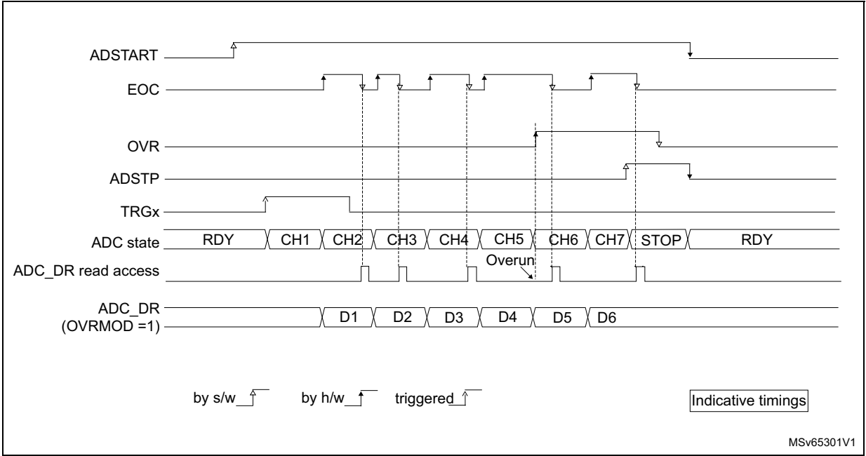
Figure 191. Example of overrun (OVRMOD = 1)
