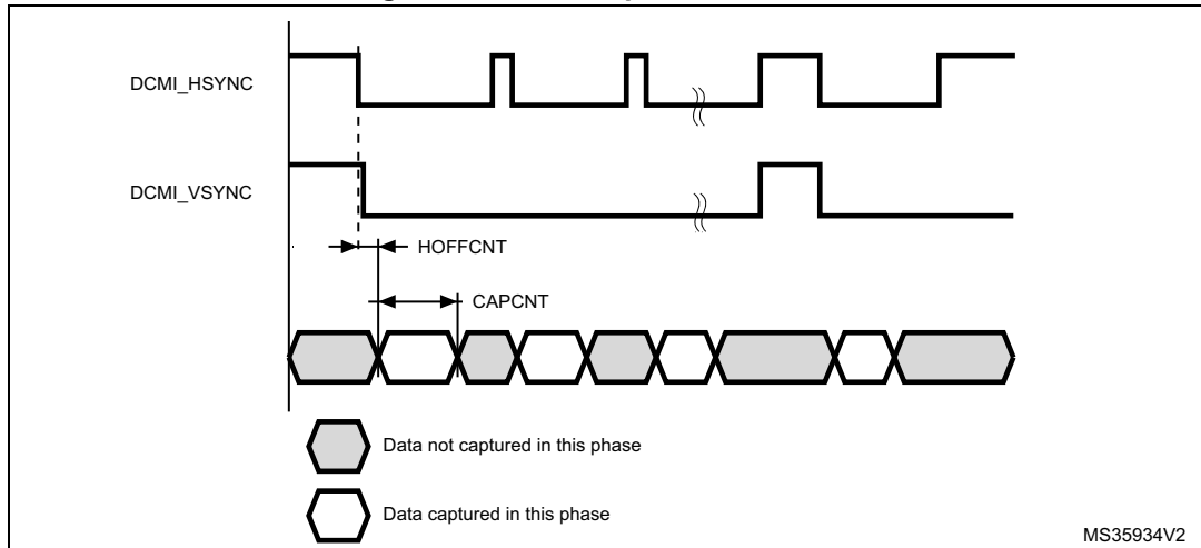
Figure 267. Data capture waveforms
