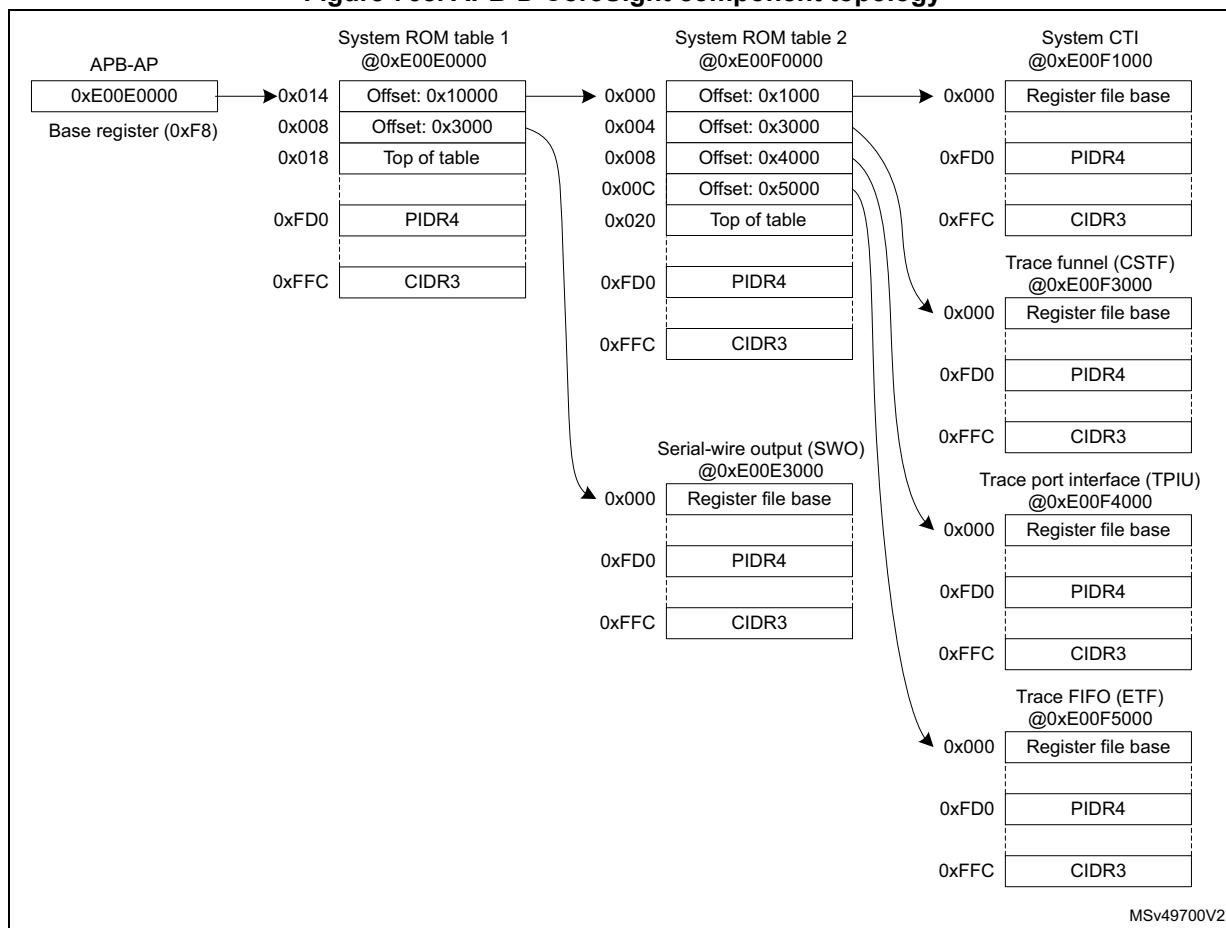
Figure 768. APB-D CoreSight component topology
