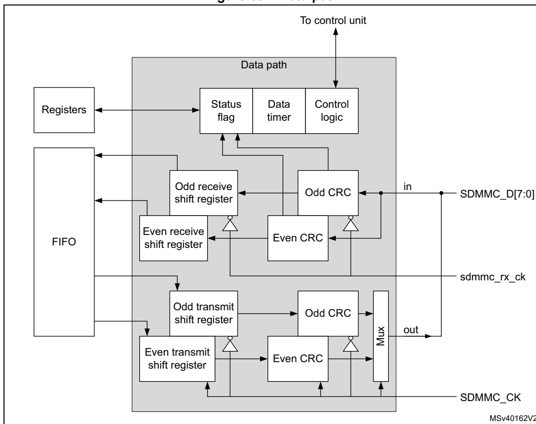
Figure 681. Data path
