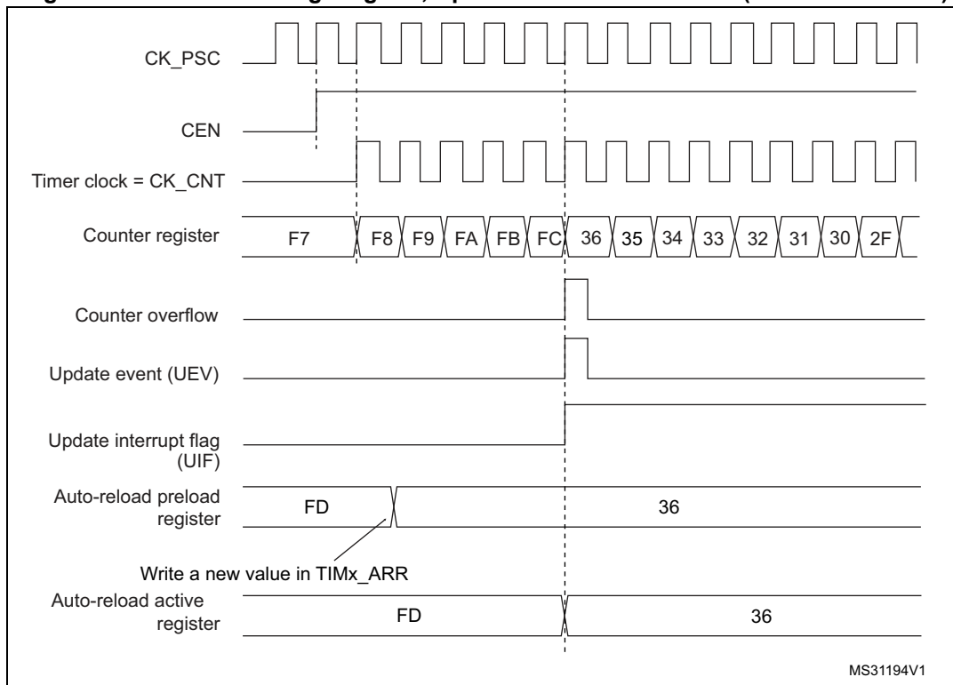
Figure 336. Counter timing diagram, Update event with ARPE=1 (counter overflow)
