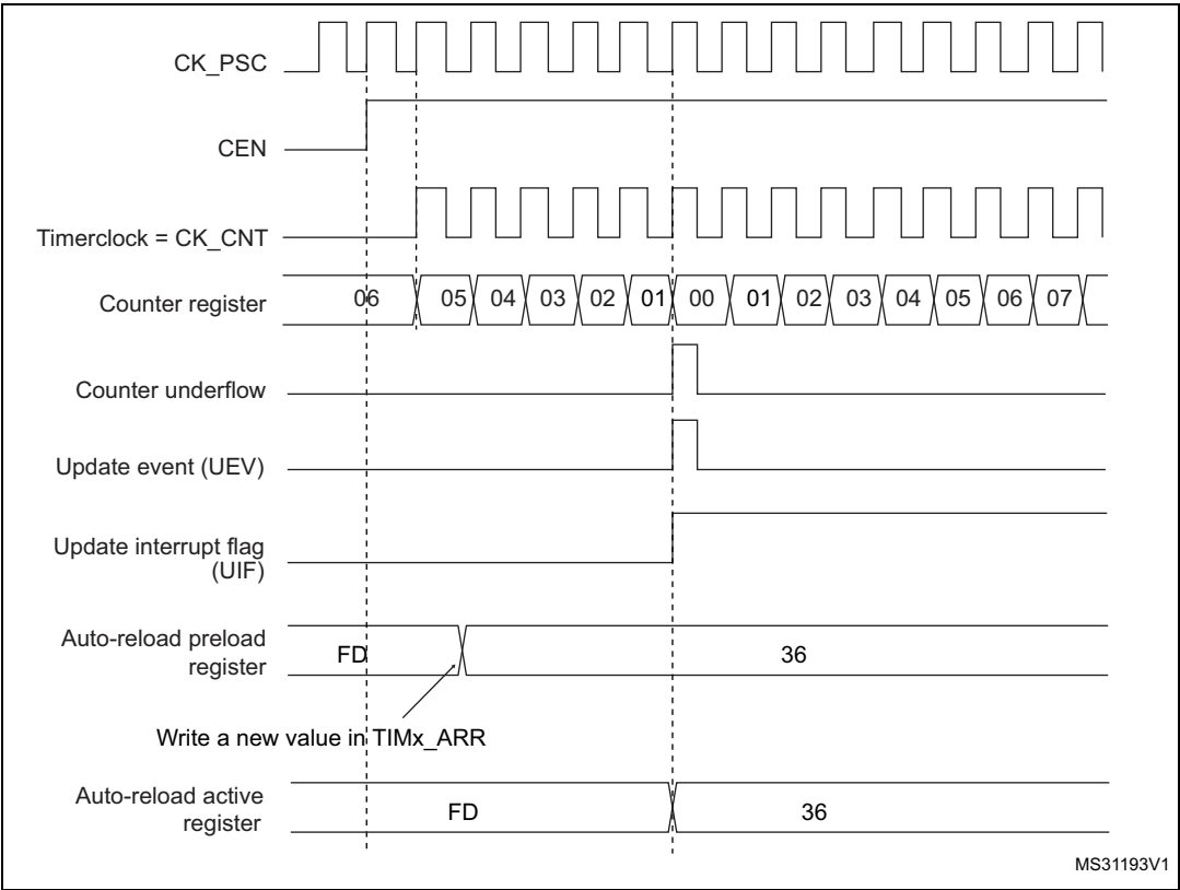
Figure 335. Counter timing diagram, update event with ARPE=1 (counter underflow)
