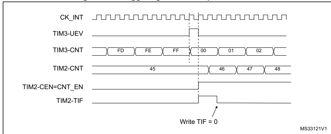
Figure 424. Triggering TIM2 with update of TIM3
