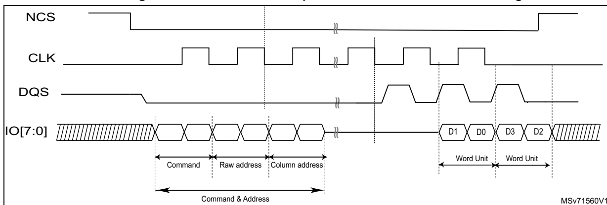
Figure 150. OctaRAM read operation with reverse data ordering D1/D0
