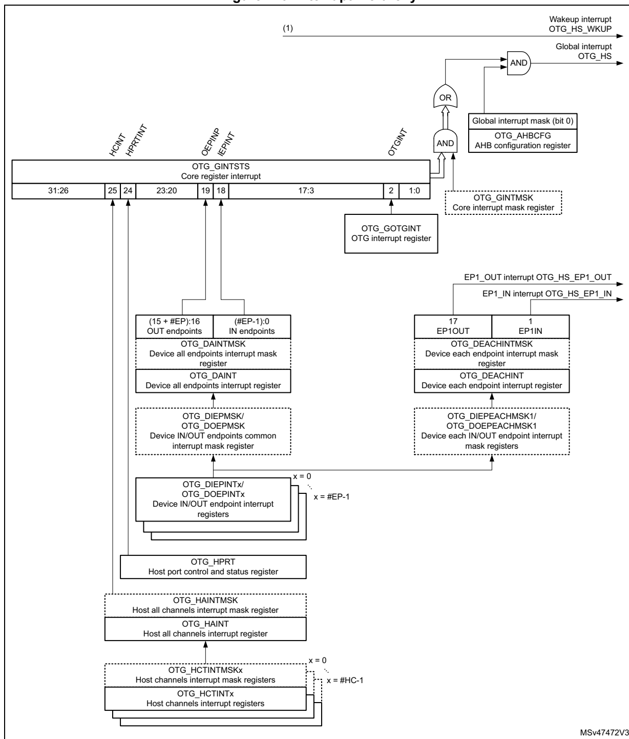
Figure 729. Interrupt hierarchy
