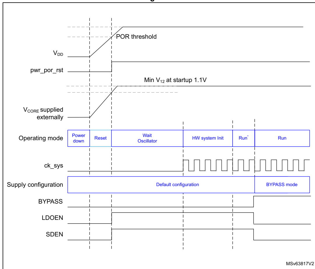
Figure 24. Device startup with V_{\text{CORE}} supplied in Bypass mode from external regulator
