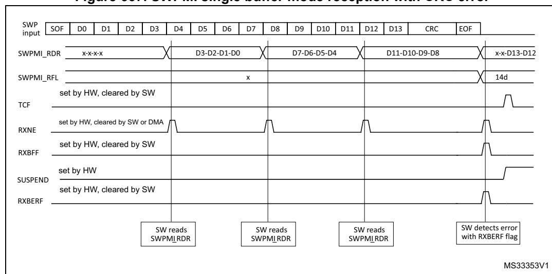
Figure 667. SWPMI single buffer mode reception with CRC error
