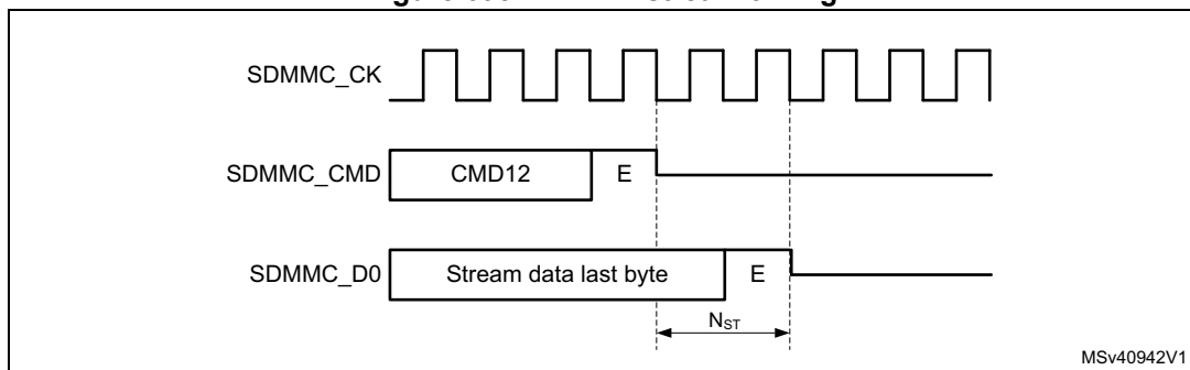
Figure 695. CMD12 stream timing
