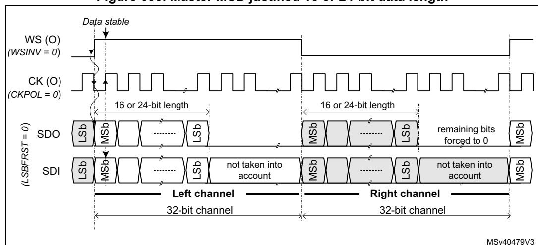
Figure 603. Master MSB justified 16 or 24-bit data length
