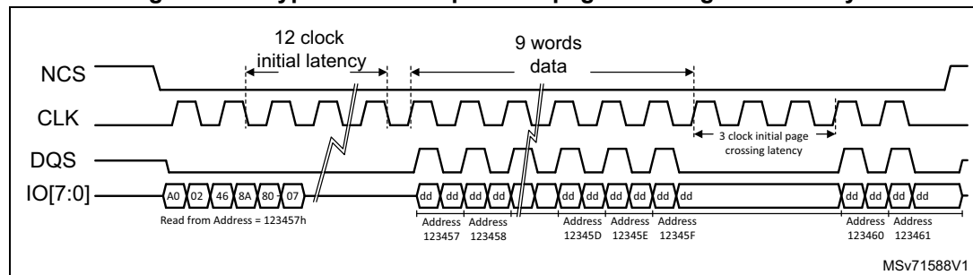
Figure 148. HyperBus read operation page crossing with latency
