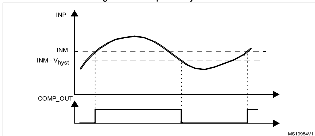
Figure 241. Comparator hysteresis
