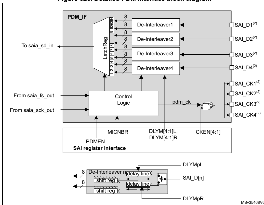
Figure 626. Detailed PDM interface block diagram
