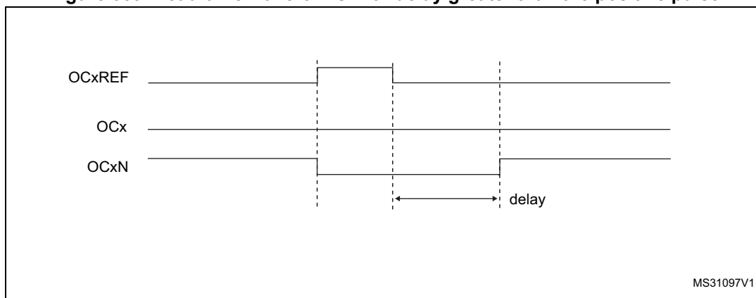
Figure 359. Dead-time waveforms with delay greater than the positive pulse
