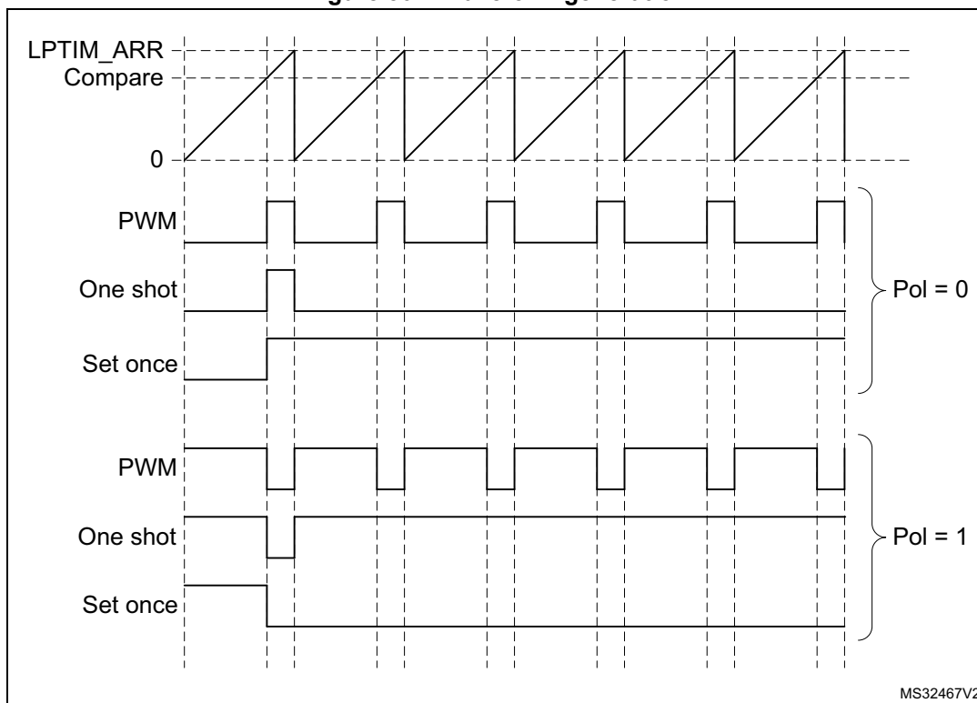
Figure 504. Waveform generation
