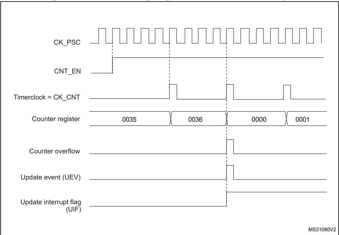
Figure 382. Counter timing diagram, internal clock divided by 4
