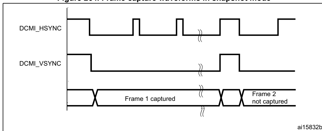
Figure 264. Frame capture waveforms in snapshot mode
