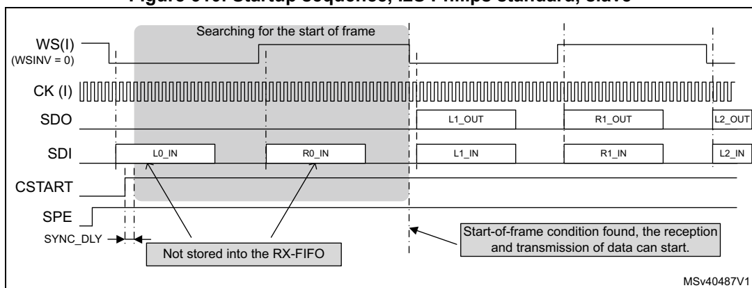
Figure 610. Startup sequence, I2S Philips standard, slave
