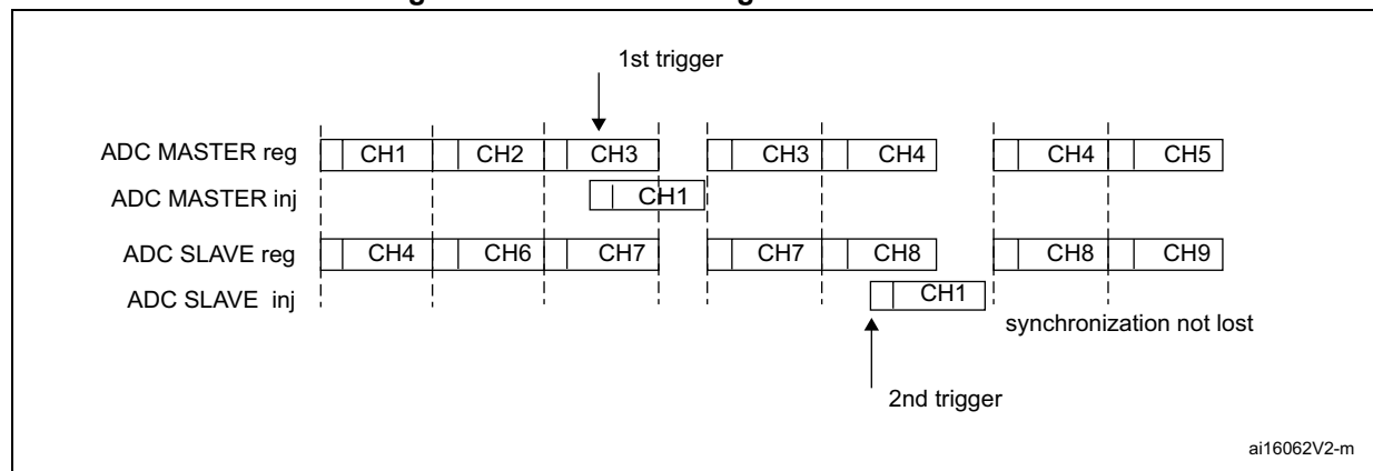
Figure 216. Alternate + regular simultaneous
