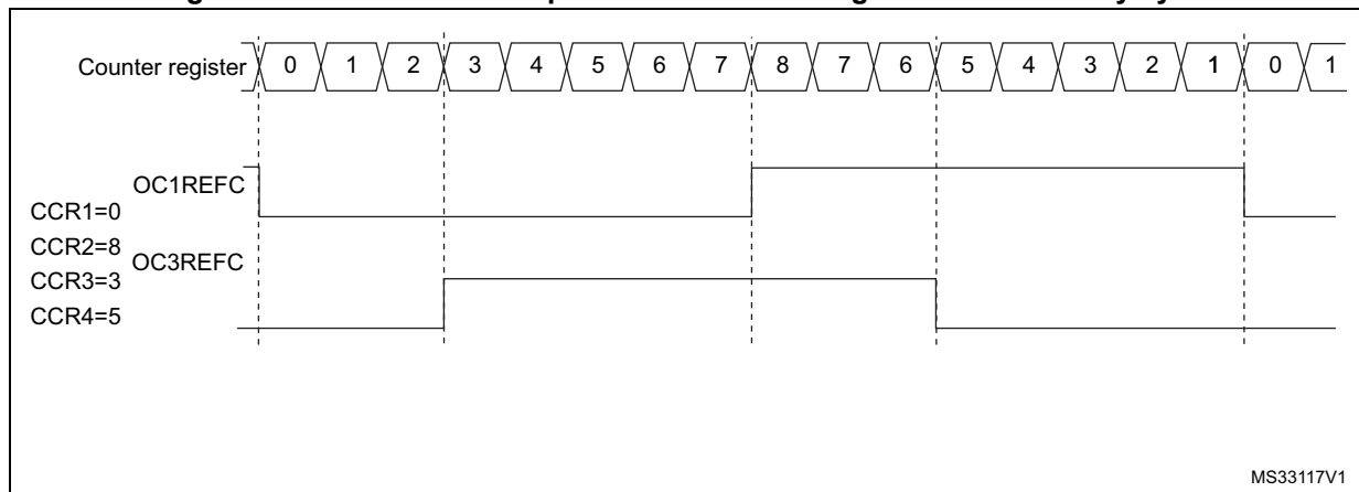
Figure 354. Generation of 2 phase-shifted PWM signals with 50% duty cycle
