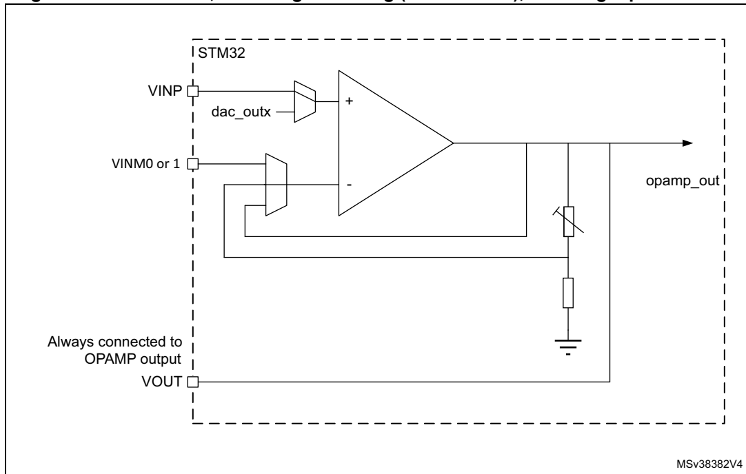
Figure 247. PGA mode, internal gain setting (x2/x4/x8/x16), inverting input not used
