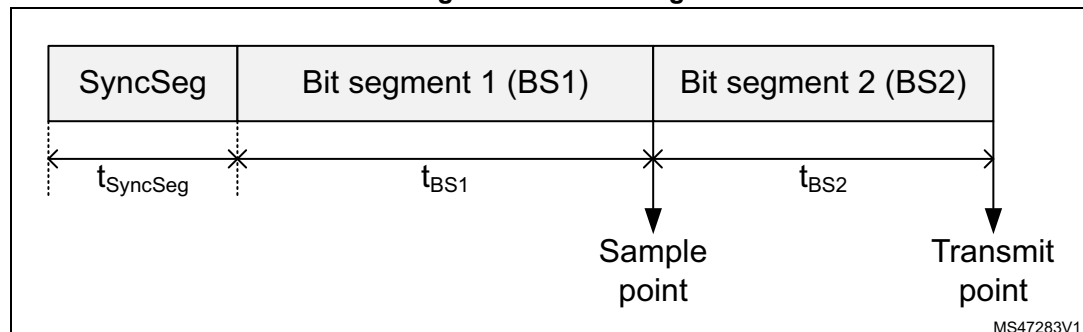
Figure 714. Bit timing
