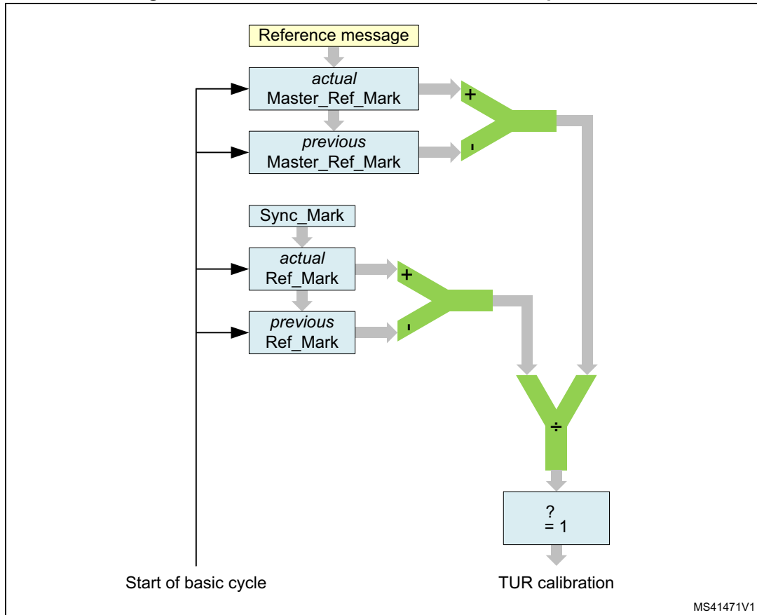
Figure 718. TTCAN level 0 and level 2 drift compensation
