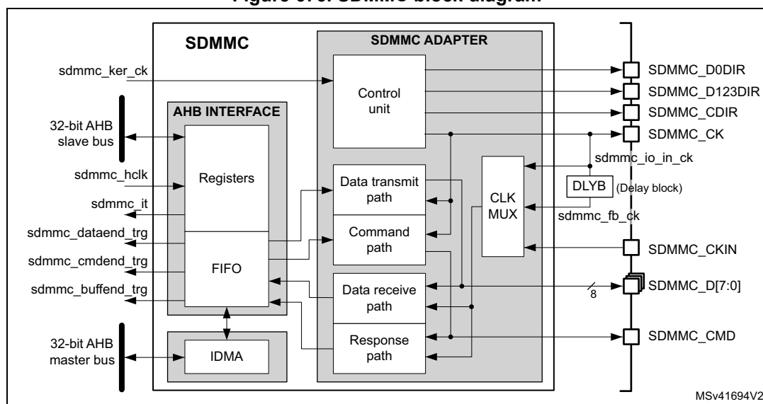
Figure 676. SDMMC block diagram
