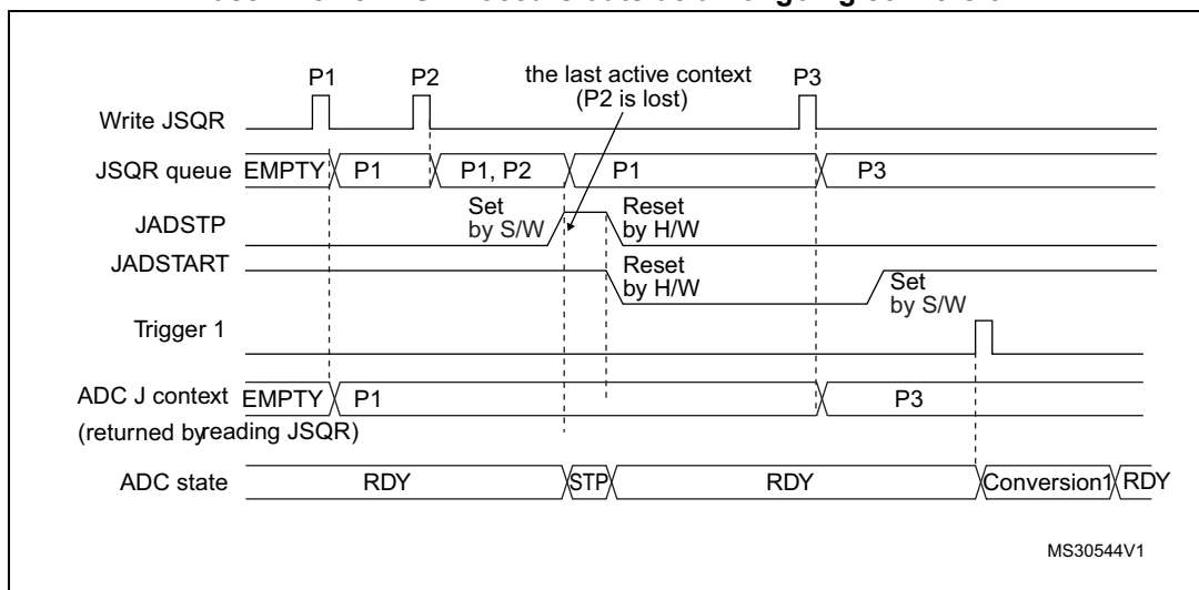
Figure 178. Flushing JSQR queue of context by setting JADSTP=1 (JQM=0). Case when JADSTP occurs outside an ongoing conversion
