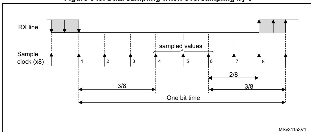
Figure 549. Data sampling when oversampling by 8
