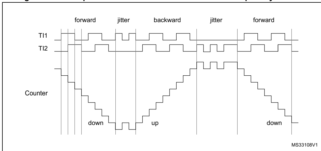
Figure 370. Example of encoder interface mode with TI1FP1 polarity inverted.
