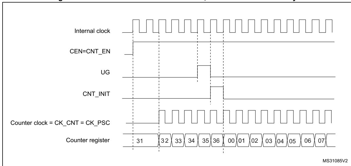
Figure 397. Control circuit in normal mode, internal clock divided by 1
