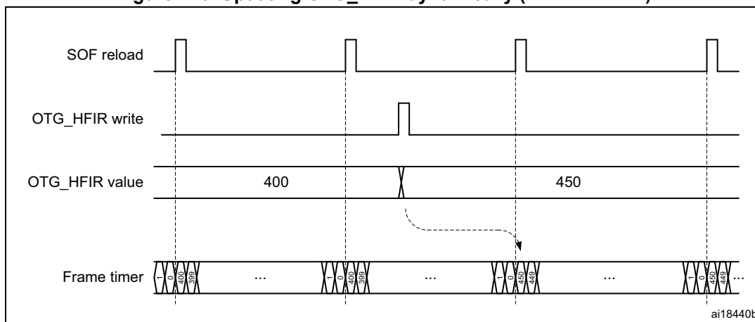
Figure 726. Updating OTG_HFIR dynamically (RLDCTRL = 1)
