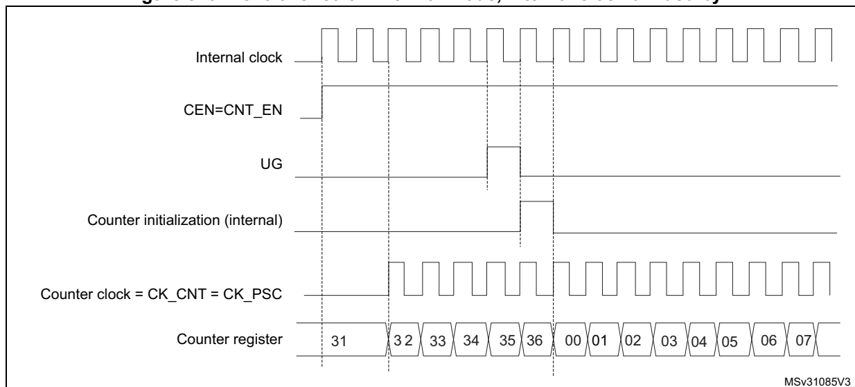
Figure 340. Control circuit in normal mode, internal clock divided by 1
