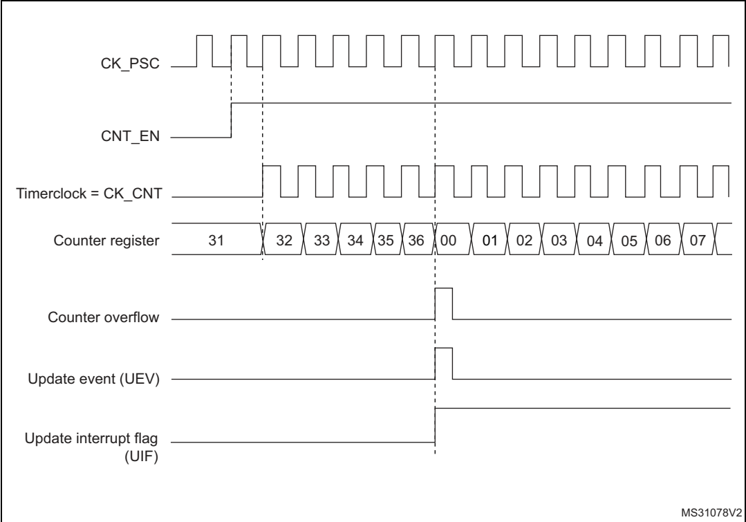
Figure 320. Counter timing diagram, internal clock divided by 1
