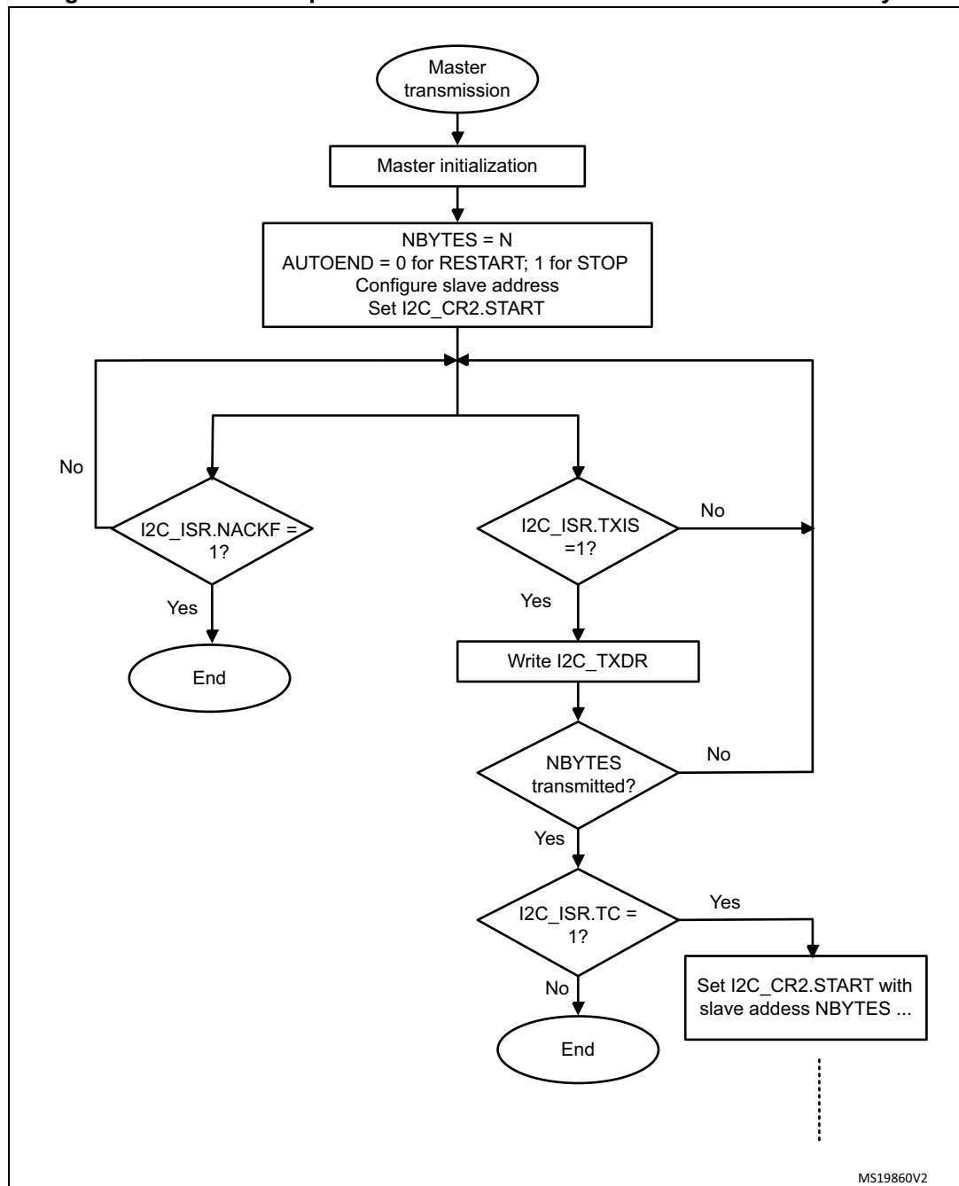
Figure 528. Transfer sequence flow for I2C master transmitter for N \leq 255 bytes
