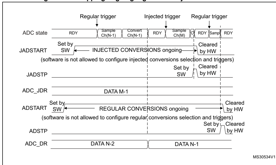
Figure 167. Stopping ongoing regular and injected conversions
