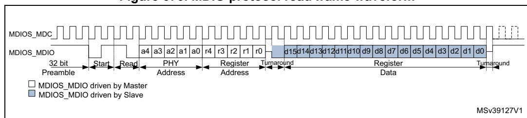
Figure 670. MDIO protocol read frame waveform
