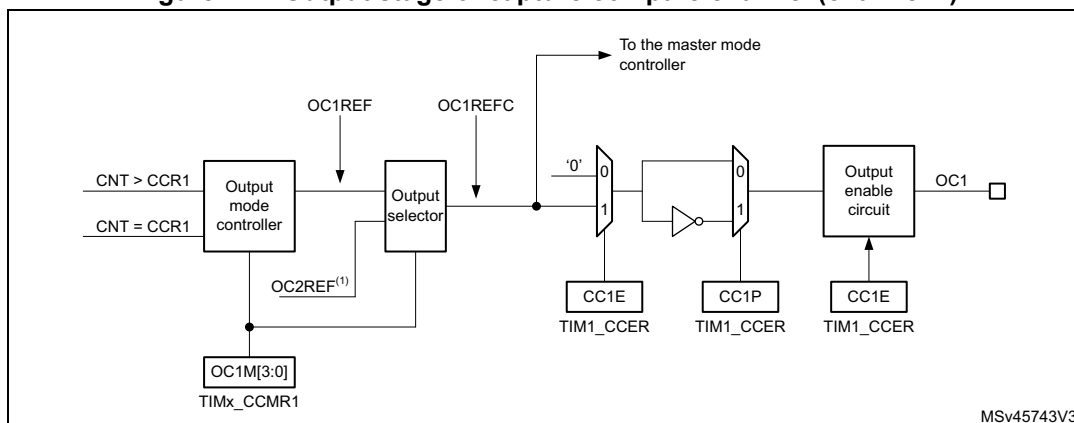
Figure 442. Output stage of capture/compare channel (channel 1)
