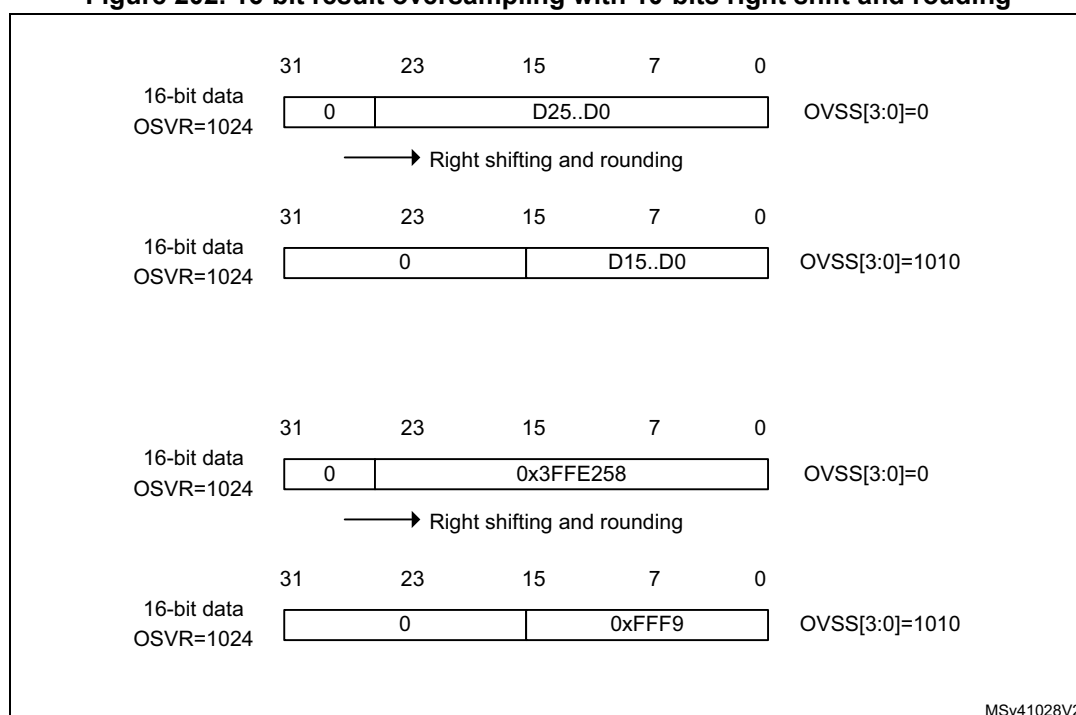
Figure 202. 16-bit result oversampling with 10-bits right shift and rounding
