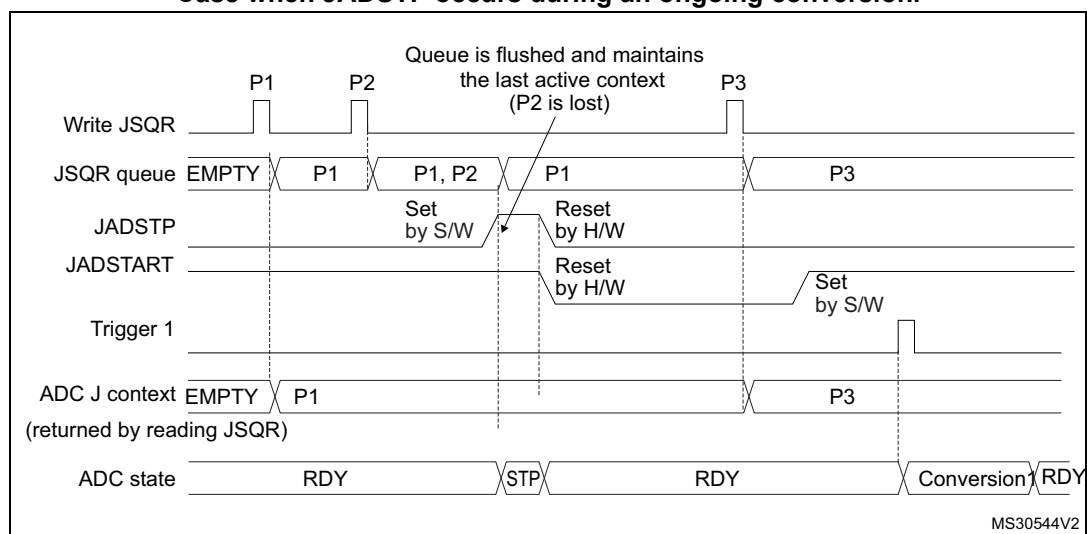
Figure 176. Flushing JSQR queue of context by setting JADSTP=1 (JQM=0). Case when JADSTP occurs during an ongoing conversion.
