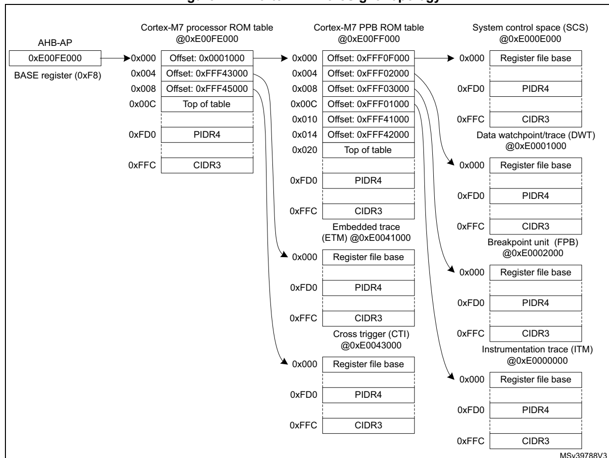
Figure 772. Cortex-M7 CoreSight Topology
