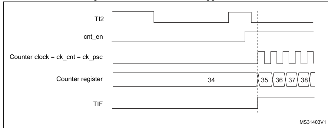
Figure 418. Control circuit in trigger mode
