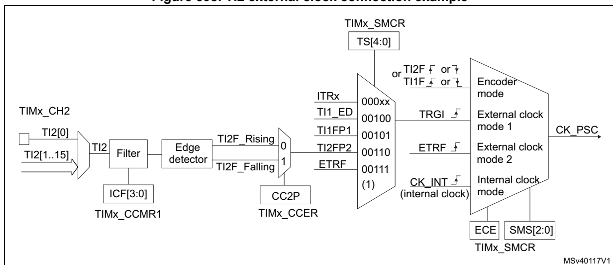
Figure 398. T12 external clock connection example
