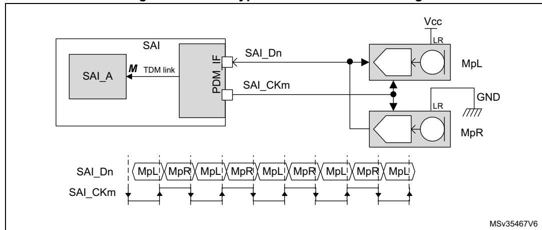
Figure 625. PDM typical connection and timing
