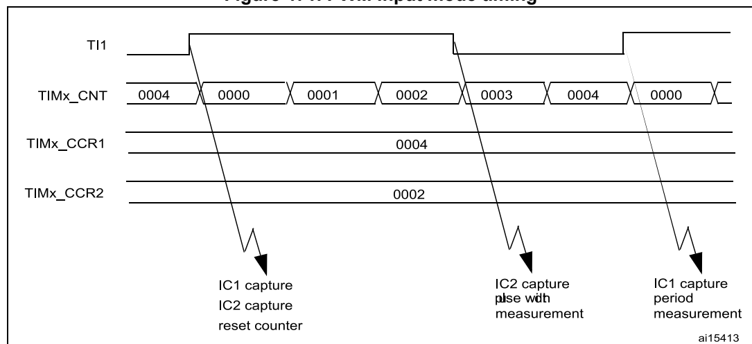
Figure 471. PWM input mode timing
