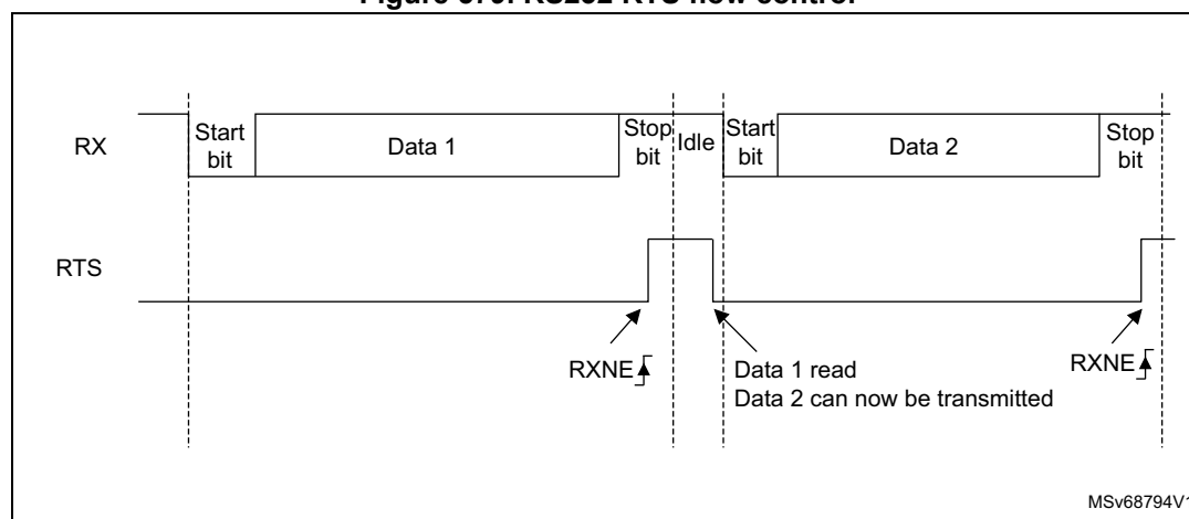
Figure 579. RS232 RTS flow control
