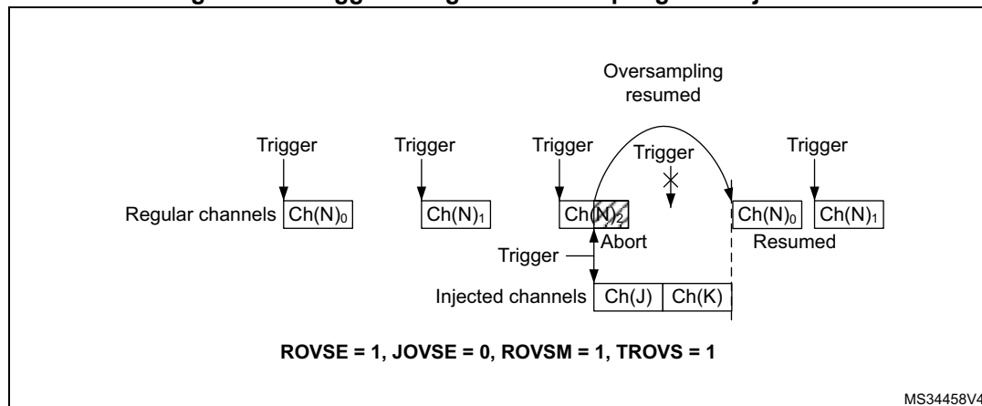
Figure 206. Triggered regular oversampling with injection
