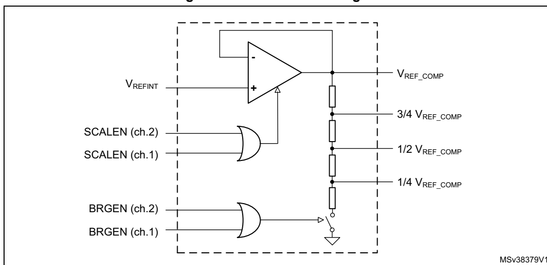
Figure 244. Scaler block diagram
