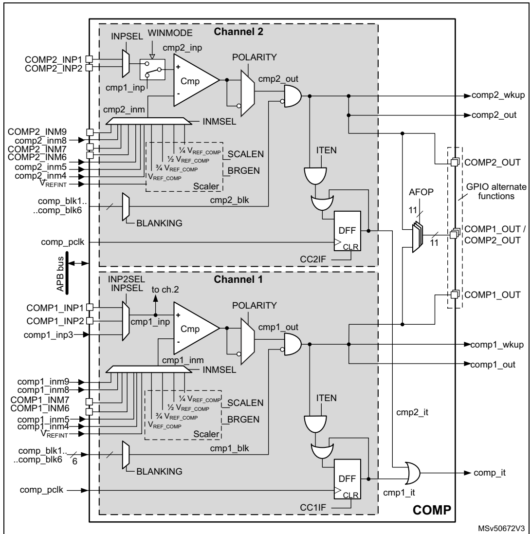
Figure 240. Comparator block diagram
