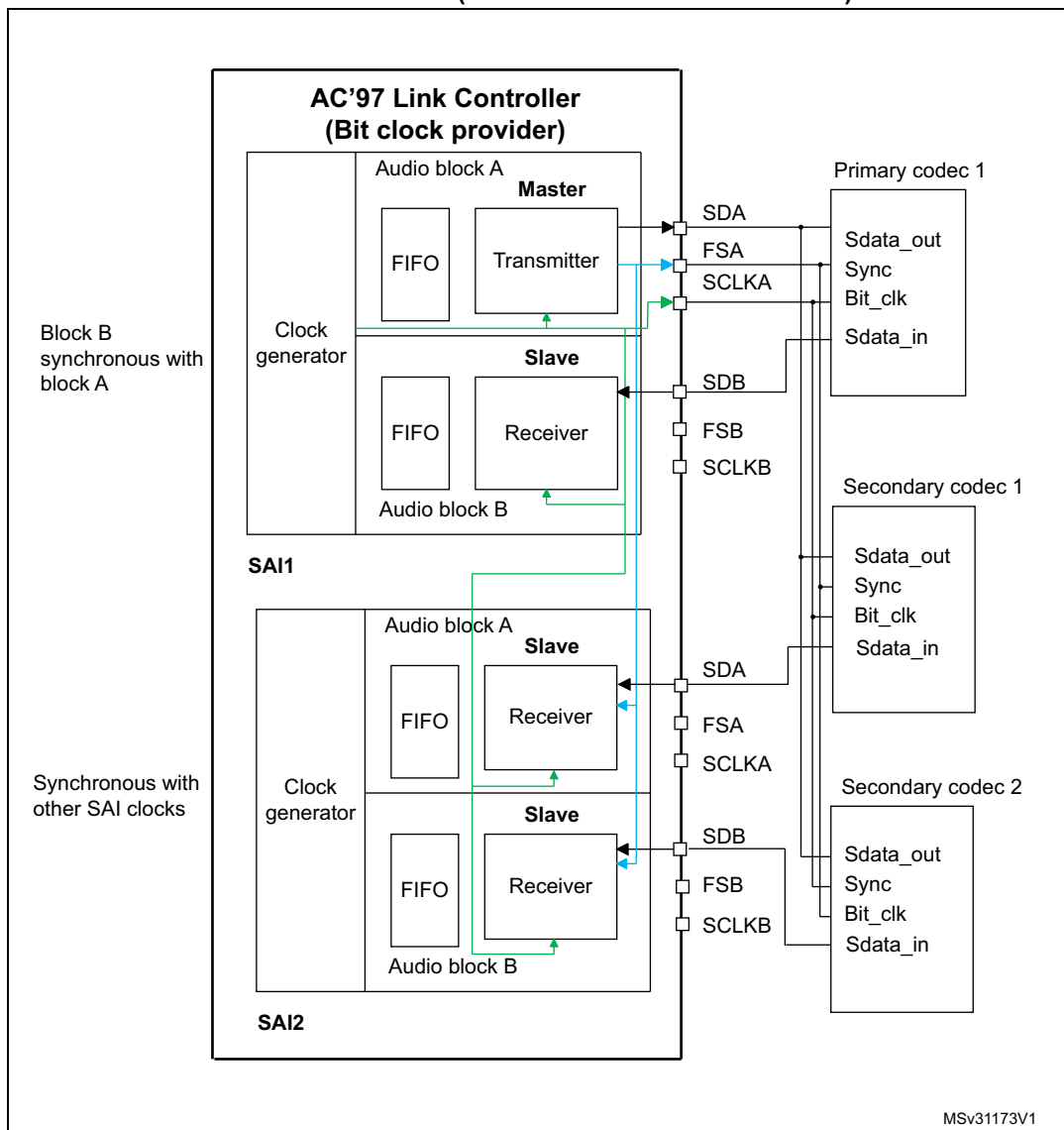
Figure 632. Example of typical AC'97 configuration on devices featuring at least 2 embedded SAIs (three external AC'97 decoders)
