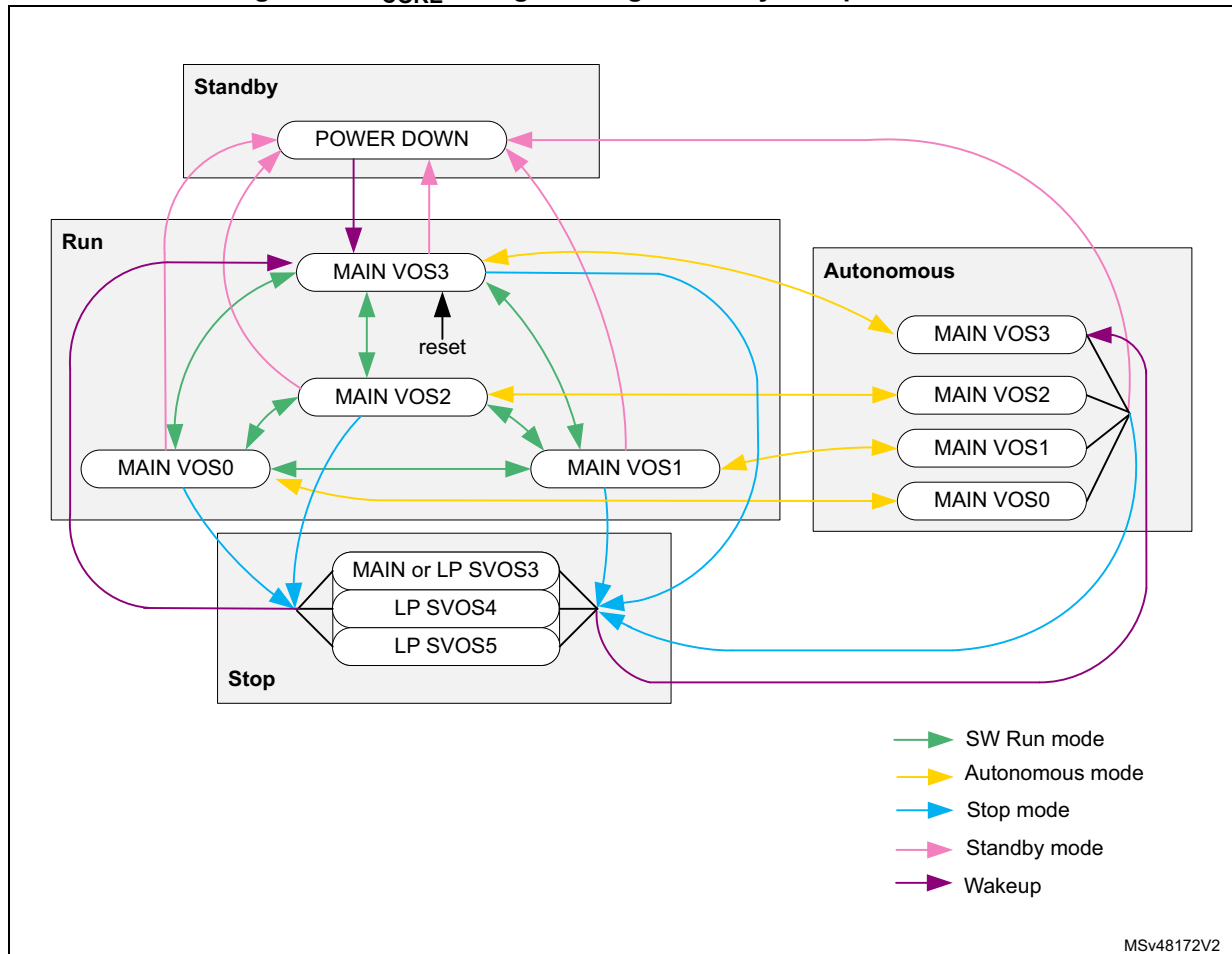
Figure 34. V_{CORE} voltage scaling versus system power modes
