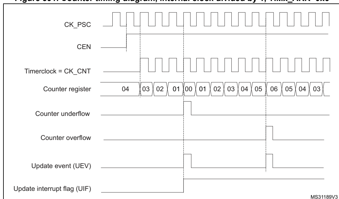
Figure 391. Counter timing diagram, internal clock divided by 1, TIMx_ARR=0x6
