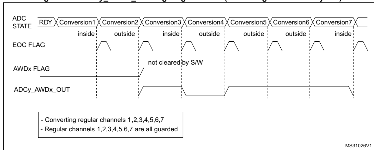
Figure 199. ADCy_AWDx_OUT signal generation (AWDx flag not cleared by SW)
