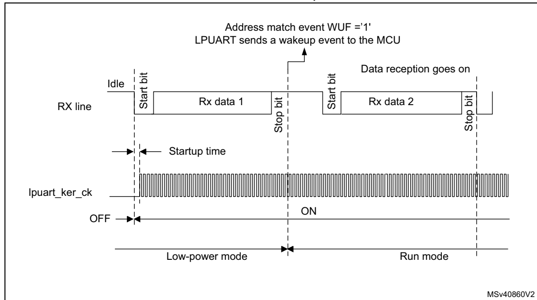
Figure 581. Wake-up event verified (wake-up event = address match, FIFO disabled)
