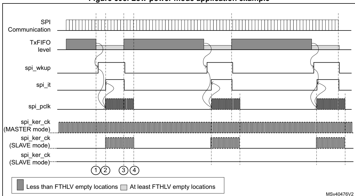
Figure 598. Low-power mode application example
