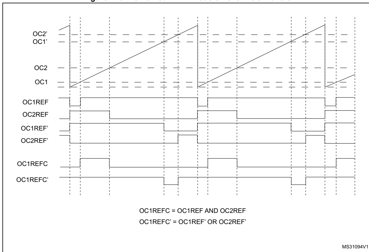
Figure 410. Combined PWM mode on channels 1 and 3
