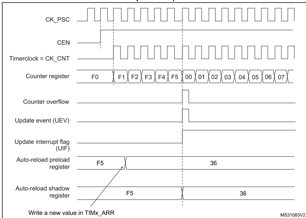
Figure 436. Counter timing diagram, update event when ARPE=1 (TIMx_ARR preloaded)
