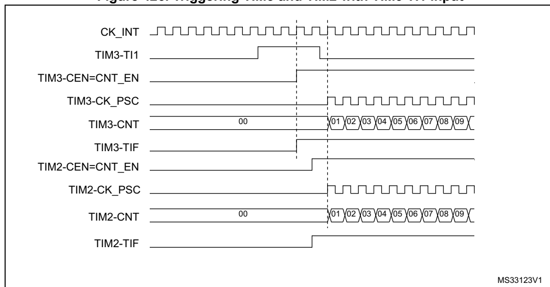
Figure 426. Triggering TIM3 and TIM2 with TIM3 TI1 input
