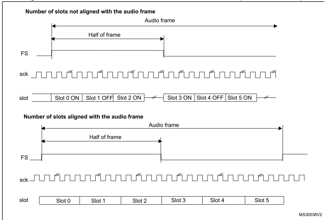
Figure 620. FS role is start of frame + channel side identification (FSDEF = TRIS = 1)
