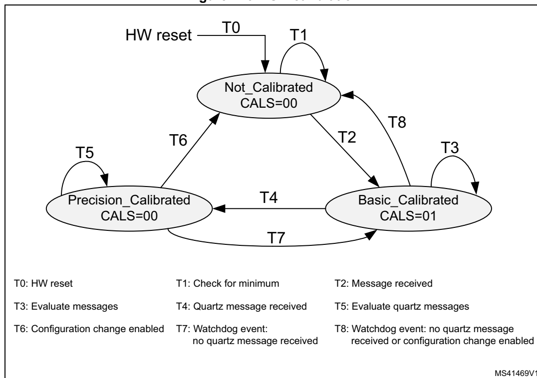
Figure 716. FSM calibration
