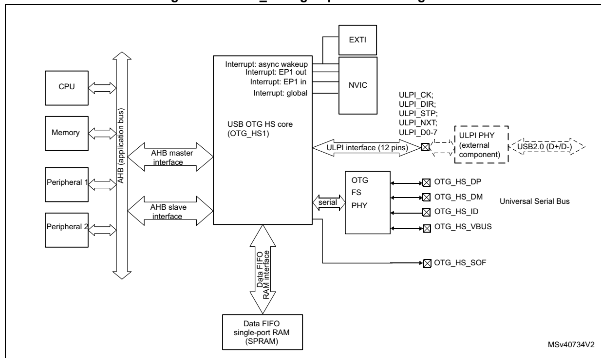
Figure 721. OTG_HS high-speed block diagram
