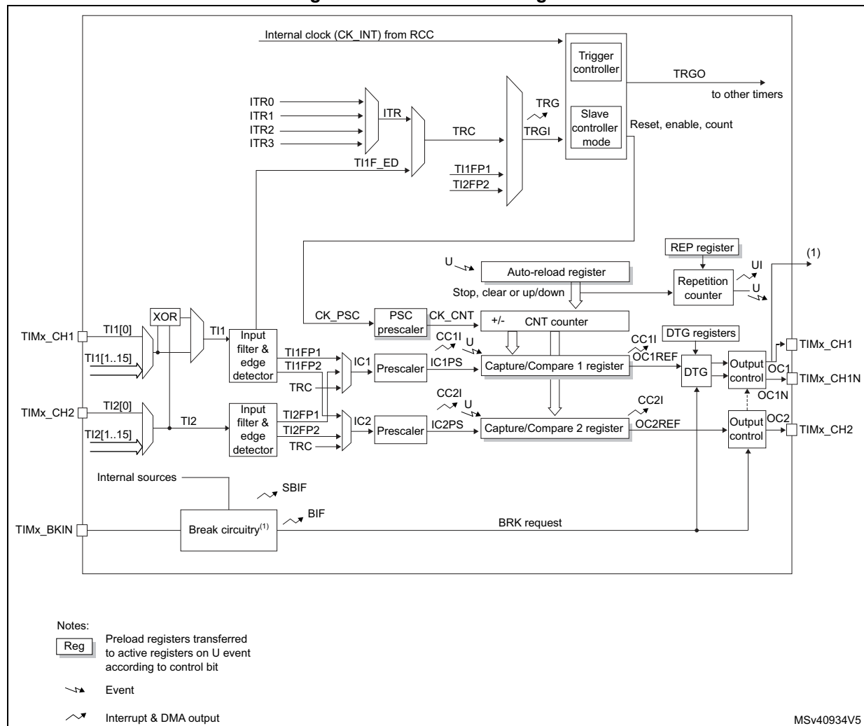
Figure 453. TIM15 block diagram
