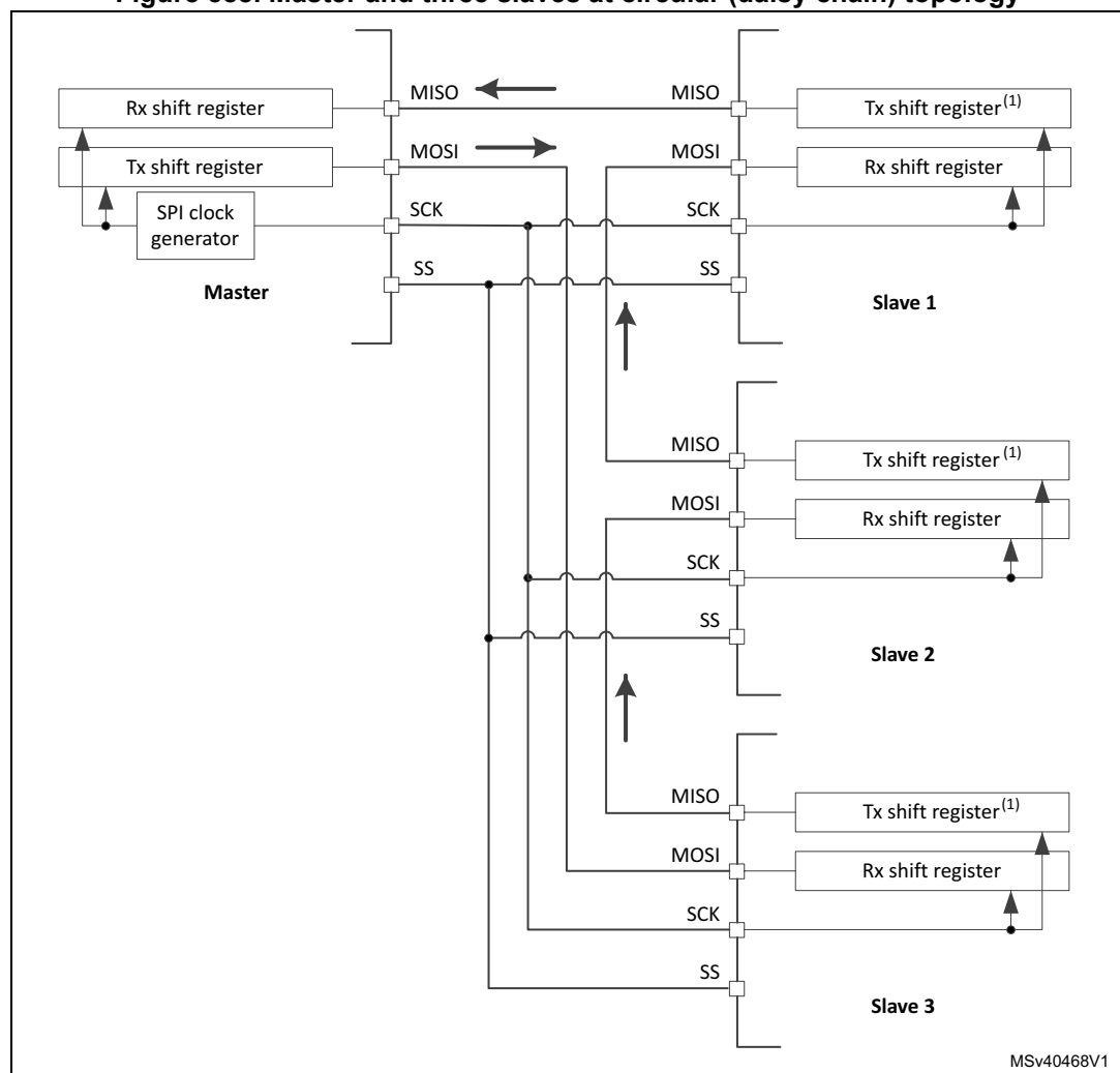
Figure 588. Master and three slaves at circular (daisy chain) topology
