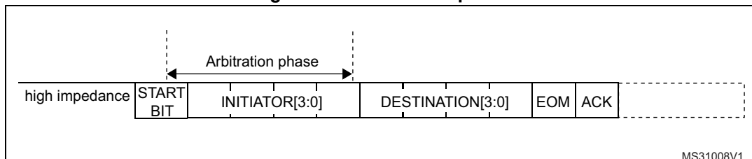
Figure 757. Arbitration phase
