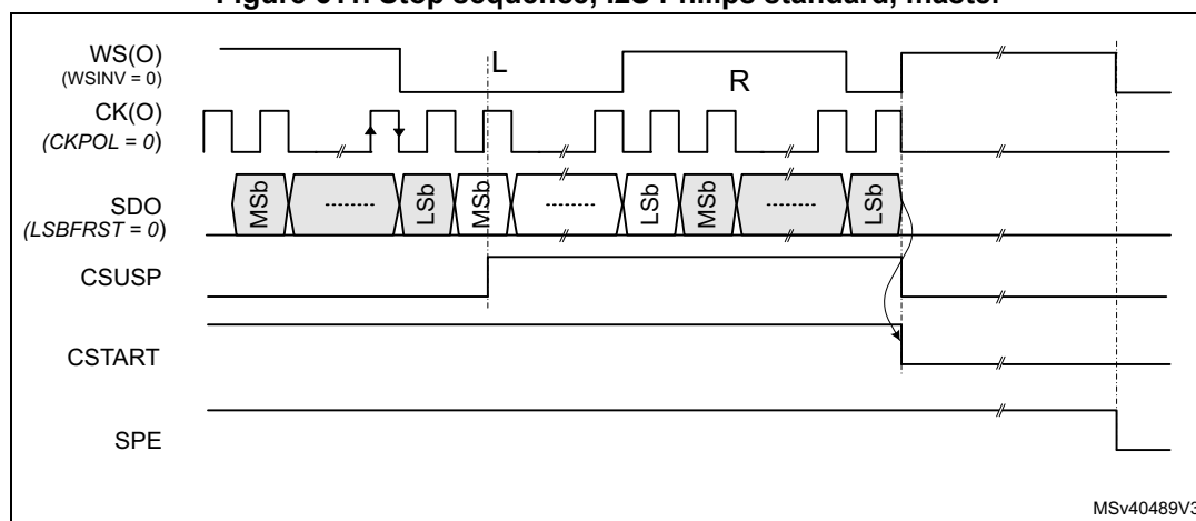
Figure 611. Stop sequence, I2S Philips standard, master
