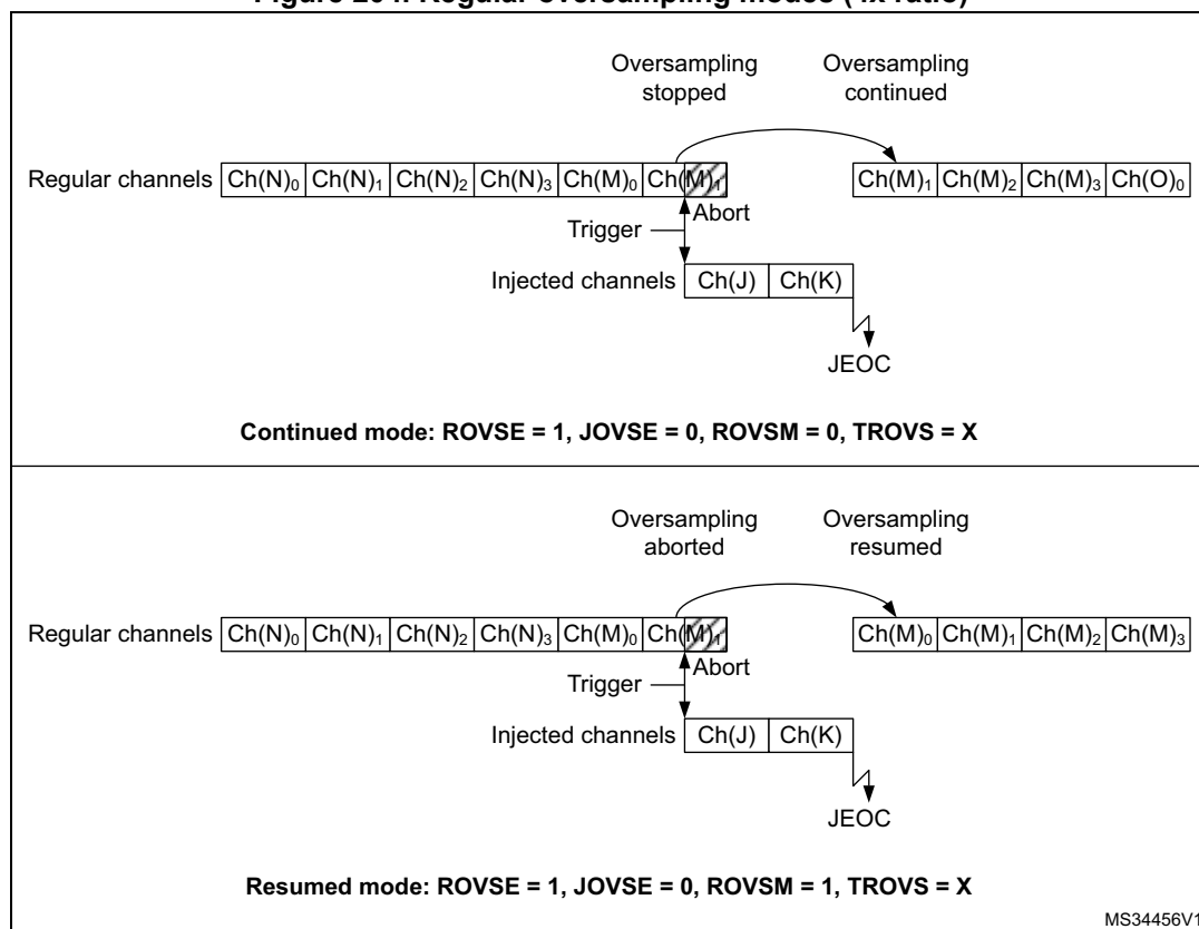
Figure 204. Regular oversampling modes (4x ratio)
