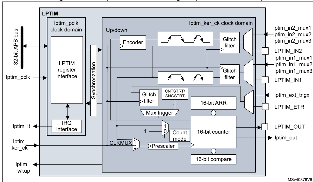
Figure 498. Low-power timer block diagram (LPTIM1 and LPTIM2)
