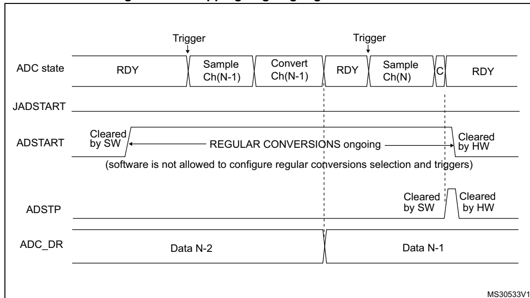
Figure 166. Stopping ongoing regular conversions
