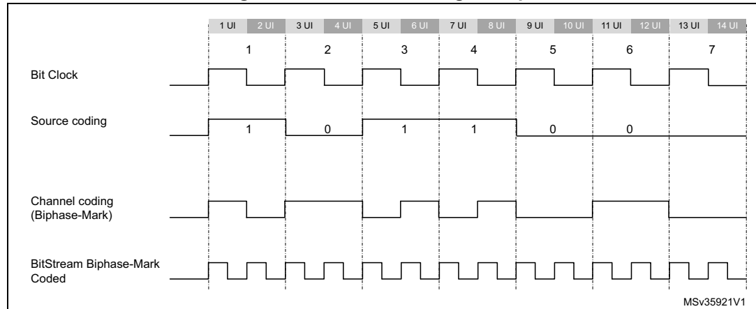
Figure 644. Channel coding example
