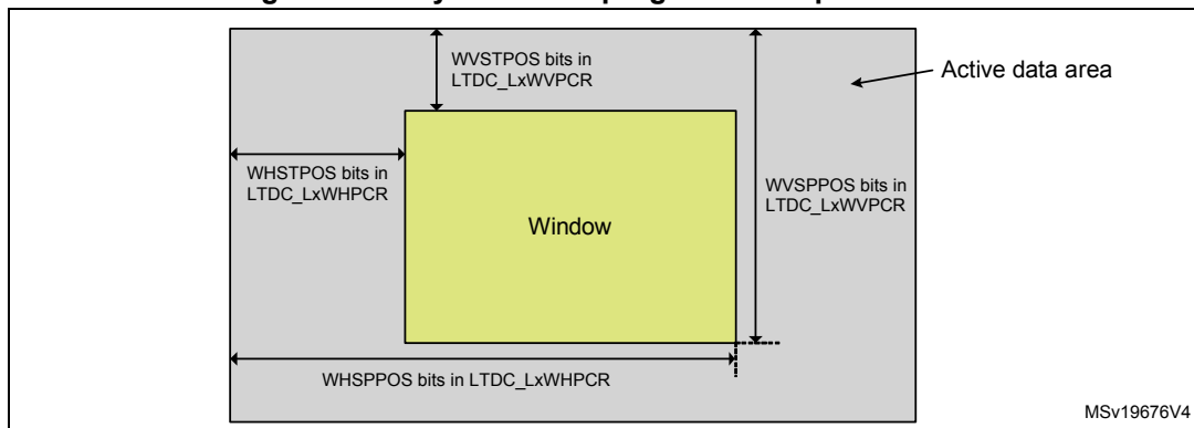
Figure 278. Layer window programmable parameters
