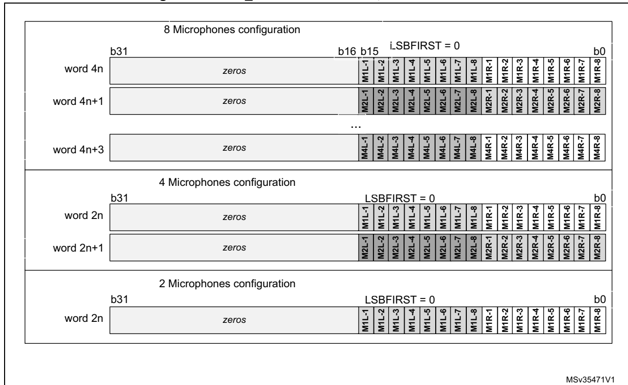
Figure 629. SAI_ADR format in TDM, 16-bit slot width
