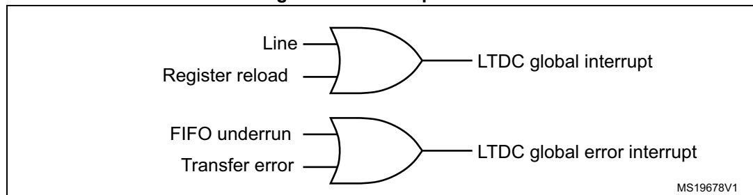
Figure 280. Interrupt events
