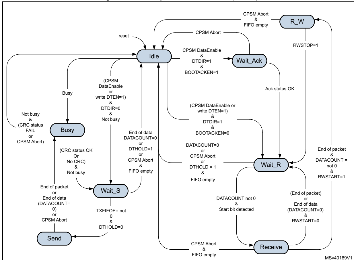
Figure 684. Data path state machine (DPSM)
