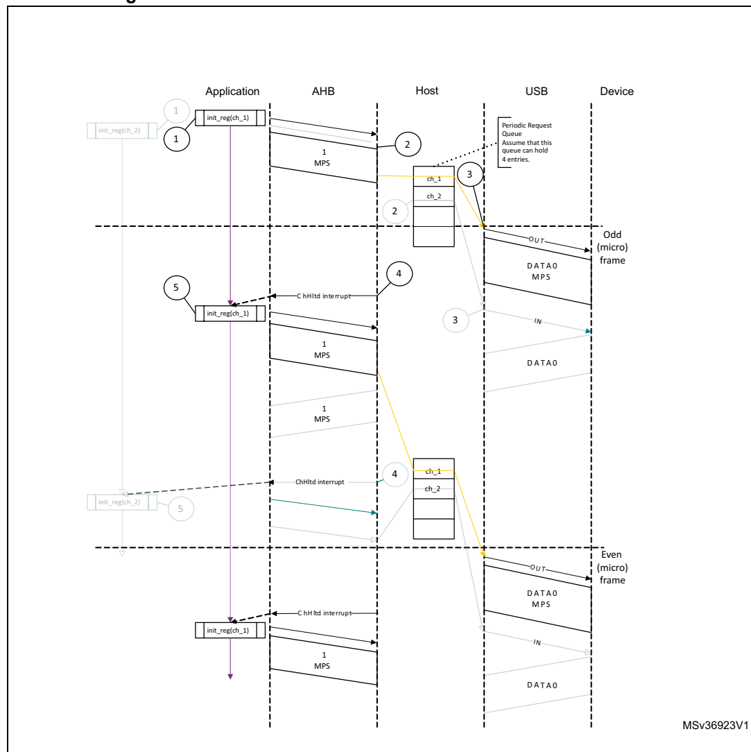
Figure 742. Normal isochronous OUT transaction - DMA mode
