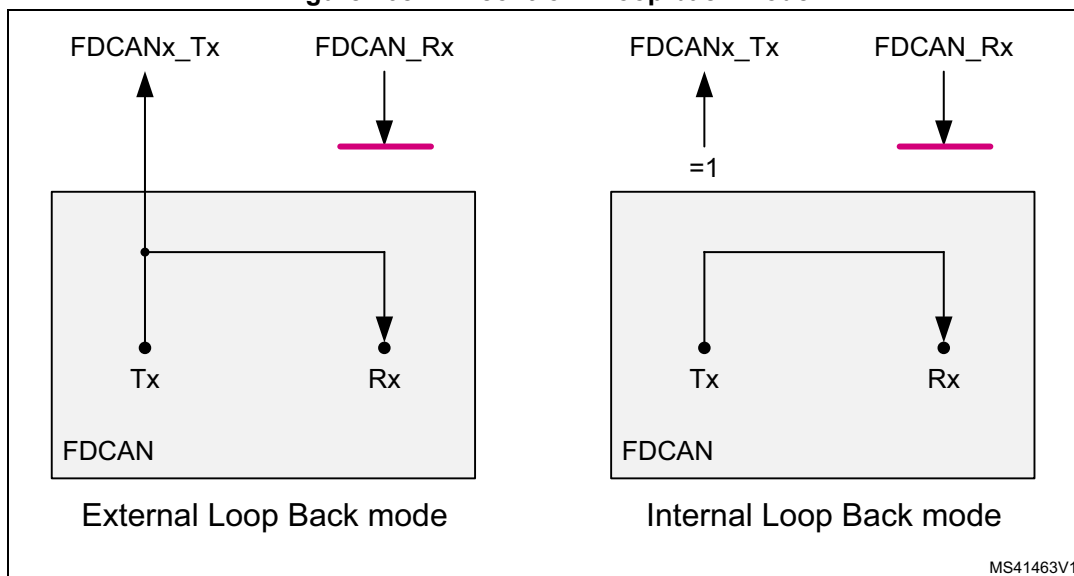
Figure 708. Pin control in loop back mode
