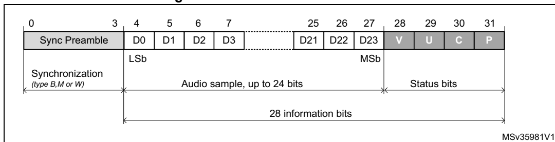
Figure 641. S/PDIF sub-frame format
