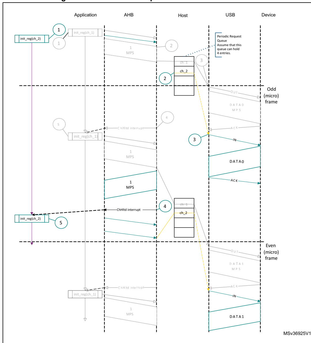
Figure 741. Normal interrupt IN transactions - DMA mode
