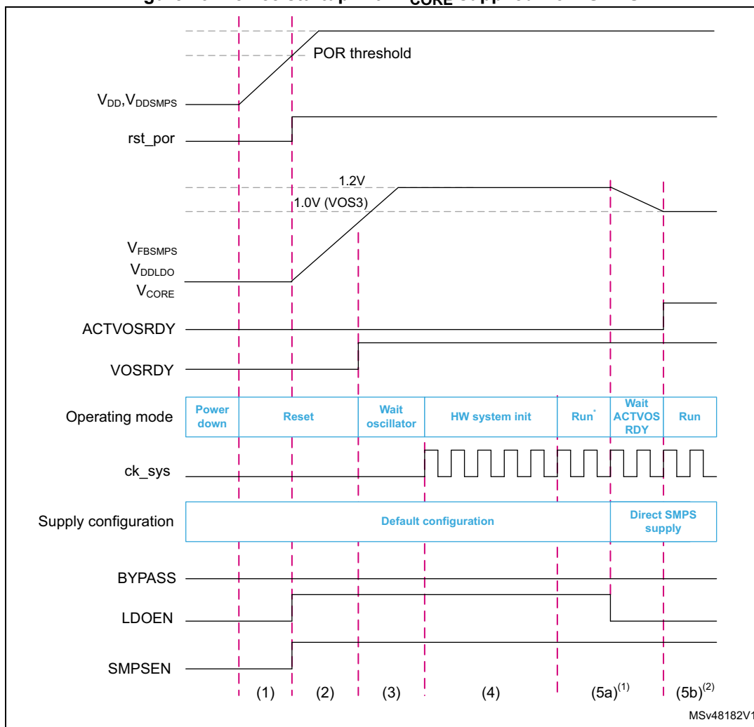
Figure 23. Device startup with V_{\text{CORE}} supplied from SMPS
