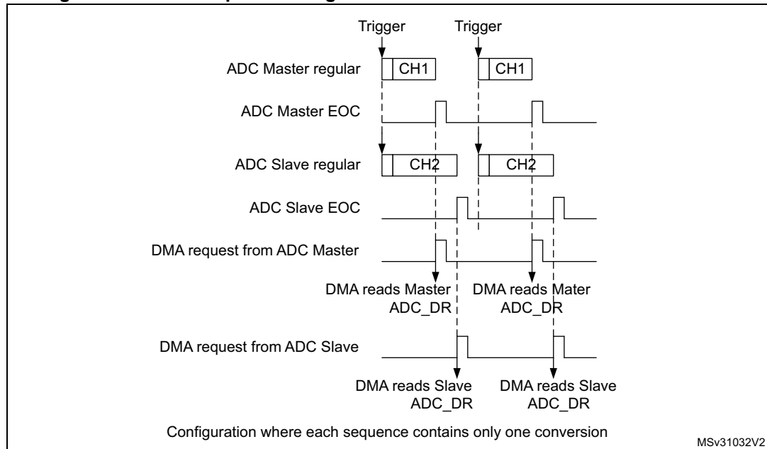
Figure 221. DMA Requests in regular simultaneous mode when DAMDF=0b00
