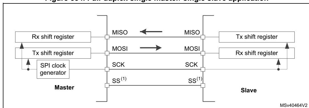
Figure 584. Full-duplex single master/ single slave application
