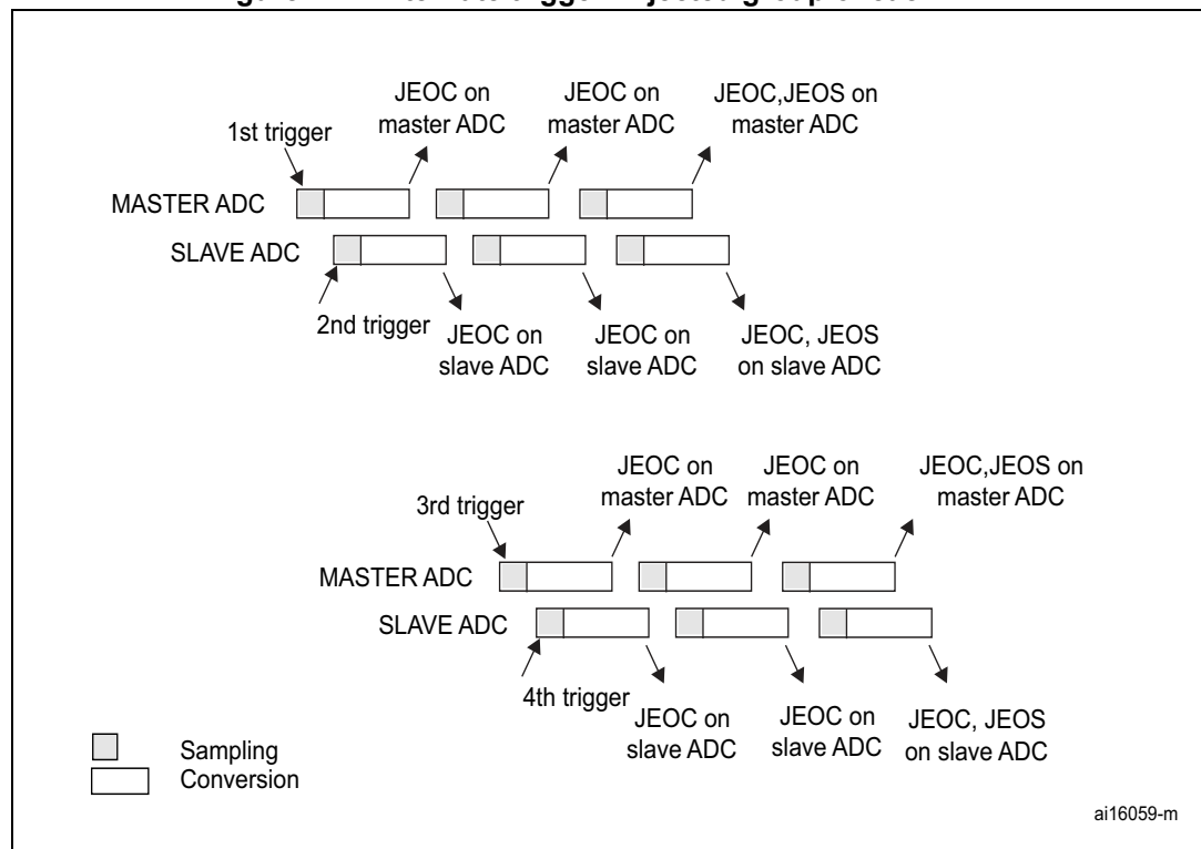
Figure 214. Alternate trigger: injected group of each ADC
