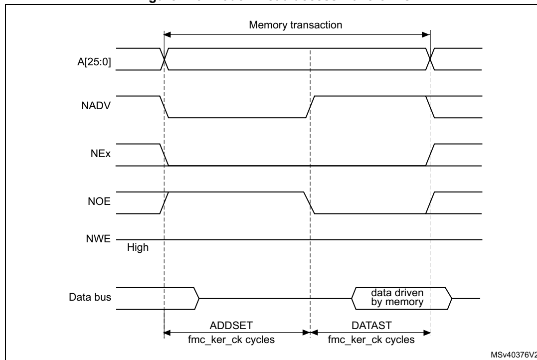
Figure 116. Mode C read access waveforms
