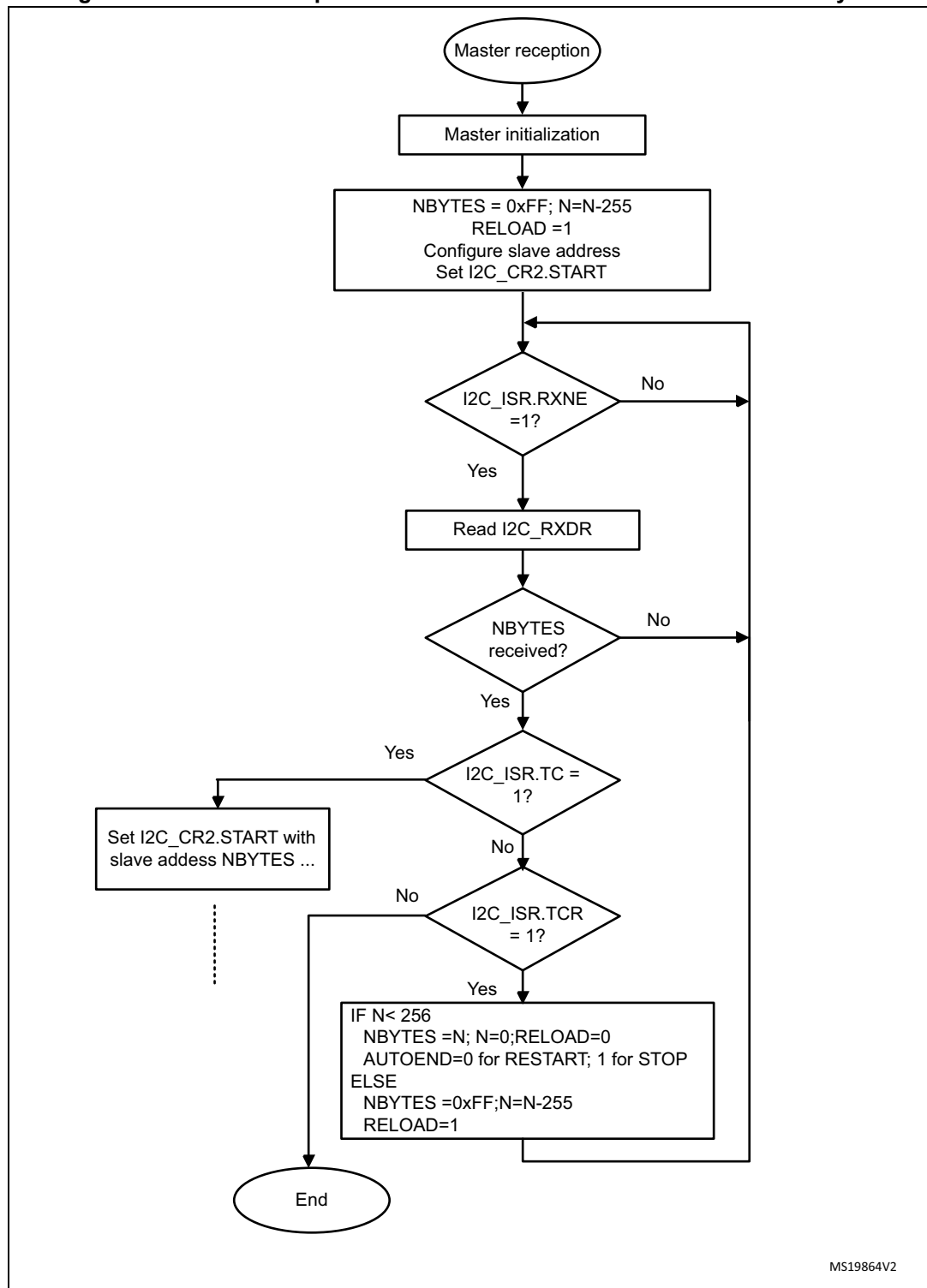
Figure 532. Transfer sequence flow for I2C master receiver for N &gt; 255 bytes
