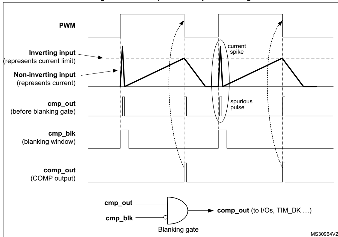
Figure 242. Comparator output blanking
