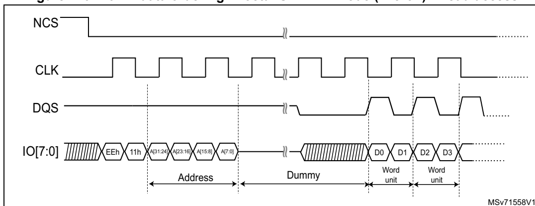
Figure 149. D0/D1 data ordering in octal-SPI DTR mode (Micron) - Read access
