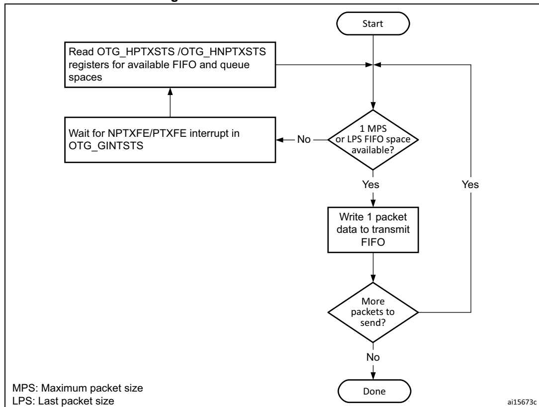
Figure 730. Transmit FIFO write task
