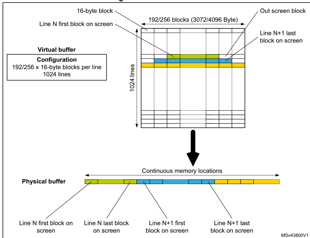
Figure 102. Virtual buffer
