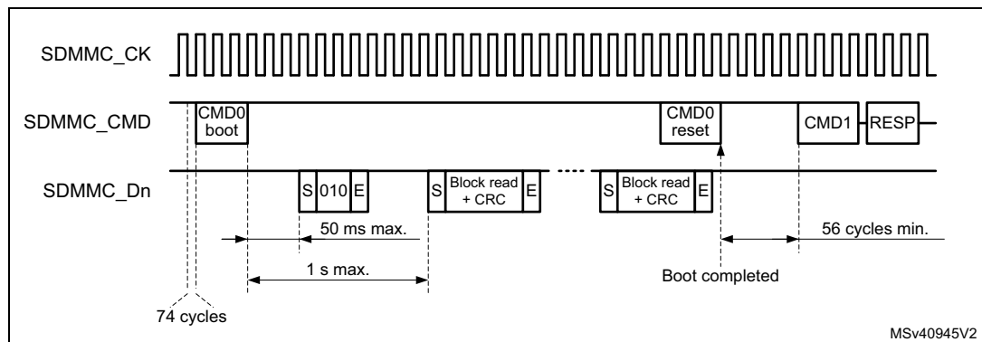
Figure 698. Alternative boot mode operation
