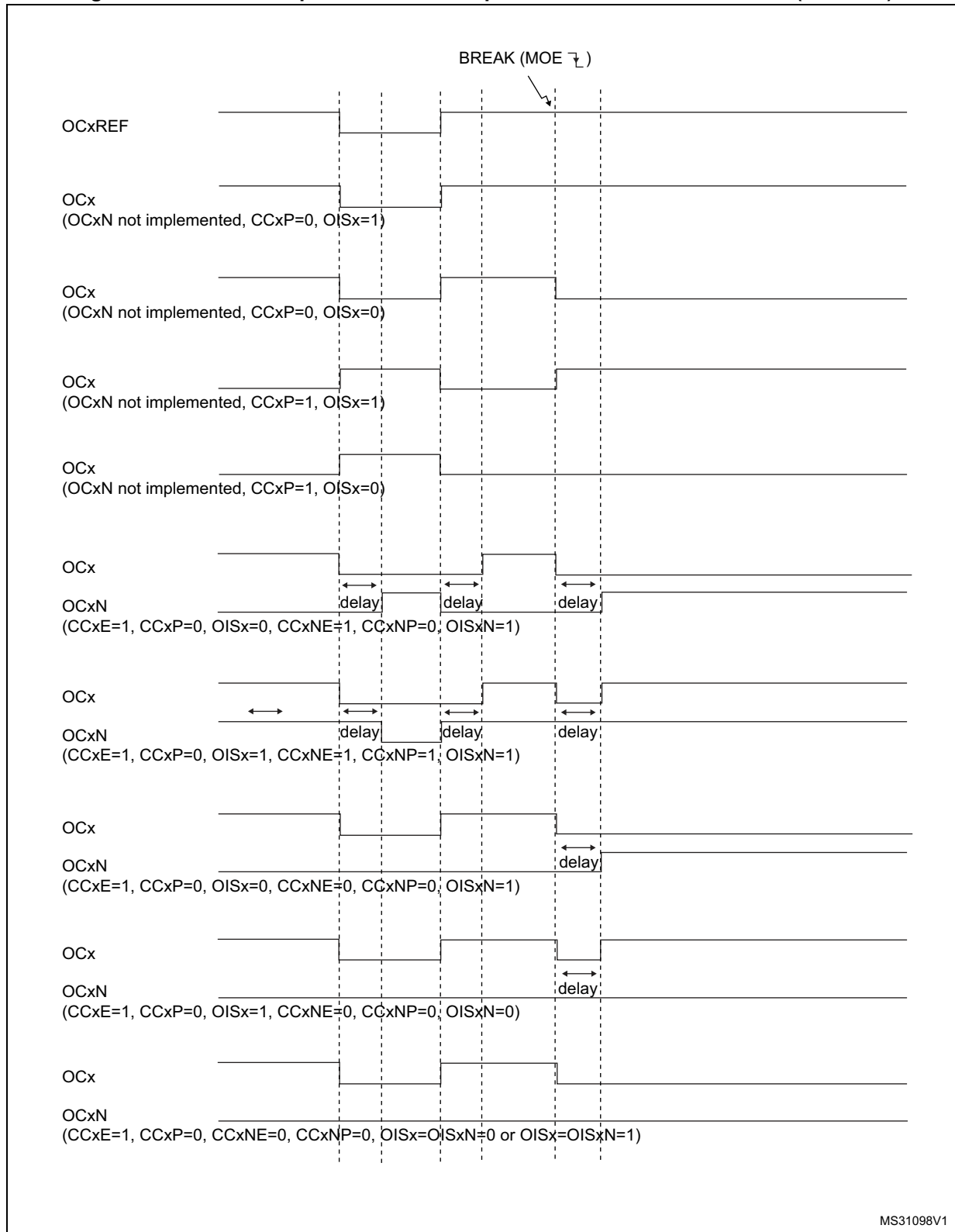
Figure 361. Various output behavior in response to a break event on BRK (OSS1 = 1)
