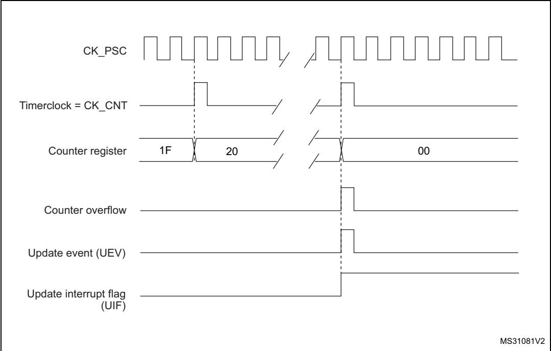
Figure 494. Counter timing diagram, internal clock divided by N
