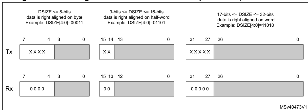
Figure 594. Data alignment when data size is not equal to 8-bit, 16-bit or 32-bit
