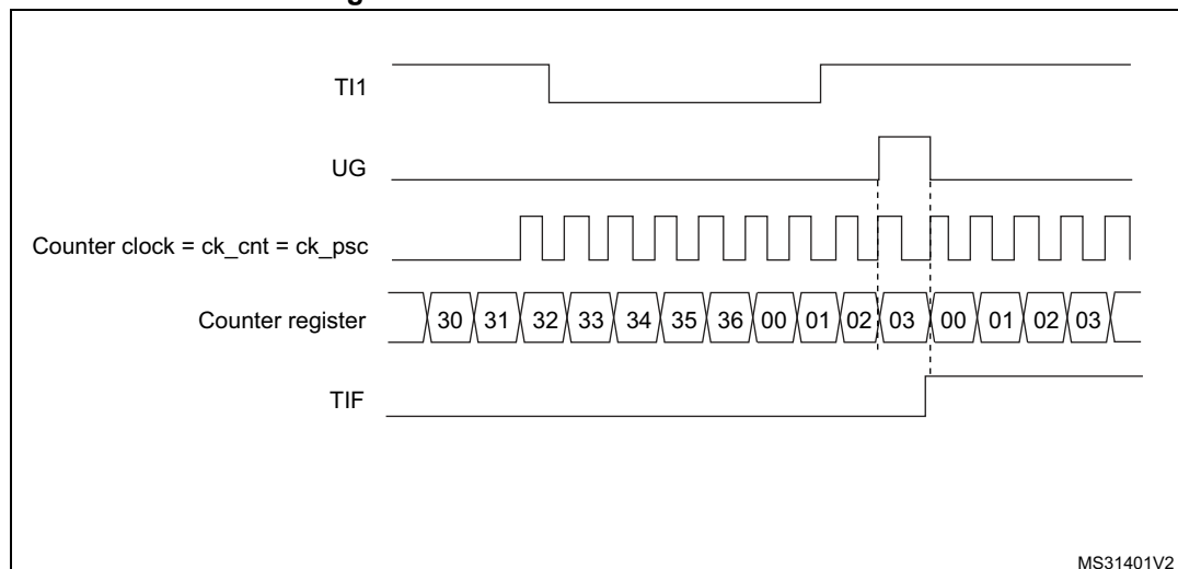
Figure 450. Control circuit in reset mode
