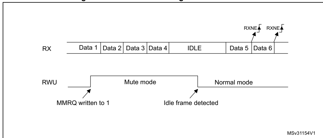
Figure 550. Mute mode using Idle line detection
