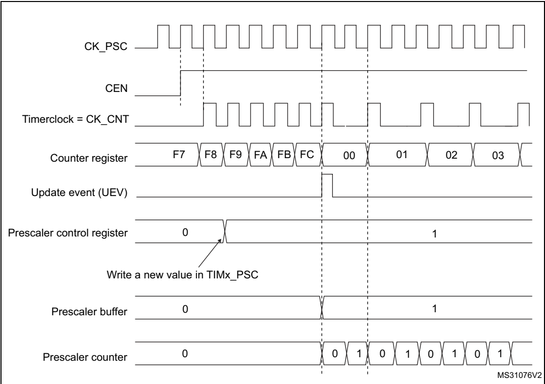
Figure 429. Counter timing diagram with prescaler division change from 1 to 2
