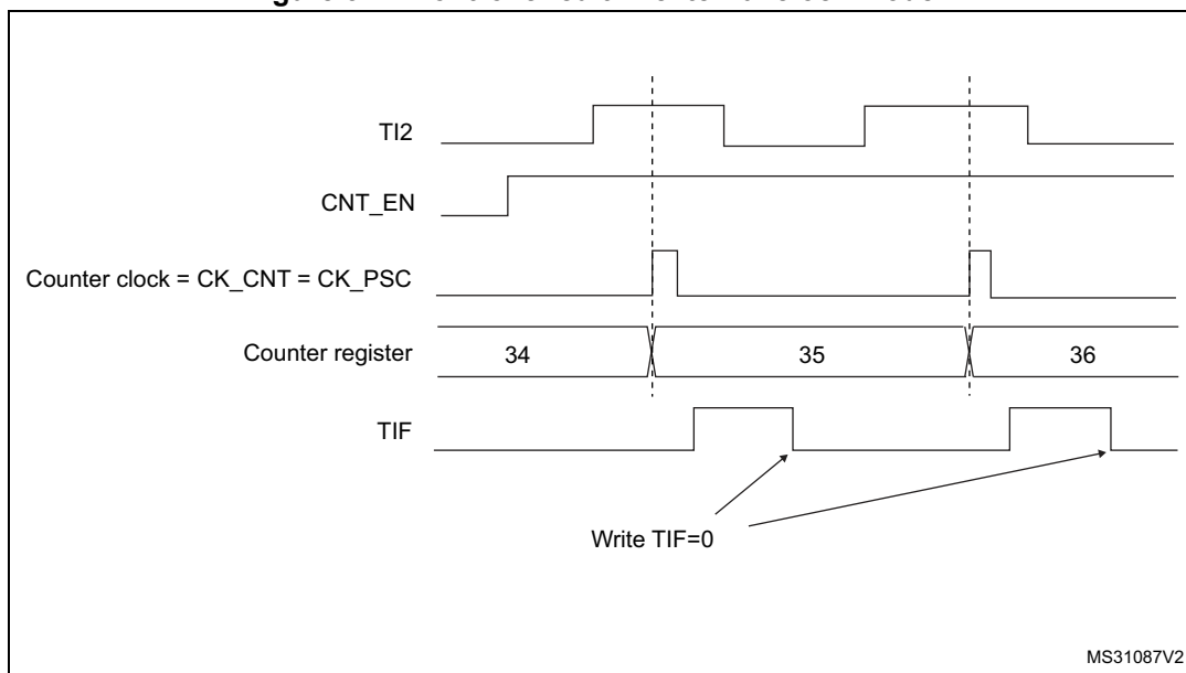
Figure 342. Control circuit in external clock mode 1
