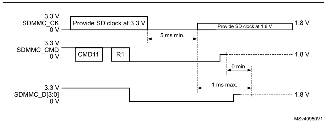
Figure 702. CMD11 signal voltage switch sequence
