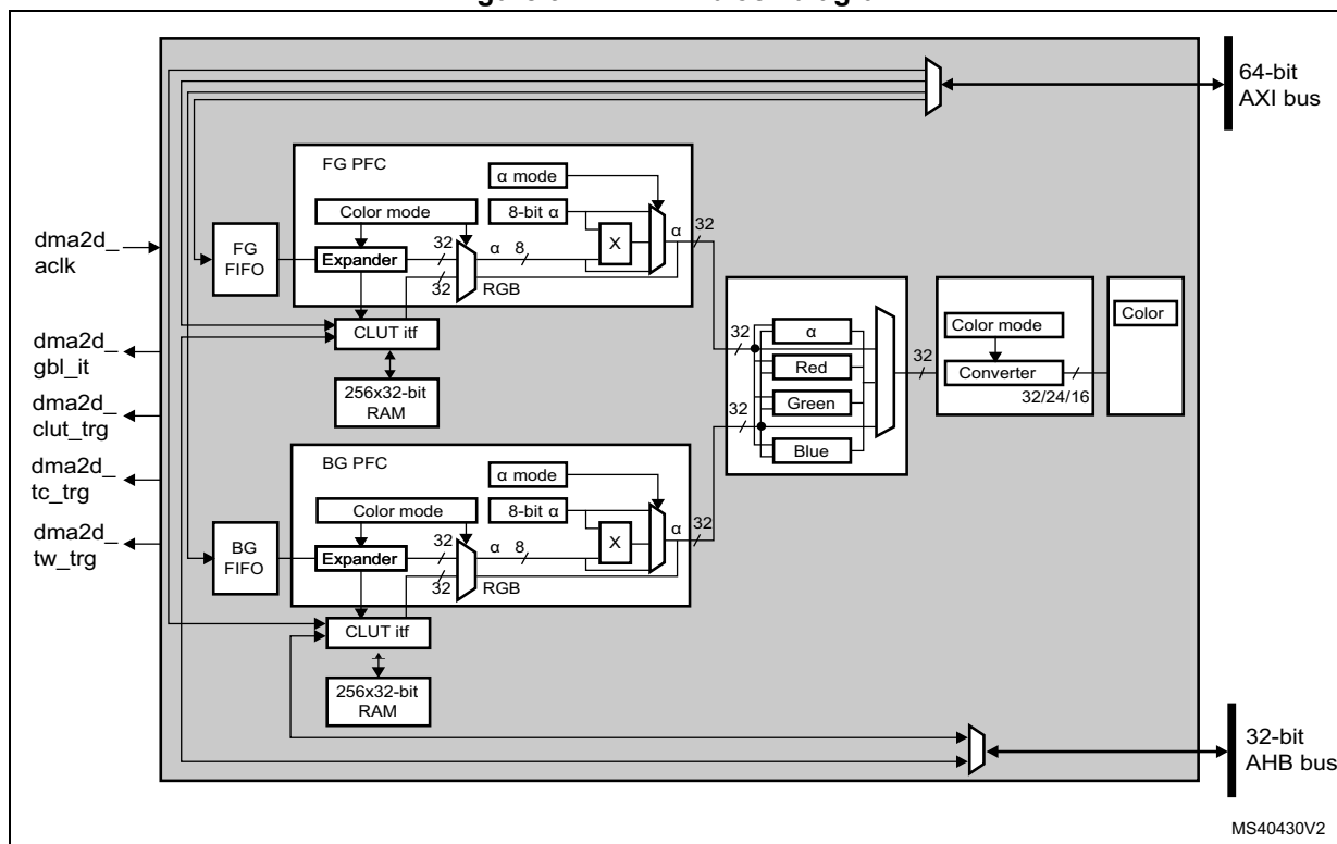
Figure 92. DMA2D block diagram
