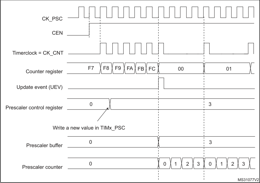
Figure 430. Counter timing diagram with prescaler division change from 1 to 4
