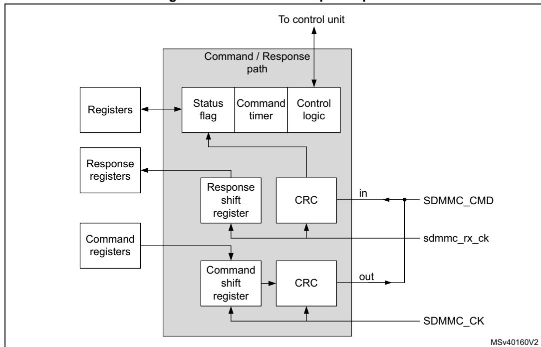
Figure 679. Command/response path
