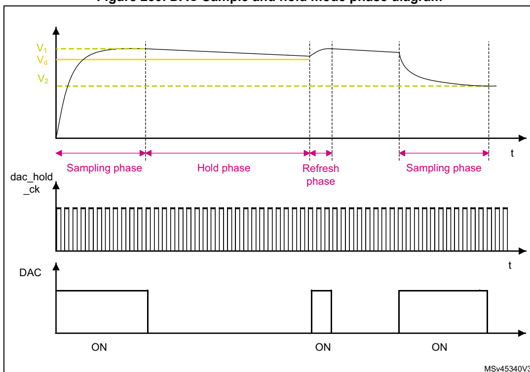
Figure 239. DAC Sample and hold mode phase diagram
