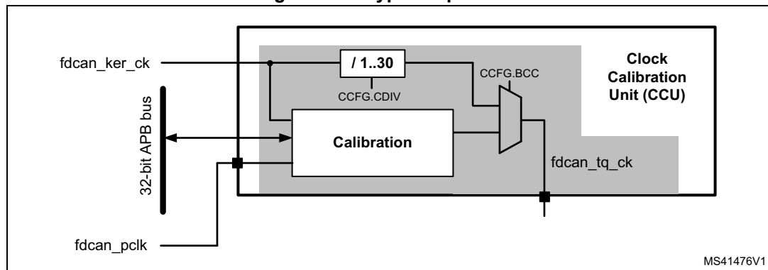
Figure 715. Bypass operation
