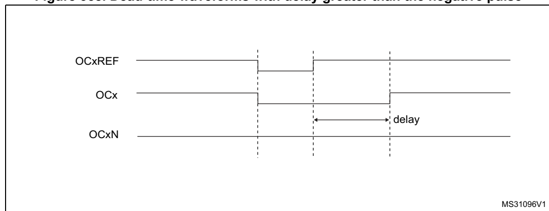
Figure 358. Dead-time waveforms with delay greater than the negative pulse
