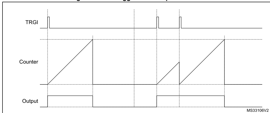
Figure 483. Retriggerable one pulse mode
