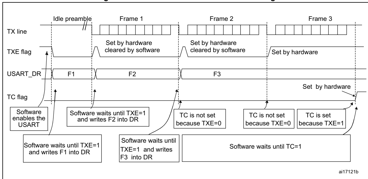
Figure 545. TC/TXE behavior when transmitting
