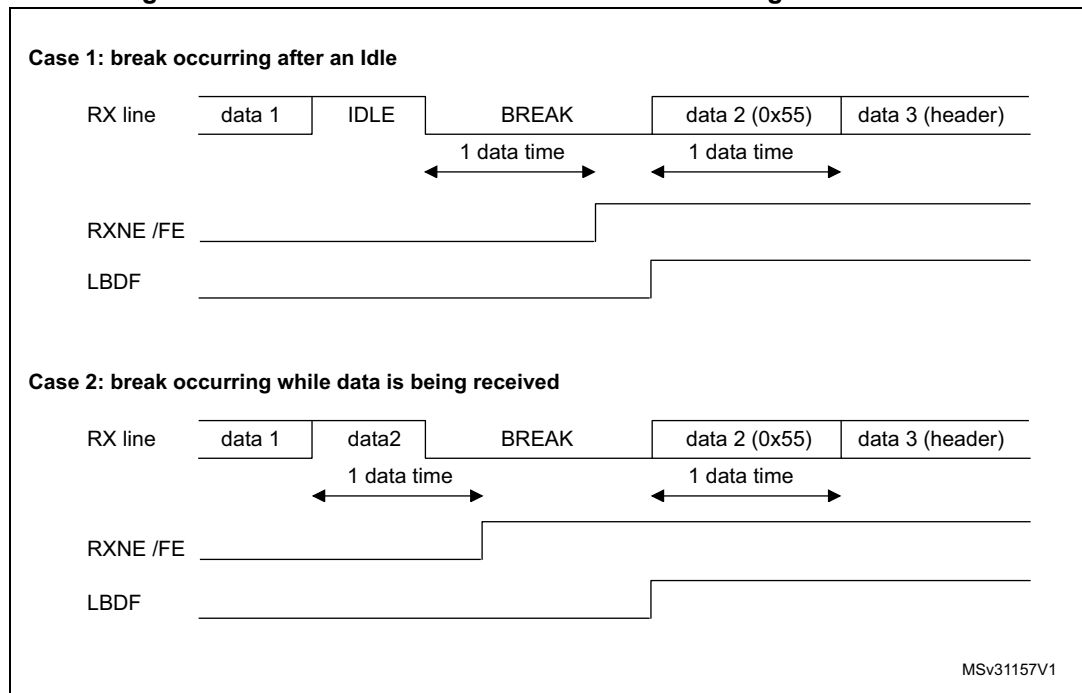
Figure 553. Break detection in LIN mode vs. Framing error detection
