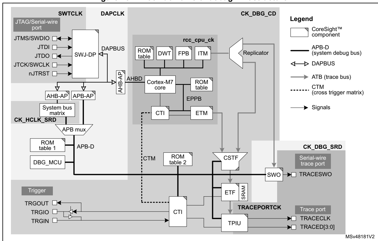
Figure 764. Clock domains of debug infrastructure
