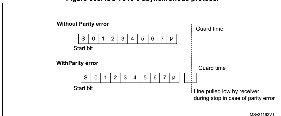
Figure 558. ISO 7816-3 asynchronous protocol
