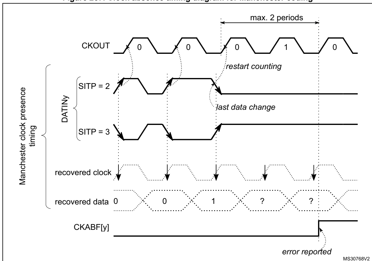
Figure 257. Clock absence timing diagram for Manchester coding
