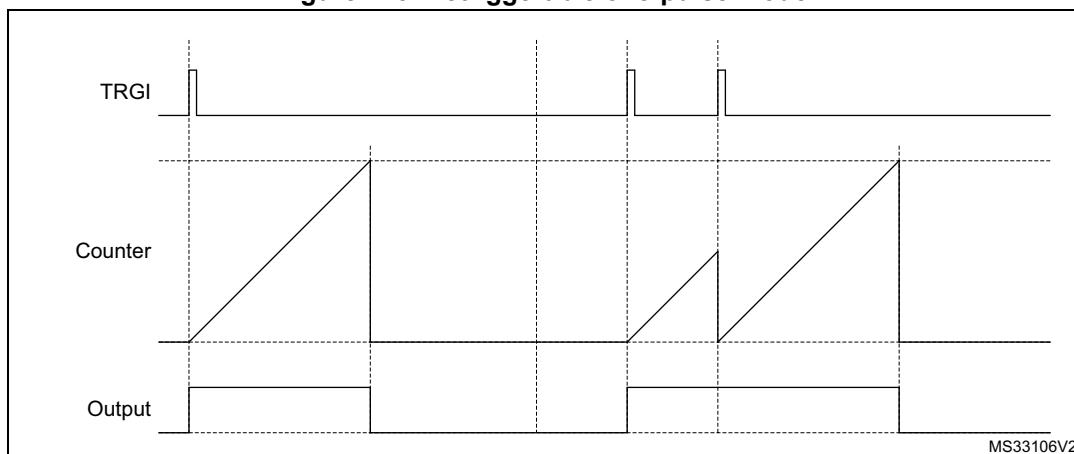
Figure 413. Retriggerable one-pulse mode.
