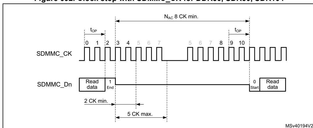
Figure 692. Clock stop with SDMMC_CK for DDR50, SDR50, SDR104
