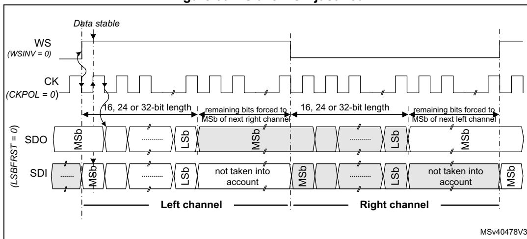
Figure 604. Slave MSB justified
