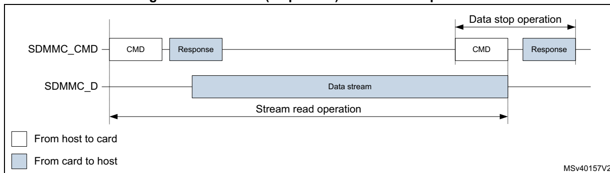
Figure 674. SDMMC (sequential) stream read operation
