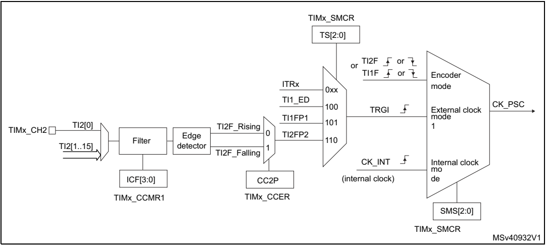
Figure 438. TI2 external clock connection example
