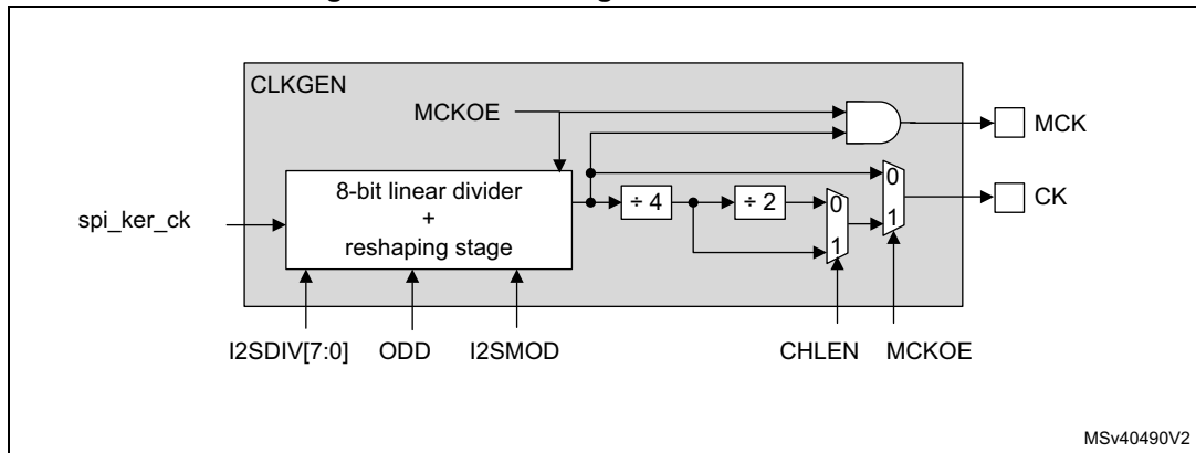
Figure 612. I 2 S clock generator architecture
