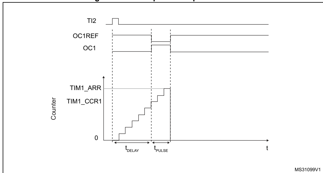
Figure 367. Example of one pulse mode.
