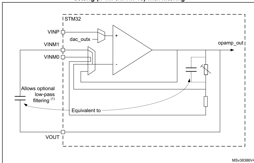
Figure 251. PGA mode, non-inverting gain setting (x2/x4/x8/x16) or inverting gain setting (x-1/x-3/x-7/x-15) with filtering
