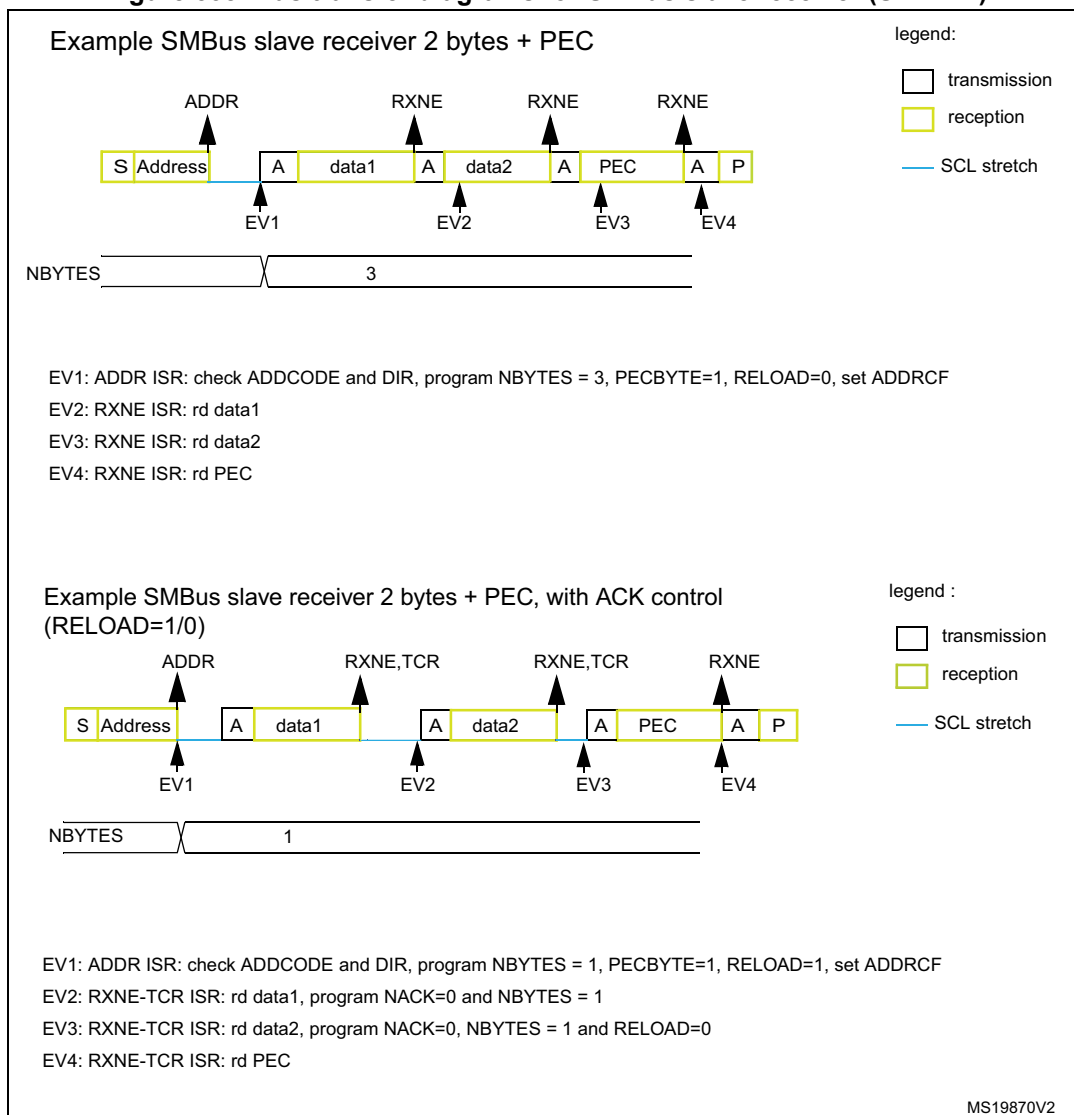
Figure 538. Bus transfer diagrams for SMBus slave receiver (SBC = 1)
