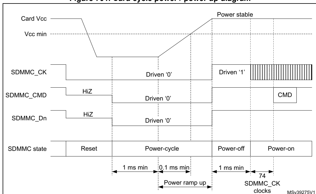
Figure 701. Card cycle power / power up diagram
