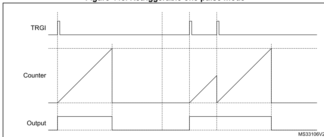
Figure 448. Retriggerable one pulse mode
