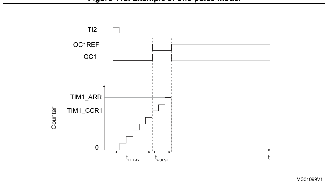
Figure 412. Example of one-pulse mode.
