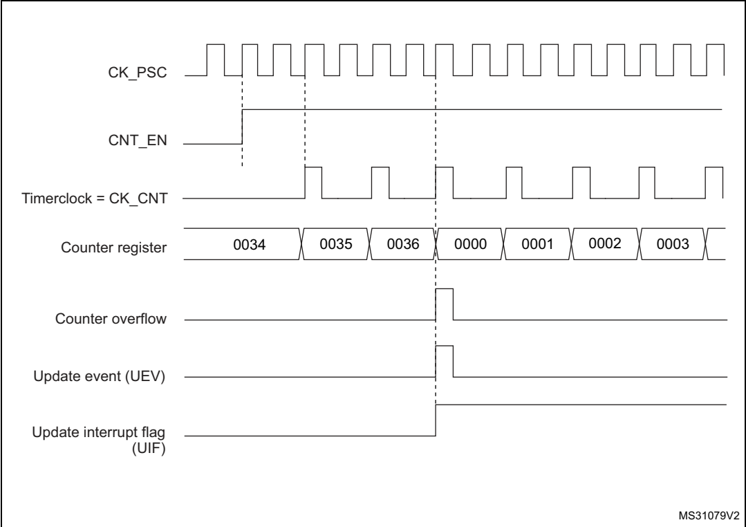
Figure 492. Counter timing diagram, internal clock divided by 2
