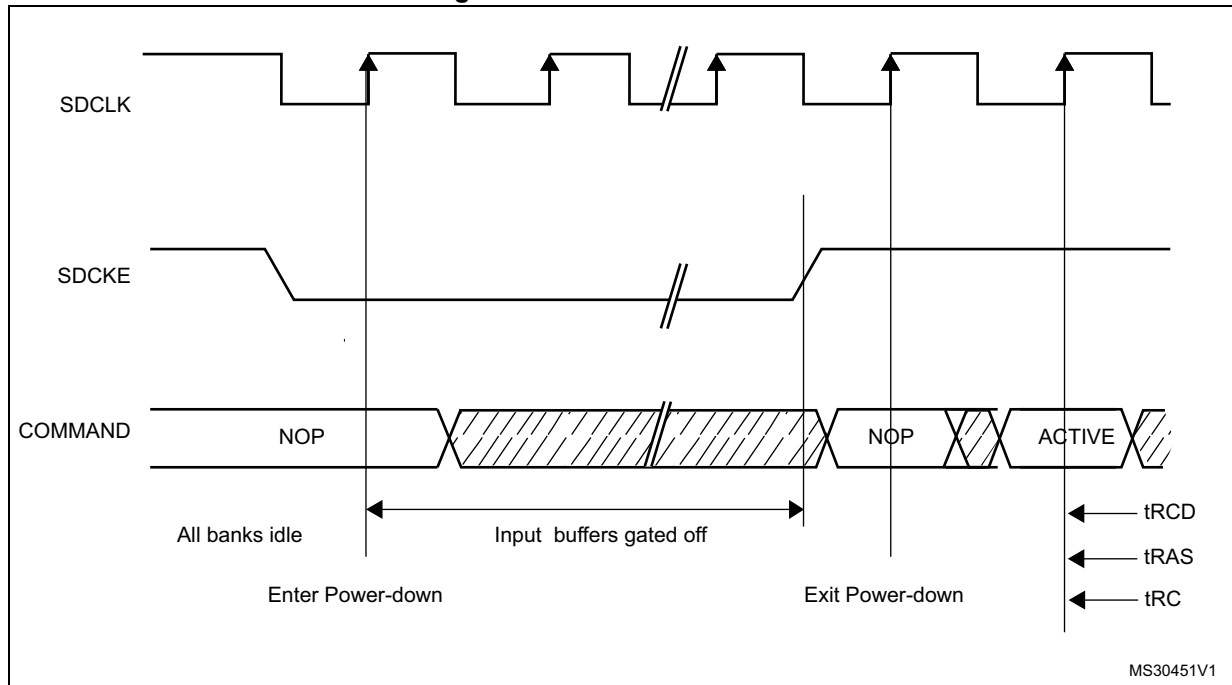
Figure 135. Power-down mode
