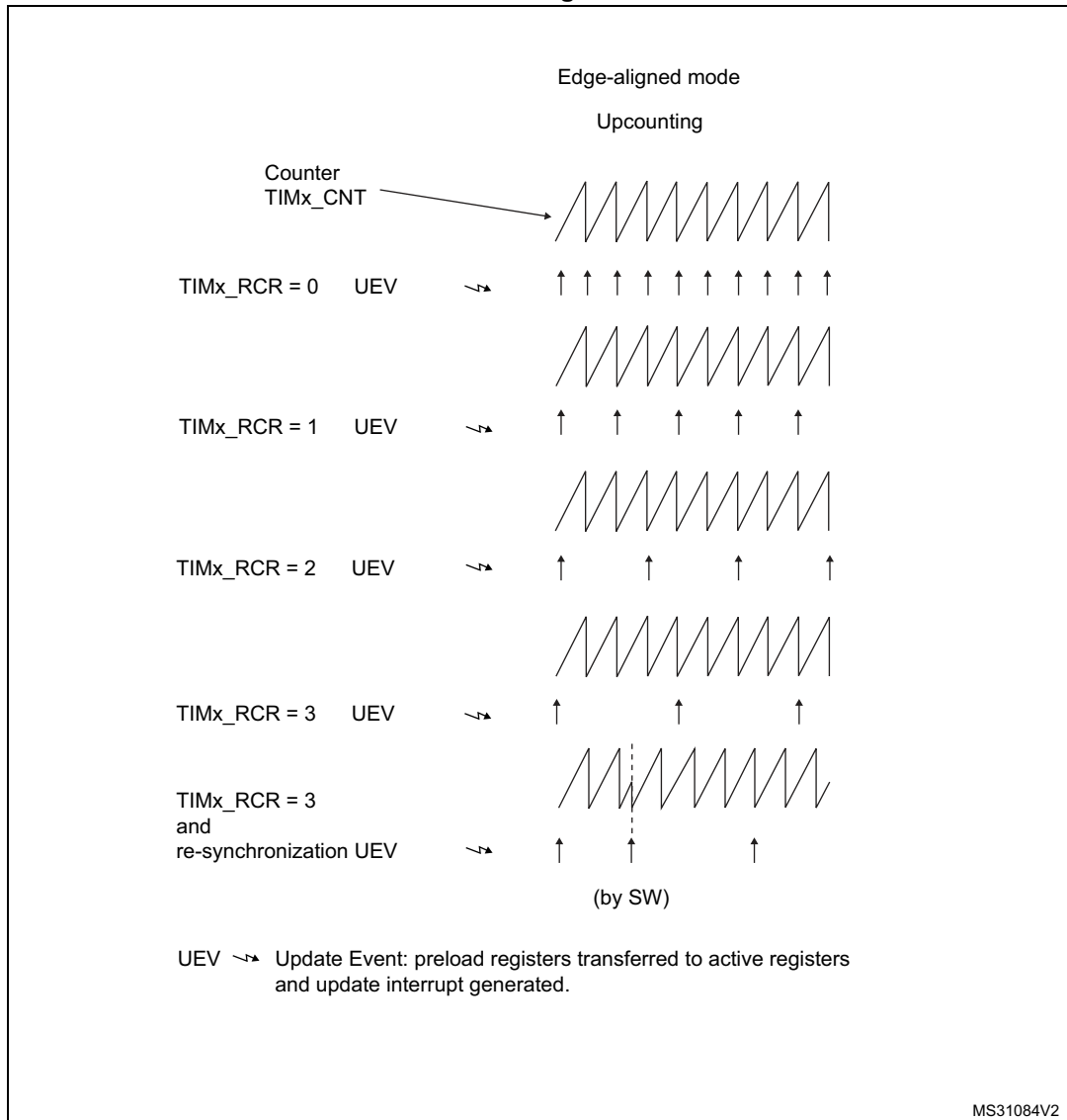
Figure 463. Update rate examples depending on mode and TIMx_RCR register settings
