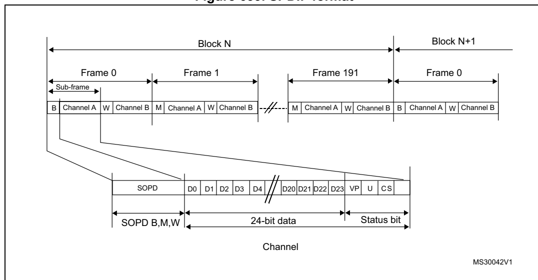
Figure 633. SPDIF format
