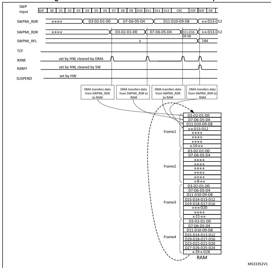
Figure 666. SWPMI Multi software buffer mode reception
