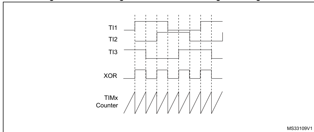
Figure 371. Measuring time interval between edges on 3 signals
