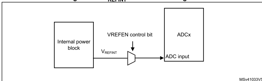
Figure 226. V_{REFINT} channel block diagram
