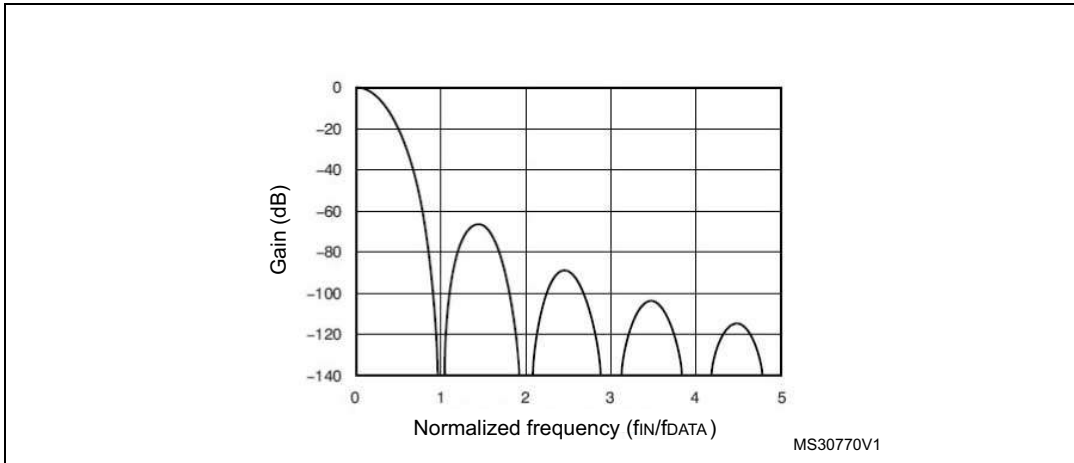
Figure 260. Example: Sinc 3 filter response
