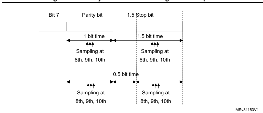
Figure 559. Parity error detection using the 1.5 stop bits
