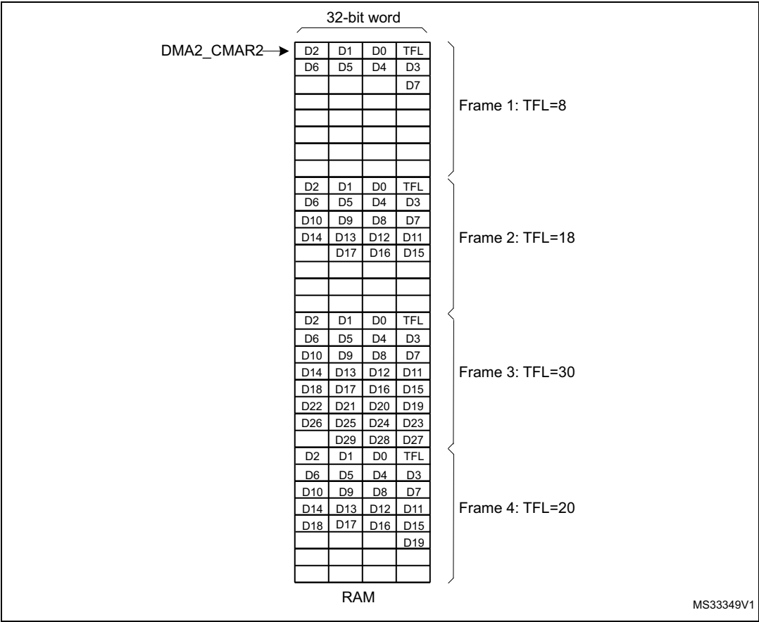
Figure 663. SWPMI Multi software buffer mode transmission
