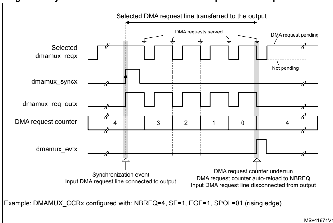
Figure 90. Synchronization mode of the DMAMUX request line multiplexer channel
