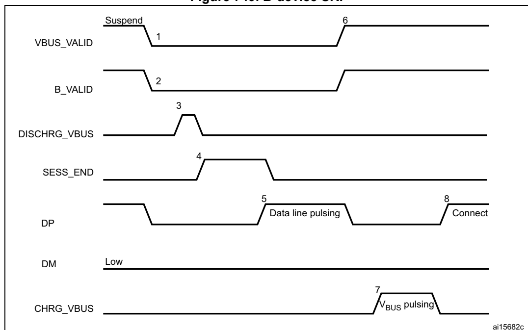
Figure 749. B-device SRP
