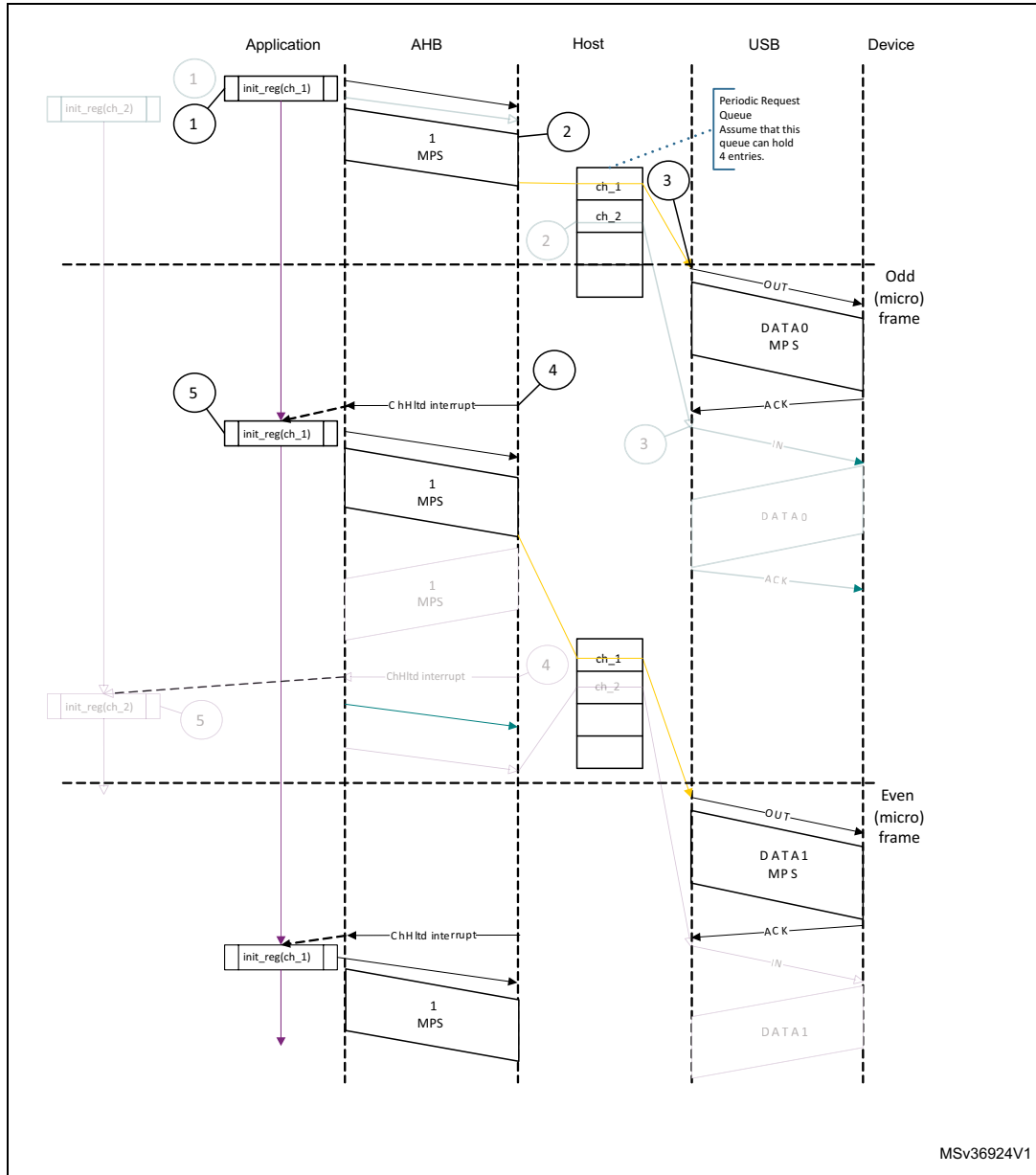
Figure 740. Normal interrupt OUT transactions - DMA mode
