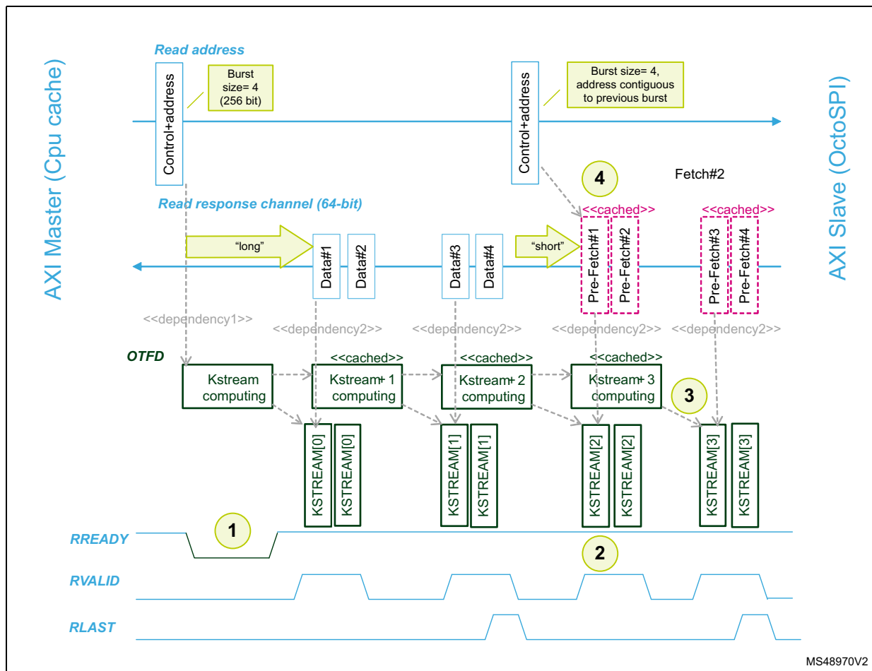
Figure 315. OTFDEC flow control overview (dual burst read request)
