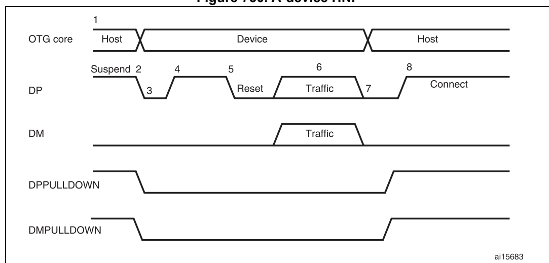
Figure 750. A-device HNP
