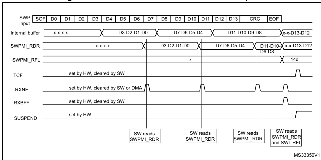
Figure 664. SWPMI No software buffer mode reception
