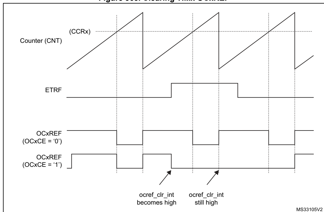
Figure 365. Clearing TIMx OCxREF
