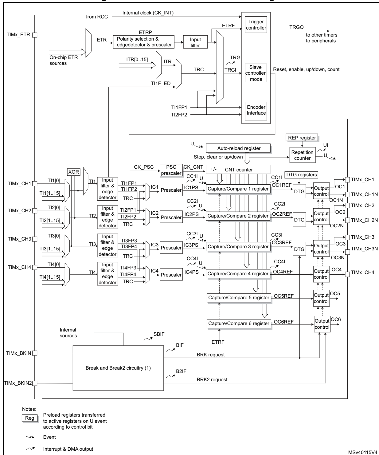
Figure 317. Advanced-control timer block diagram
