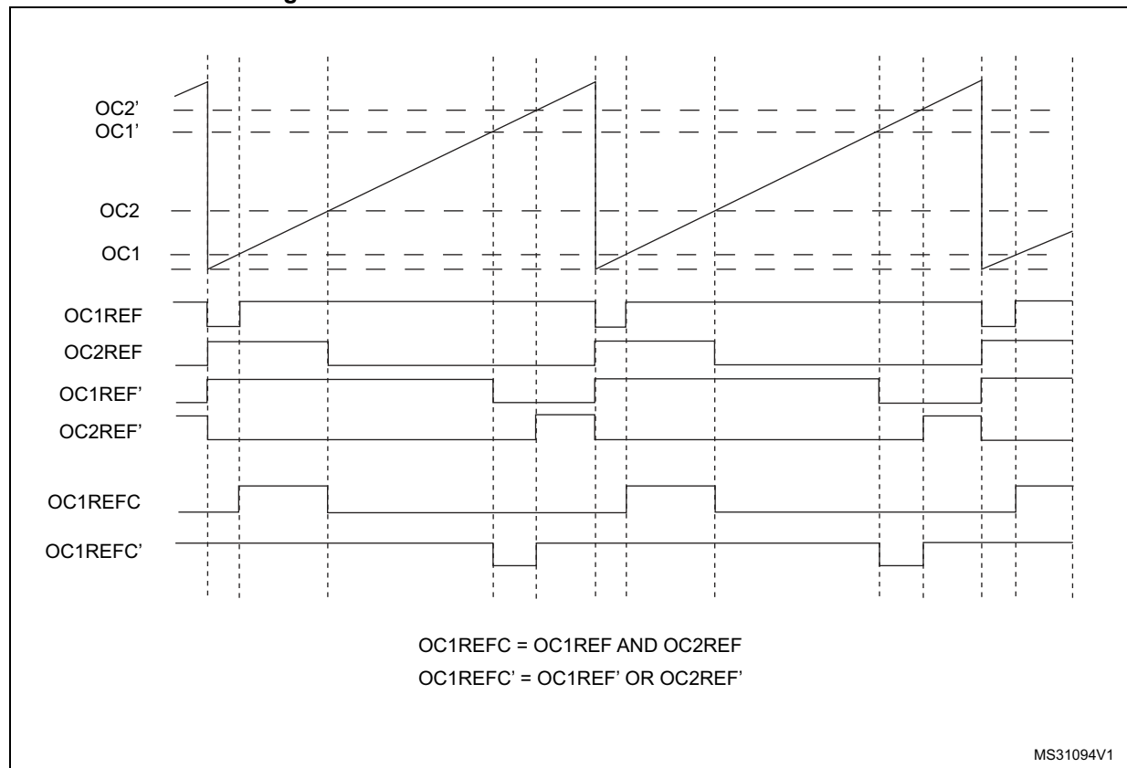
Figure 355. Combined PWM mode on channel 1 and 3
