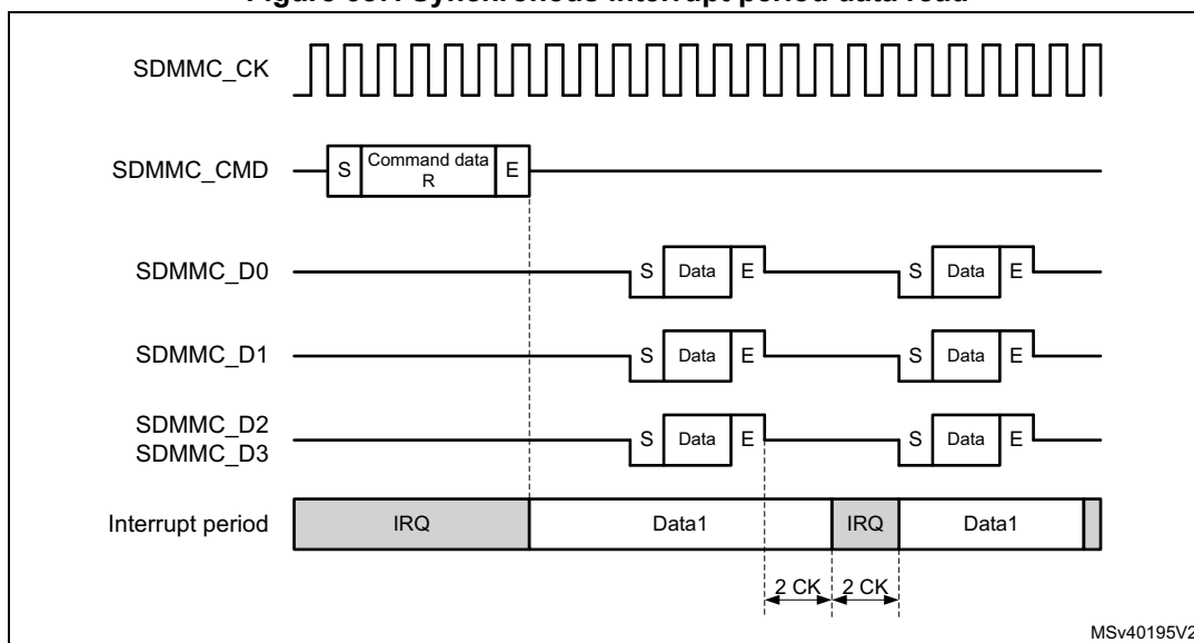
Figure 687. Synchronous interrupt period data read
