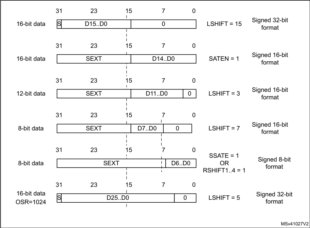
Figure 189. Left alignment (offset enabled, signed value)
