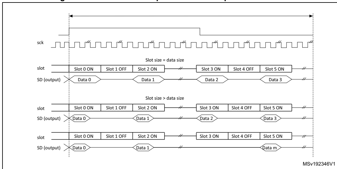
Figure 637. Tristate on output data line in a protocol like I2S
