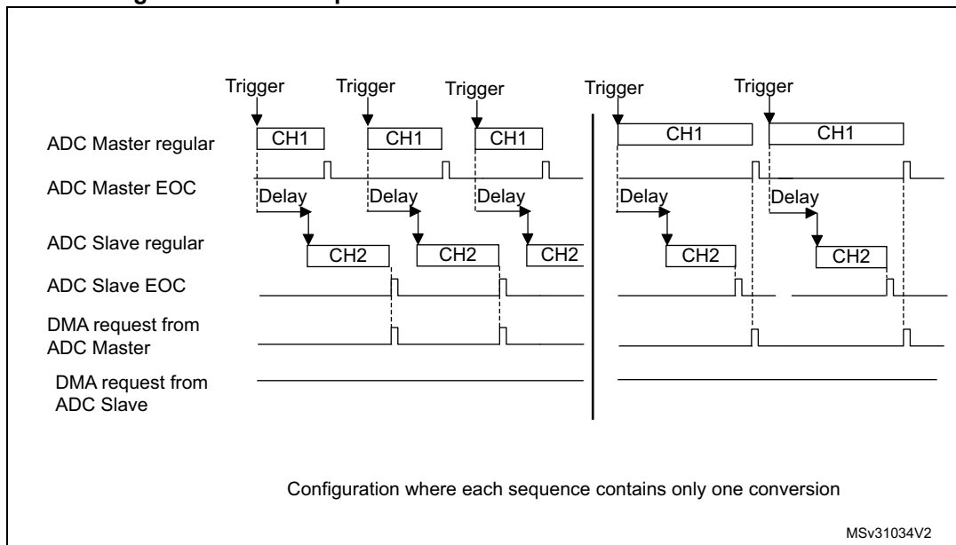
Figure 223. DMA requests in interleaved mode when DAMDF=0b10
