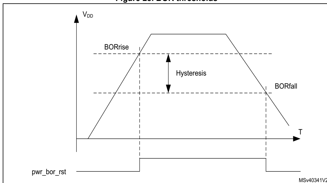
Figure 28. BOR thresholds
