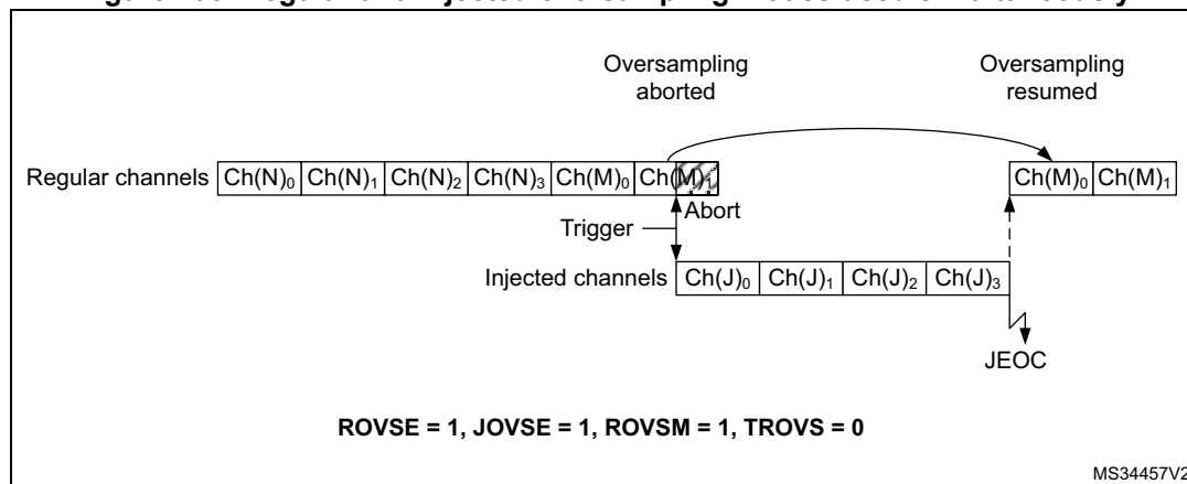
Figure 205. Regular and injected oversampling modes used simultaneously
