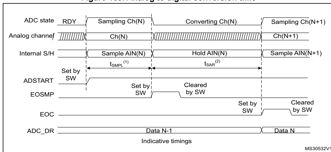
Figure 165. Analog to digital conversion time
