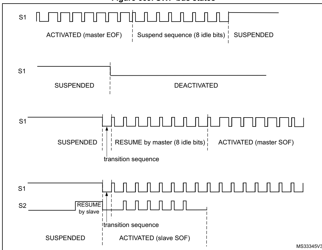
Figure 659. SWP bus states
