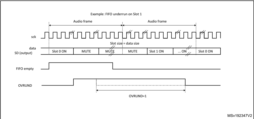
Figure 639. FIFO underrun event
