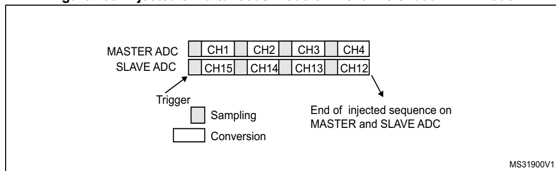
Figure 209. Injected simultaneous mode on 4 channels: dual ADC mode
