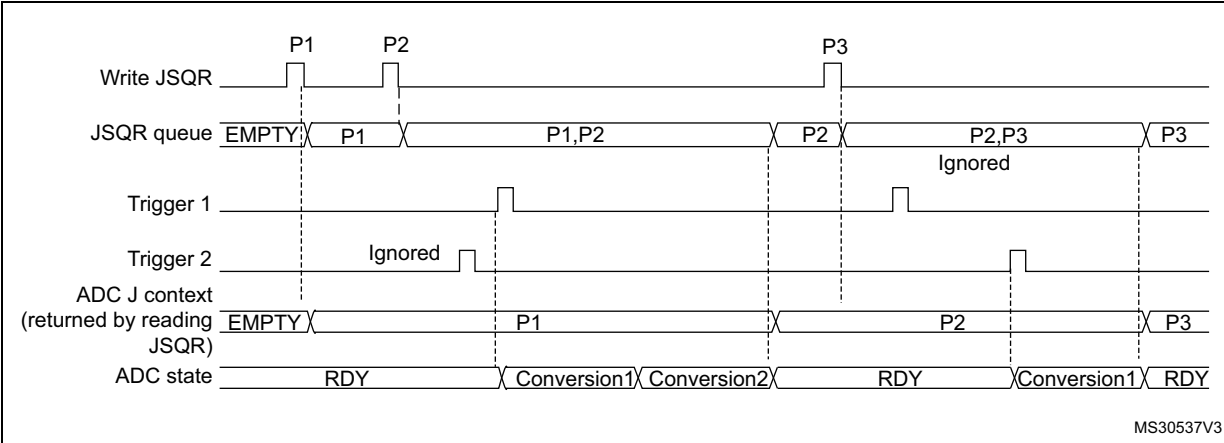
Figure 171. Example of JSQR queue of context (trigger change)
