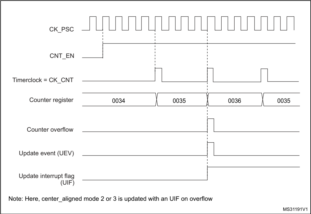
Figure 393. Counter timing diagram, internal clock divided by 4, TIMx_ARR=0x36
