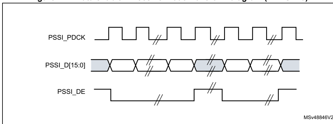
Figure 271. Data enable in receive mode waveform diagram (CKPOL=0)
