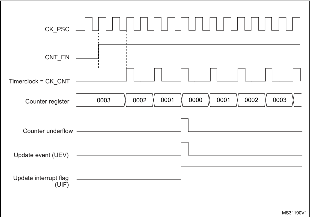
Figure 392. Counter timing diagram, internal clock divided by 2
