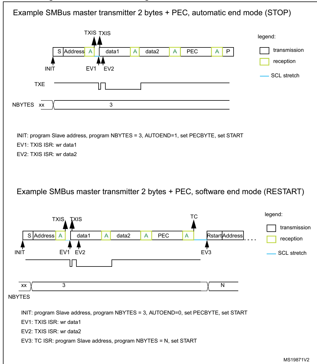
Figure 539. Bus transfer diagrams for SMBus master transmitter
