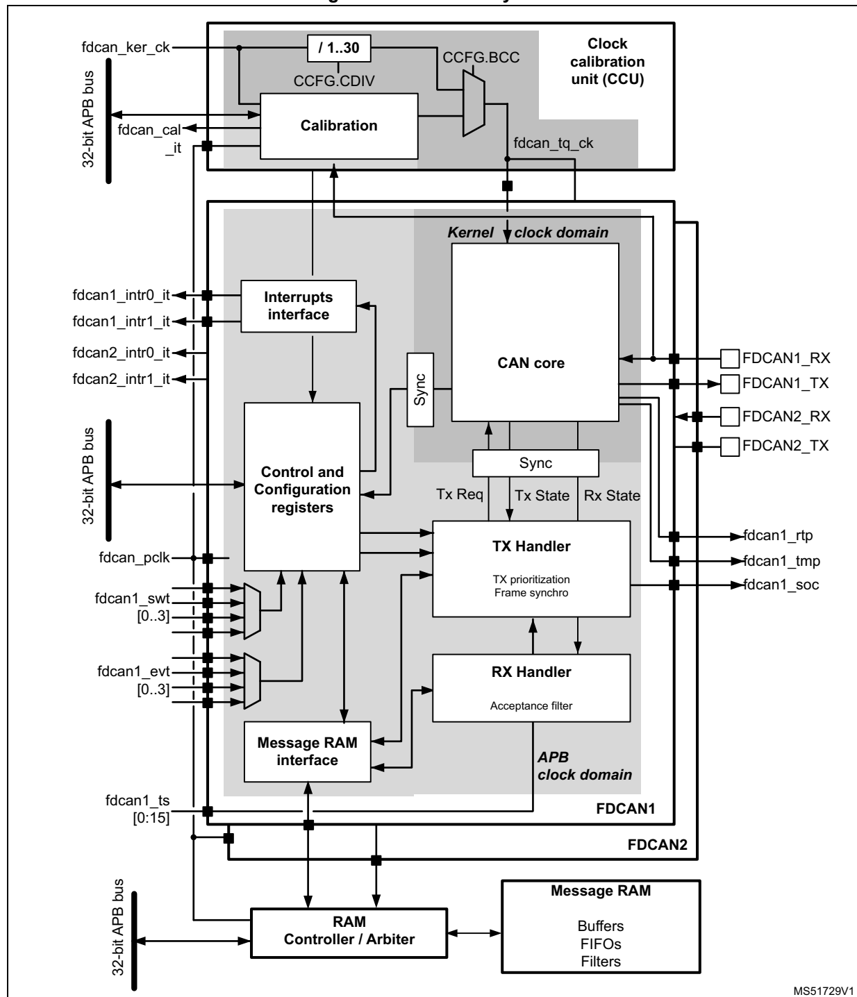
Figure 704. CAN subsystem
