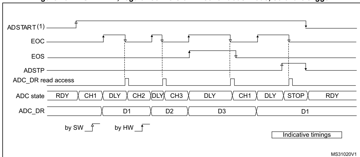
Figure 192. AUTDLY=1, regular conversion in continuous mode, software trigger
