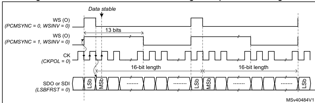
Figure 606. Master PCM when the frame length is equal the data length
