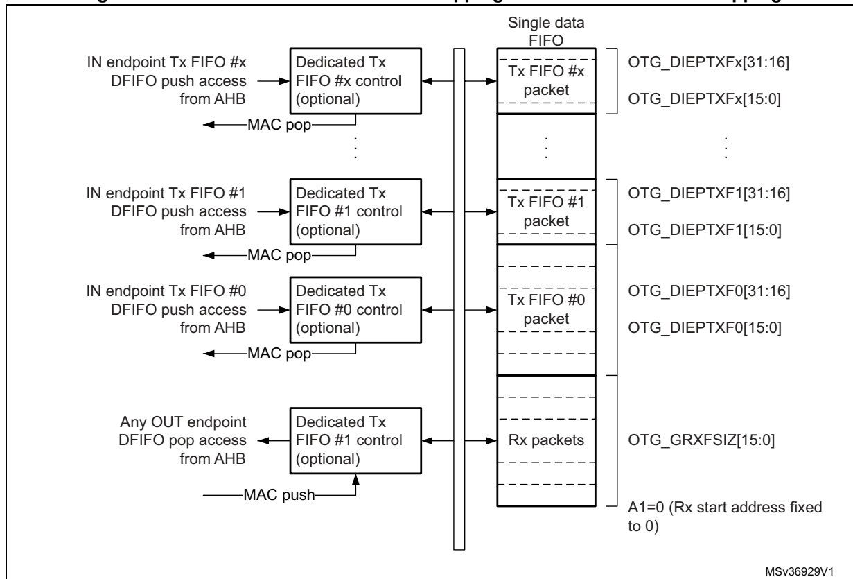
Figure 727. Device-mode FIFO address mapping and AHB FIFO access mapping
