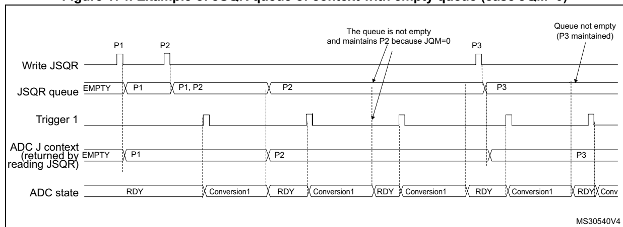
Figure 174. Example of JSQR queue of context with empty queue (case JQM=0)
