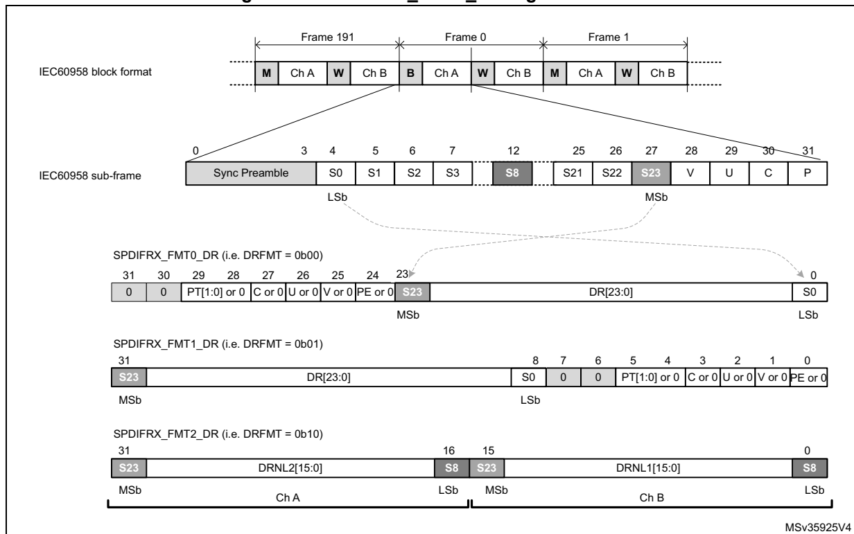
Figure 651. SPDIFRX_FMTx_DR register format
