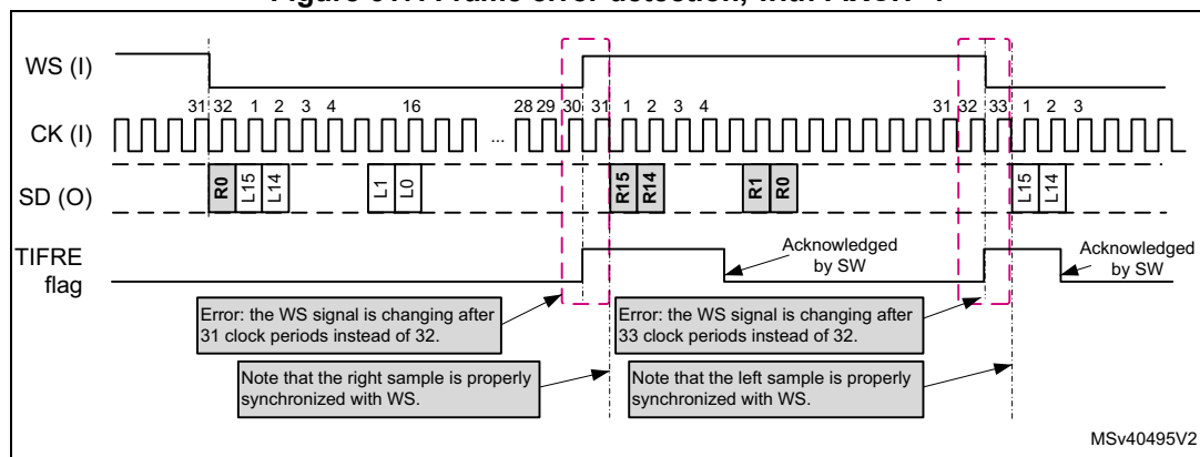
Figure 617. Frame error detection, with FIXCH=1
