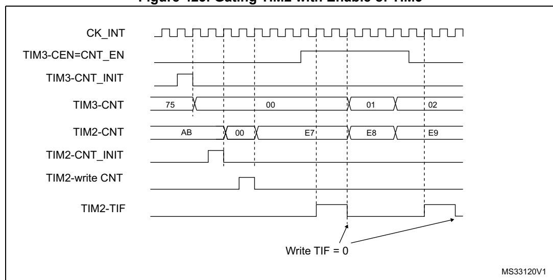
Figure 423. Gating TIM2 with Enable of TIM3
