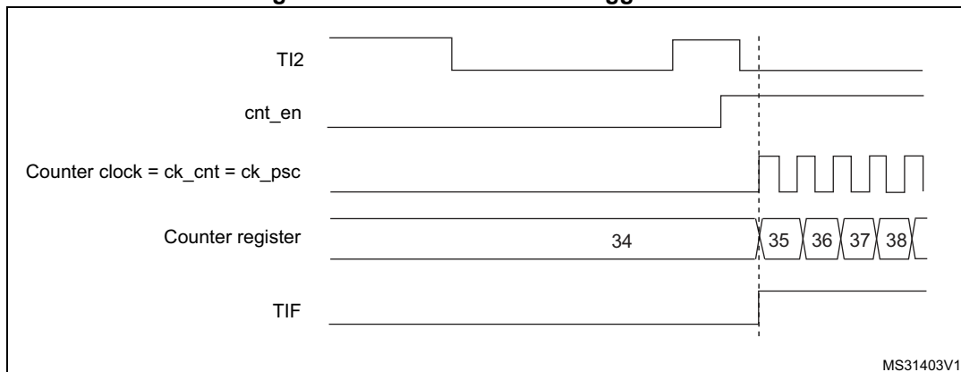
Figure 452. Control circuit in trigger mode
