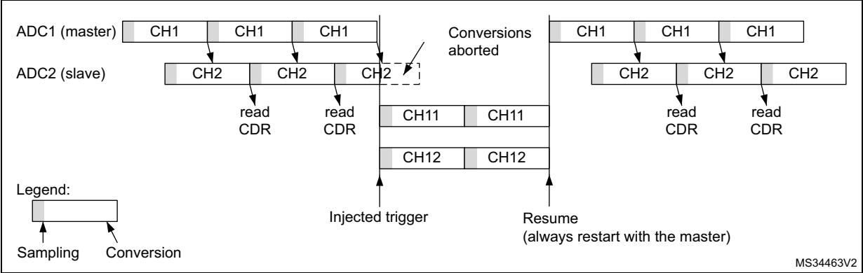
Figure 220. Two Interleaved channels (CH1, CH2) with injected sequence CH11, CH12 - case 2: Slave interrupted first
