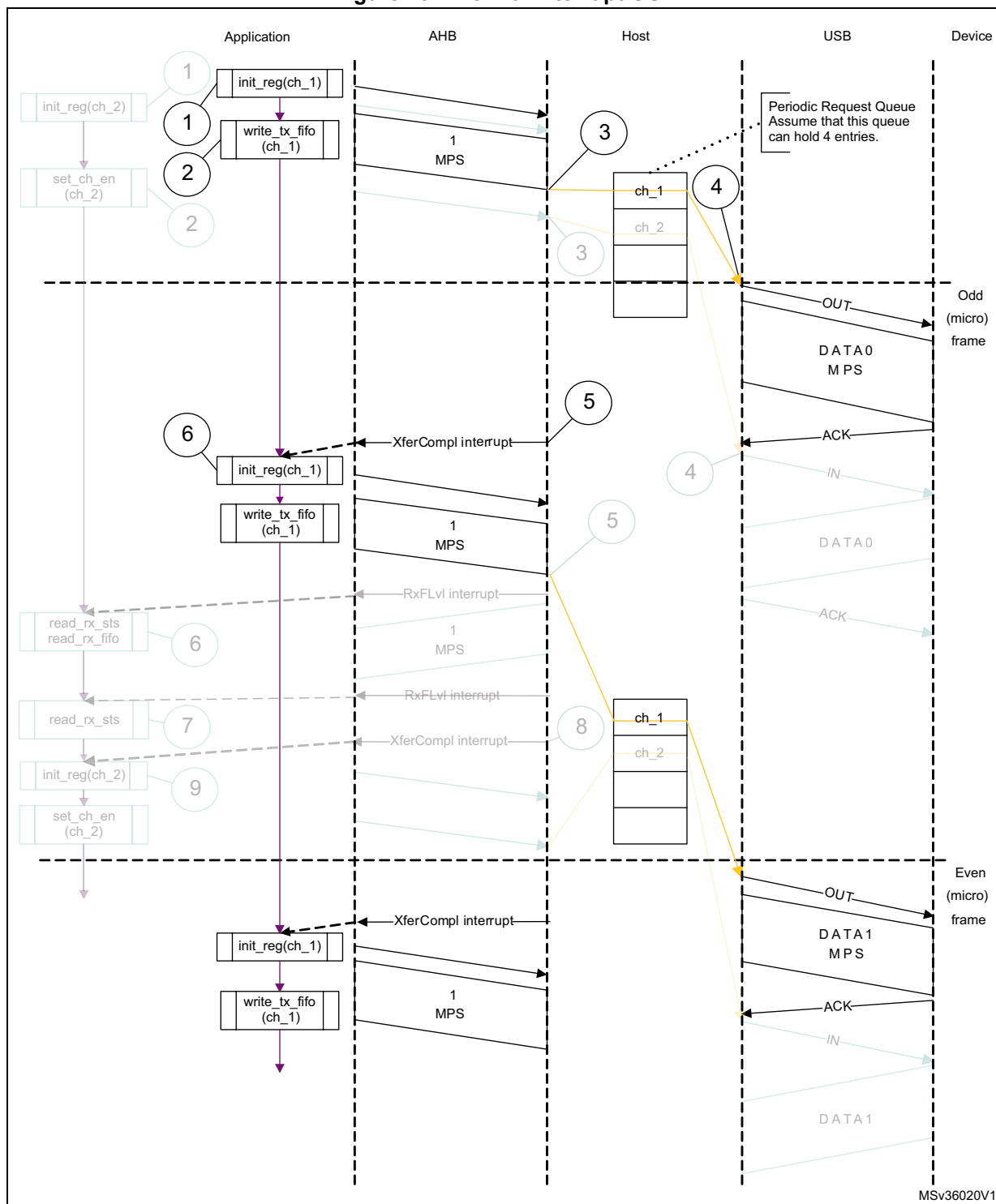
Figure 734. Normal interrupt OUT
