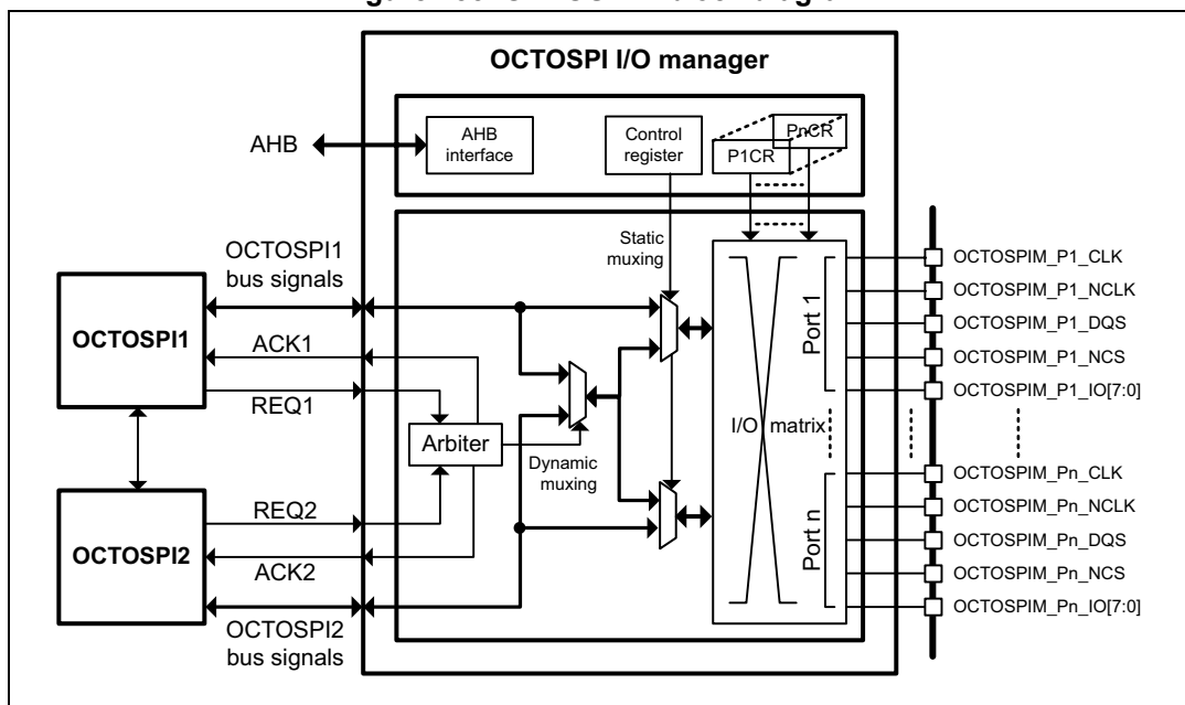
Figure 155. OCTOSPIM block diagram
