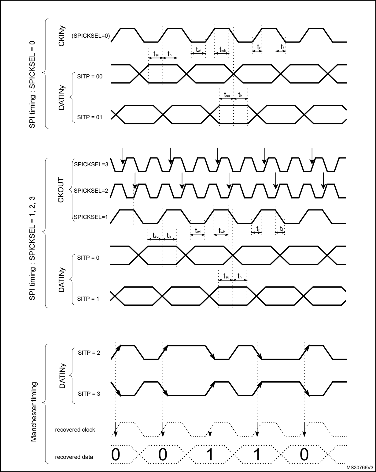
Figure 255. Channel transceiver timing diagrams
