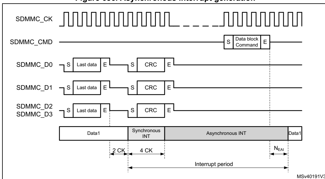
Figure 686. Asynchronous interrupt generation
