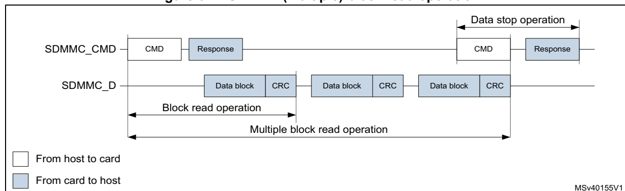
Figure 672. SDMMC (multiple) block read operation
