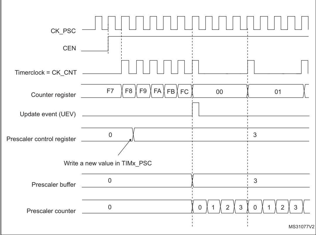
Figure 490. Counter timing diagram with prescaler division change from 1 to 4
