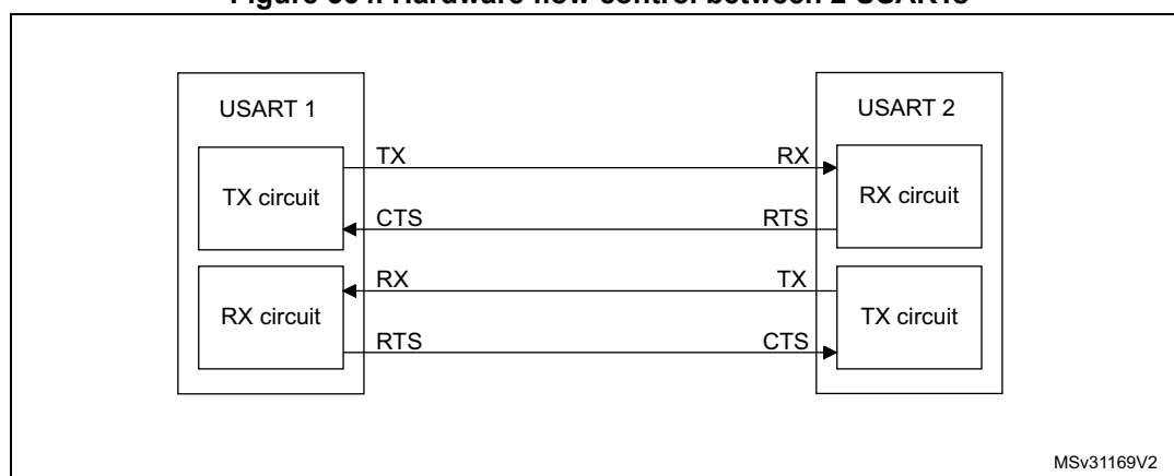
Figure 564. Hardware flow control between 2 USARTs
