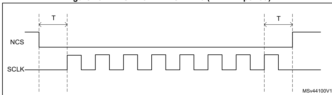
Figure 151. NCS when CKMODE = 0 ( T = \text{CLK period} )
