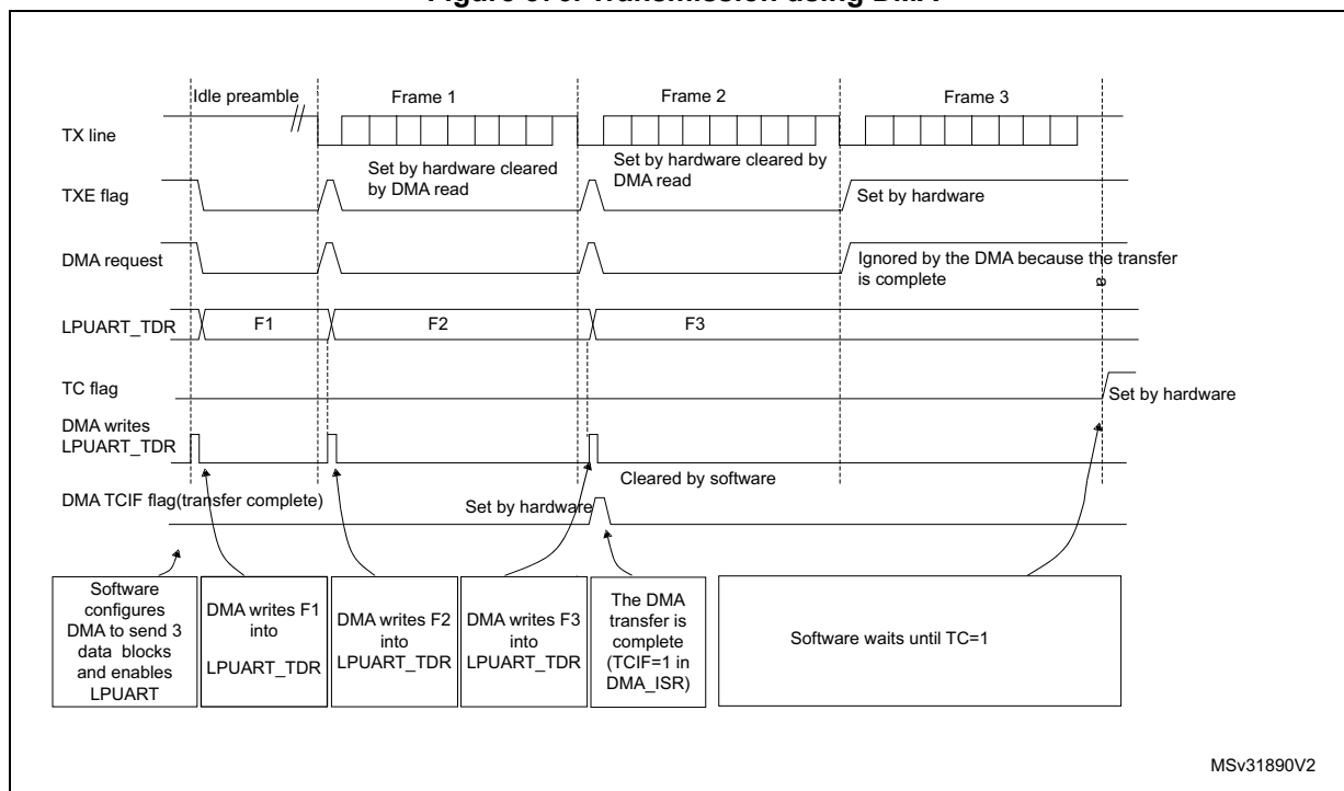
Figure 576. Transmission using DMA
