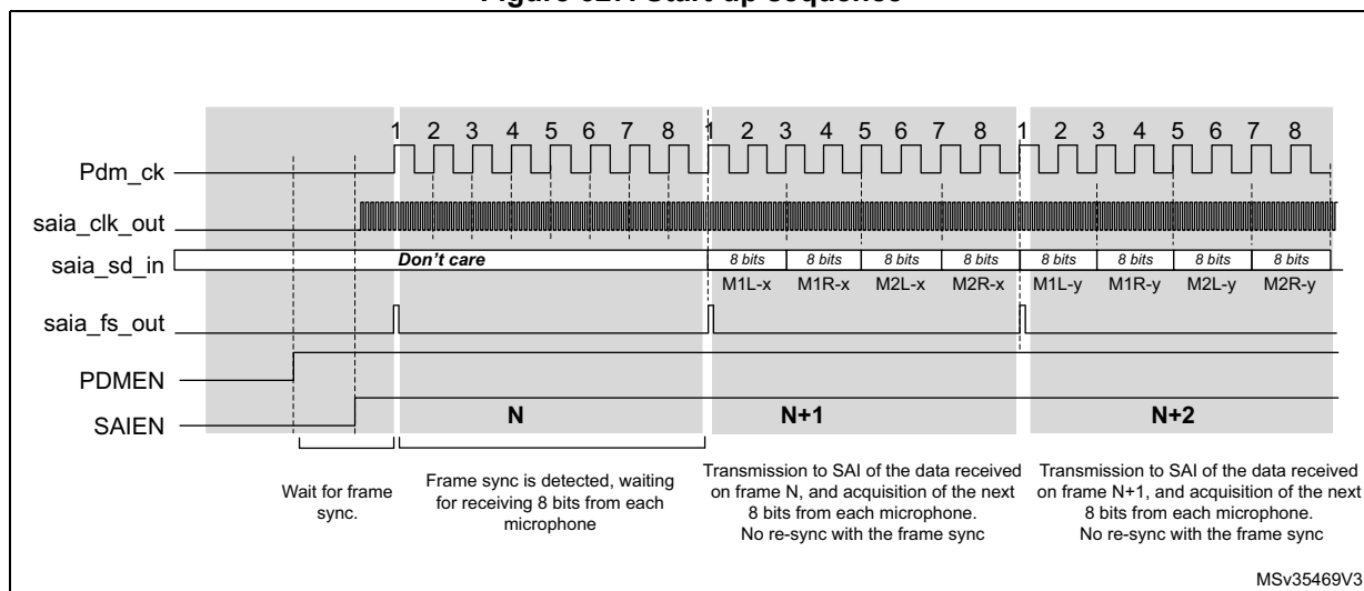
Figure 627. Start-up sequence
