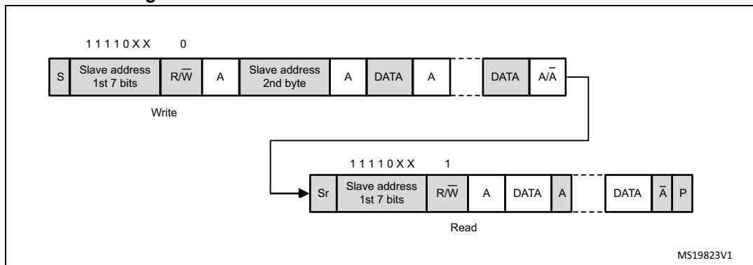
Figure 527. 10-bit address read access with HEAD10R = 1
