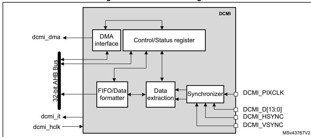
Figure 261. DCMI block diagram
