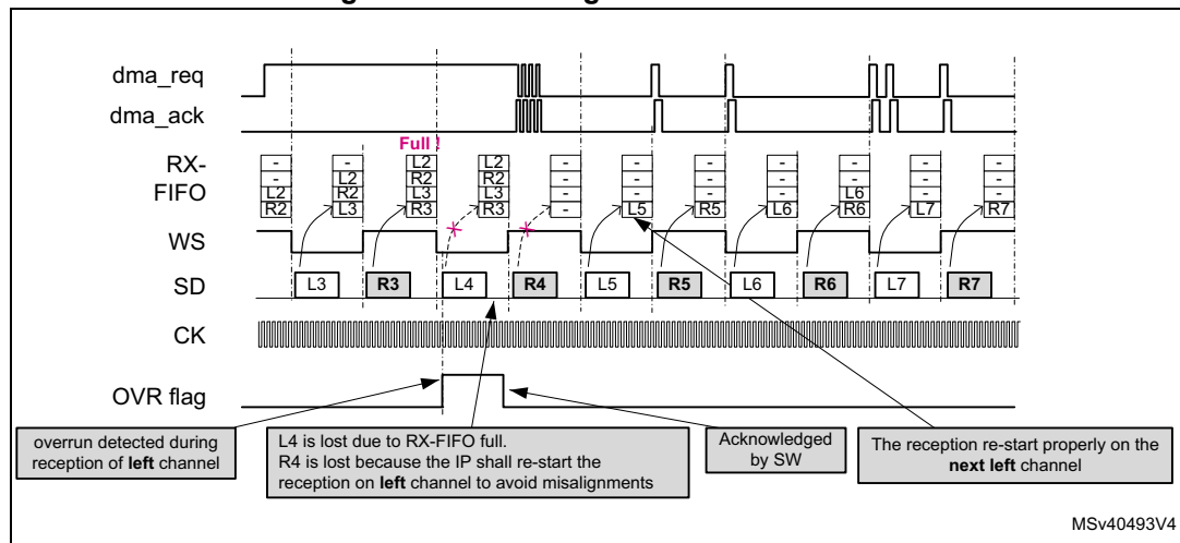
Figure 615. Handling of overrun situation
