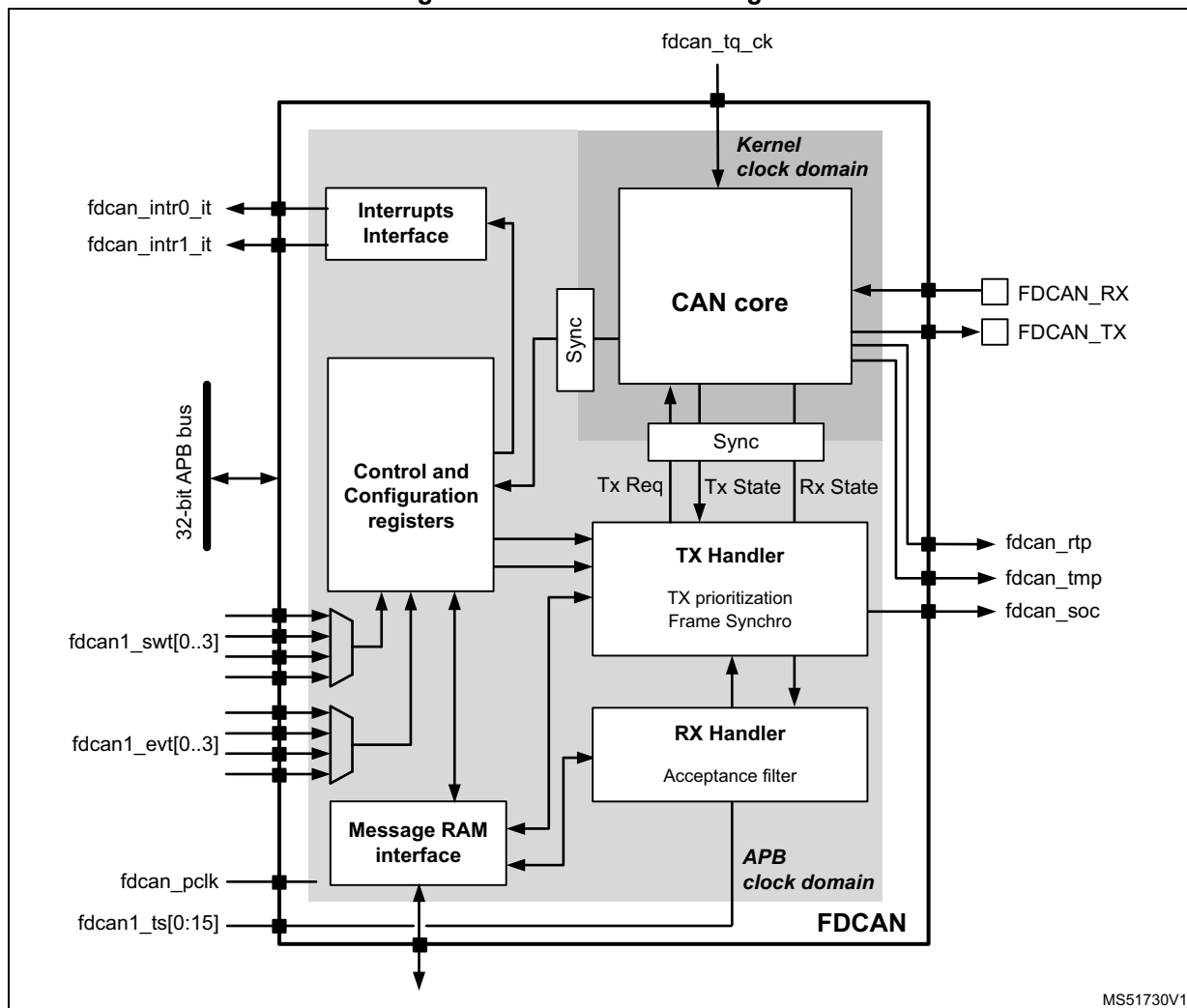
Figure 705. FDCAN block diagram
