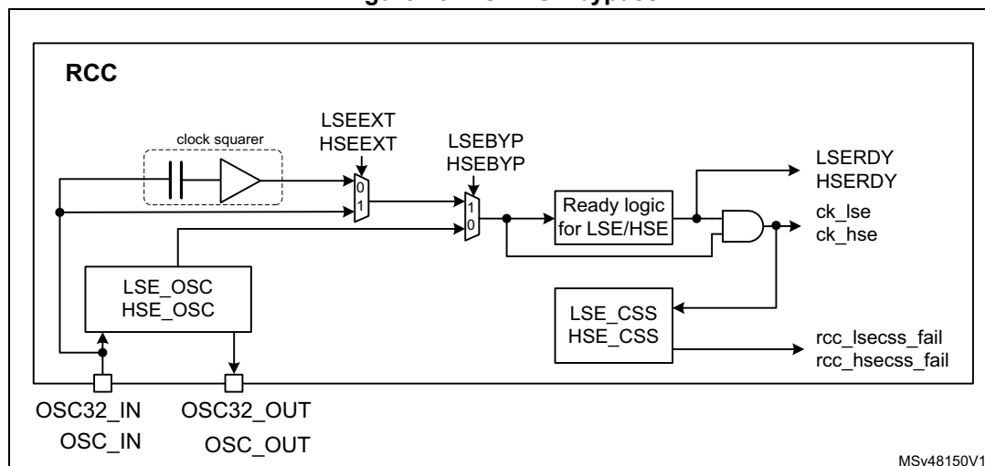
Figure 49. HSE/LSE bypass
