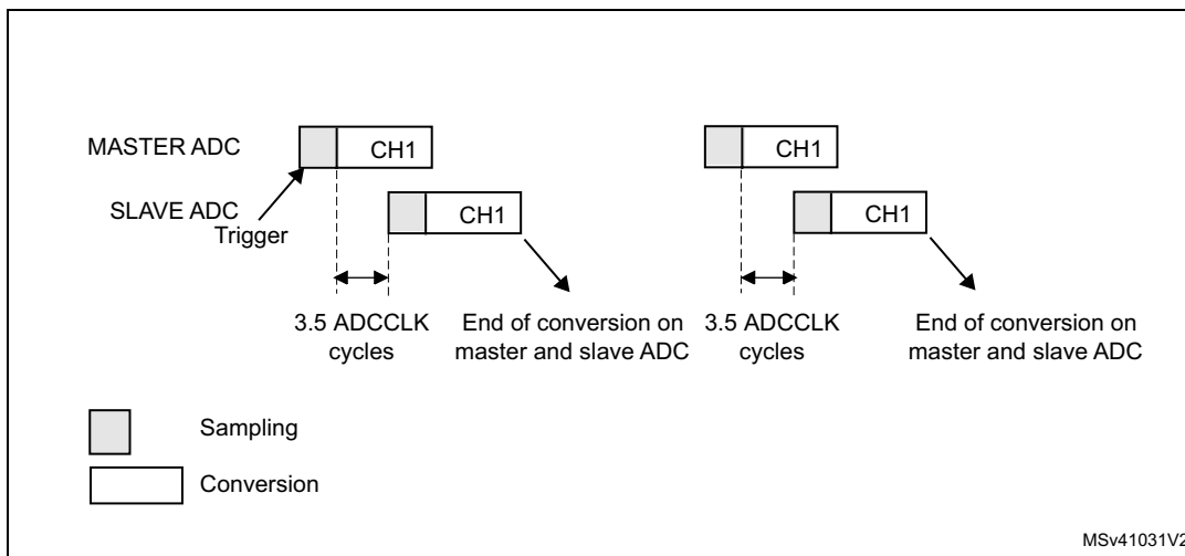
Figure 212. Interleaved mode on 1 channel in single conversion mode: dual ADC mode
