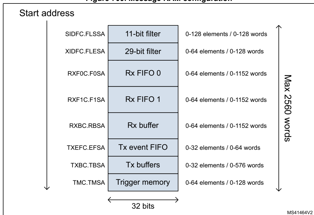
Figure 709. Message RAM configuration
