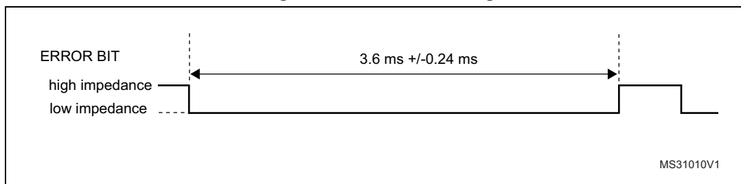
Figure 759. Error bit timing
