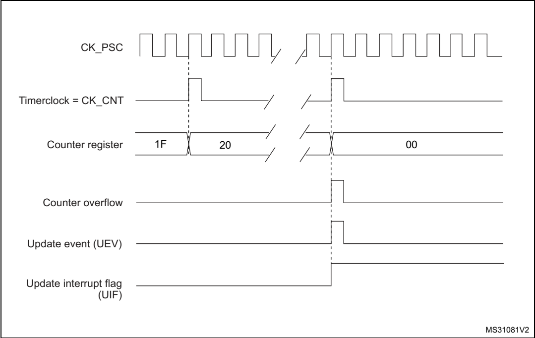
Figure 323. Counter timing diagram, internal clock divided by N
