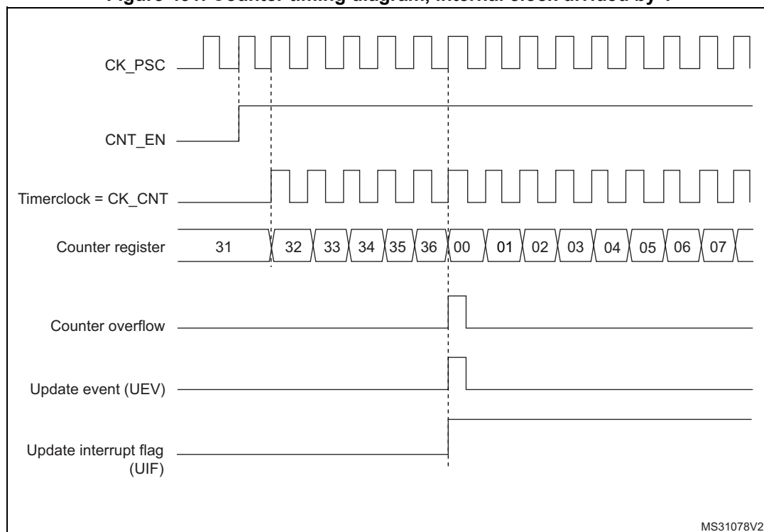
Figure 431. Counter timing diagram, internal clock divided by 1
