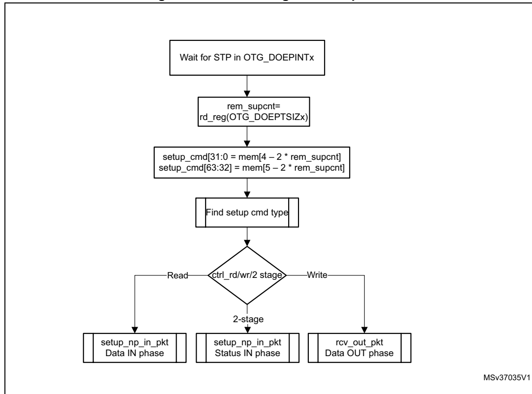
Figure 745. Processing a SETUP packet
