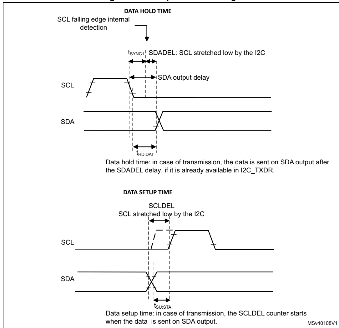
Figure 513. Setup and hold timings
