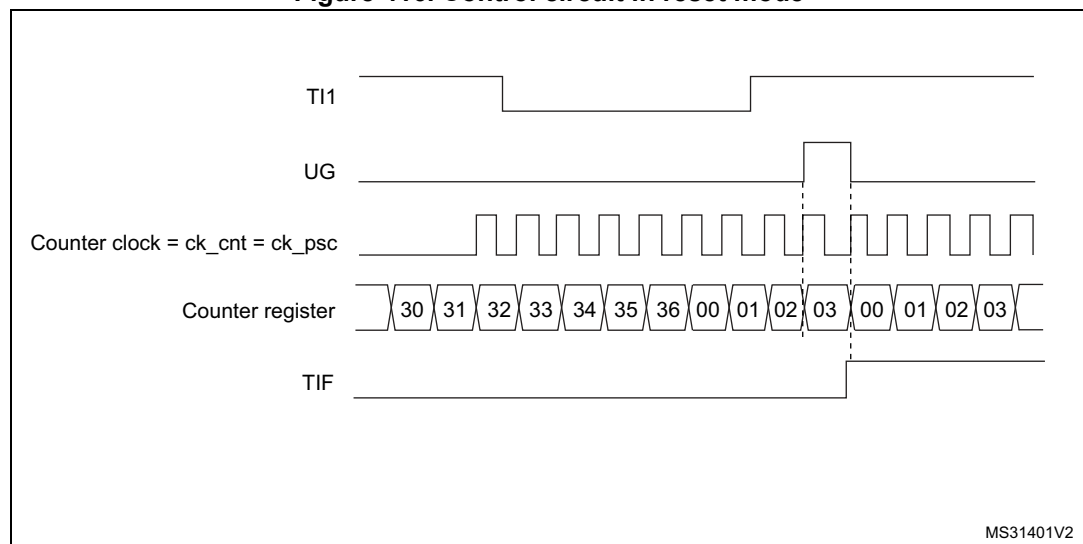
Figure 416. Control circuit in reset mode
