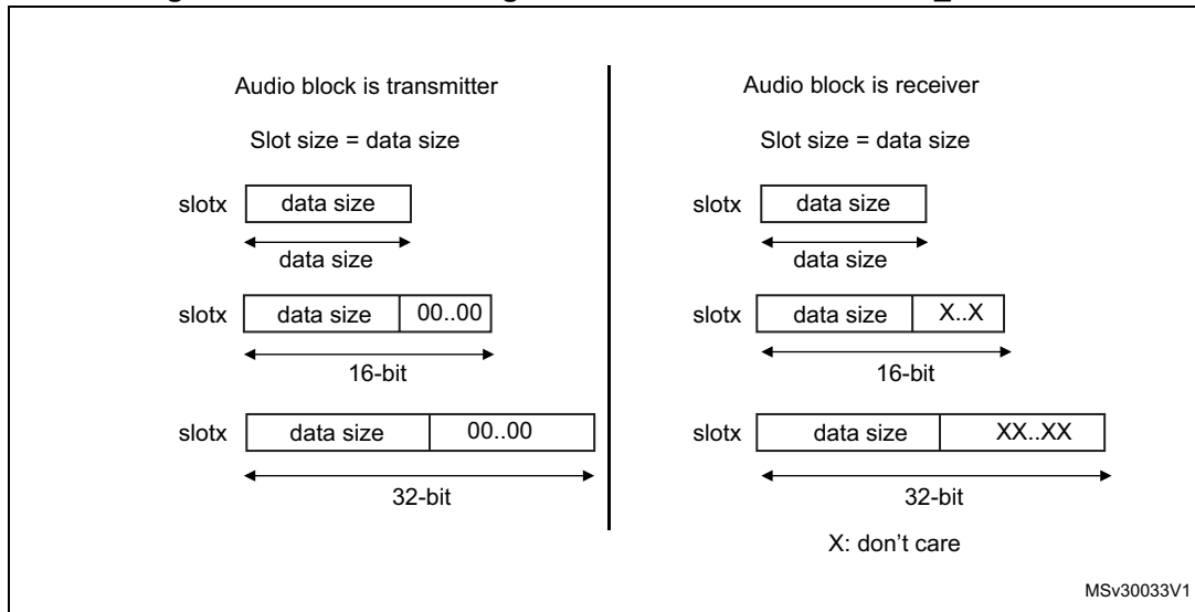
Figure 622. Slot size configuration with FBOFF = 0 in SAI_xSLOTR
