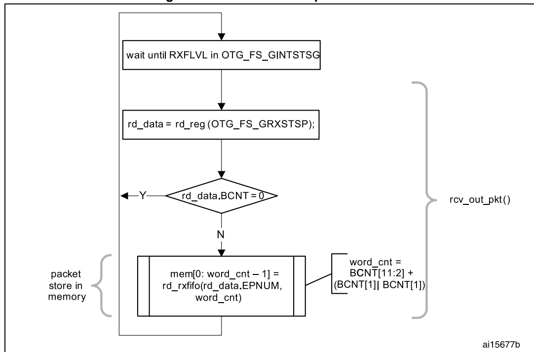
Figure 744. Receive FIFO packet read
