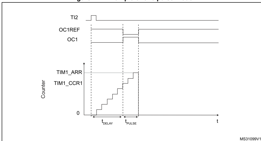
Figure 447. Example of one pulse mode.
