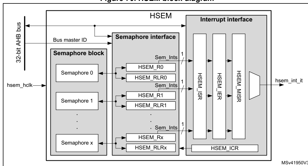
Figure 70. HSEM block diagram
