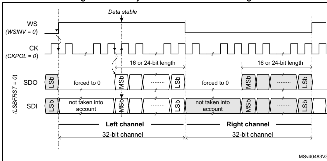
Figure 605. LSB justified 16 or 24-bit data length
