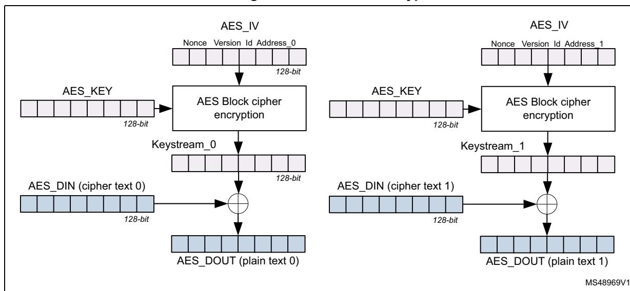
Figure 314. AES CTR decryption flow
