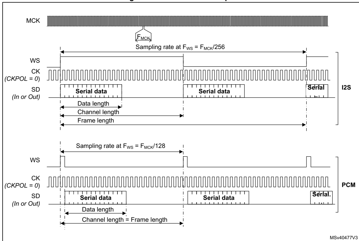
Figure 599. Waveform examples
