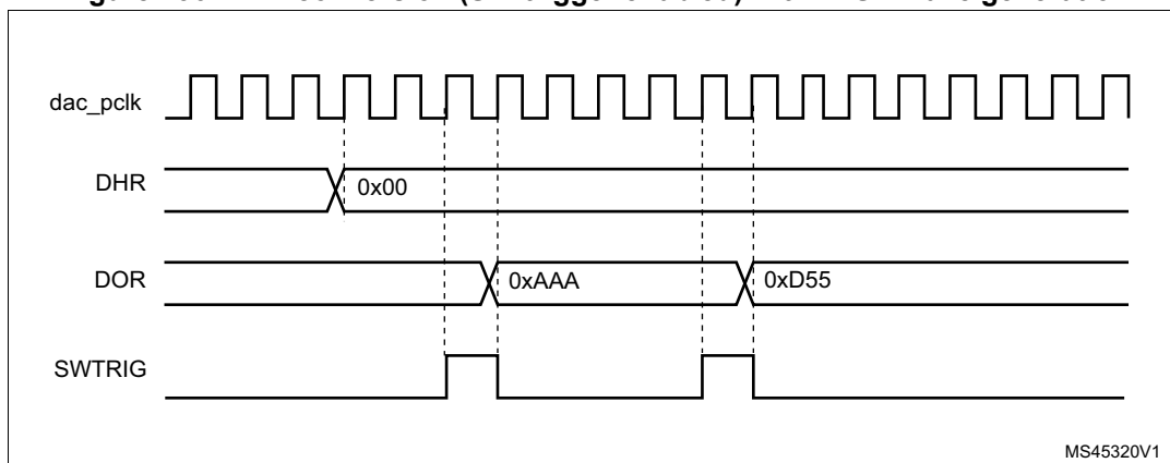
Figure 236. DAC conversion (SW trigger enabled) with LFSR wave generation
