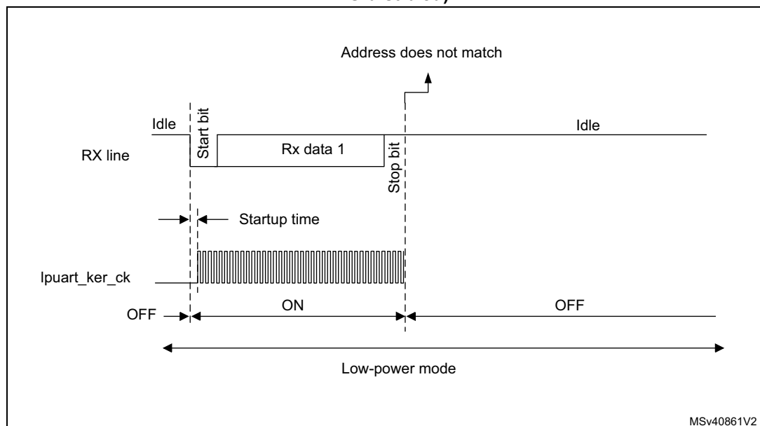
Figure 582. Wake-up event not verified (wake-up event = address match, FIFO disabled)
