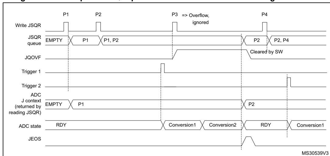
Figure 173. Example of JSQR queue of context with overflow during conversion
