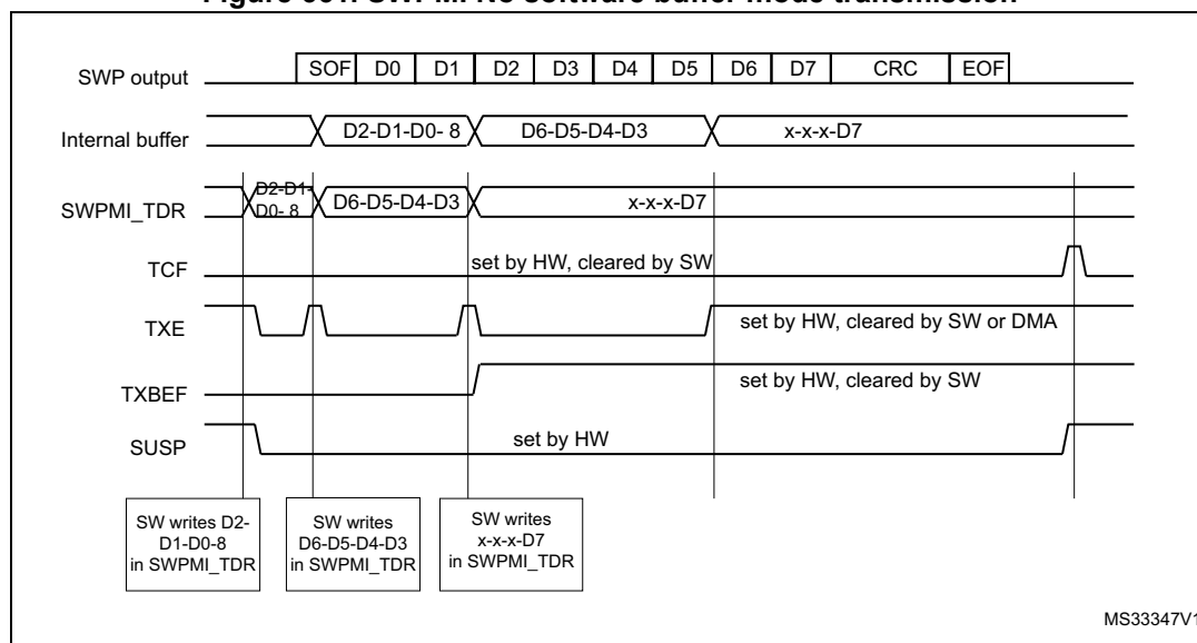
Figure 661. SWPMI No software buffer mode transmission
