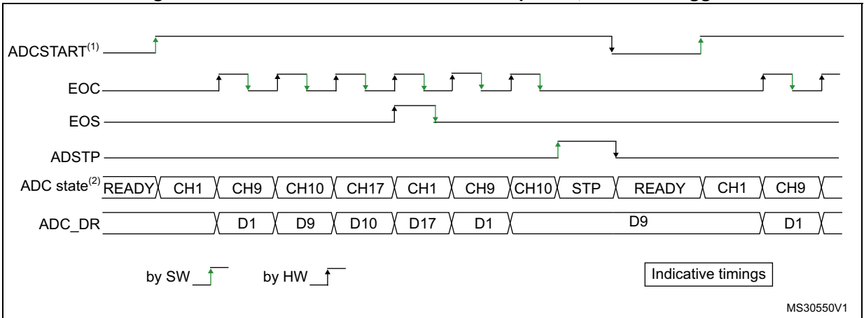
Figure 183. Continuous conversion of a sequence, software trigger
