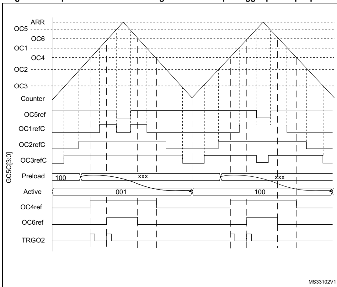
Figure 356. 3-phase combined PWM signals with multiple trigger pulses per period
