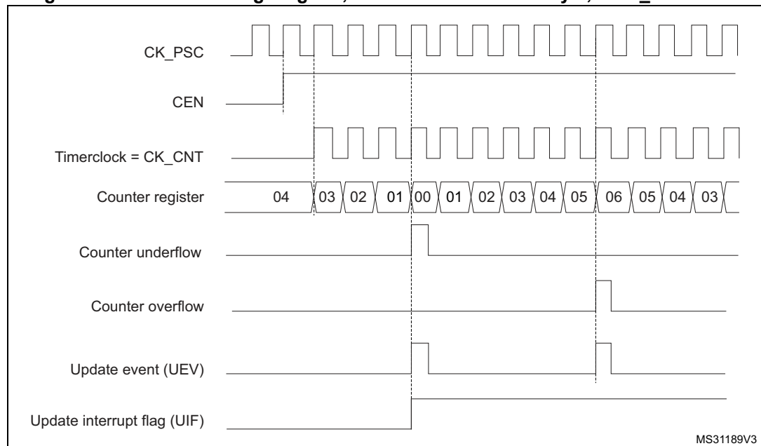
Figure 331. Counter timing diagram, internal clock divided by 1, TIMx_ARR = 0x6
