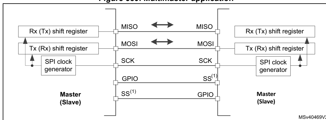
Figure 589. Multimaster application
