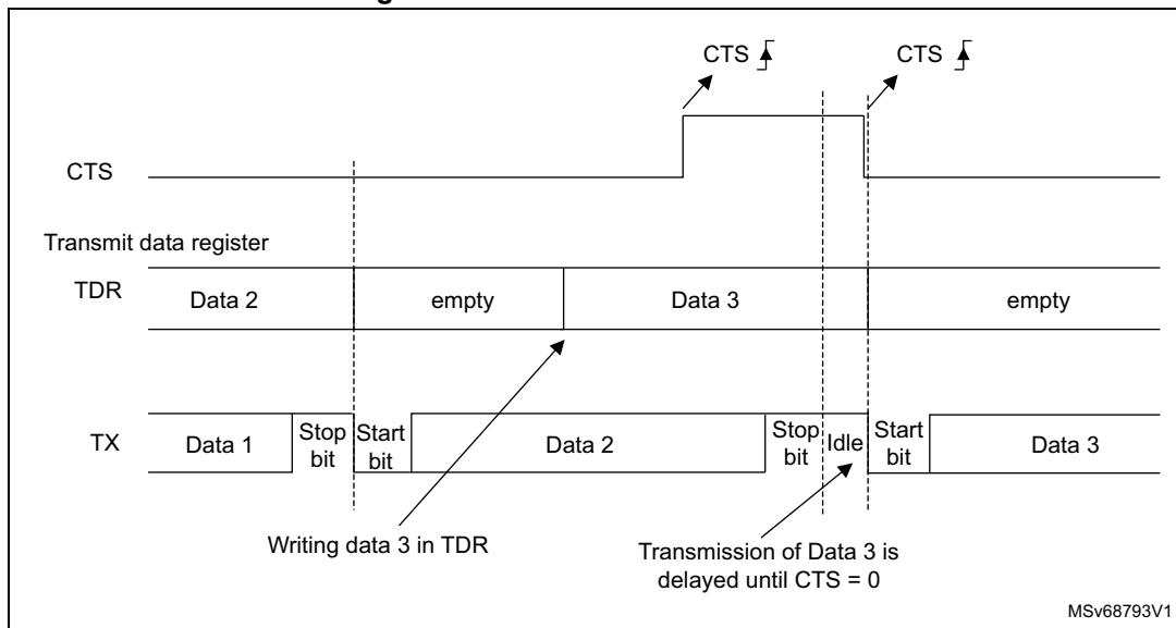
Figure 566. RS232 CTS flow control
