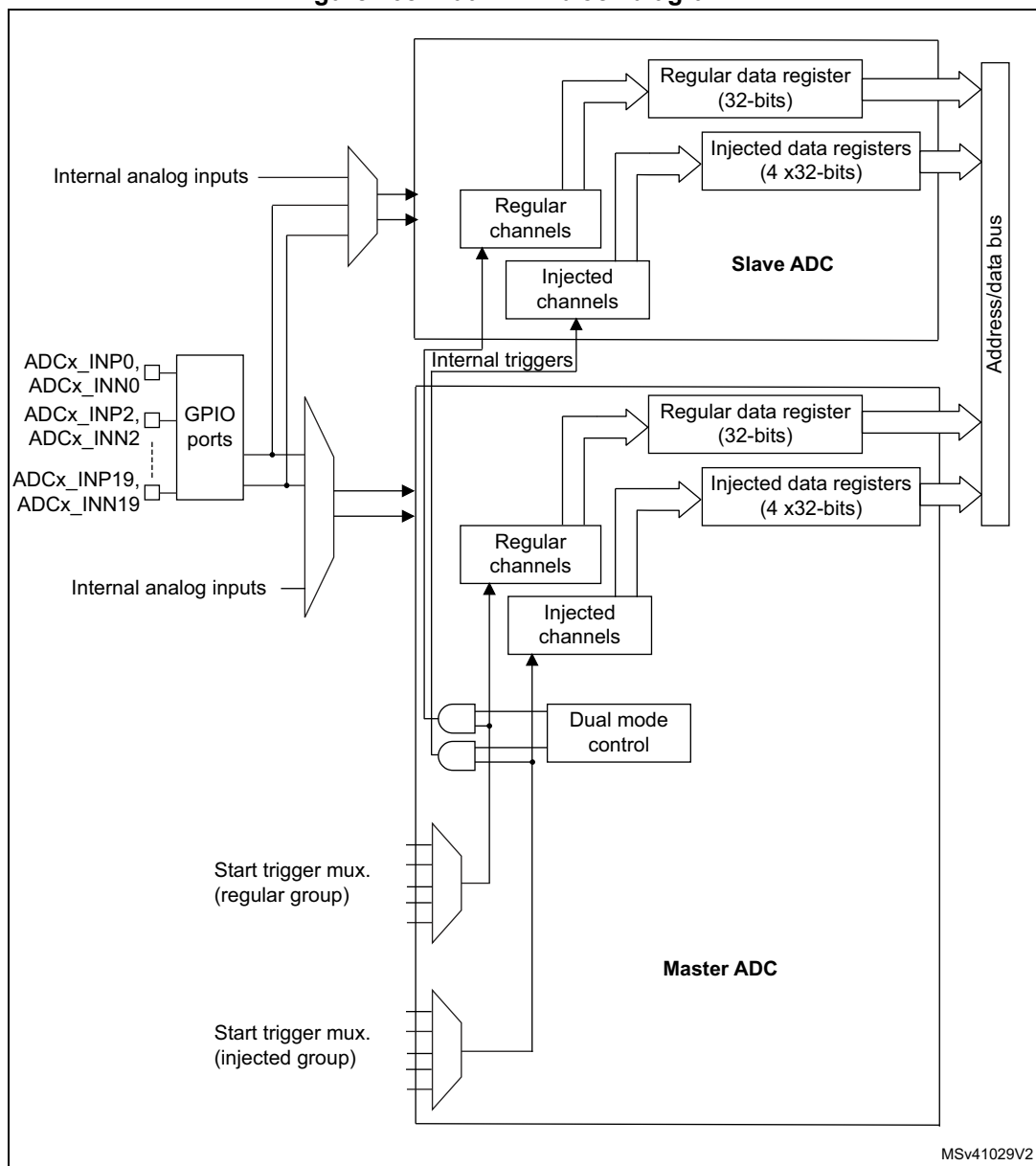
Figure 208. Dual ADC block diagram (1)
