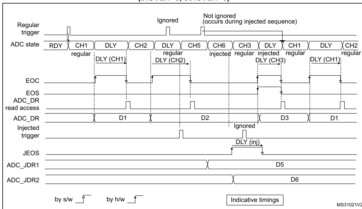
Figure 193. AUTDLY=1, regular HW conversions interrupted by injected conversions (DISCEN=0; JDISCEN=0)
