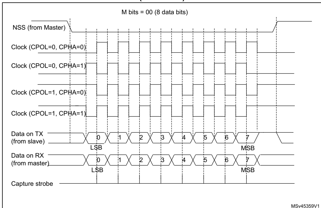
Figure 557. USART data clock timing diagram in synchronous slave mode (M bits = 00)
