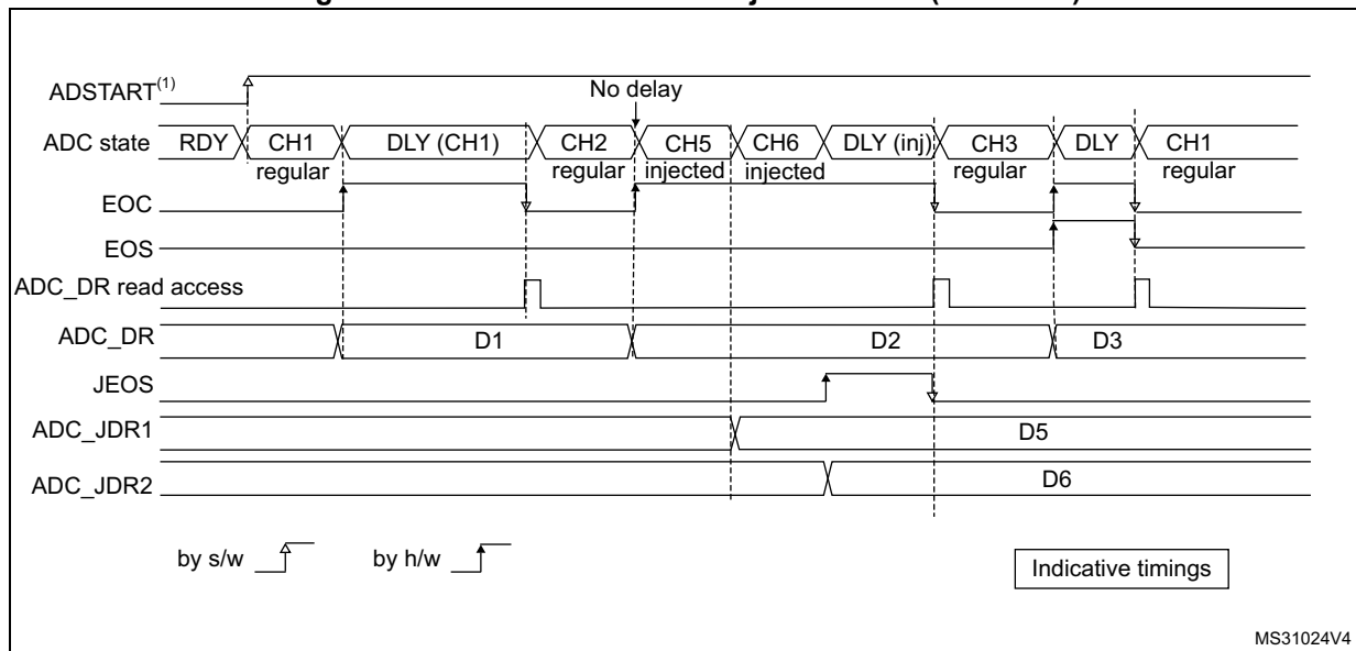
Figure 196. AUTDLY=1 in auto-injected mode ( JAUTO=1 )
