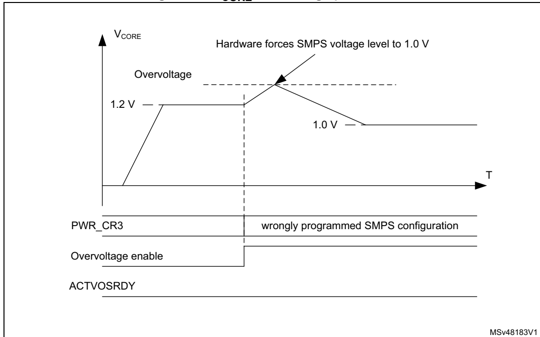
Figure 33. V_{\text{CORE}} overvoltage protection
