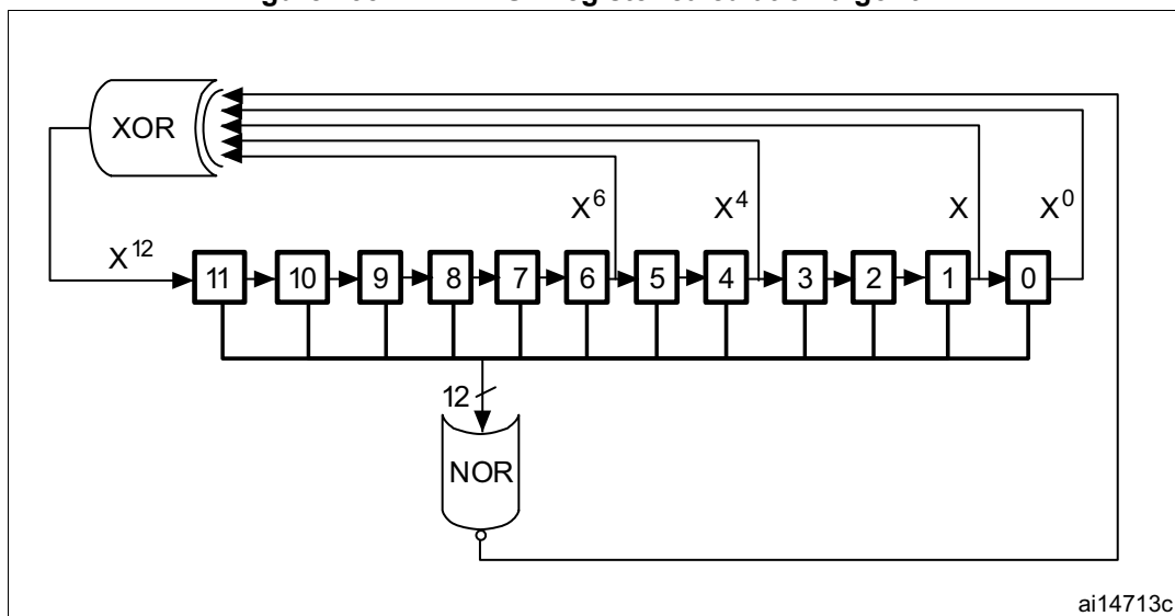
Figure 235. DAC LFSR register calculation algorithm
