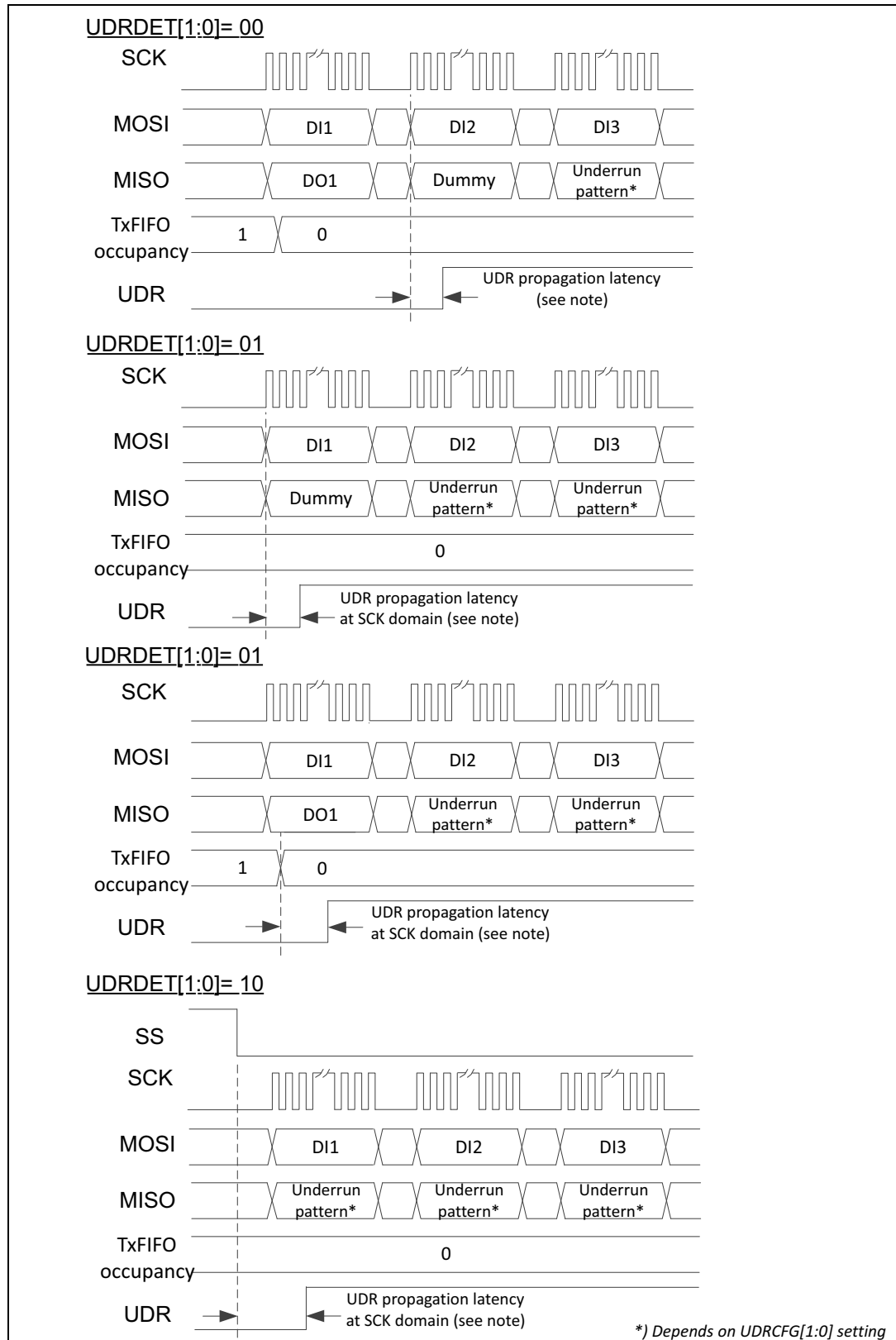
Figure 597. Optional configurations of slave behavior at detection of underrun condition
