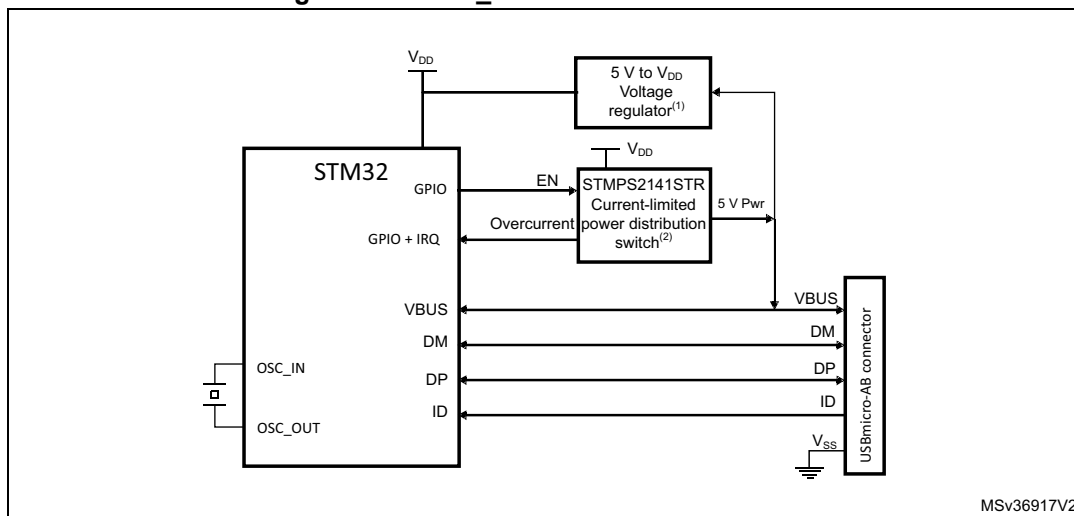
Figure 722. OTG_HS A-B device connection
