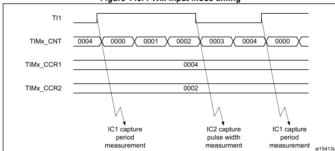
Figure 443. PWM input mode timing
