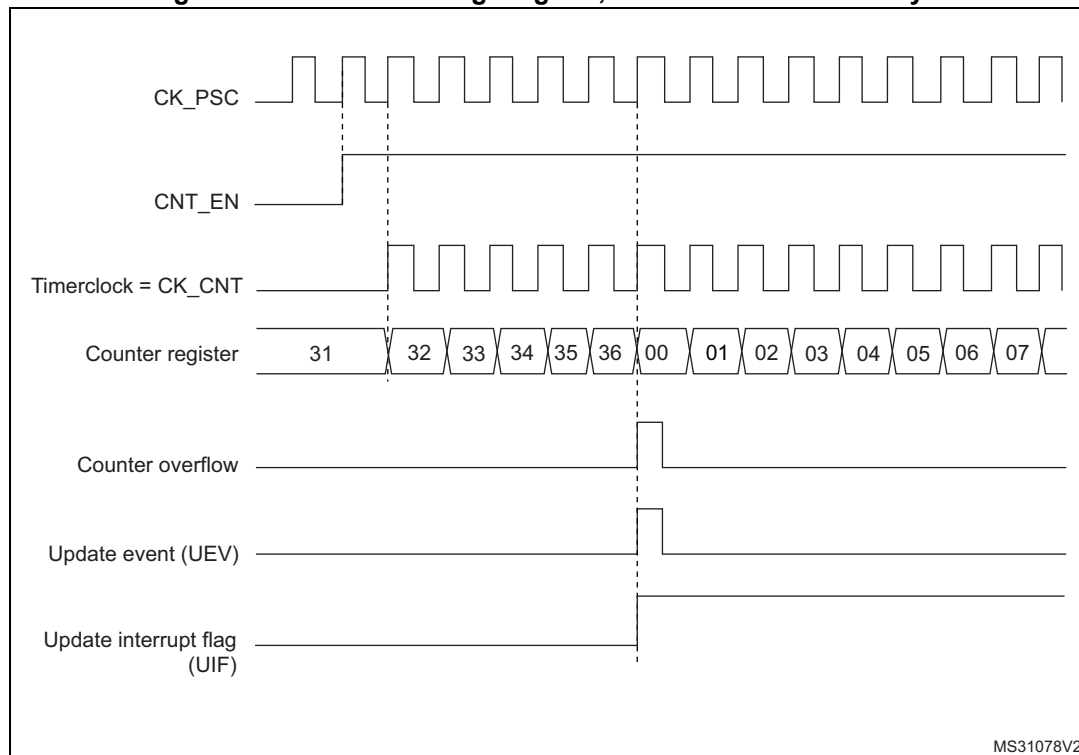
Figure 491. Counter timing diagram, internal clock divided by 1
