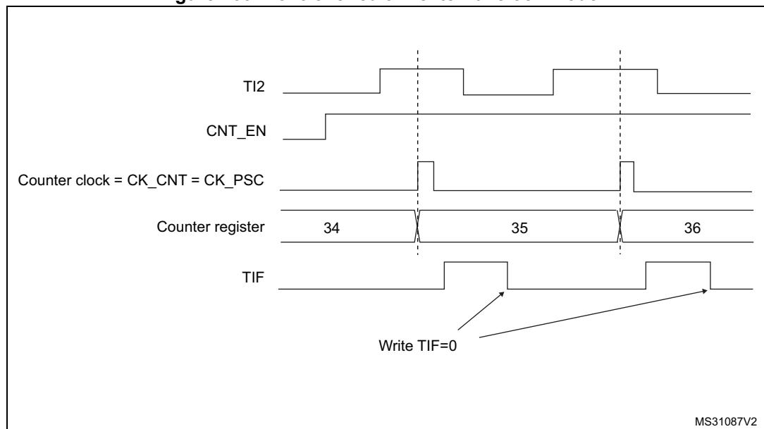
Figure 466. Control circuit in external clock mode 1
