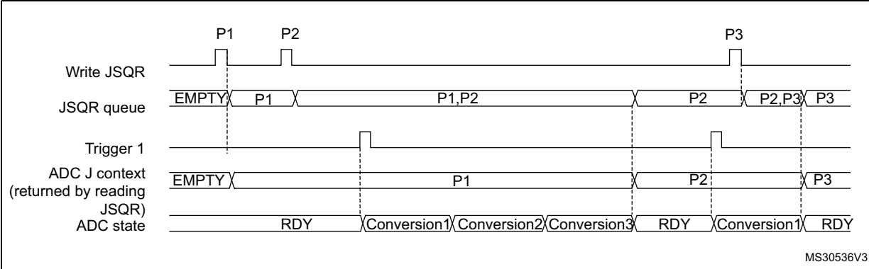
Figure 170. Example of JSQR queue of context (sequence change)
