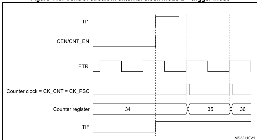
Figure 419. Control circuit in external clock mode 2 + trigger mode
