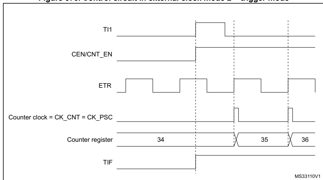
Figure 376. Control circuit in external clock mode 2 + trigger mode
