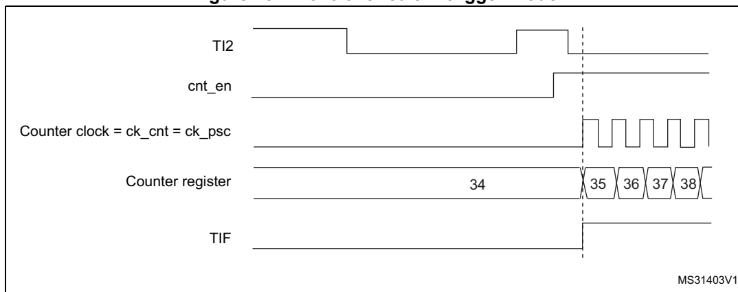
Figure 487. Control circuit in trigger mode
