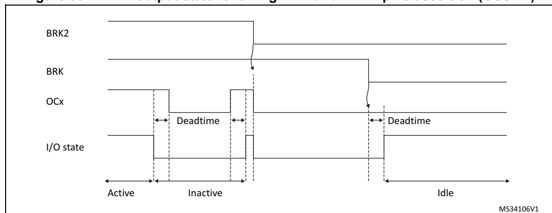
Figure 362. PWM output state following BRK and BRK2 pins assertion (OSSl=1)
