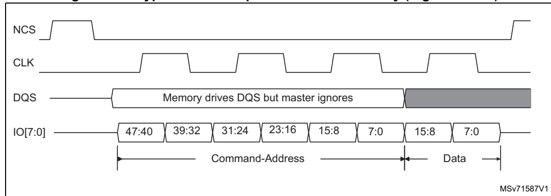
Figure 147. HyperBus write operation with no latency (register write)
