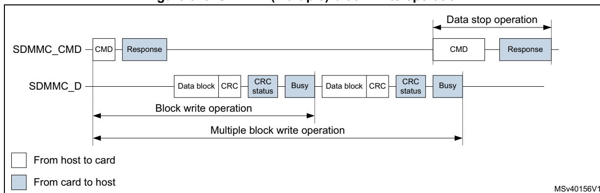
Figure 673. SDMMC (multiple) block write operation
