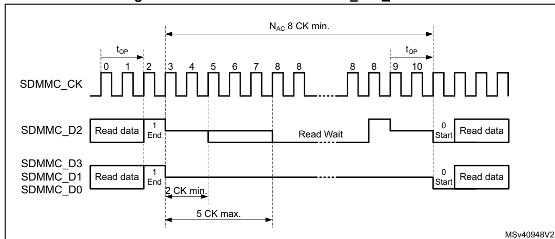
Figure 694. Read Wait with SDMMC_CK \geq 50 MHz
