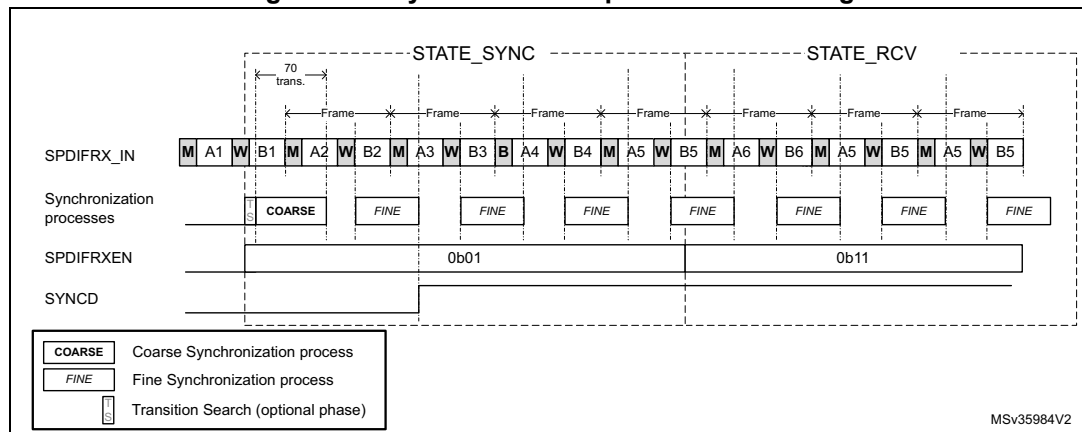
Figure 649. Synchronization process scheduling
