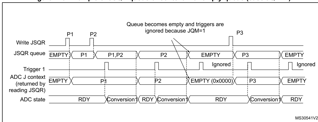
Figure 175. Example of JSQR queue of context with empty queue (case JQM=1)
