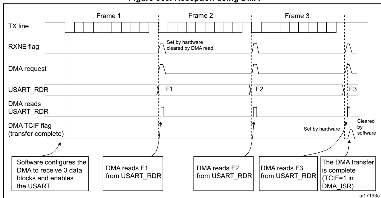
Figure 563. Reception using DMA
