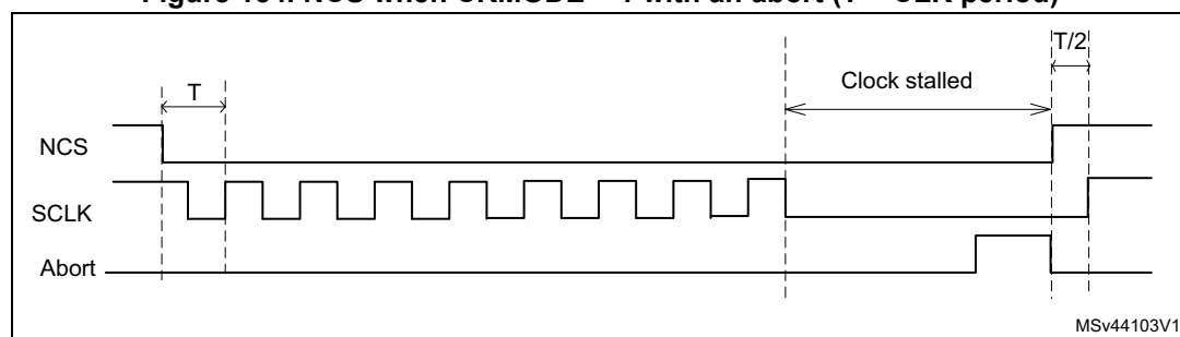
Figure 154. NCS when CKMODE = 1 with an abort ( T = \text{CLK period} )
