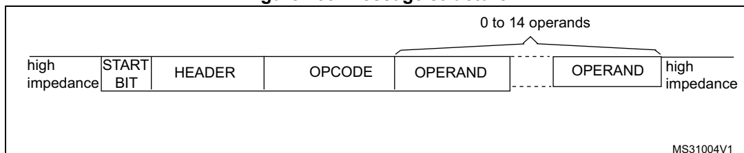
Figure 753. Message structure
