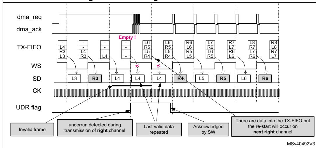
Figure 614. Handling of underrun situation
