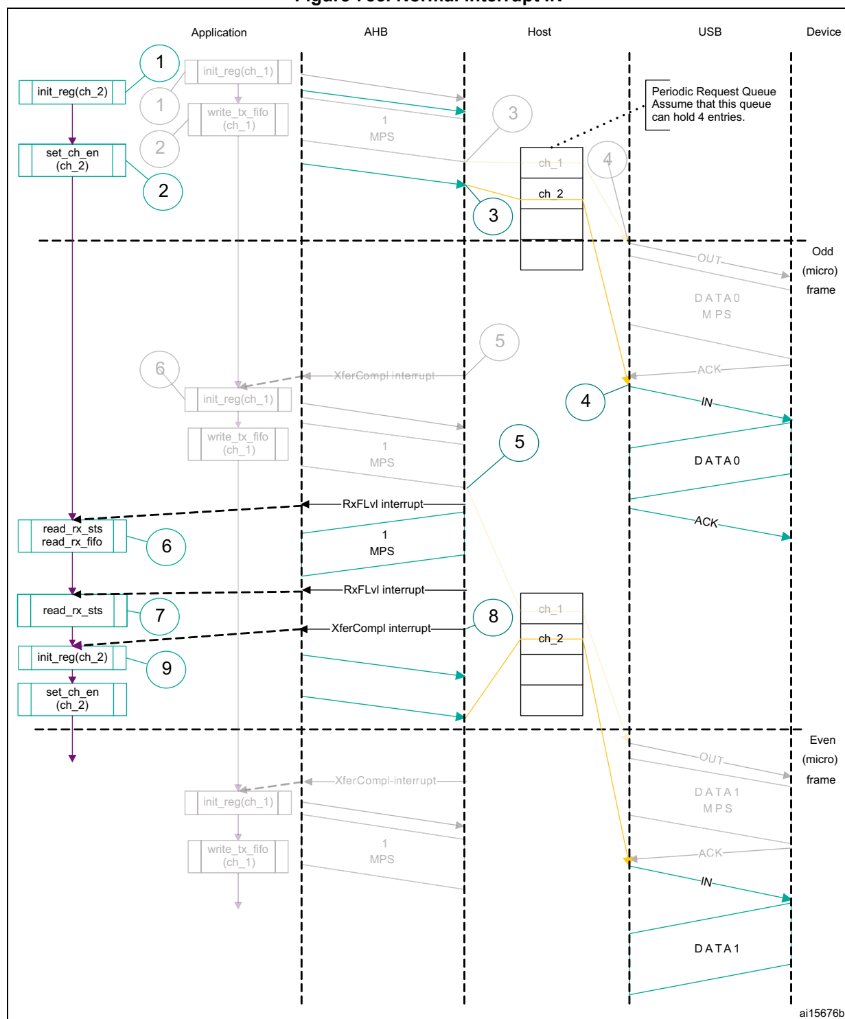
Figure 735. Normal interrupt IN
