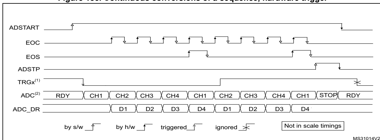
Figure 185. Continuous conversions of a sequence, hardware trigger
