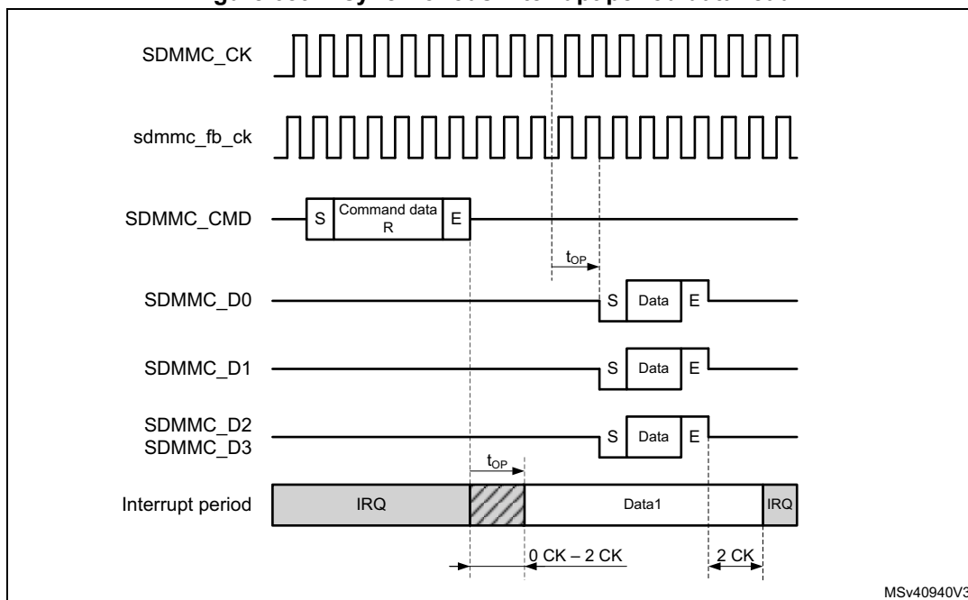
Figure 689. Asynchronous interrupt period data read
