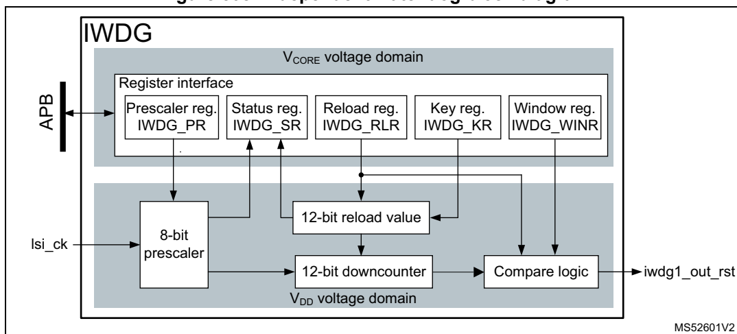
Figure 508. Independent watchdog block diagram
