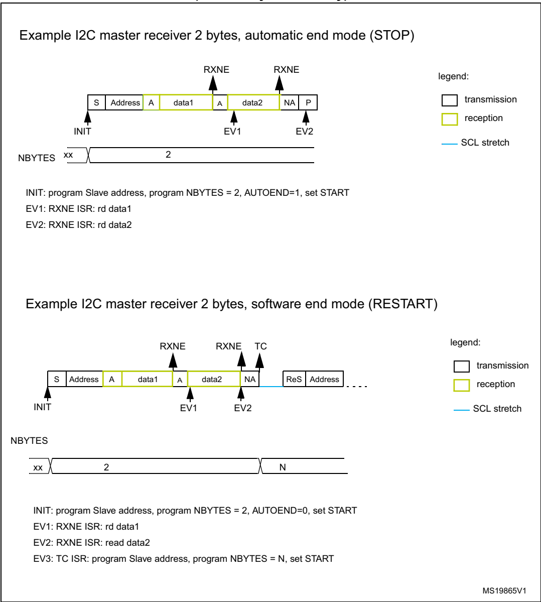
Figure 533. Transfer bus diagrams for I2C master receiver (mandatory events only)
