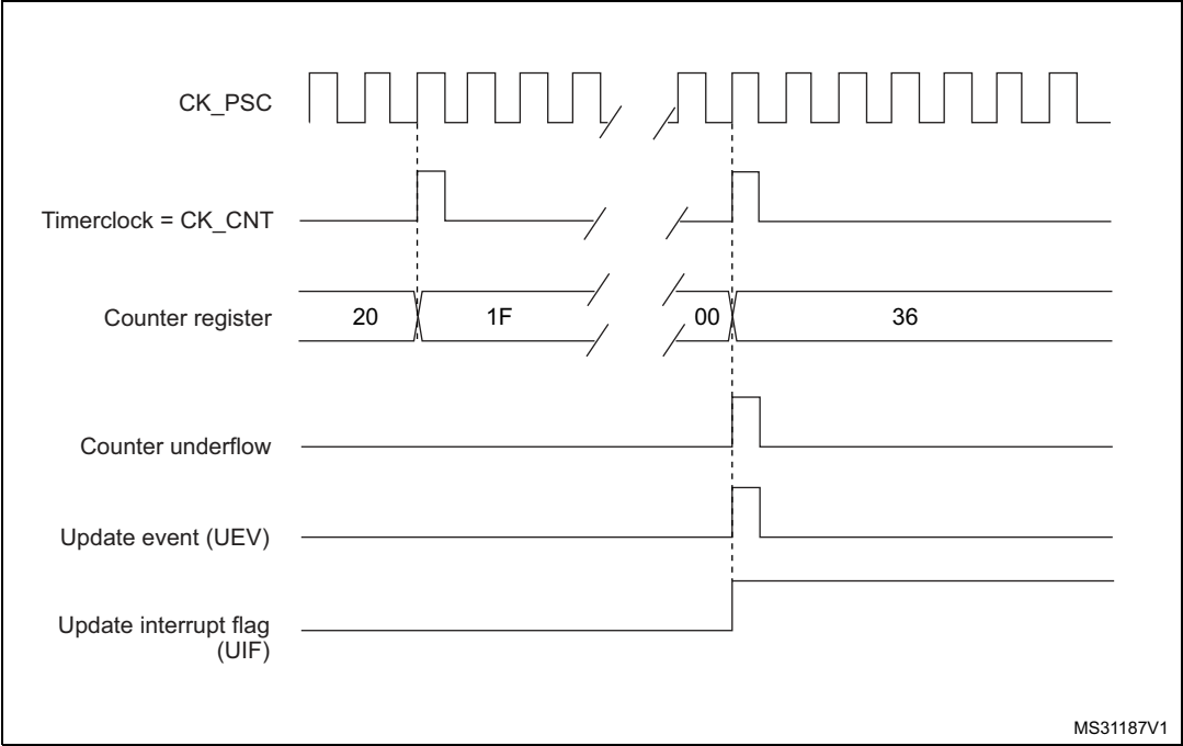
Figure 389. Counter timing diagram, internal clock divided by N
