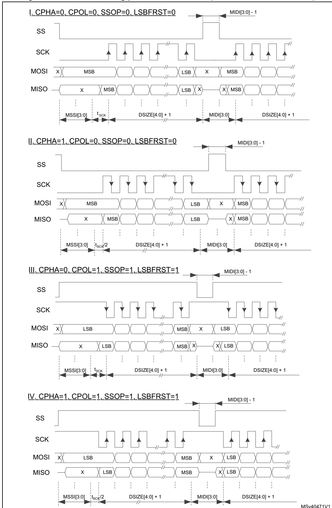
Figure 592. SS interleaving pulses between data (SSOE=1, SSOM=1,SSM=0)
