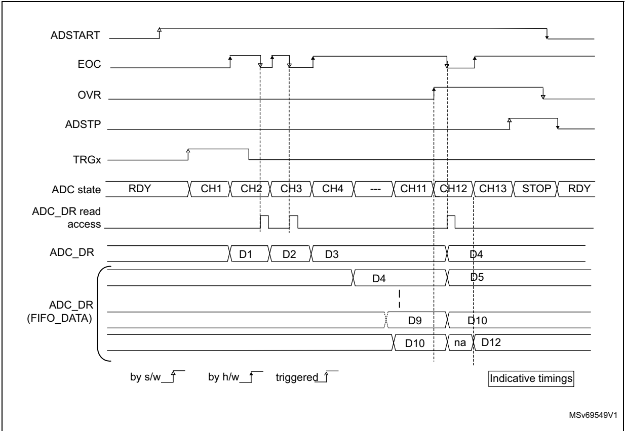
Figure 190. Example of overrun (OVRMOD = 0)
