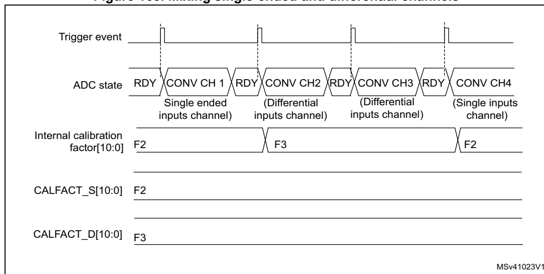
Figure 163. Mixing single-ended and differential channels
