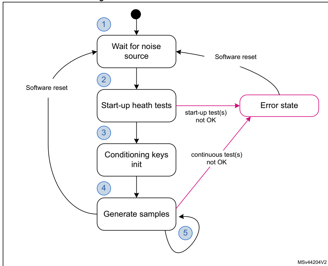
Figure 284. RNG initialization overview
