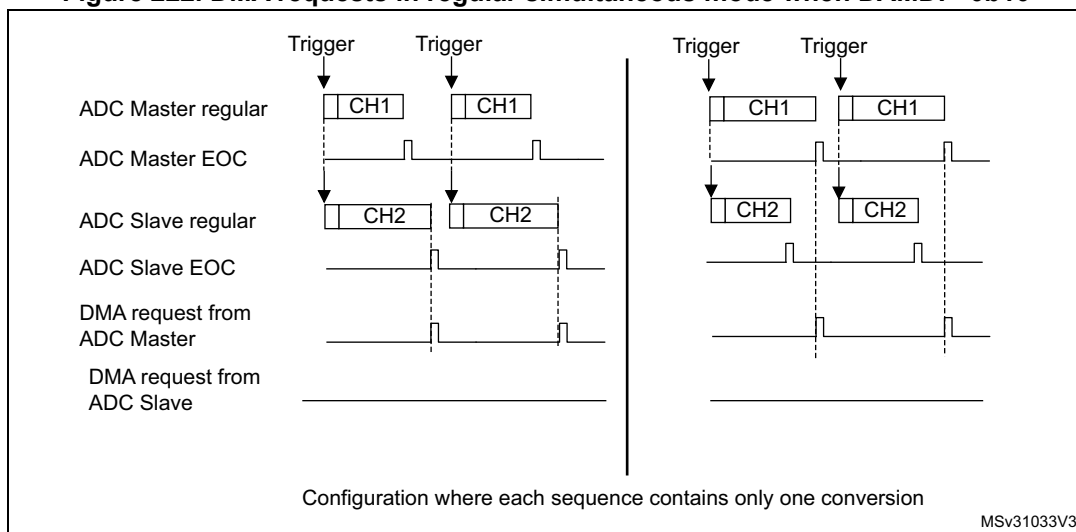
Figure 222. DMA requests in regular simultaneous mode when DAMDF=0b10
