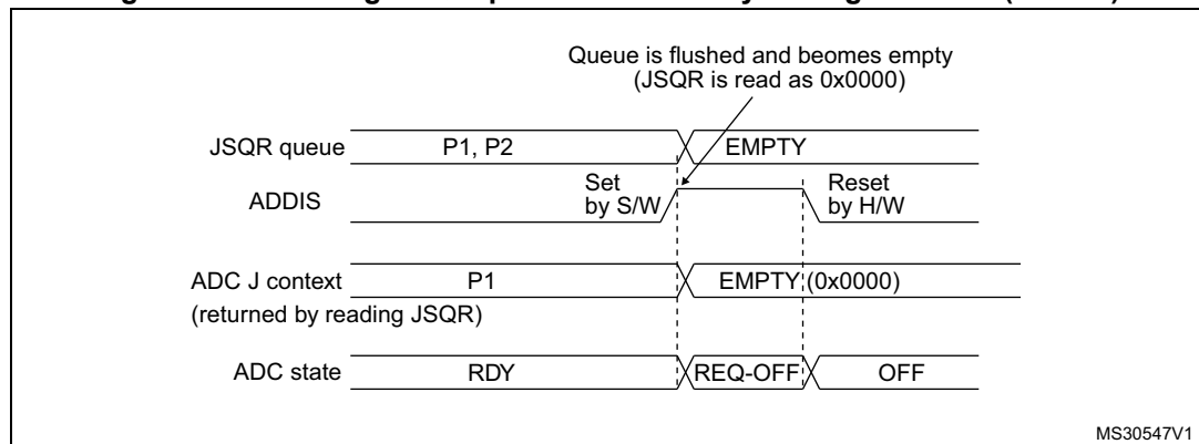
Figure 181. Flushing JSQR queue of context by setting ADDIS=1 (JQM=1)
