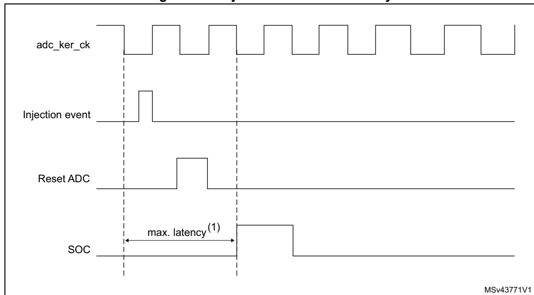
Figure 169. Injected conversion latency
