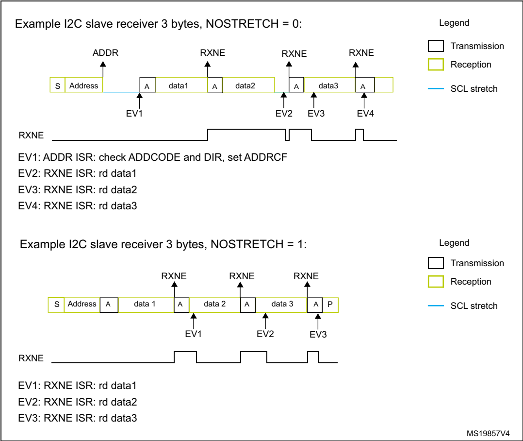
Figure 523. Transfer bus diagrams for I2C slave receiver (mandatory events only)
