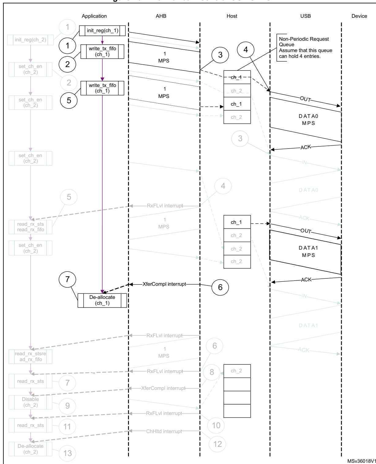
Figure 732. Normal bulk/control OUT/SETUP
