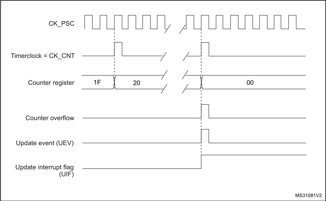
Figure 434. Counter timing diagram, internal clock divided by N
