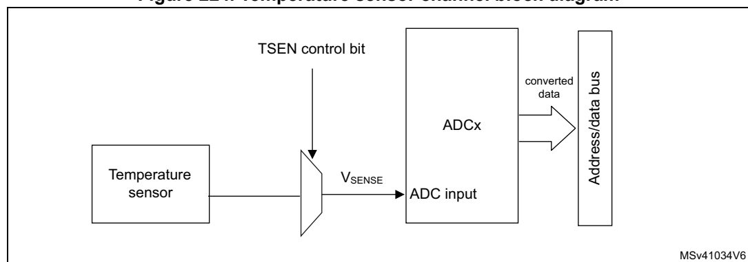
Figure 224. Temperature sensor channel block diagram
