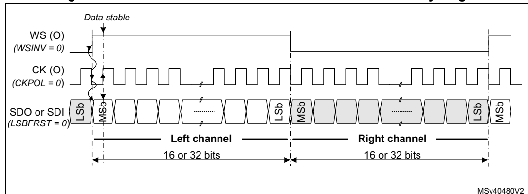
Figure 602. Master MSB Justified 16-bit or 32-bit full-accuracy length
