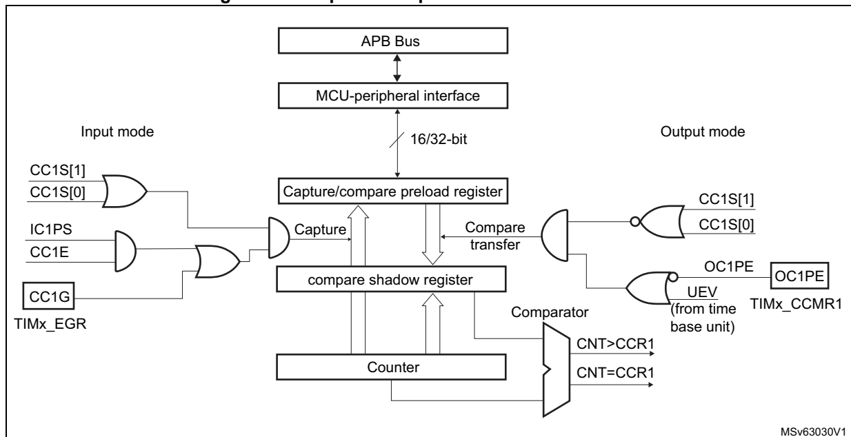
Figure 441. Capture/compare channel 1 main circuit
