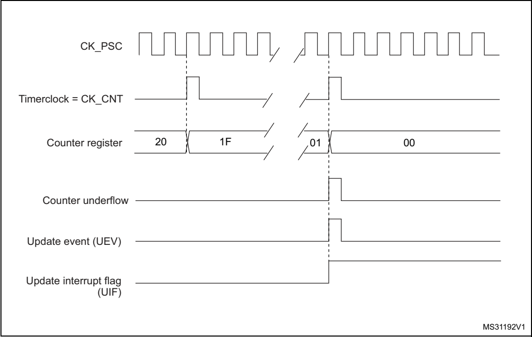
Figure 394. Counter timing diagram, internal clock divided by N
