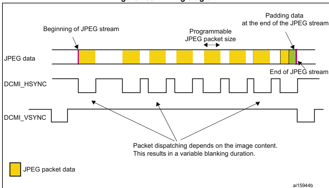
Figure 263. Timing diagram
