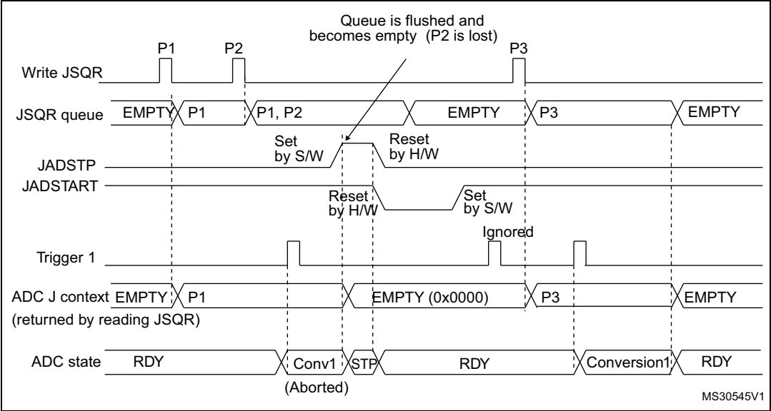
Figure 179. Flushing JSQR queue of context by setting JADSTP=1 (JQM=1)
