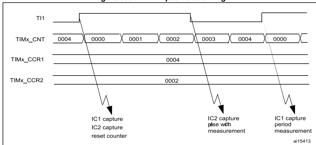
Figure 350. PWM input mode timing
