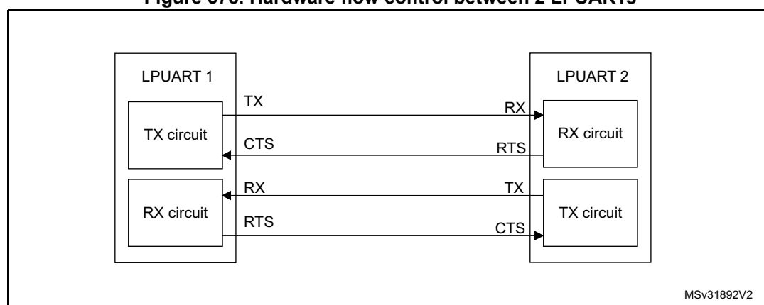
Figure 578. Hardware flow control between 2 LPUARTs
