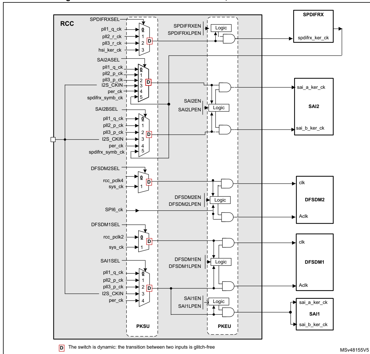
Figure 55. Kernel clock distribution for SAI1s, DFSDMs and SPDIFRX
