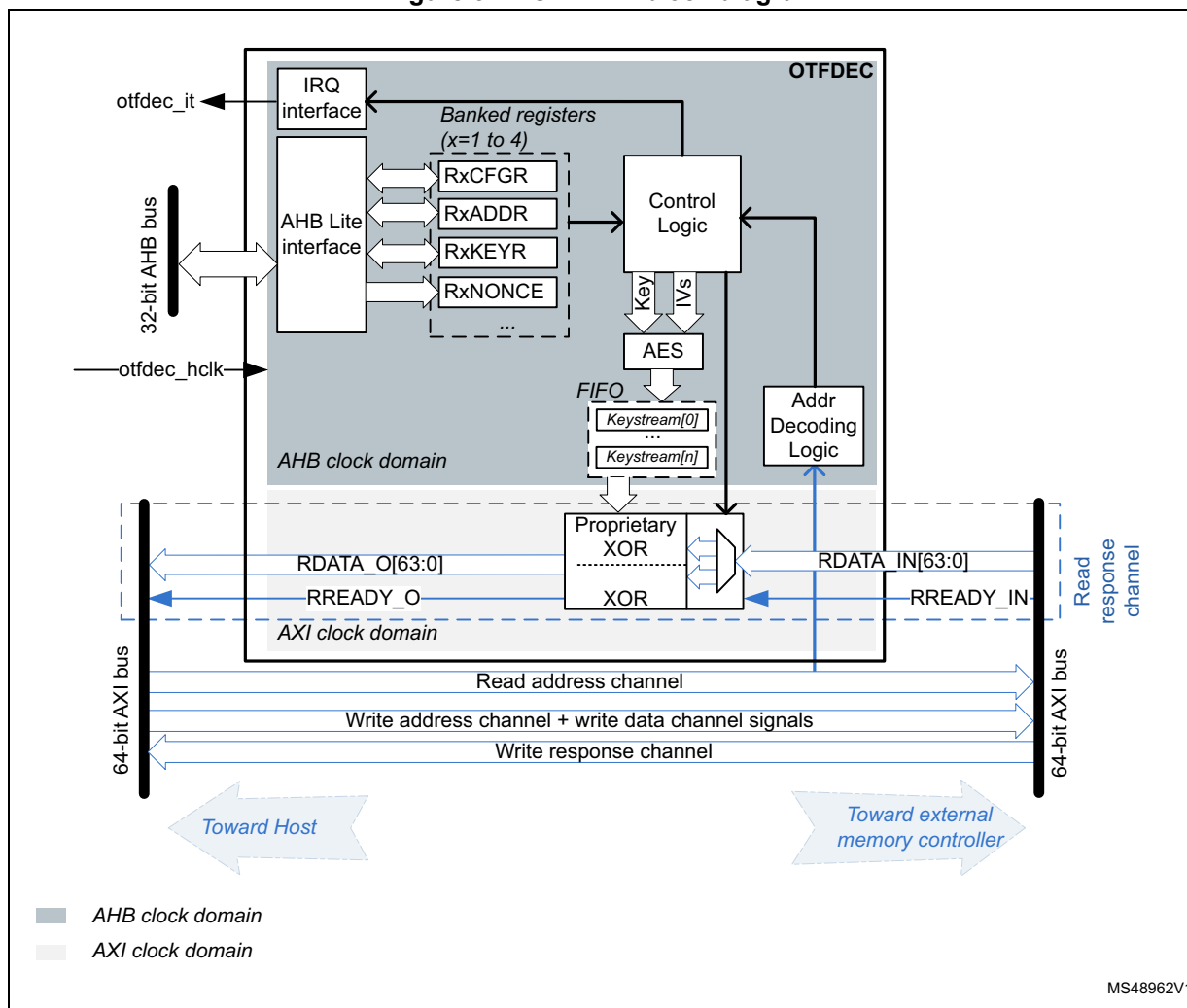
Figure 312. OTFDEC block diagram
