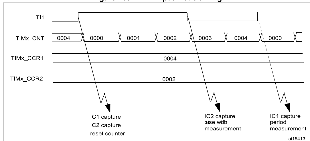
Figure 405. PWM input mode timing
