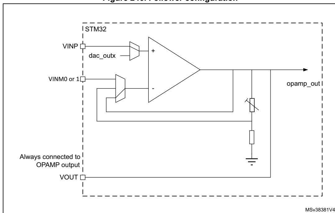
Figure 246. Follower configuration
