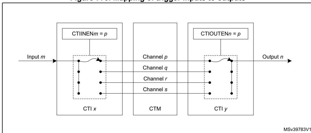
Figure 770. Mapping of trigger inputs to outputs
