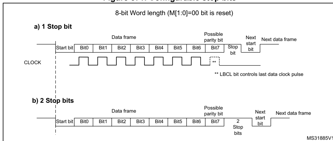
Figure 571. Configurable stop bits
