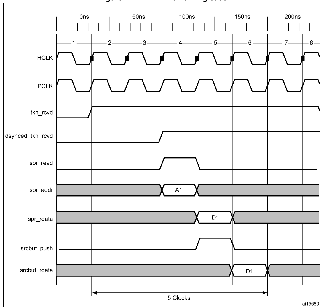
Figure 747. TRDT max timing case
