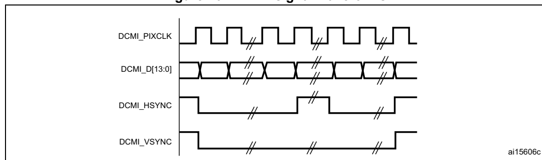
Figure 262. DCMI signal waveforms
