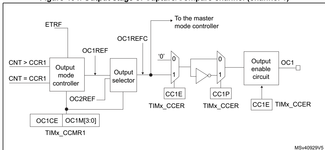
Figure 404. Output stage of Capture/Compare channel (channel 1)
