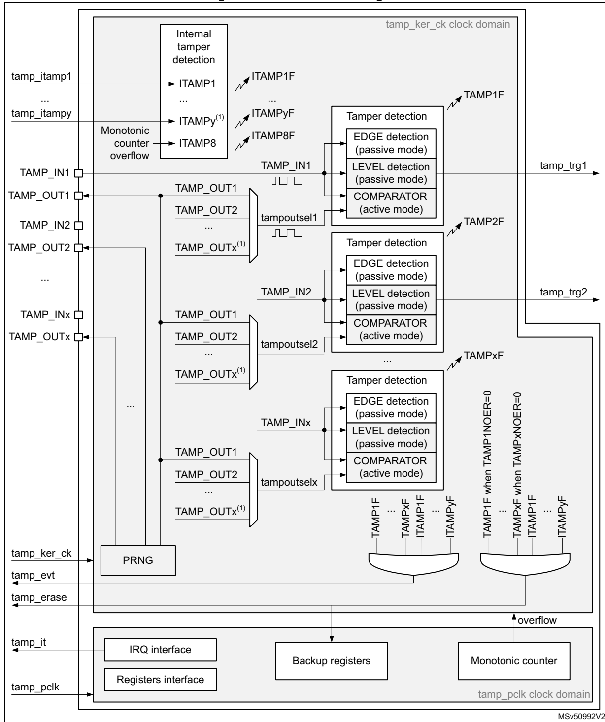
Figure 510. TAMP block diagram
