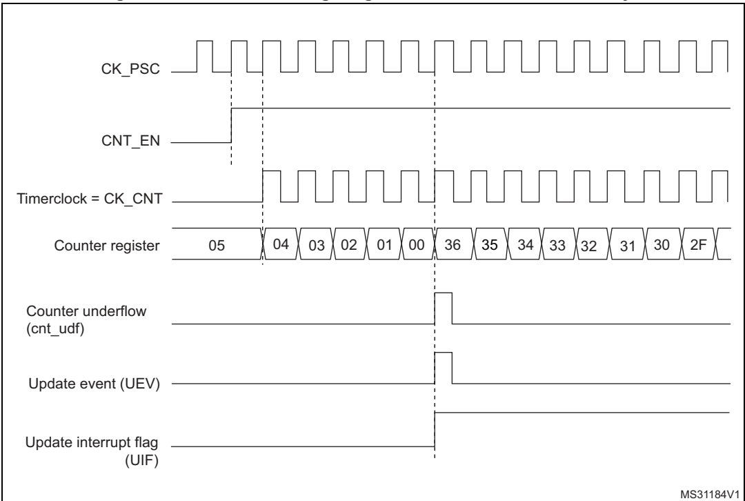
Figure 386. Counter timing diagram, internal clock divided by 1
