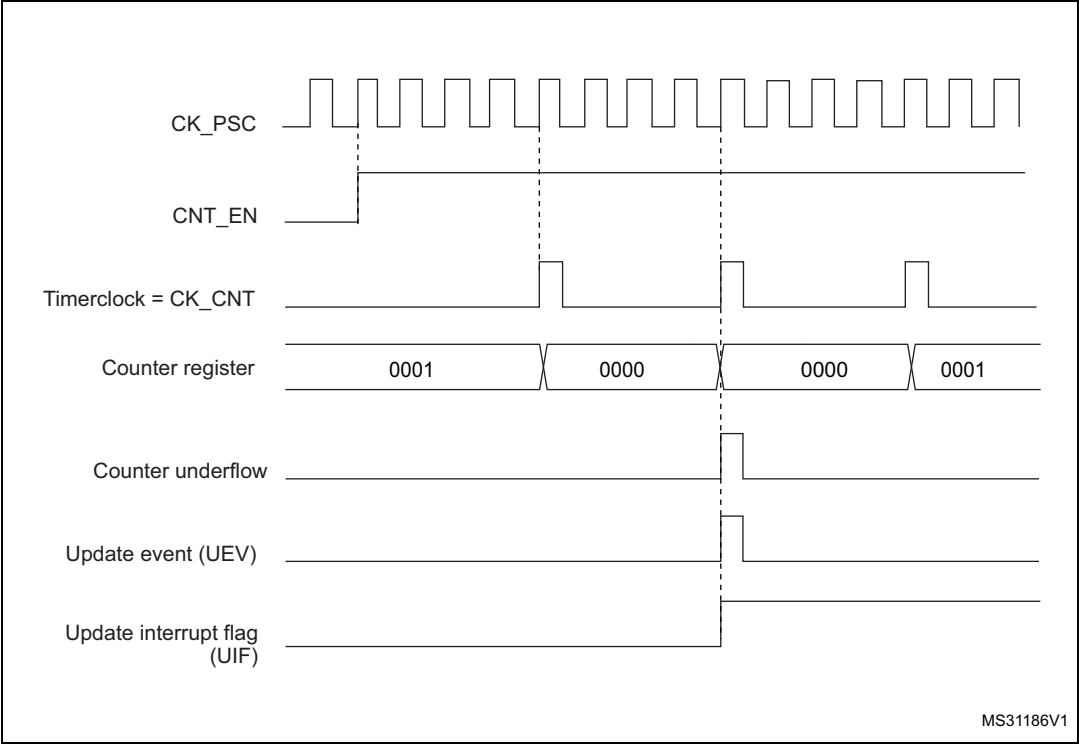
Figure 388. Counter timing diagram, internal clock divided by 4
