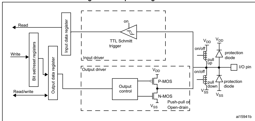
Figure 76. Output configuration
