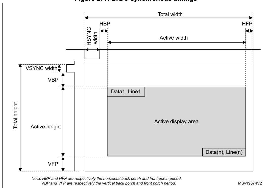
Figure 277. LTDC synchronous timings
