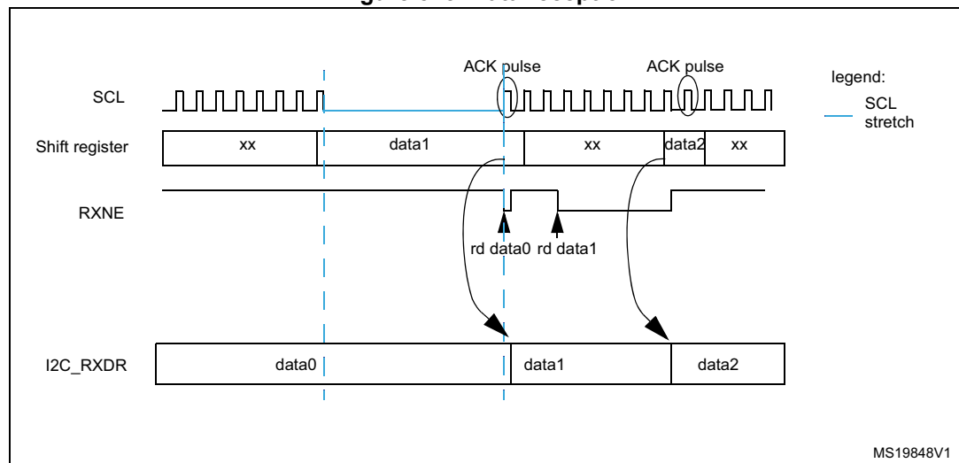
Figure 515. Data reception
