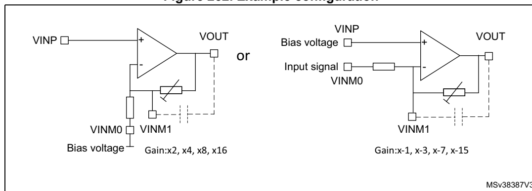
Figure 252. Example configuration
