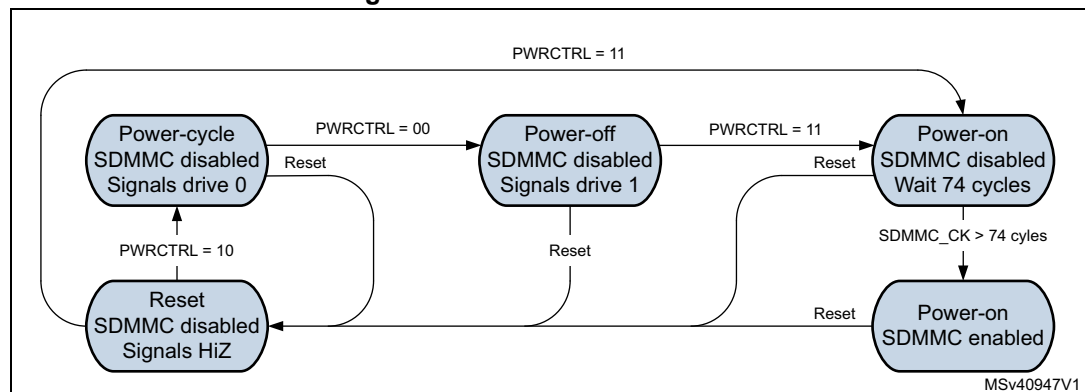
Figure 700. SDMMC state control
