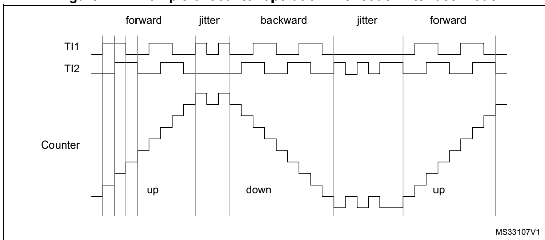
Figure 414. Example of counter operation in encoder interface mode
