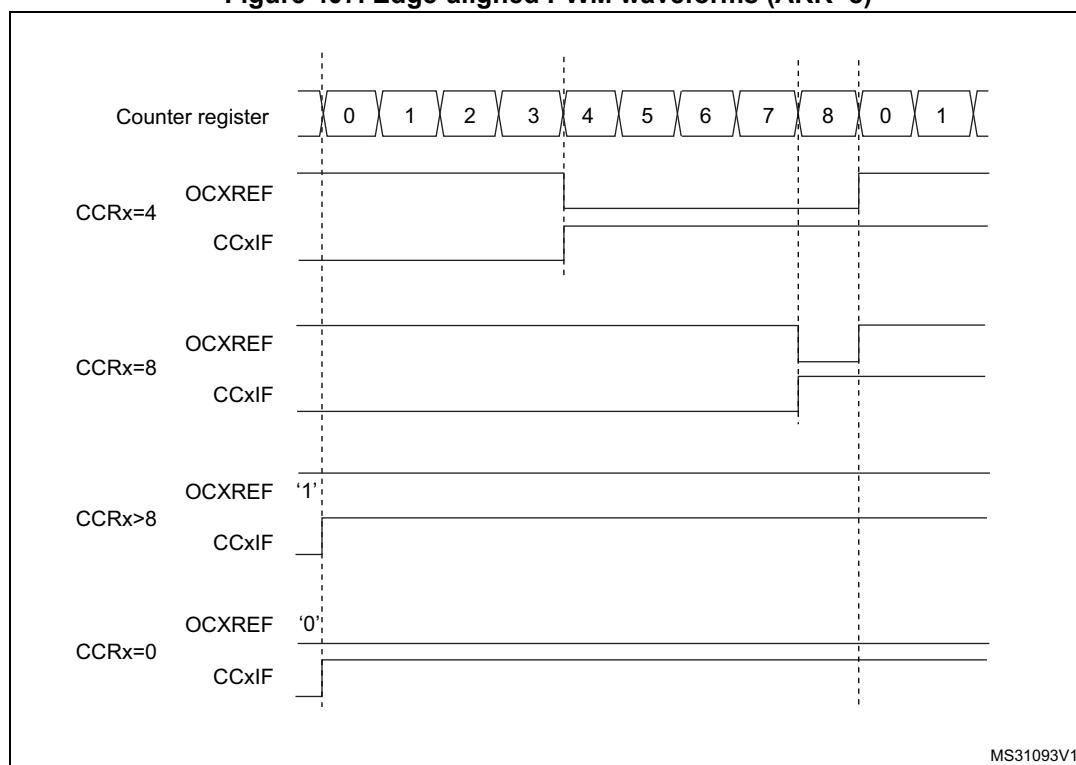
Figure 407. Edge-aligned PWM waveforms (ARR=8)
