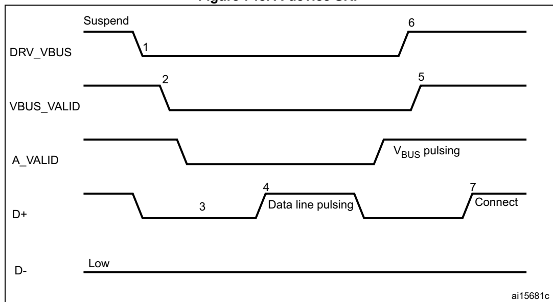
Figure 748. A-device SRP
