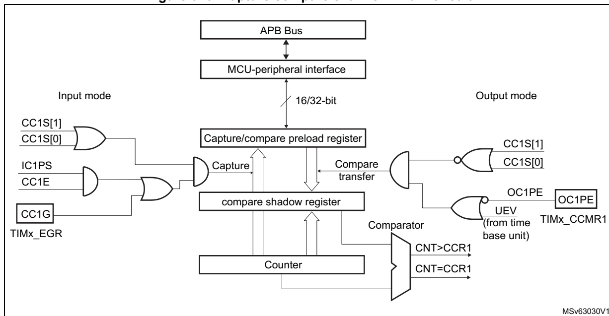
Figure 346. Capture/compare channel 1 main circuit
