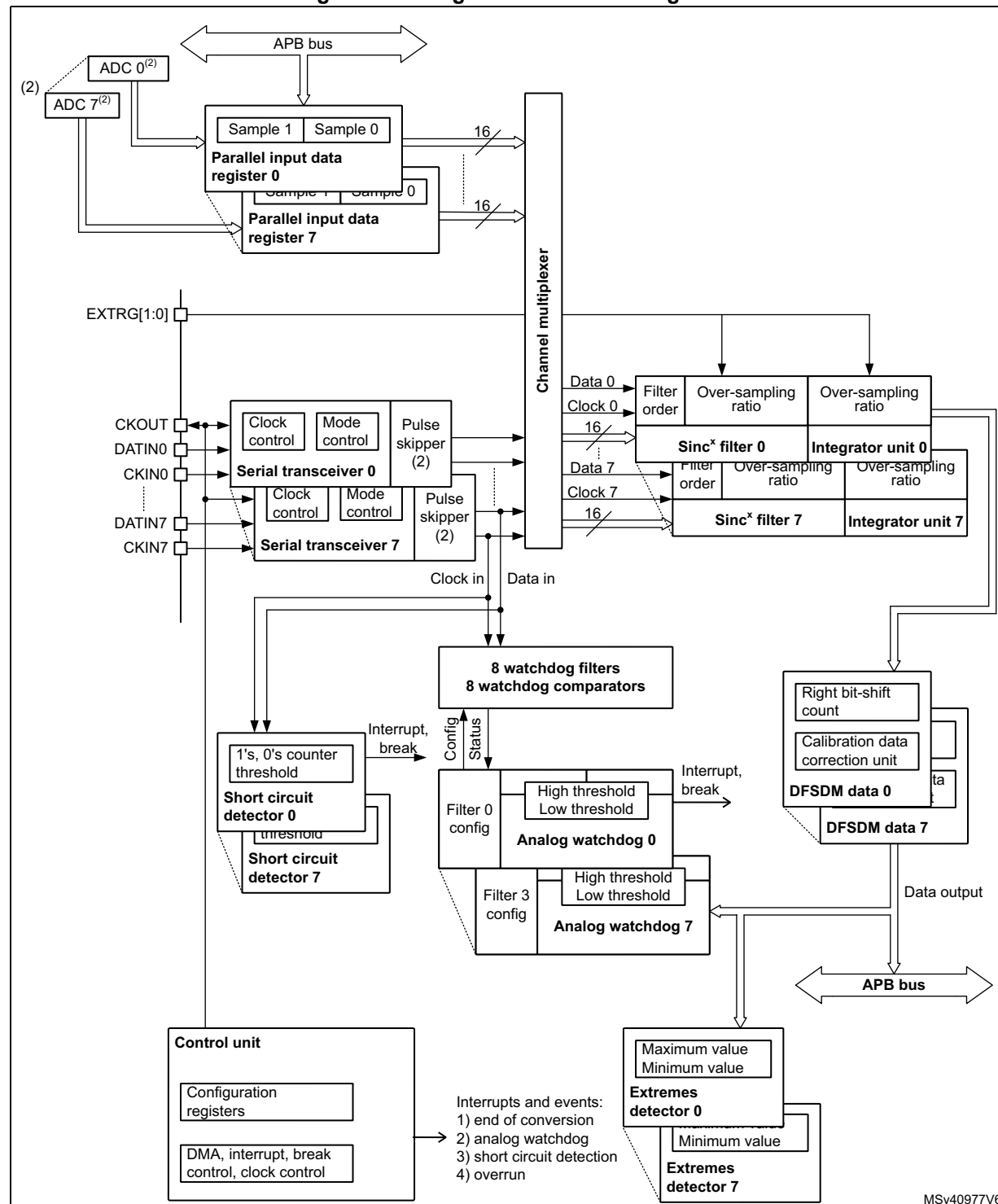
Figure 253. Single DFSDM block diagram
