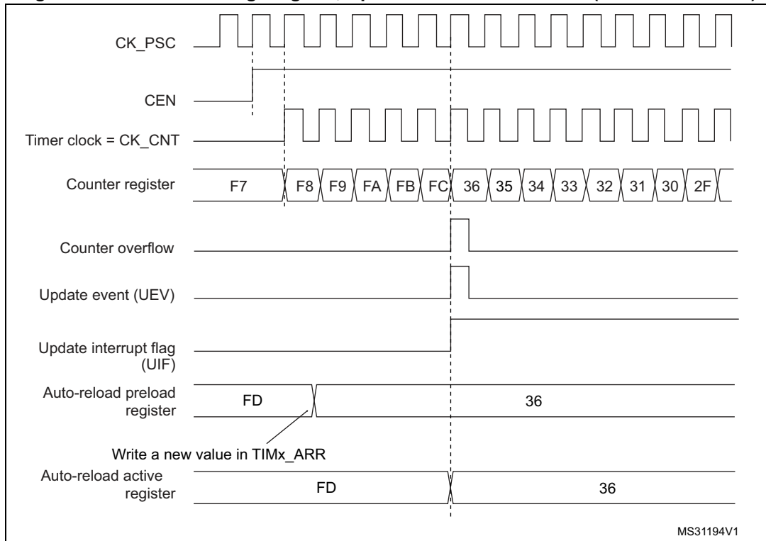
Figure 396. Counter timing diagram, Update event with ARPE=1 (counter overflow)
