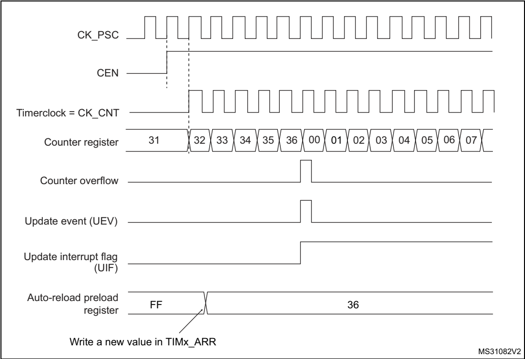
Figure 495. Counter timing diagram, update event when ARPE = 0 (TIMx_ARR not preloaded)
