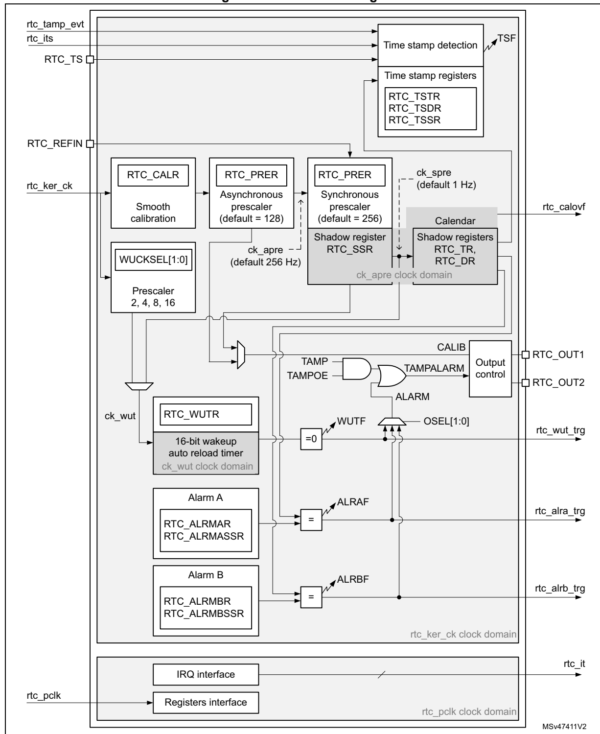
Figure 509. RTC block diagram
