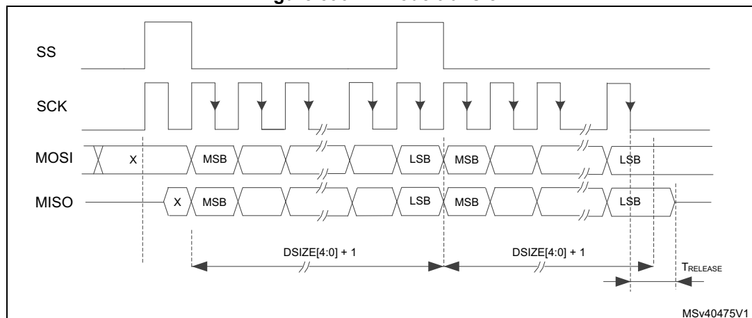
Figure 596. TI mode transfer
