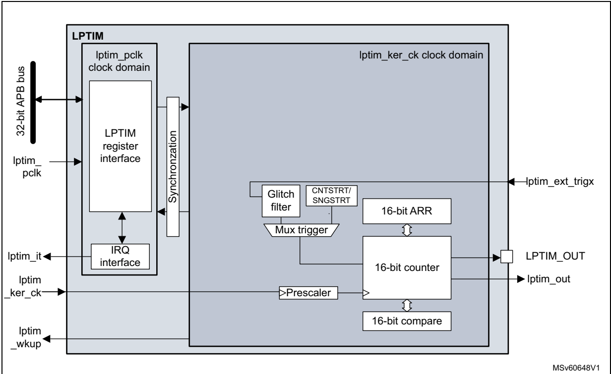
Figure 499. Low-power timer block diagram (LPTIM3)
