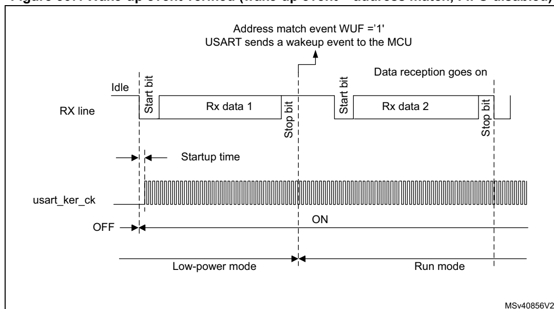
Figure 567. Wake-up event verified (wake-up event = address match, FIFO disabled)
