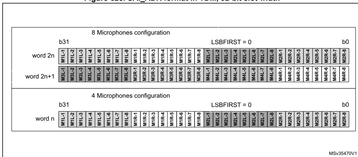
Figure 628. SAI_ADR format in TDM, 32-bit slot width
