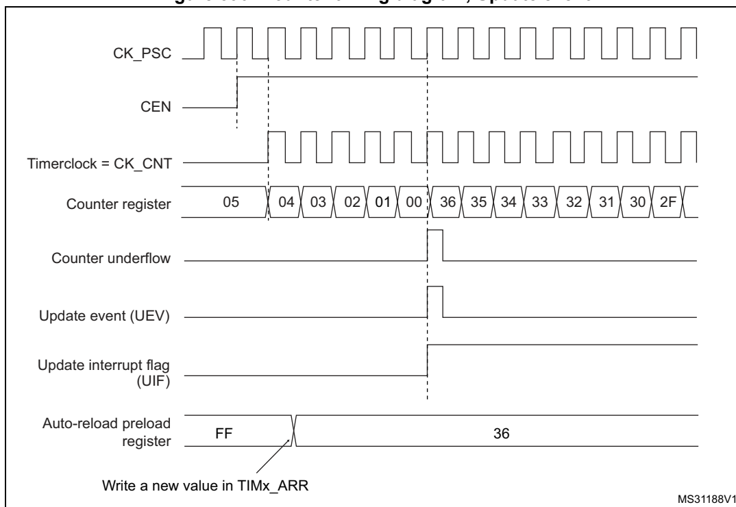
Figure 390. Counter timing diagram, Update event
