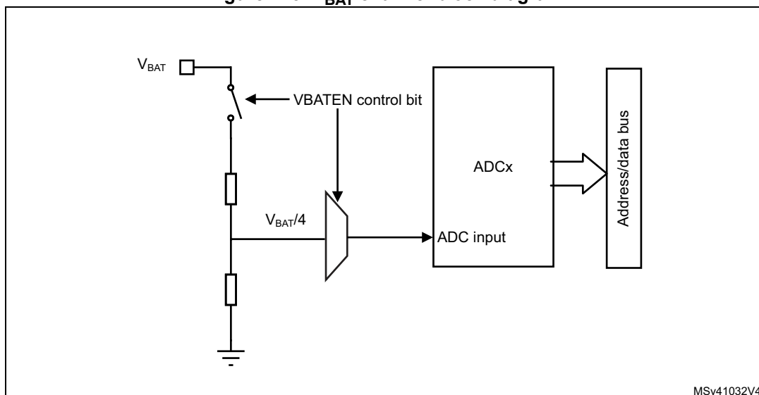
Figure 225. V_{BAT} channel block diagram
