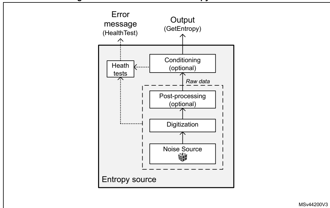
Figure 283. NIST SP800-90B entropy source model
