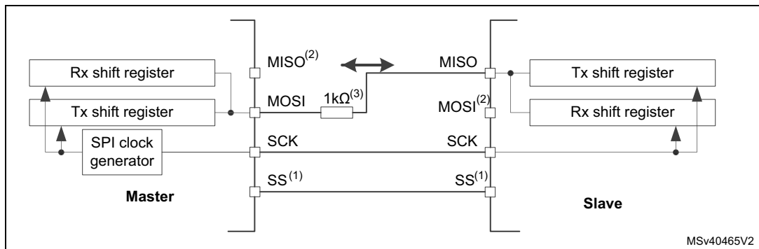
Figure 585. Half-duplex single master/ single slave application
