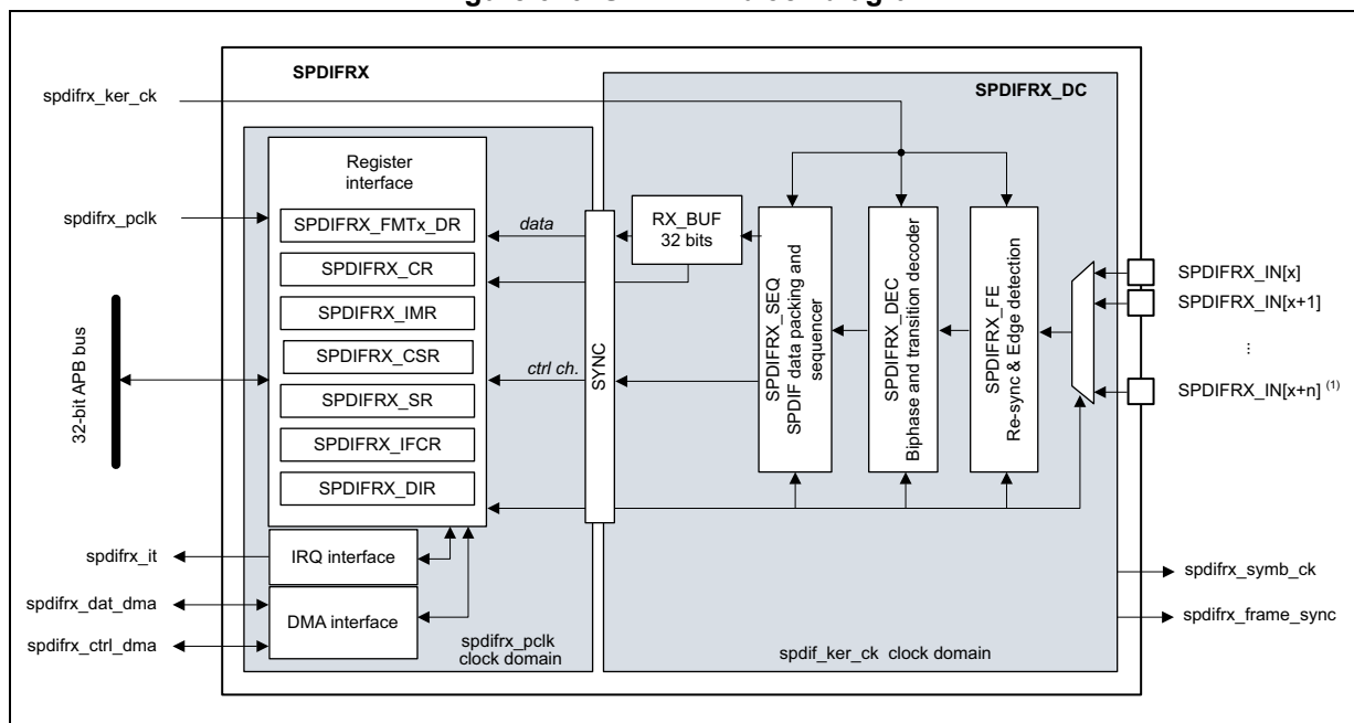
Figure 640. SPDIFRX block diagram
