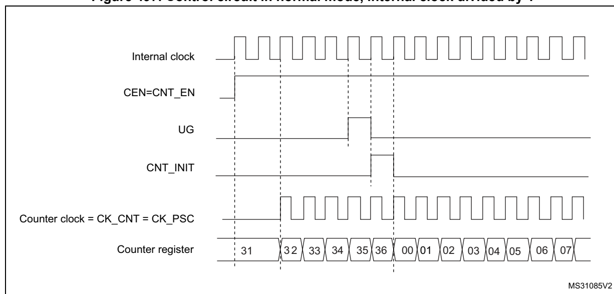
Figure 497. Control circuit in normal mode, internal clock divided by 1
