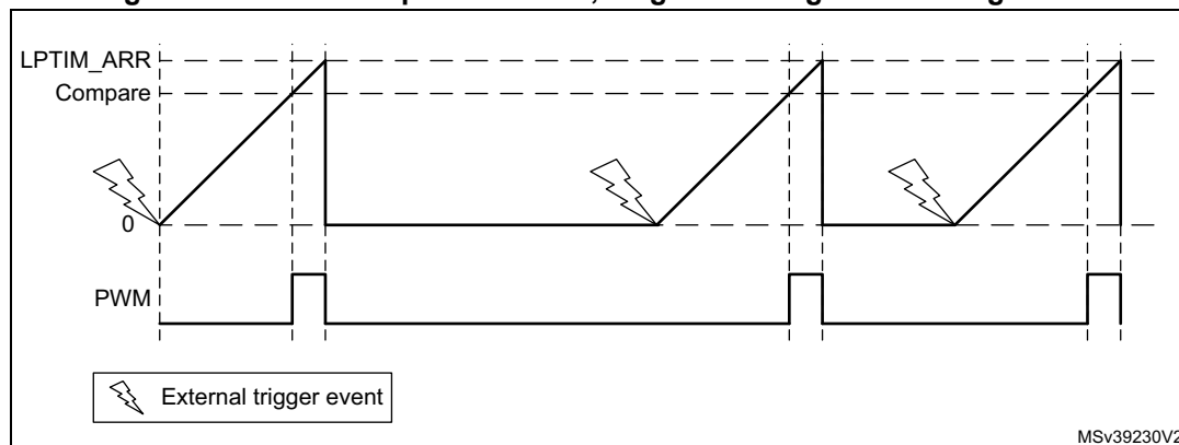
Figure 501. LPTIM output waveform, single counting mode configuration
