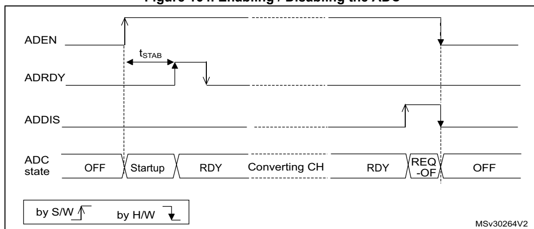
Figure 164. Enabling / Disabling the ADC
