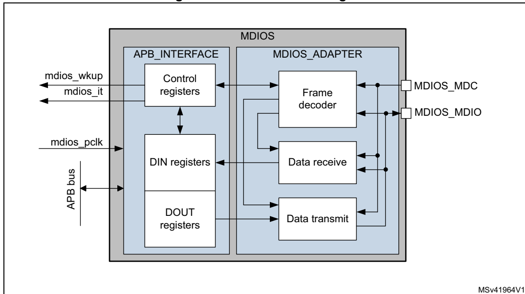
Figure 668. MDIOS block diagram
