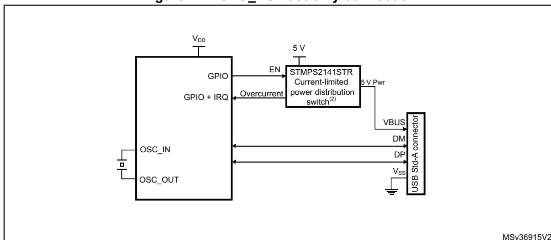
Figure 724. OTG_HS host-only connection
