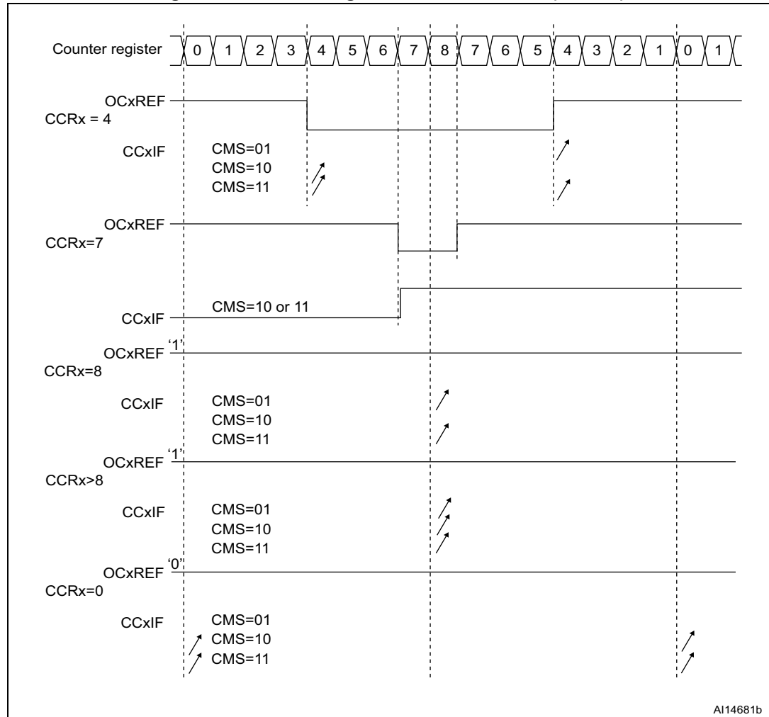
Figure 353. Center-aligned PWM waveforms (ARR=8)
