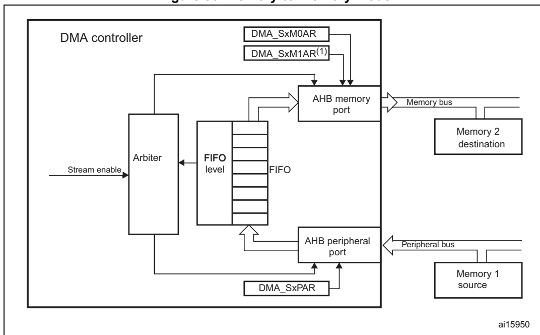
Figure 86. Memory-to-memory mode
