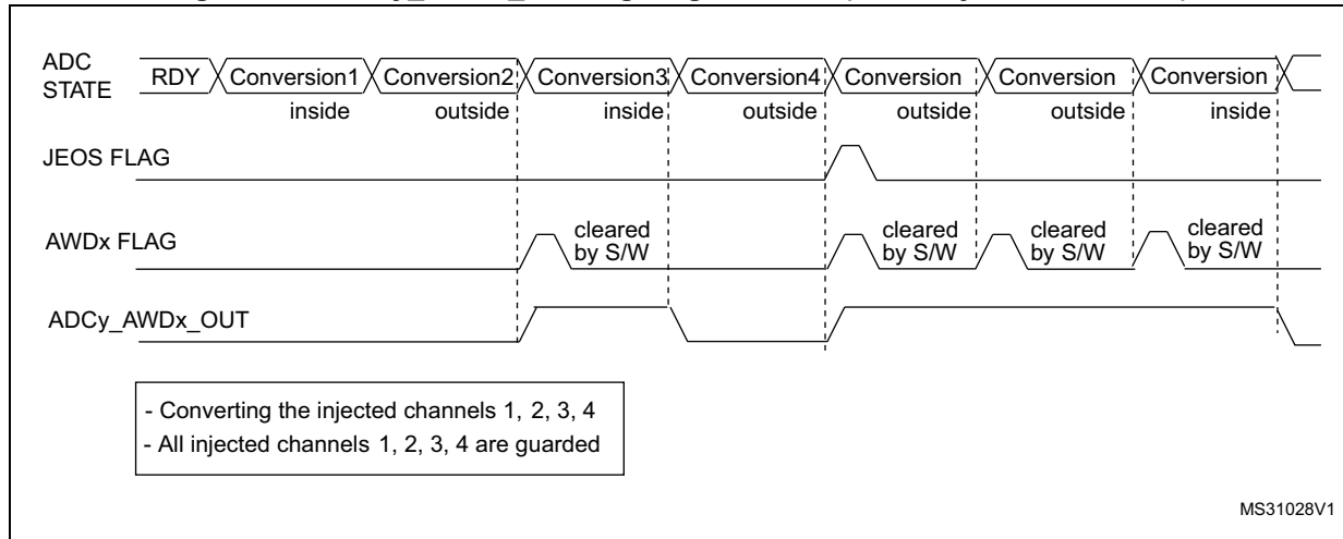
Figure 201. ADCy_AWDx_OUT signal generation (on all injected channels)
