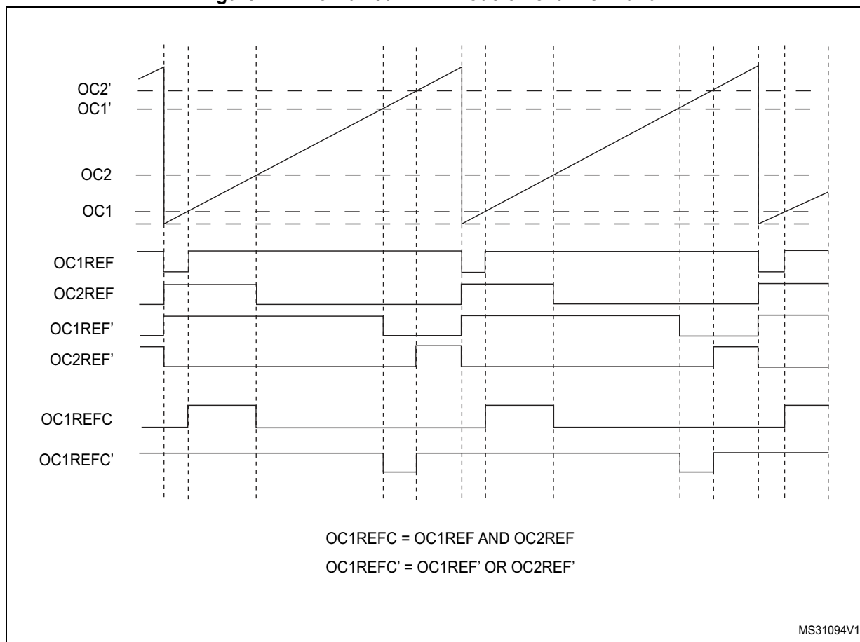
Figure 474. Combined PWM mode on channel 1 and 2
