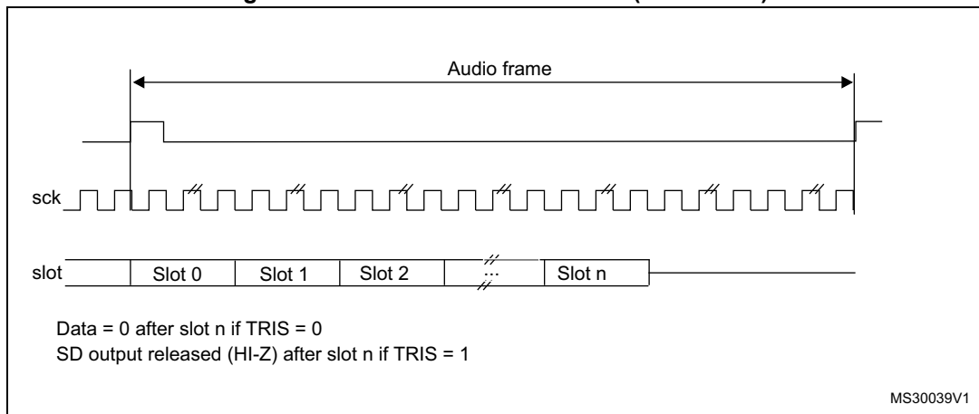
Figure 621. FS role is start of frame (FSDEF = 0)
