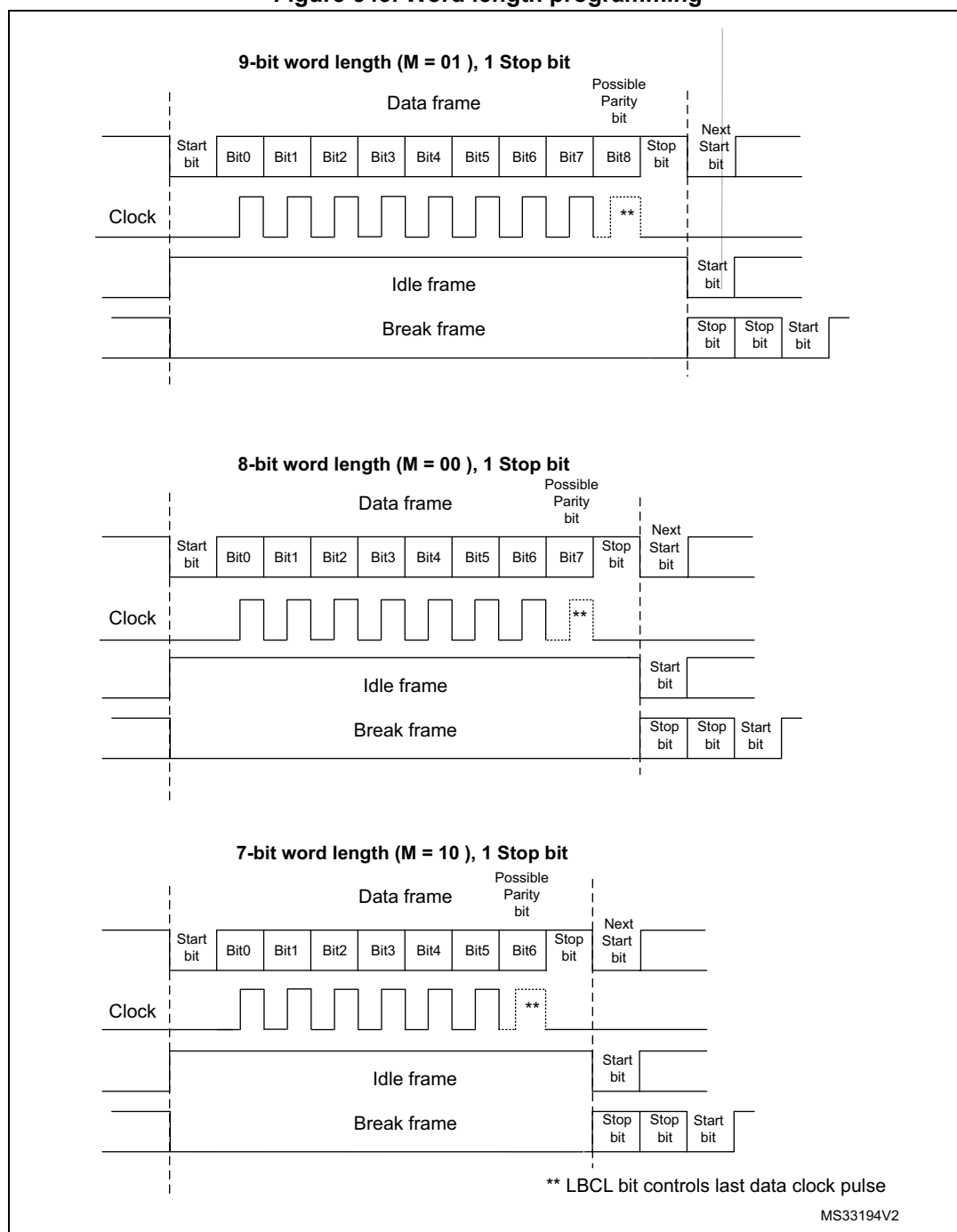
Figure 543. Word length programming
