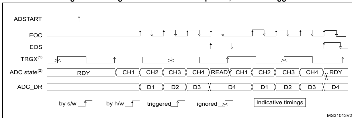
Figure 184. Single conversions of a sequence, hardware trigger
