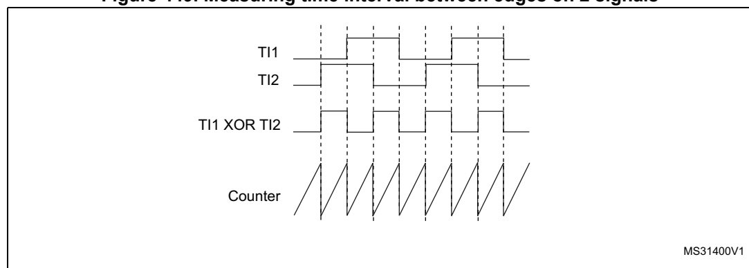
Figure 449. Measuring time interval between edges on 2 signals
