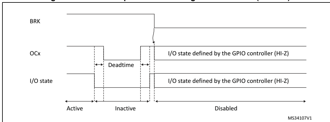
Figure 363. PWM output state following BRK assertion (OSSR=0)
