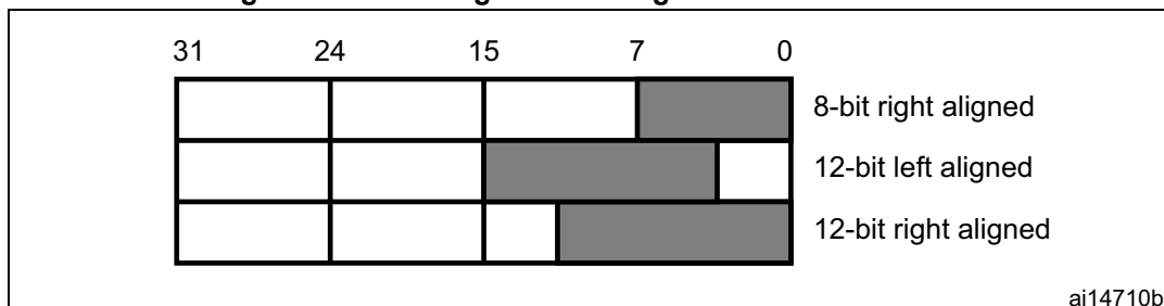
Figure 232. Data registers in single DAC channel mode
