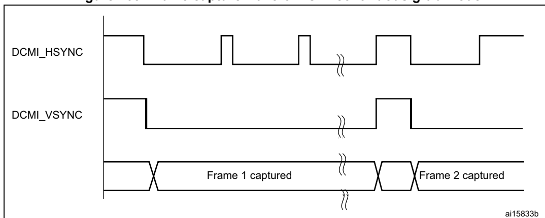
Figure 265. Frame capture waveforms in continuous grab mode
