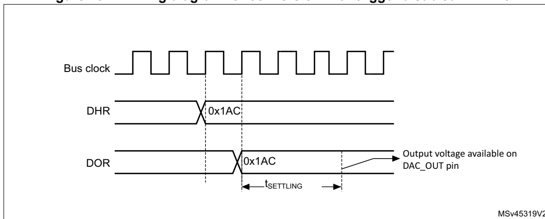
Figure 234. Timing diagram for conversion with trigger disabled TEN = 0
