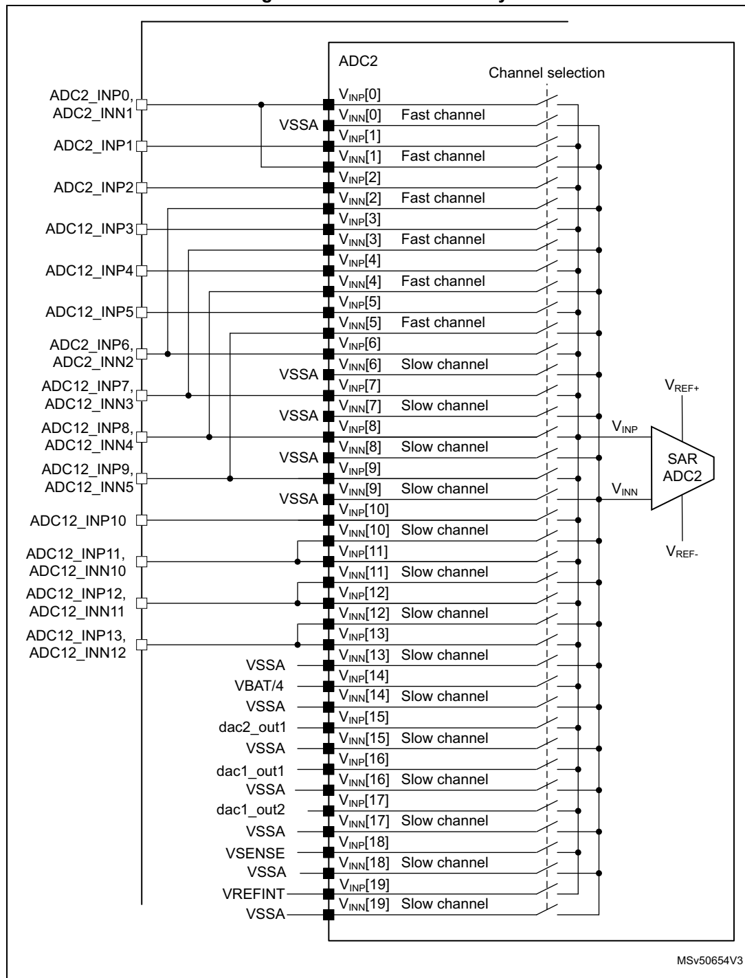
Figure 160. ADC2 connectivity
