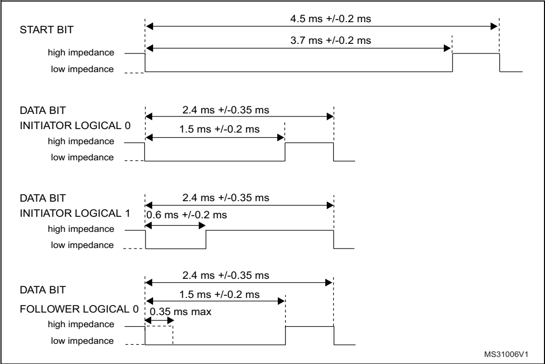
Figure 755. Bit timings
