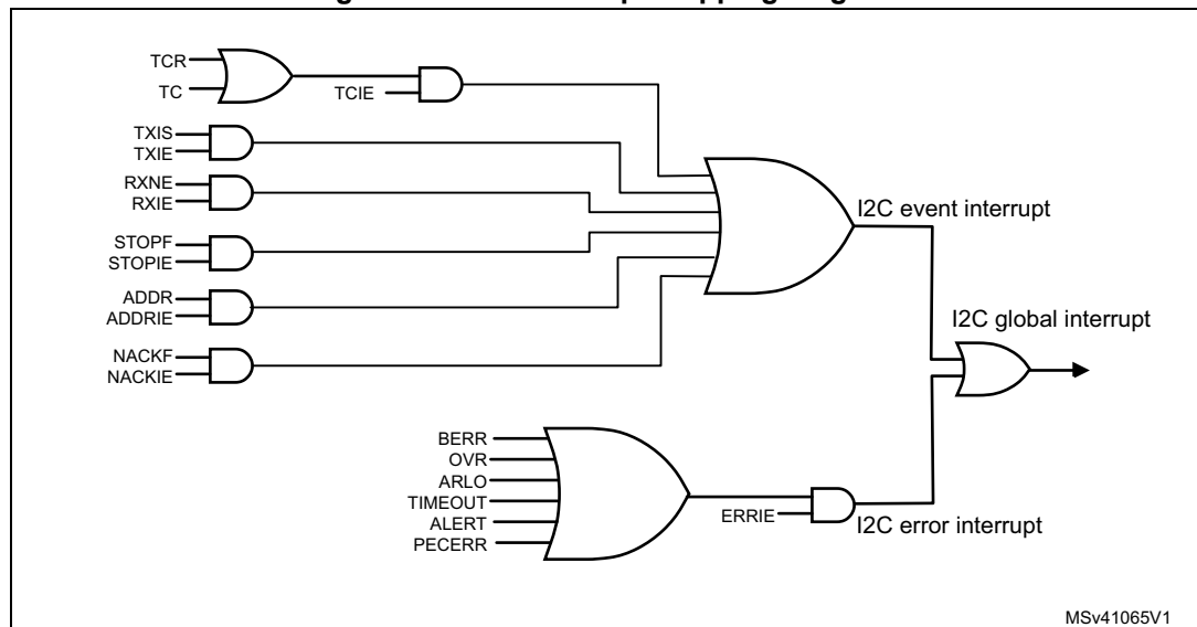
Figure 541. I2C interrupt mapping diagram
