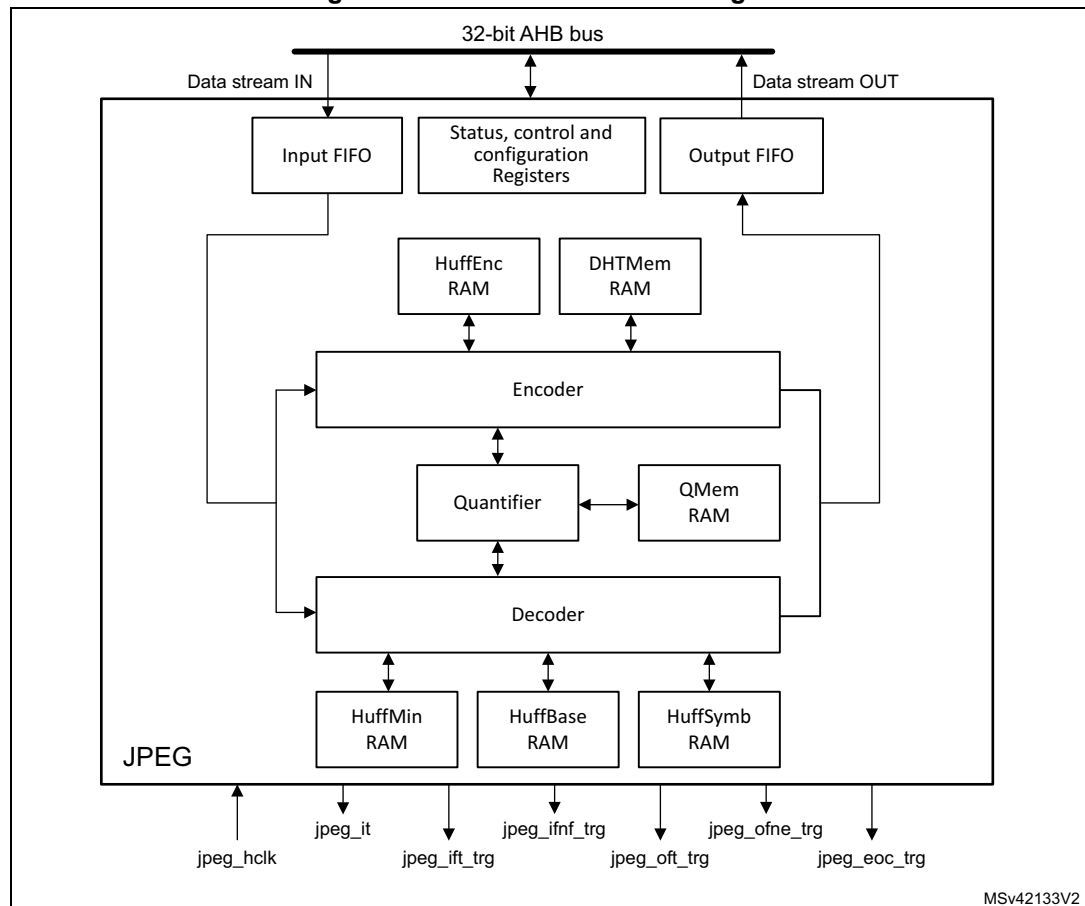
Figure 281. JPEG codec block diagram
