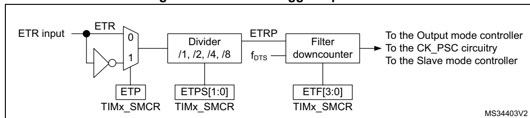
Figure 338. External trigger input block
