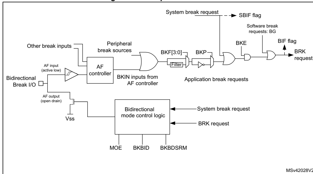
Figure 480. Output redirection
