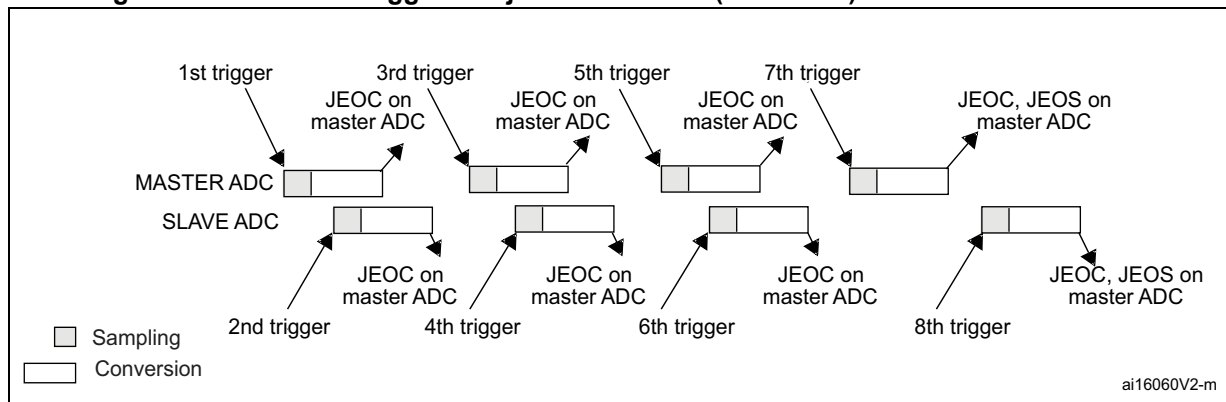
Figure 215. Alternate trigger: 4 injected channels (each ADC) in discontinuous mode
