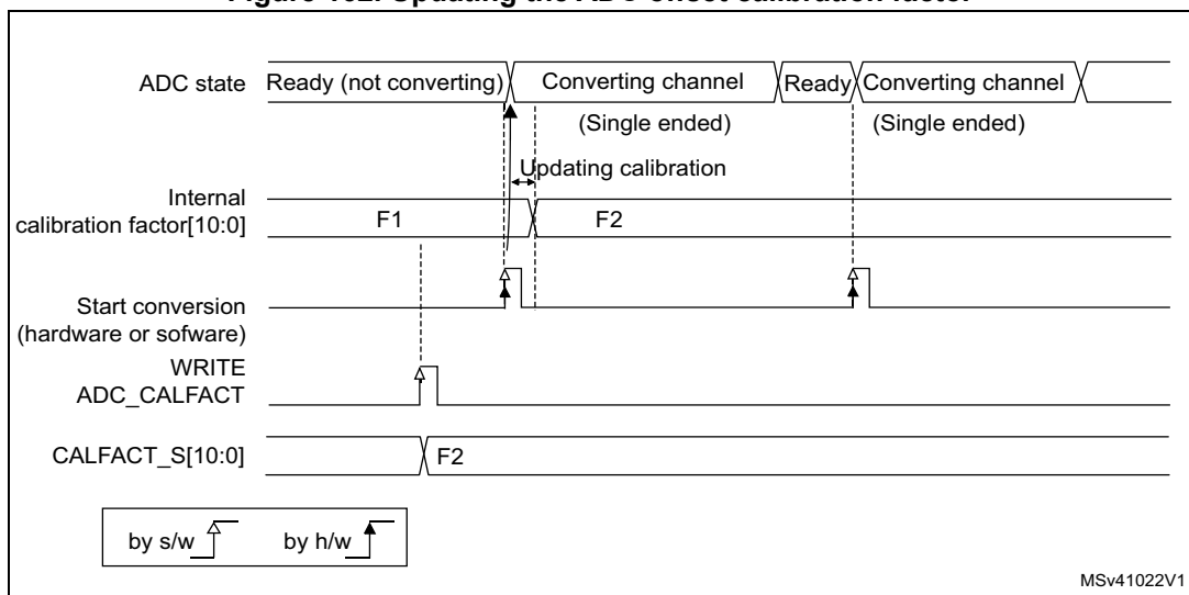
Figure 162. Updating the ADC offset calibration factor
