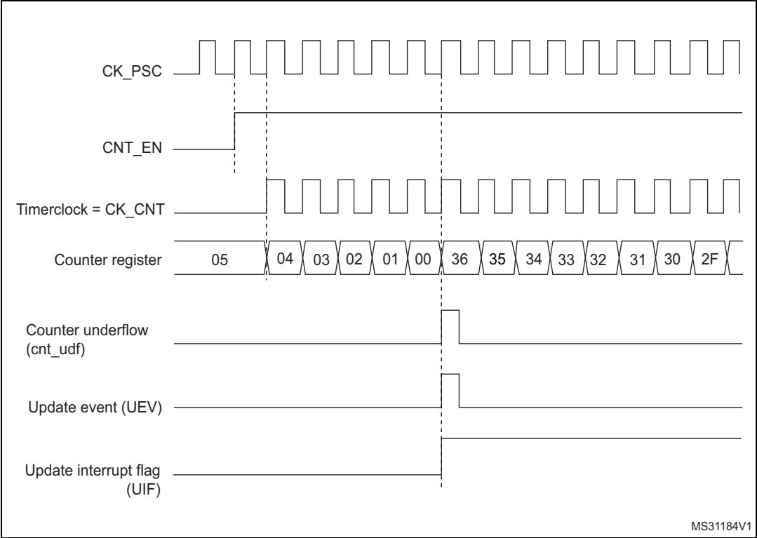
Figure 326. Counter timing diagram, internal clock divided by 1
