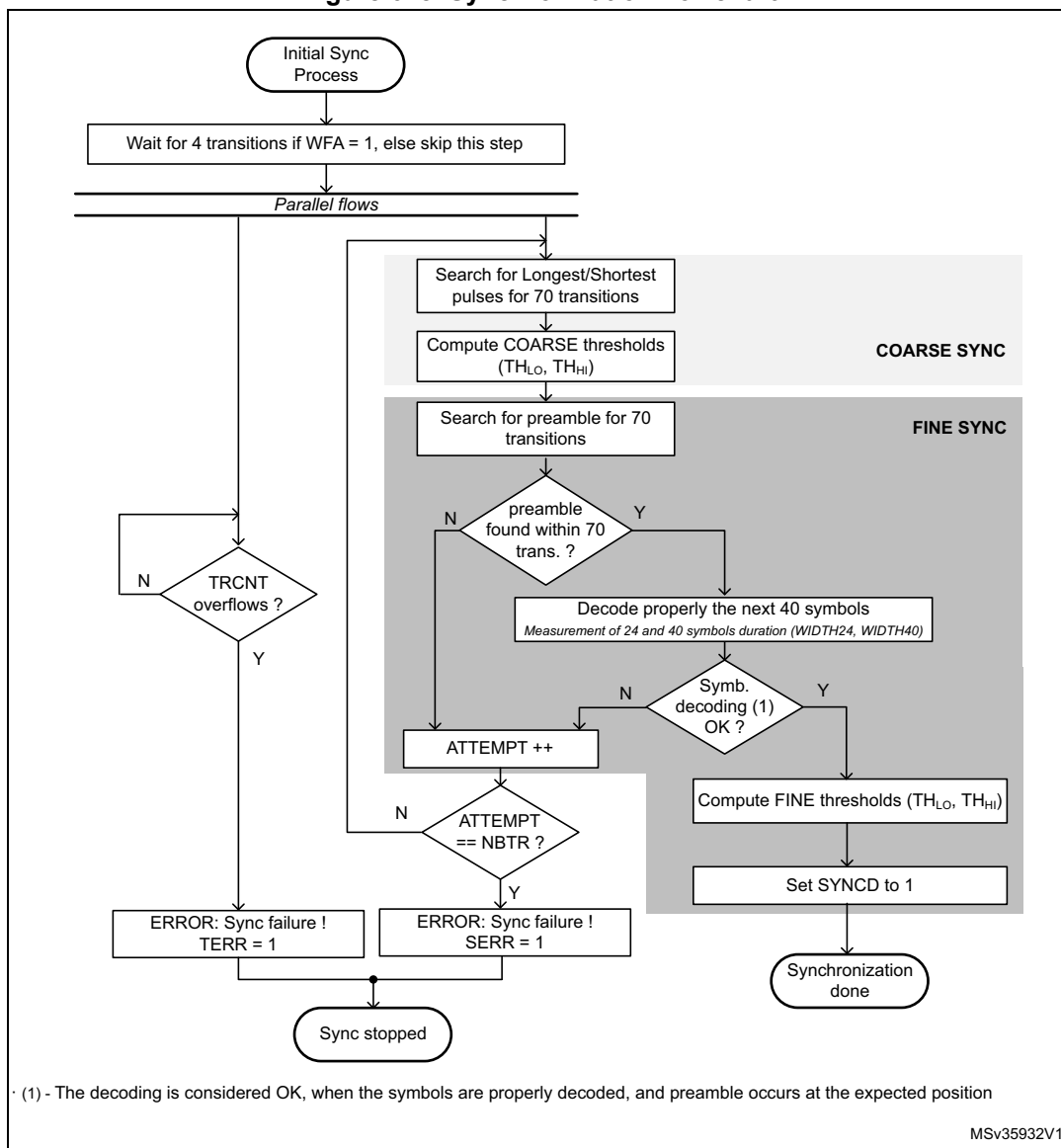
Figure 648. Synchronization flowchart
