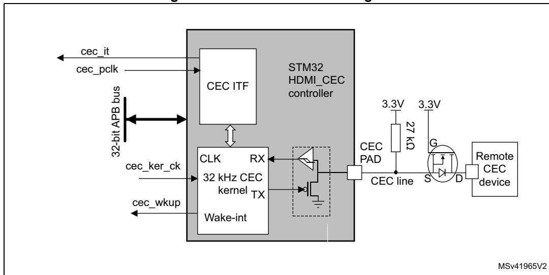
Figure 752. HDMI-CEC block diagram
