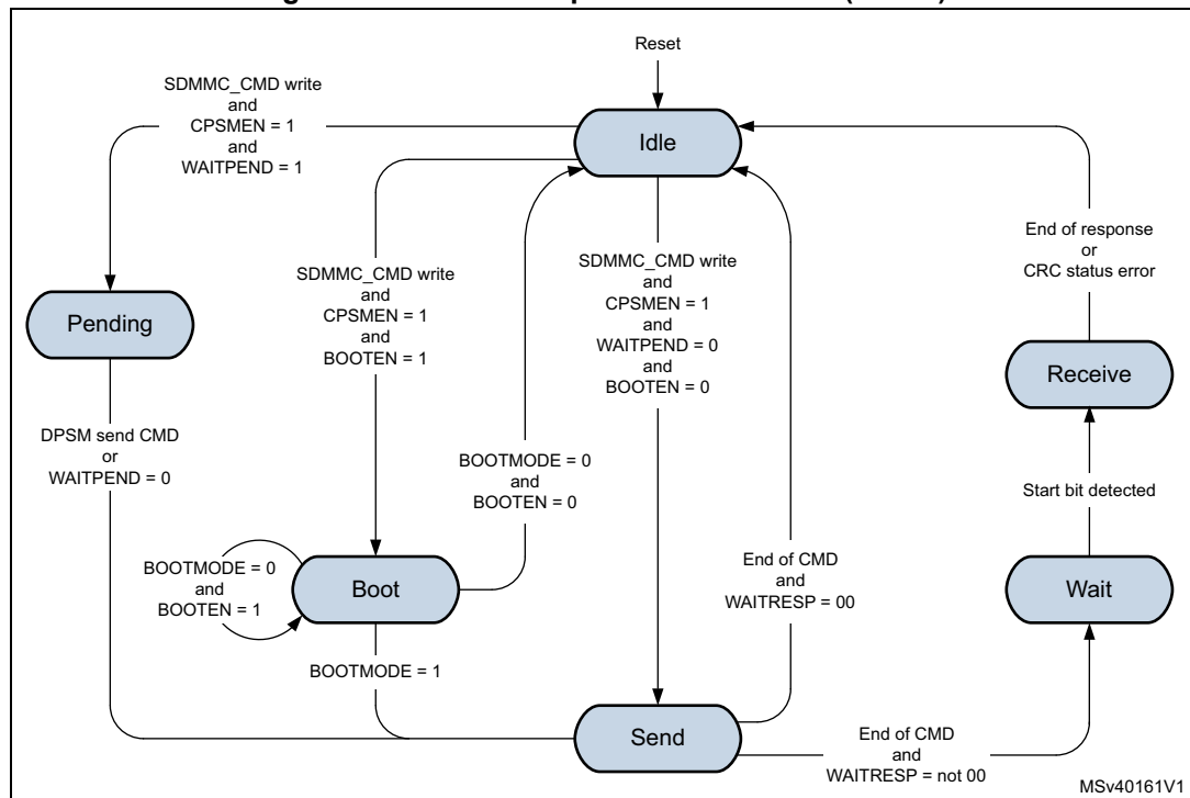
Figure 680. Command path state machine (CPSM)
