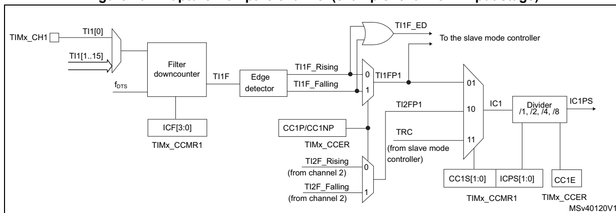
Figure 402. Capture/Compare channel (example: channel 1 input stage)
