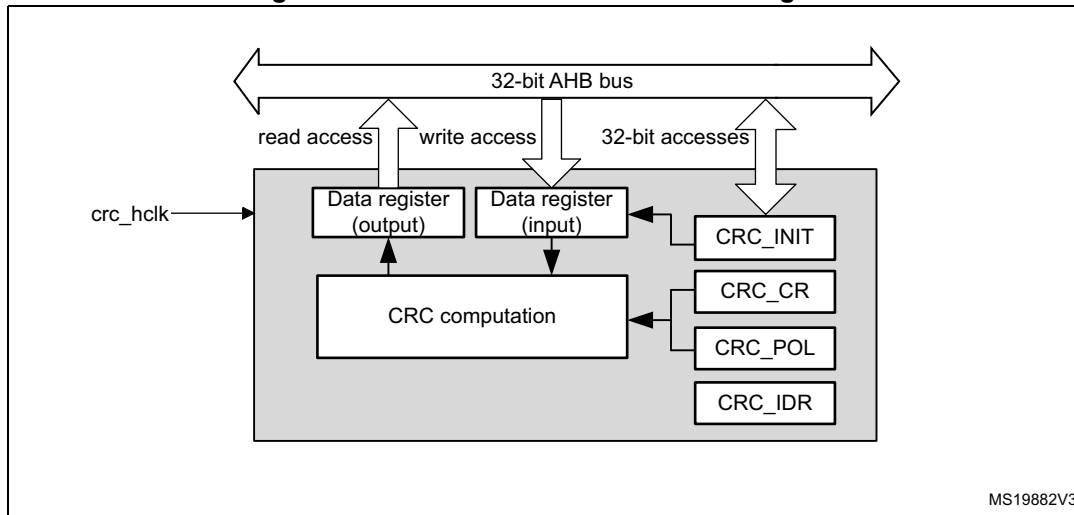
Figure 106. CRC calculation unit block diagram
