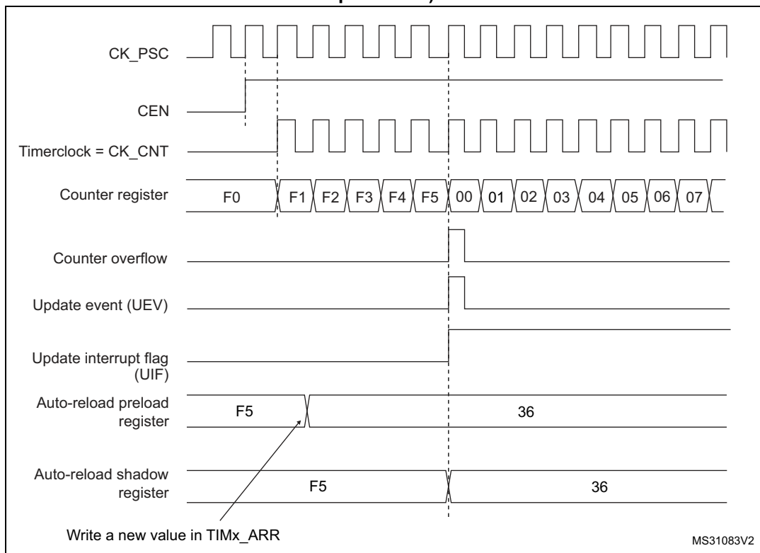
Figure 496. Counter timing diagram, update event when ARPE=1 (TIMx_ARR preloaded)
