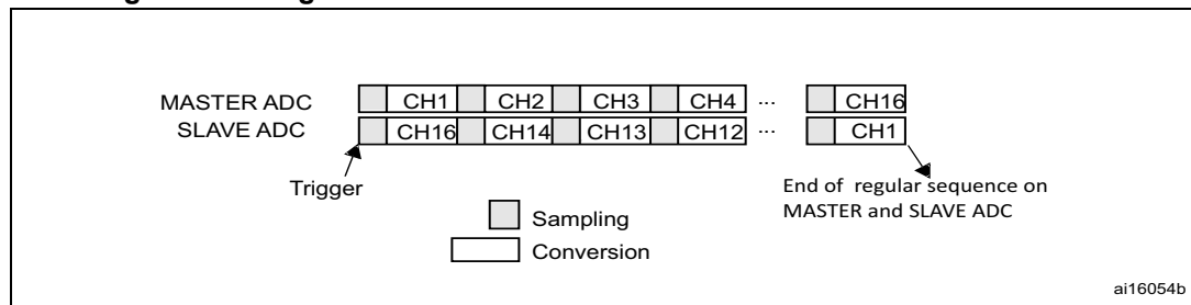
Figure 210. Regular simultaneous mode on 16 channels: dual ADC mode
