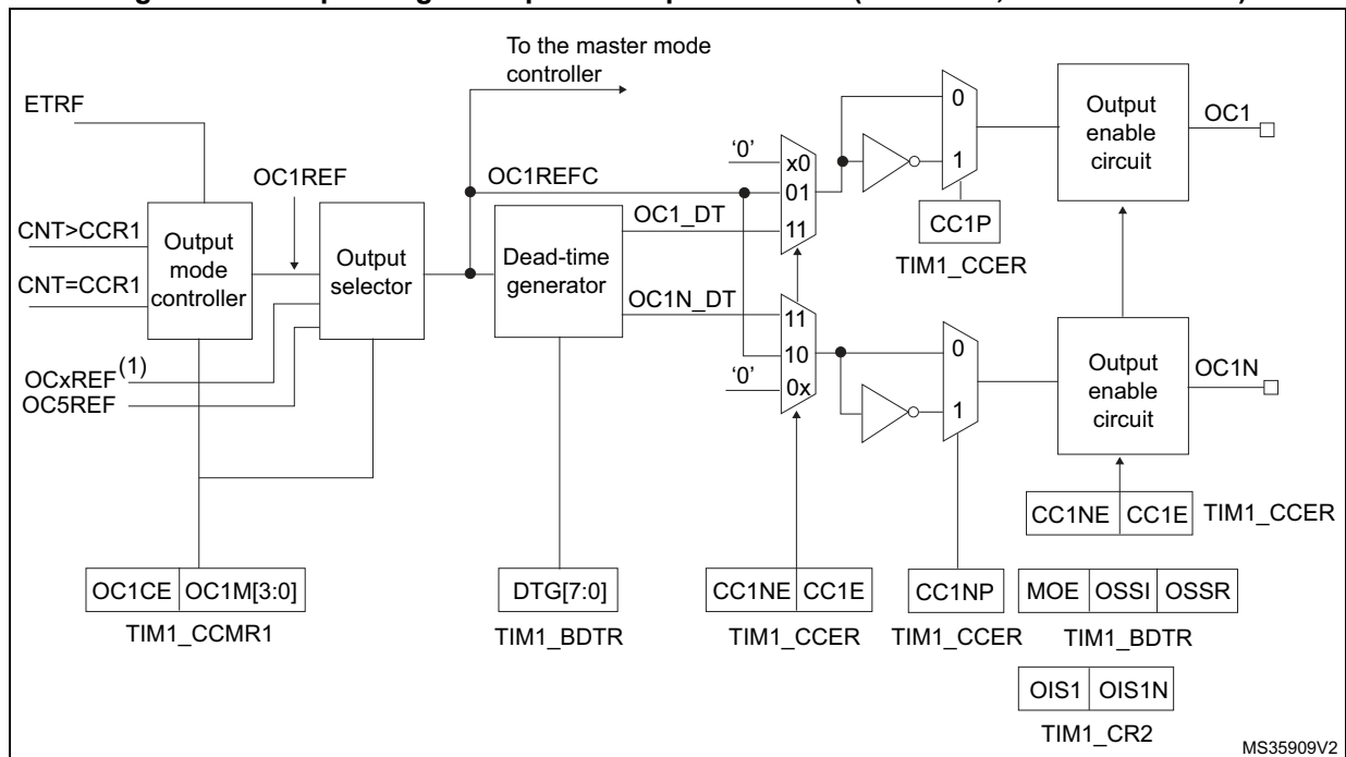
Figure 347. Output stage of capture/compare channel (channel 1, idem ch. 2 and 3)
