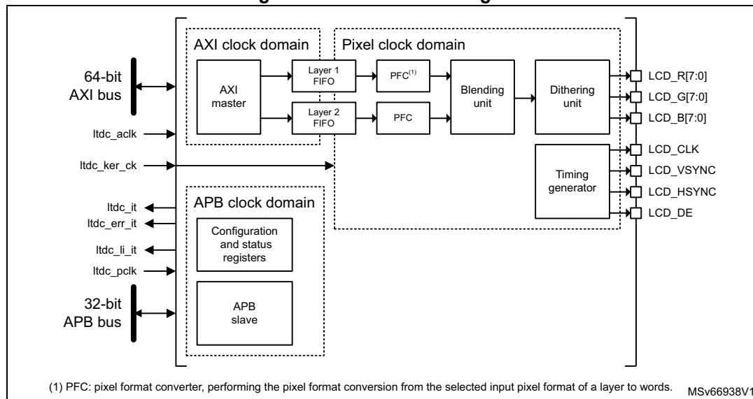
Figure 276. LTDC block diagram
