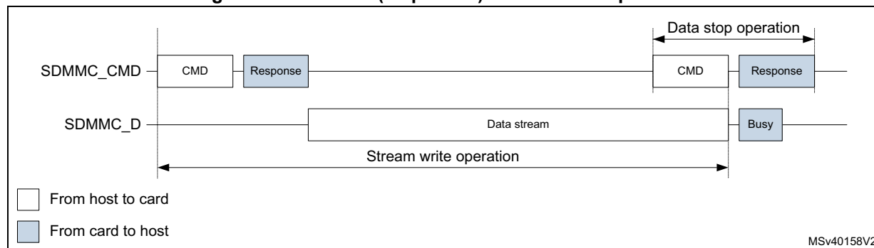
Figure 675. SDMMC (sequential) stream write operation
