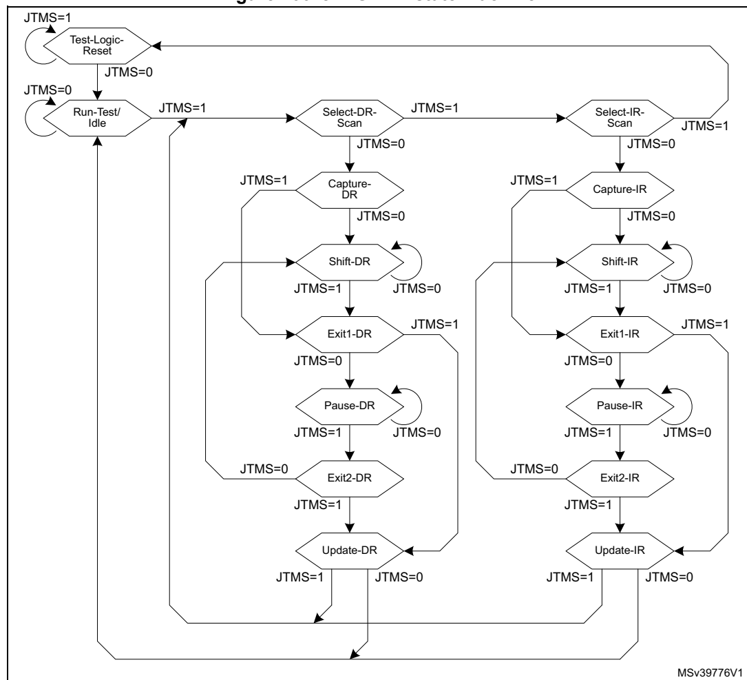
Figure 766. JTAG TAP state machine
