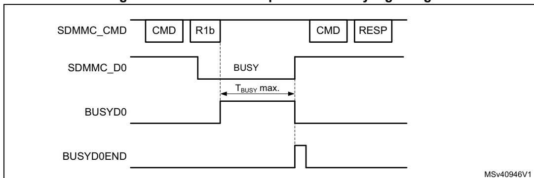
Figure 699. Command response R1b busy signaling
