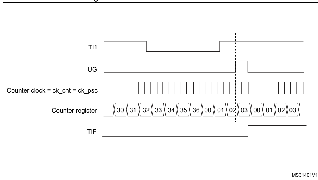
Figure 373. Control circuit in reset mode
