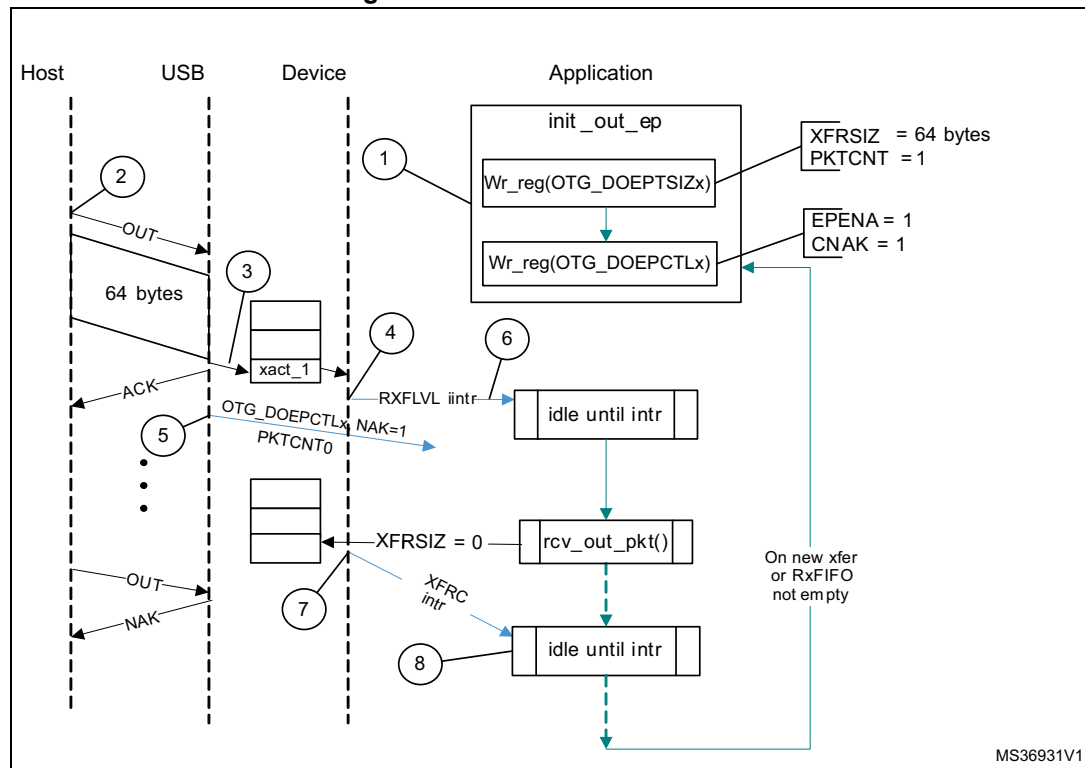
Figure 746. Bulk OUT transaction
