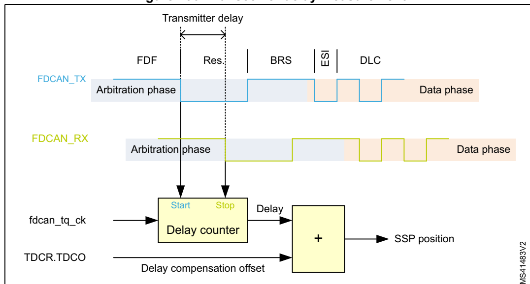
Figure 706. Transceiver delay measurement
