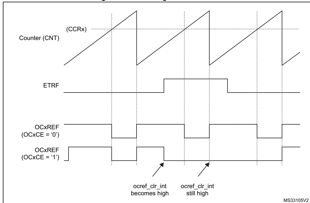
Figure 411. Clearing TIMx OCxREF
