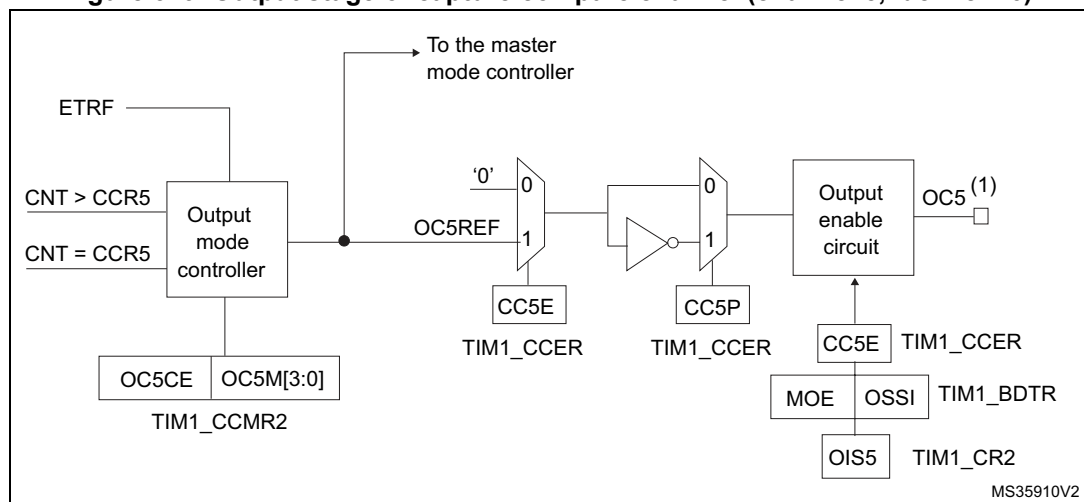
Figure 349. Output stage of capture/compare channel (channel 5, idem ch. 6)
