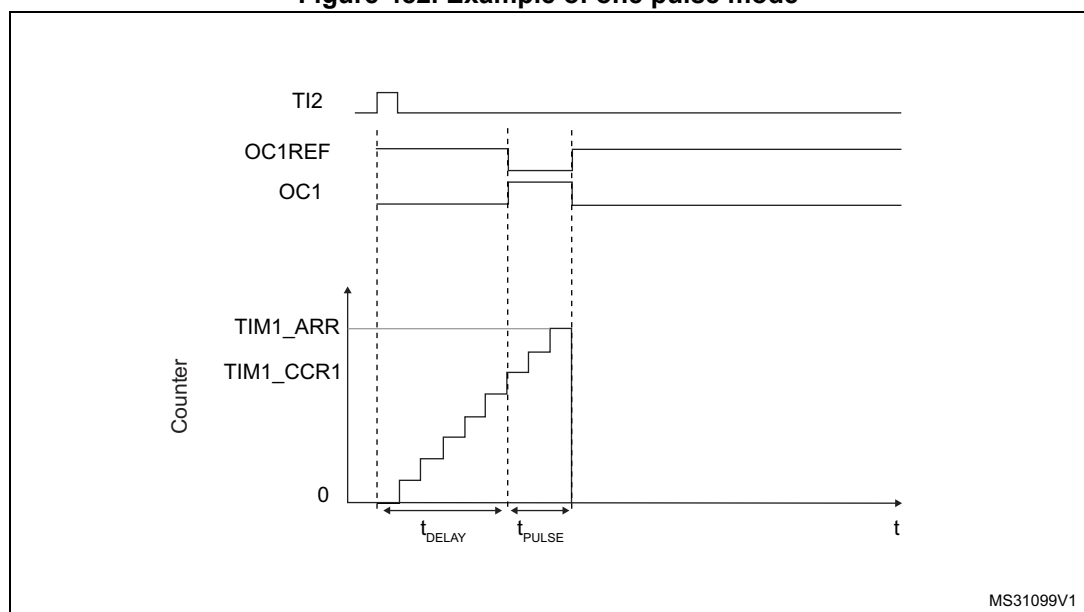
Figure 482. Example of one pulse mode
