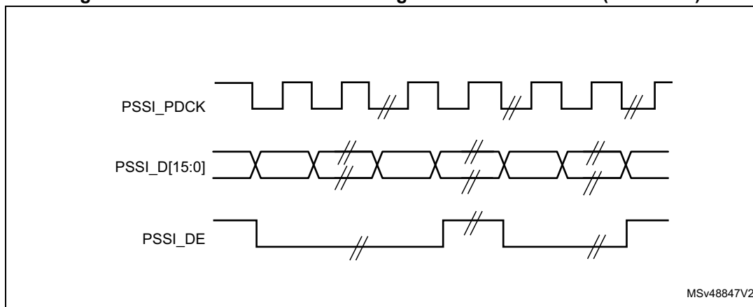
Figure 272. Data enable waveform diagram in transmit mode (CKPOL=0)
