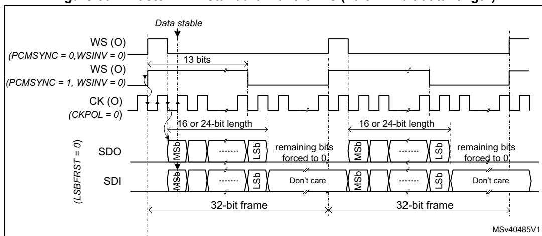
Figure 607. Master PCM standard waveforms (16 or 24-bit data length)
