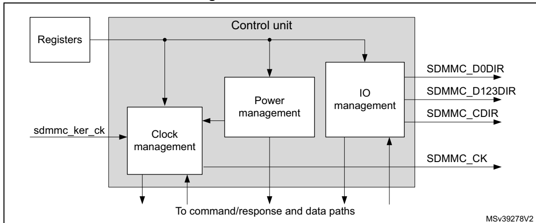
Figure 678. Control unit
