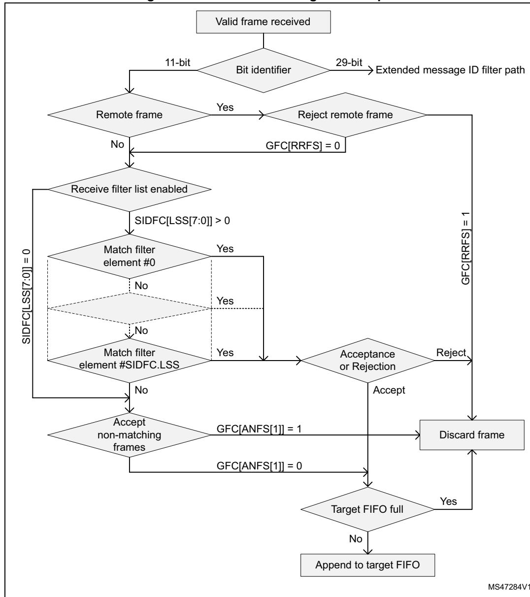
Figure 710. Standard message ID filter path
