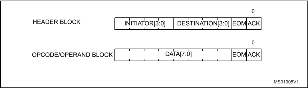
Figure 754. Blocks
