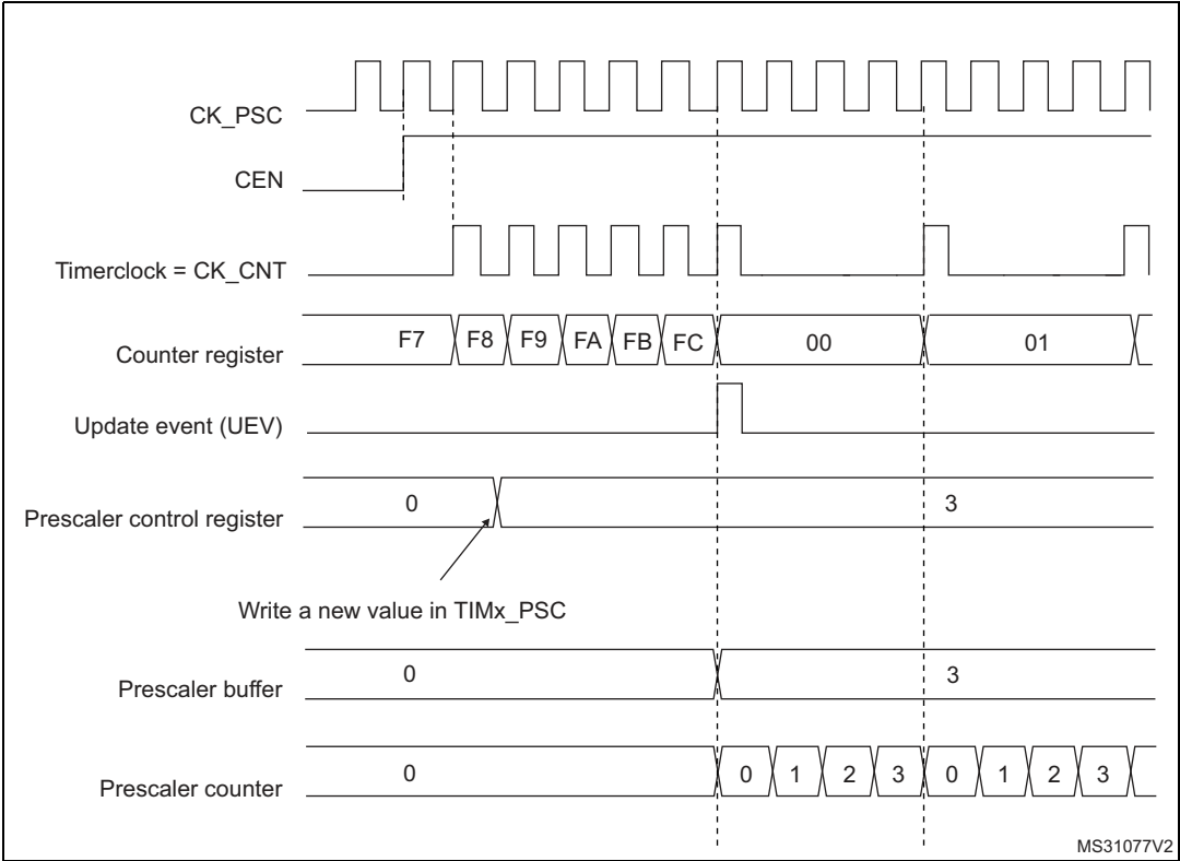
Figure 379. Counter timing diagram with prescaler division change from 1 to 4
