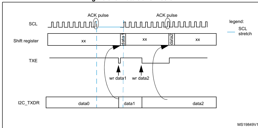
Figure 516. Data transmission
