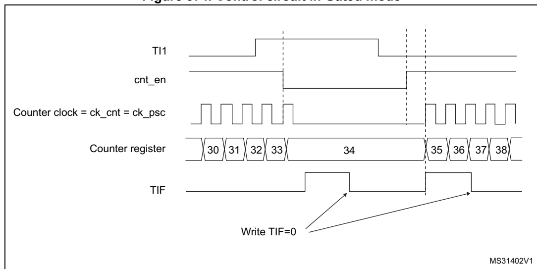
Figure 374. Control circuit in Gated mode
