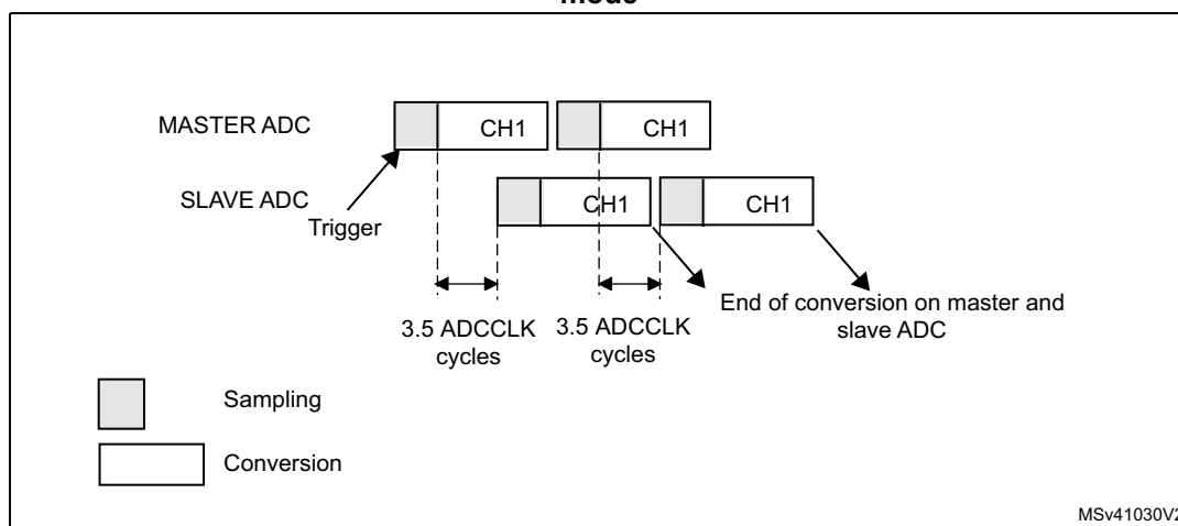
Figure 211. Interleaved mode on 1 channel in continuous conversion mode: dual ADC mode
