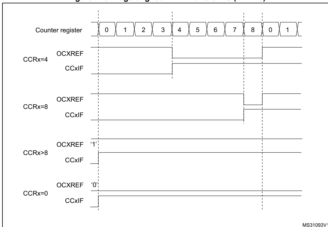
Figure 445. Edge-aligned PWM waveforms (ARR=8)
