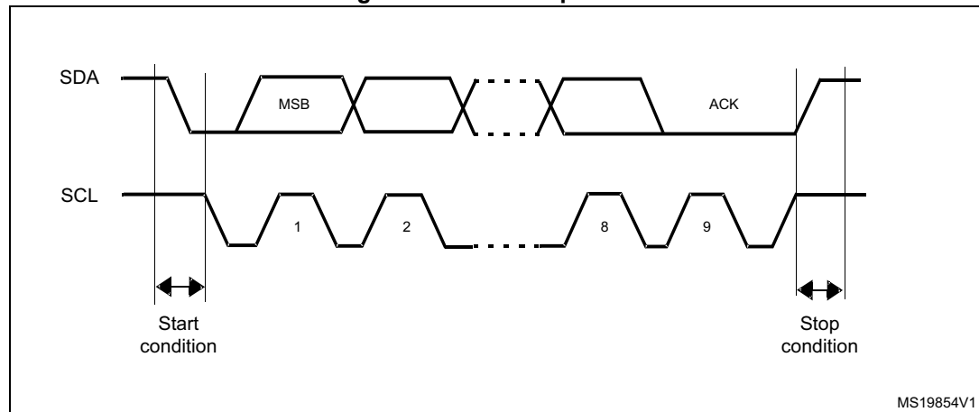
Figure 512. I 2 C bus protocol
