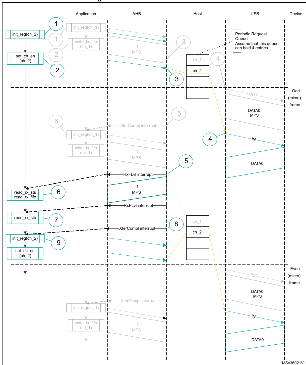
Figure 737. Isochronous IN transactions
