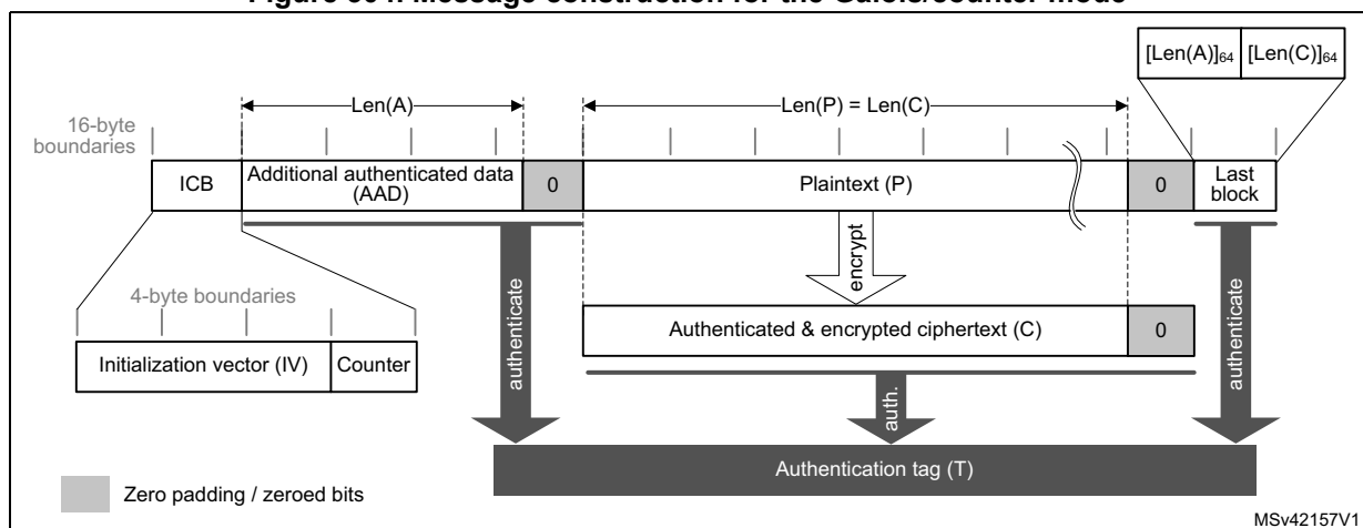
Figure 304. Message construction for the Galois/counter mode
