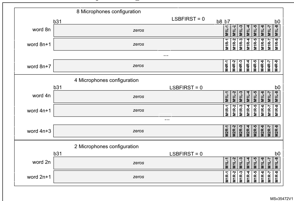
Figure 630. SAI_ADR format in TDM, 8-bit slot width
