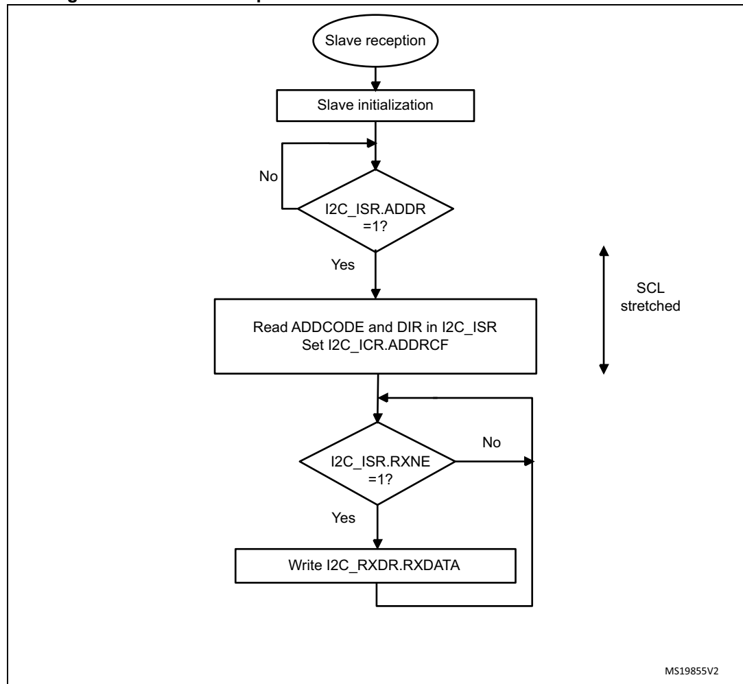
Figure 521. Transfer sequence flow for slave receiver with NOSTRETCH = 0
