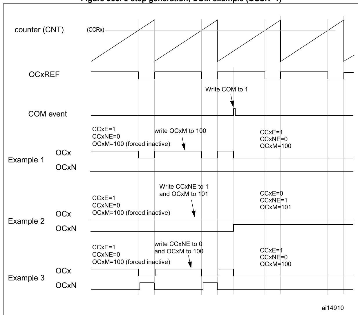
Figure 366. 6-step generation, COM example (OSSR=1)
