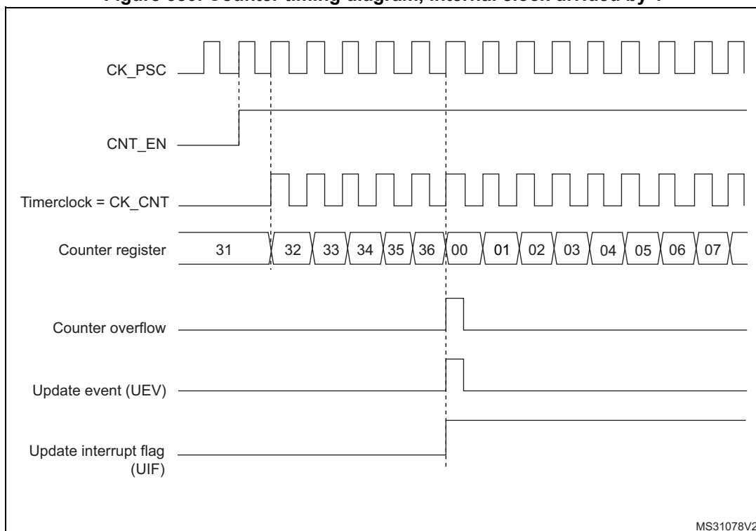
Figure 380. Counter timing diagram, internal clock divided by 1
