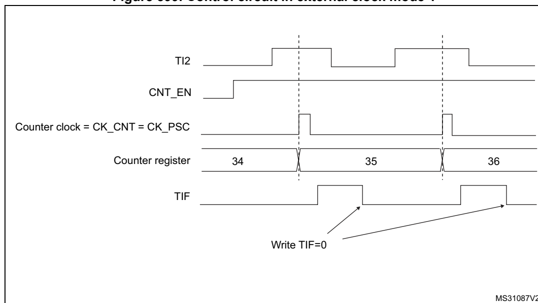
Figure 399. Control circuit in external clock mode 1
