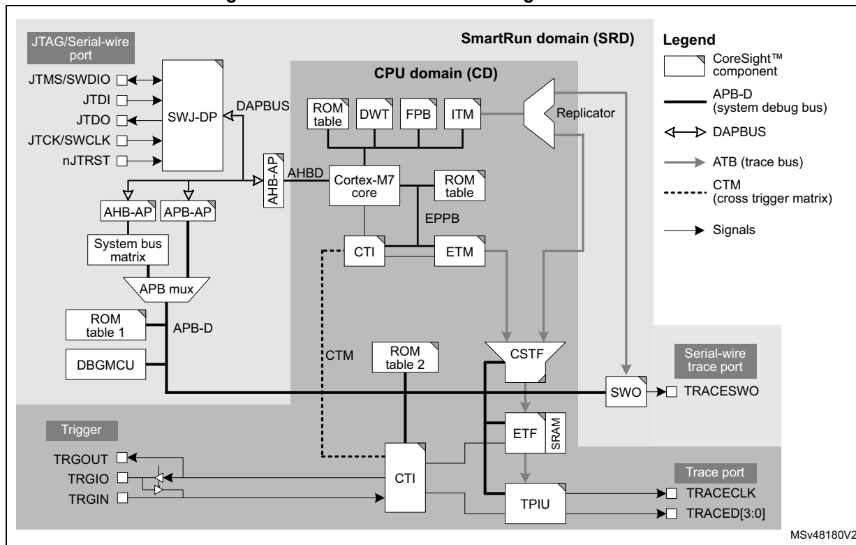
Figure 763. Power domains of debug infrastructure
