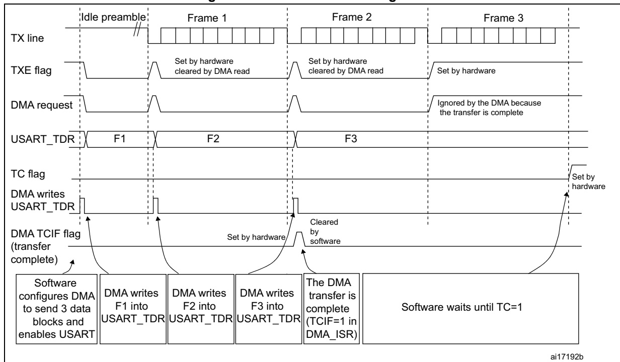
Figure 562. Transmission using DMA
