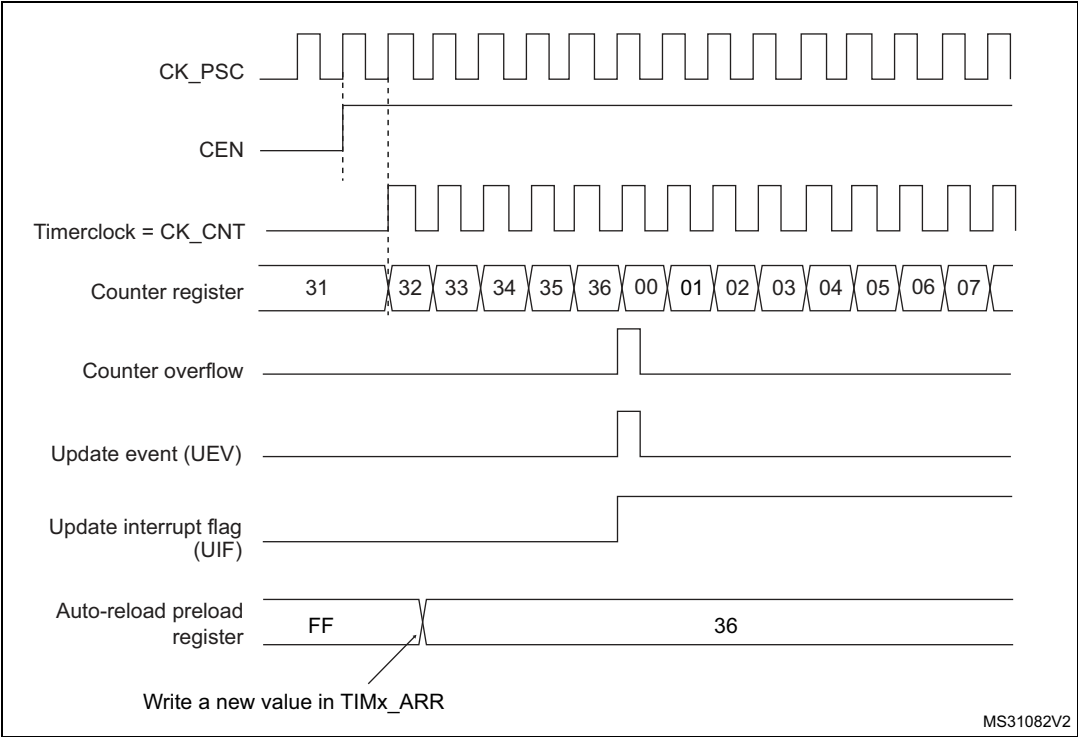
Figure 384. Counter timing diagram, Update event when ARPE=0 (TIMx_ARR not preloaded)
