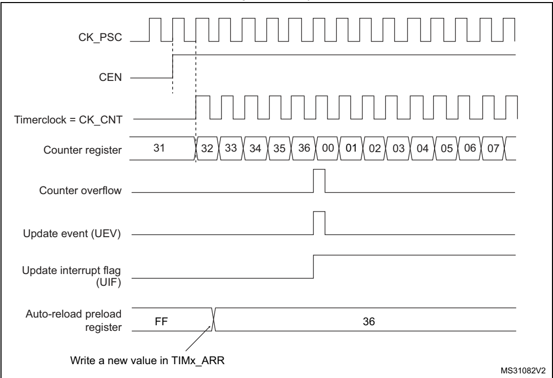
Figure 435. Counter timing diagram, update event when ARPE=0 (TIMx_ARR not preloaded)
