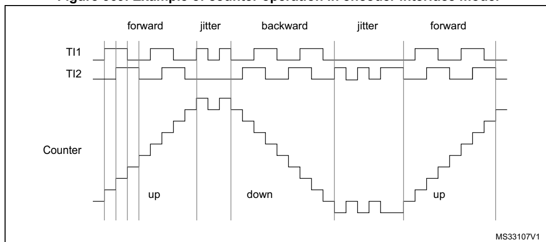
Figure 369. Example of counter operation in encoder interface mode.
