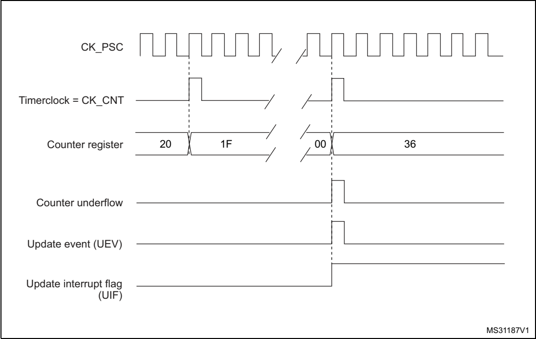
Figure 329. Counter timing diagram, internal clock divided by N
