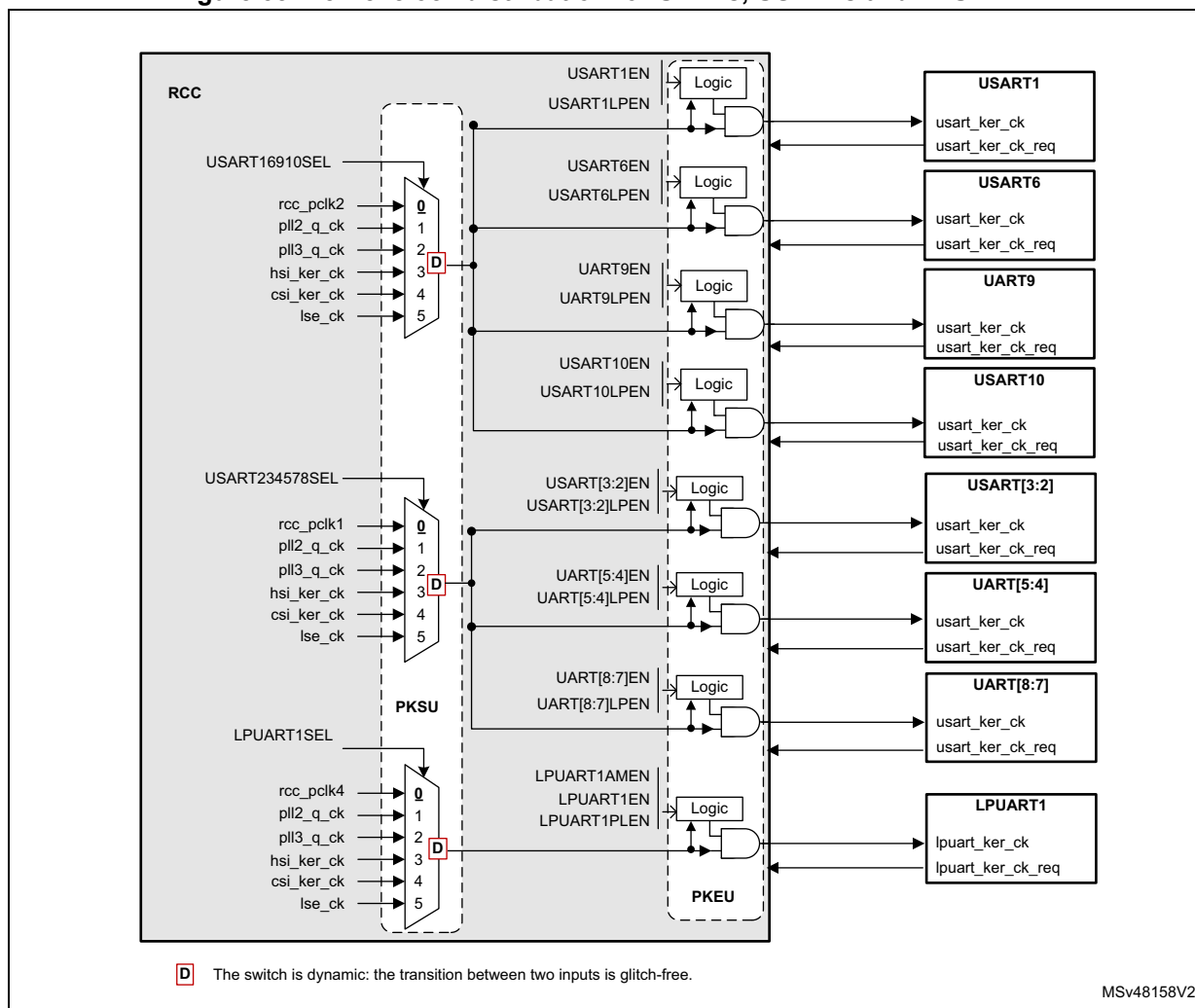
Figure 58. Kernel clock distribution for UARTs, USARTs and LPUART1
