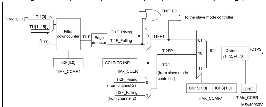
Figure 440. Capture/compare channel (example: channel 1 input stage)
