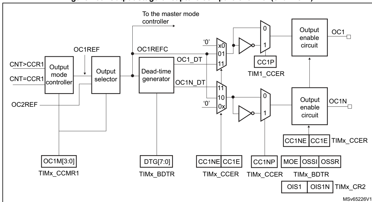
Figure 469. Output stage of capture/compare channel (channel 1)
