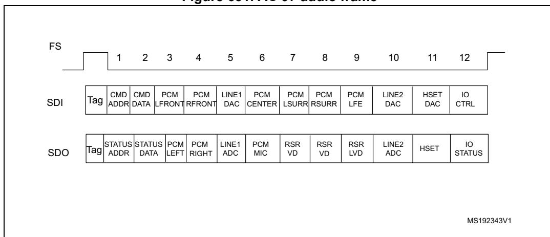
Figure 631. AC'97 audio frame
