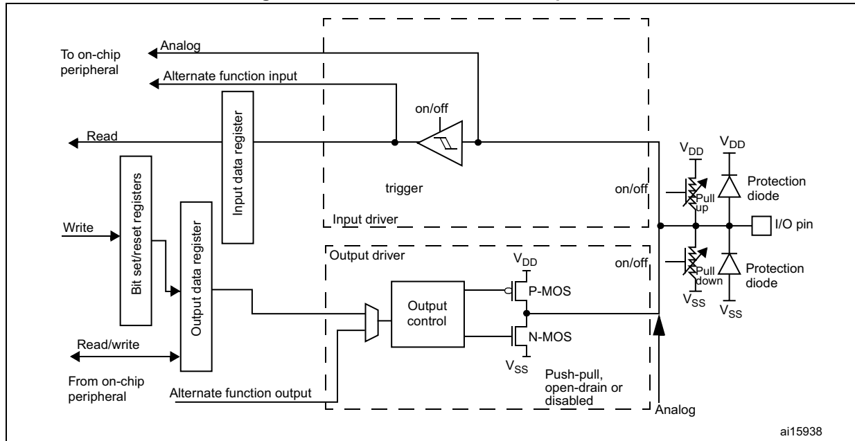
Figure 73. Basic structure of an I/O port bit
