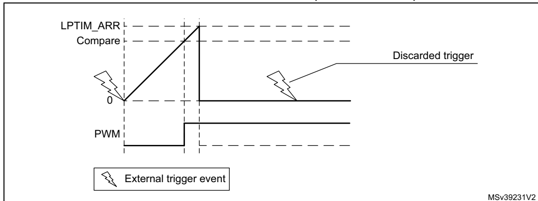
Figure 502. LPTIM output waveform, Single counting mode configuration and Set-once mode activated (WAVE bit is set)
