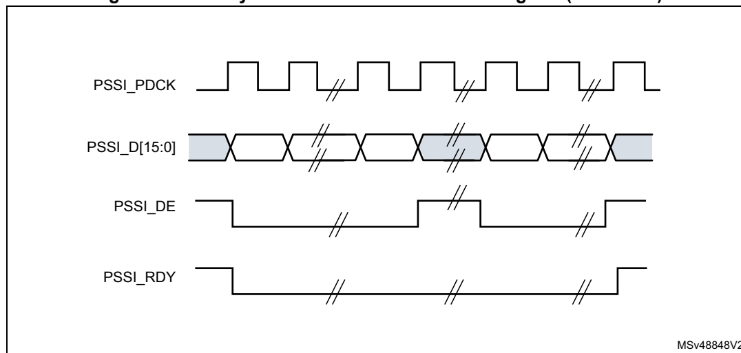
Figure 273. Ready in receive mode waveform diagram (CKPOL=0)
