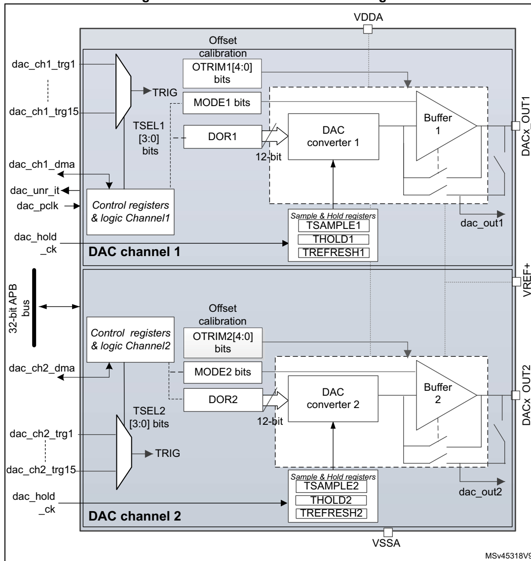
Figure 231. Dual-channel DAC block diagram
