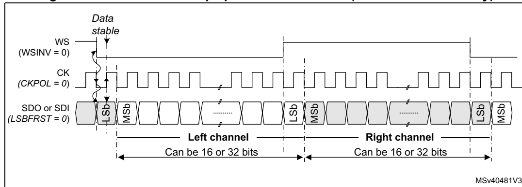
Figure 600. Master I2S Philips protocol waveforms (16/32-bit full accuracy)
