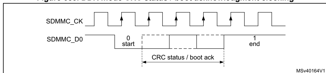
Figure 683. DDR mode CRC status / boot acknowledgment clocking
