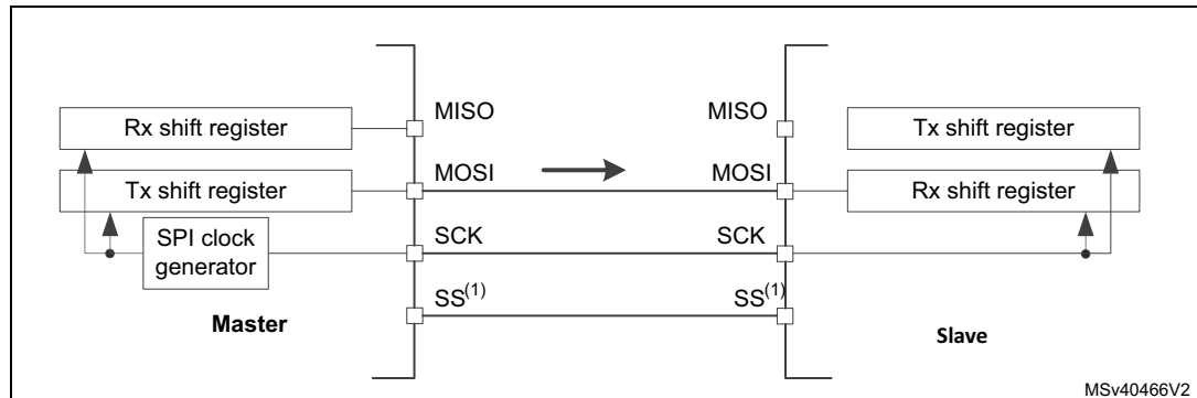
Figure 586. Simplex single master/single slave application (master in transmit-only/ slave in receive-only mode)
