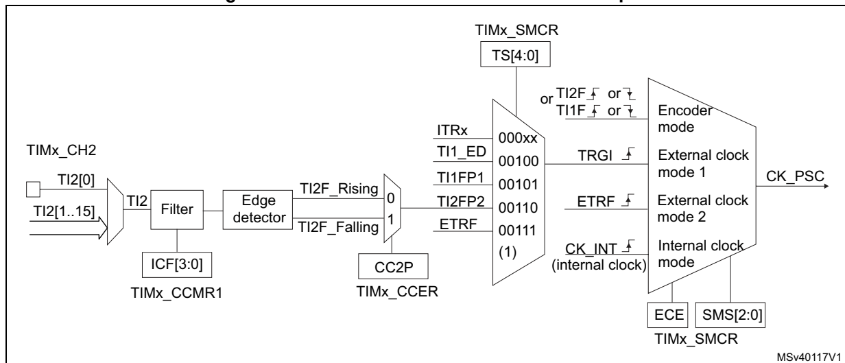
Figure 341. TI2 external clock connection example
