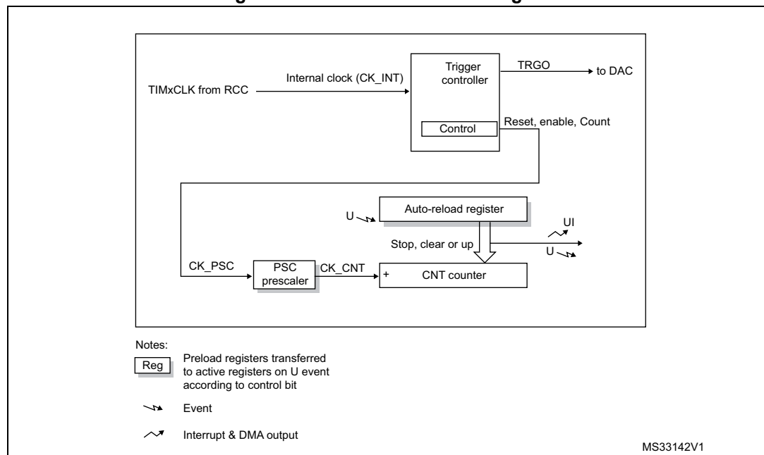
Figure 488. Basic timer block diagram
