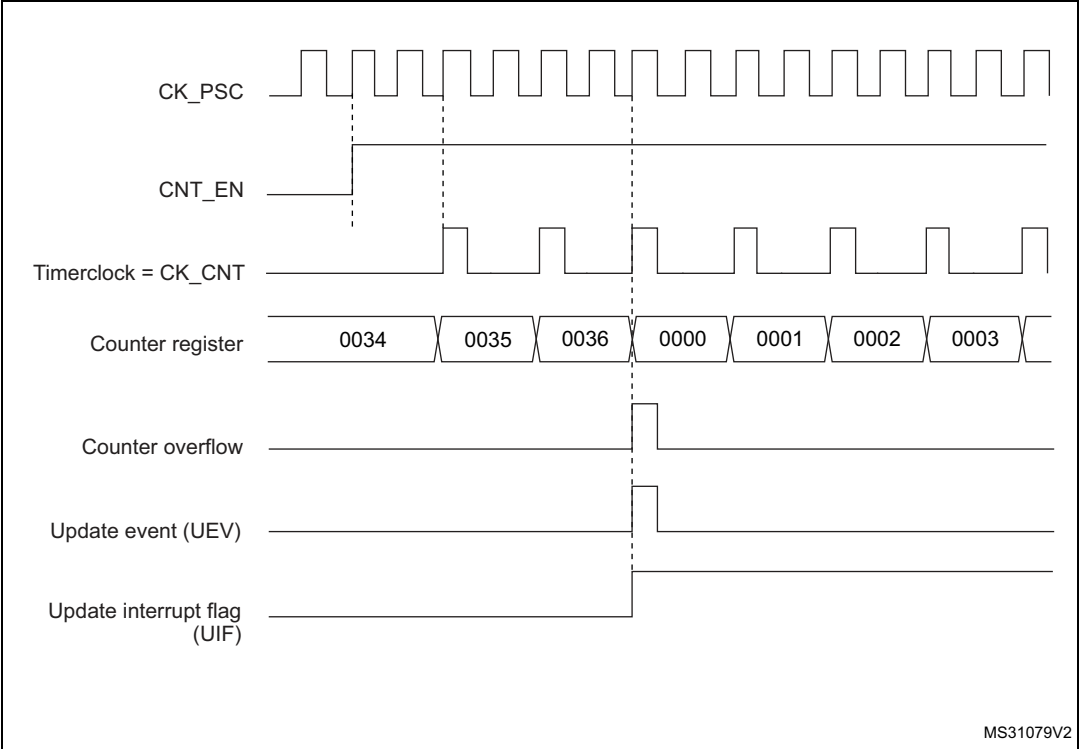
Figure 432. Counter timing diagram, internal clock divided by 2
