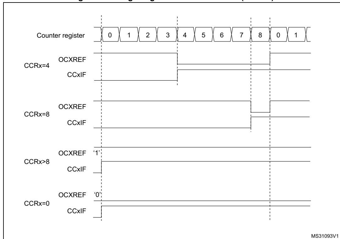
Figure 473. Edge-aligned PWM waveforms (ARR=8)
