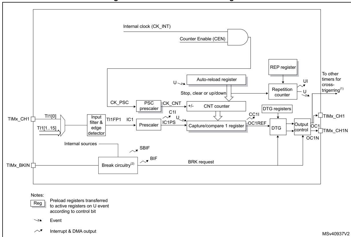
Figure 454. TIM16/TIM17 block diagram
