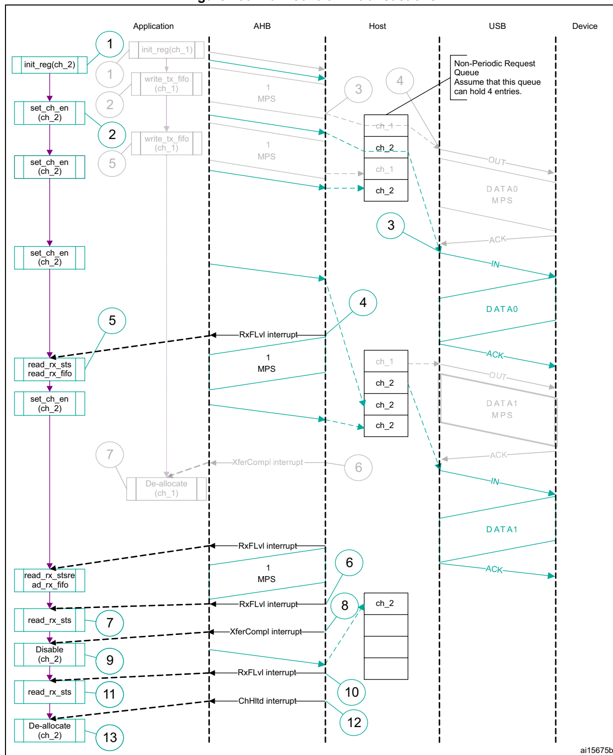
Figure 733. Bulk/control IN transactions
