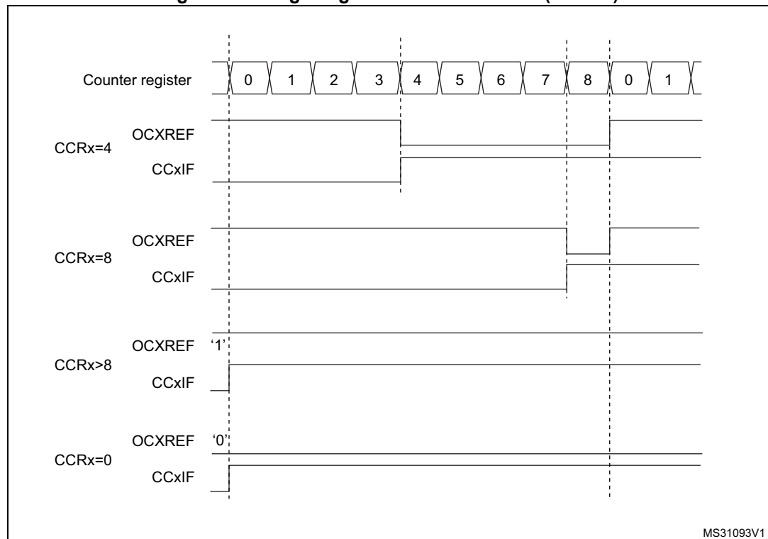
Figure 352. Edge-aligned PWM waveforms (ARR=8)
