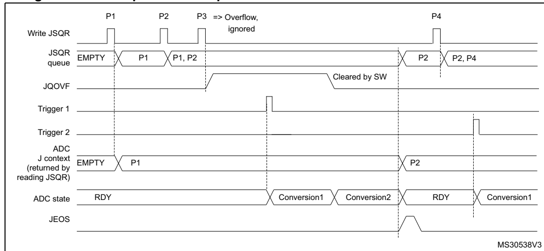
Figure 172. Example of JSQR queue of context with overflow before conversion
