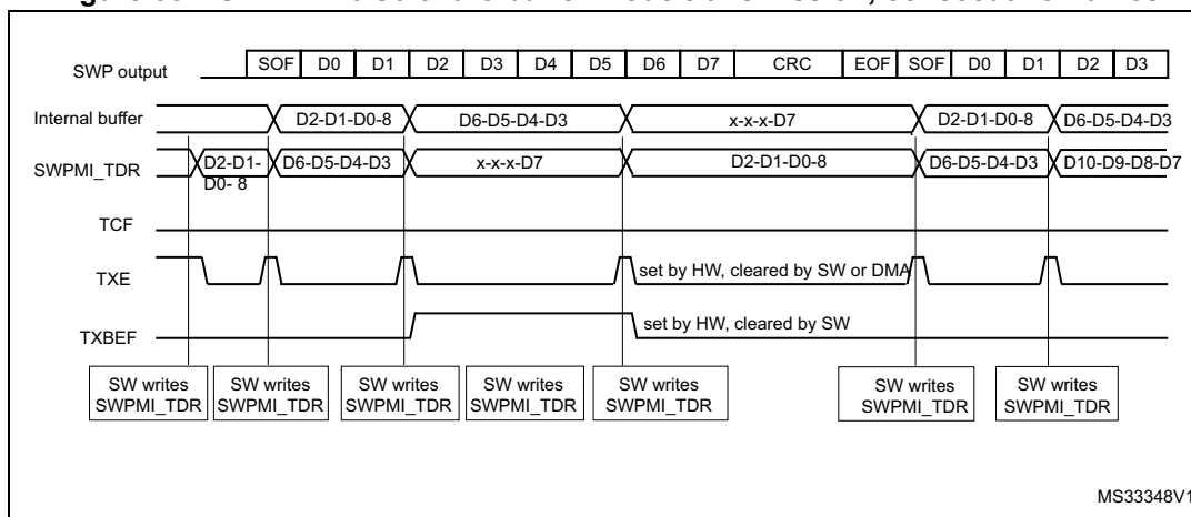
Figure 662. SWPMI No software buffer mode transmission, consecutive frames
