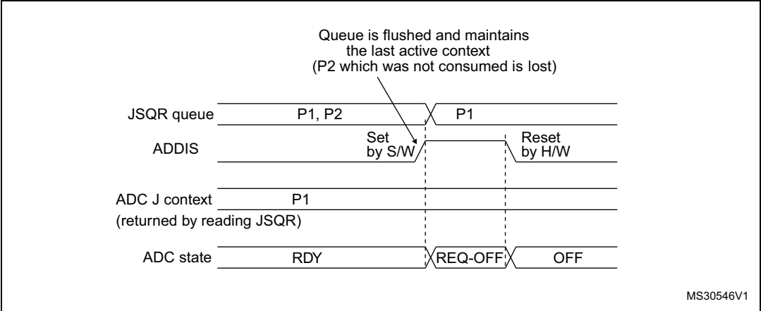
Figure 180. Flushing JSQR queue of context by setting ADDIS=1 (JQM=0)
