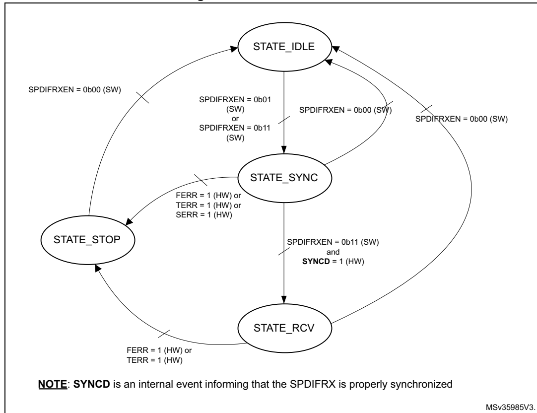
Figure 650. SPDIFRX States
