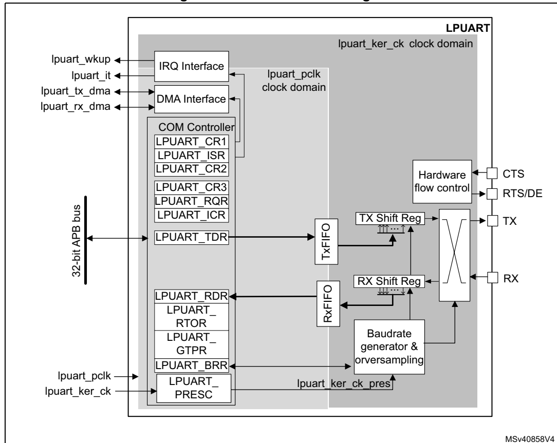
Figure 569. LPUART block diagram
