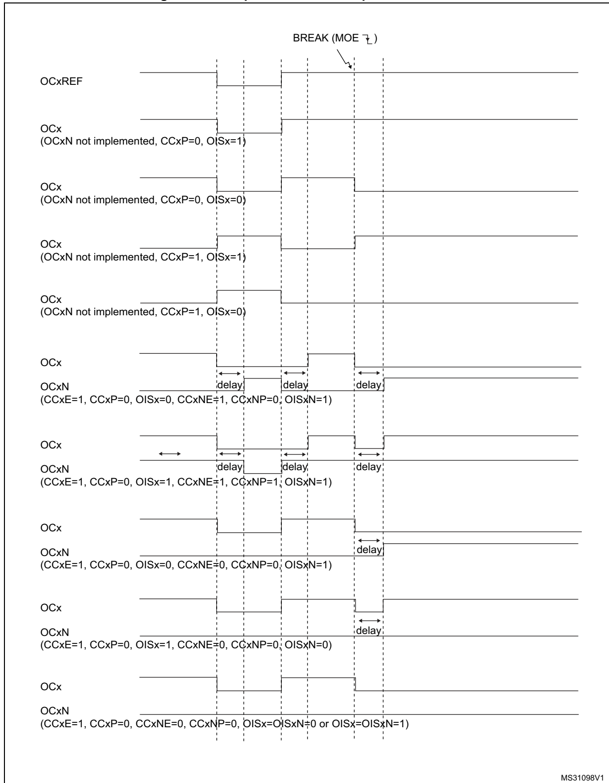
Figure 479. Output behavior in response to a break
