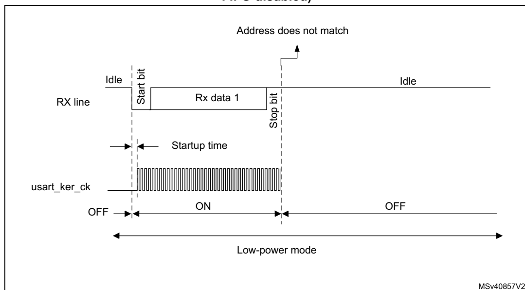
Figure 568. Wake-up event not verified (wake-up event = address match, FIFO disabled)
