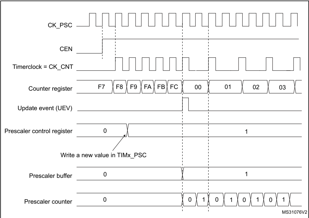
Figure 318. Counter timing diagram with prescaler division change from 1 to 2
