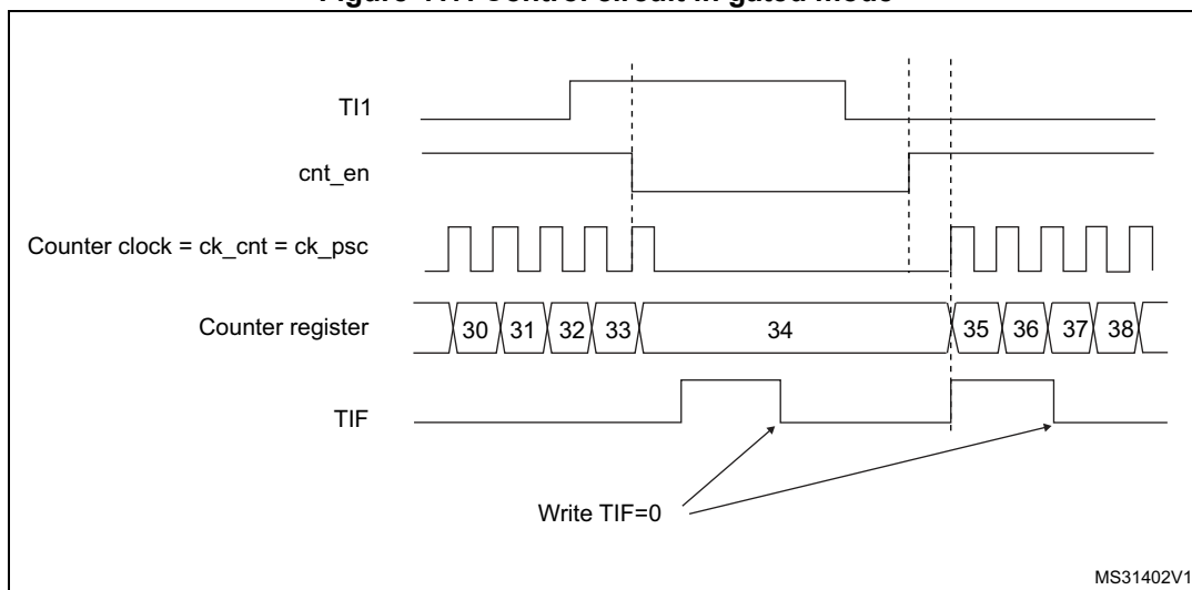
Figure 417. Control circuit in gated mode
