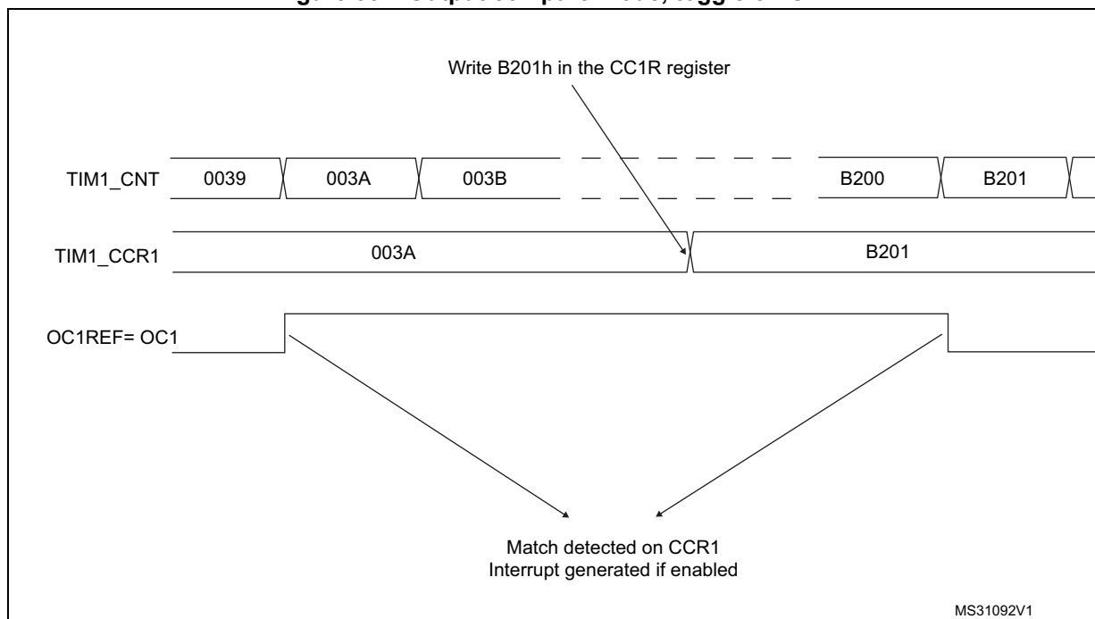
Figure 351. Output compare mode, toggle on OC1
