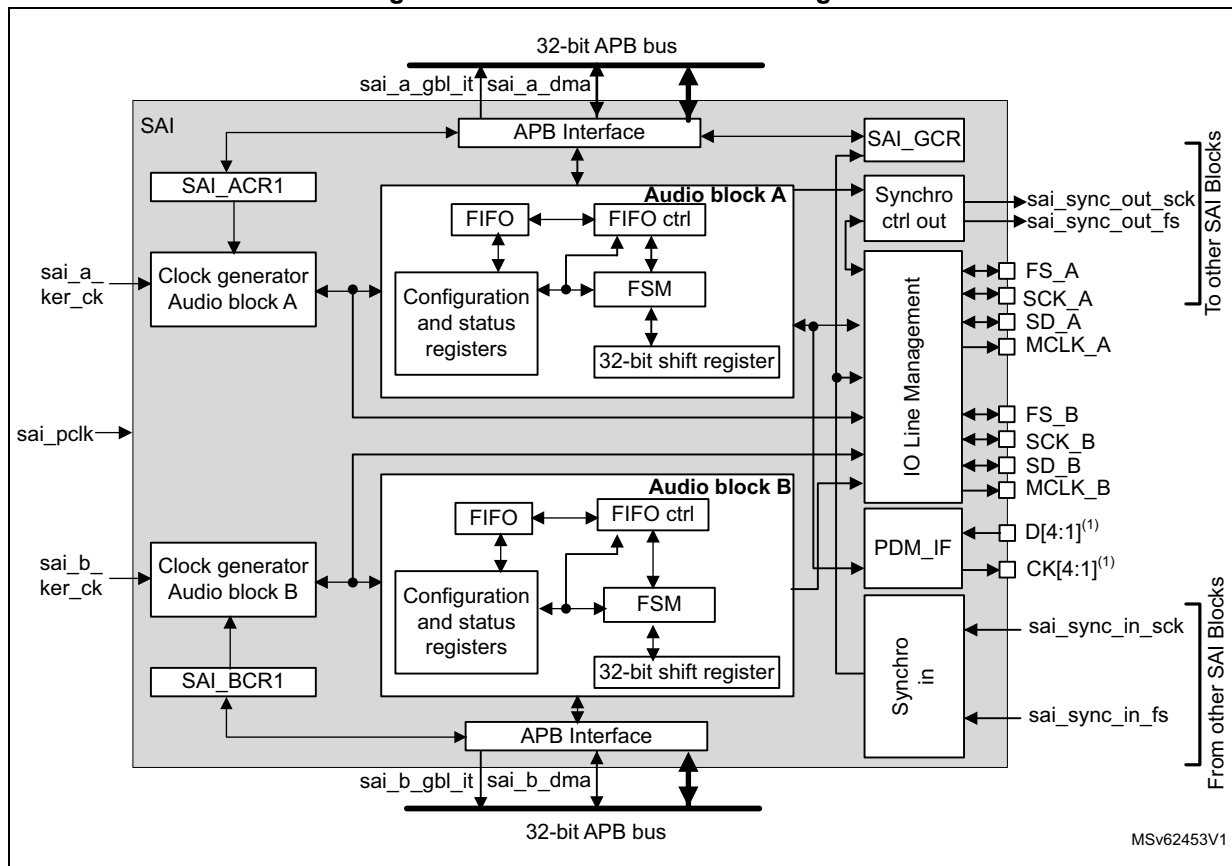
Figure 618. SAI functional block diagram
