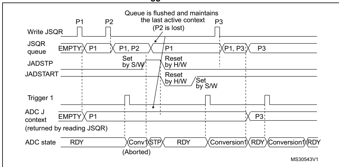
Figure 177. Flushing JSQR queue of context by setting JADSTP=1 (JQM=0). Case when JADSTP occurs during an ongoing conversion and a new trigger occurs.
