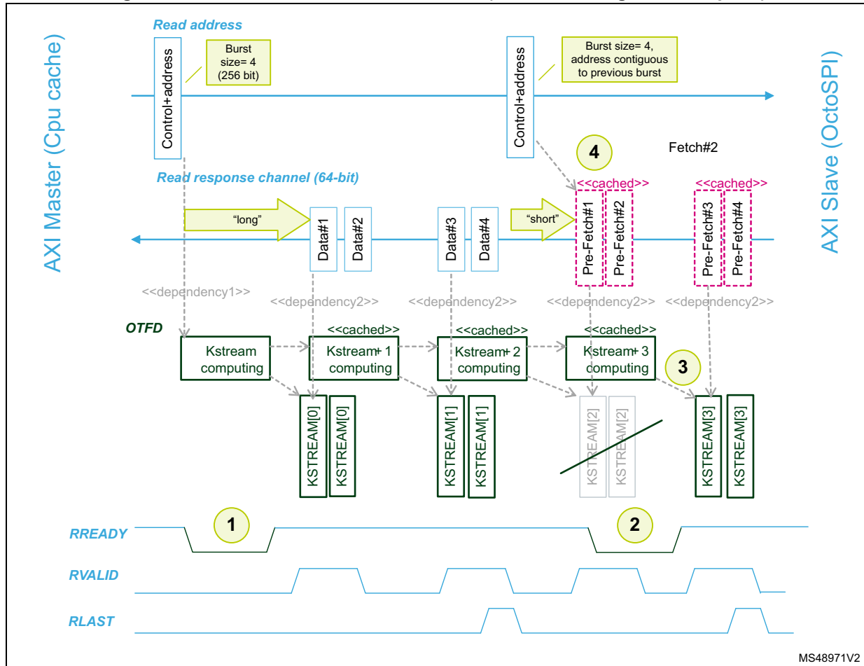
Figure 316. OTFDEC flow control overview (burst then single read request)
