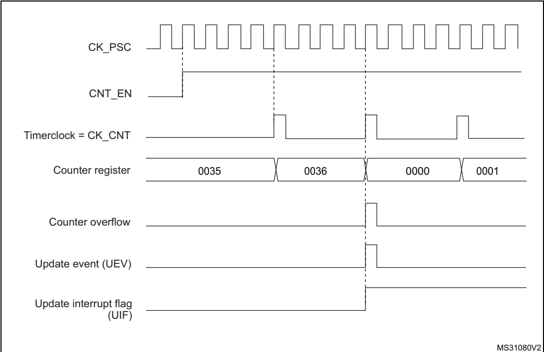
Figure 433. Counter timing diagram, internal clock divided by 4
