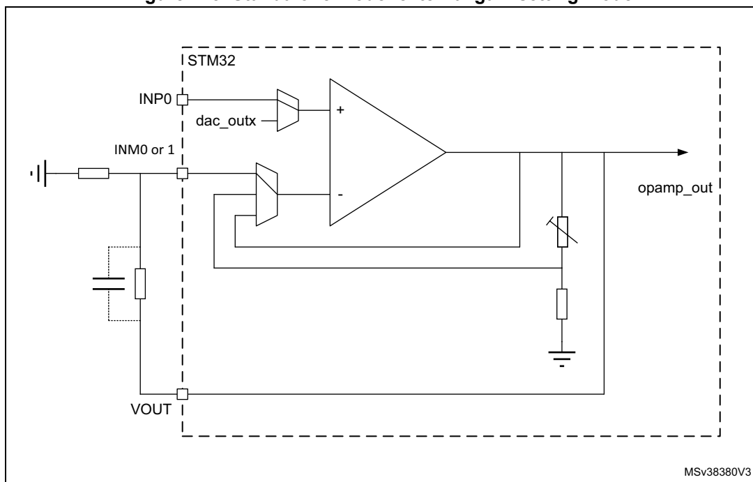
Figure 245. Standalone mode: external gain setting mode
