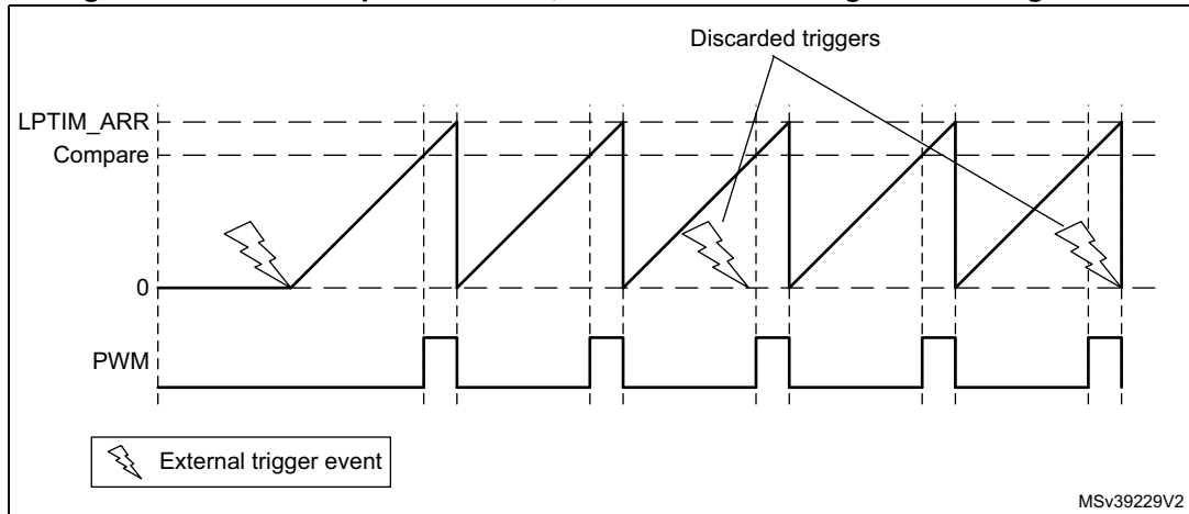
Figure 503. LPTIM output waveform, Continuous counting mode configuration
