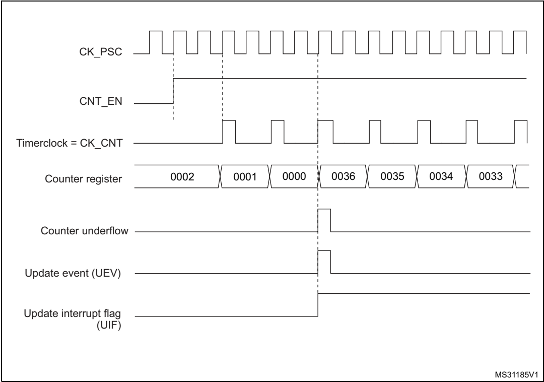
Figure 387. Counter timing diagram, internal clock divided by 2
