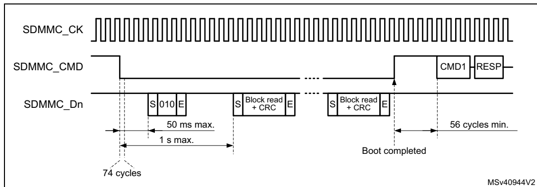
Figure 697. Normal boot mode operation
