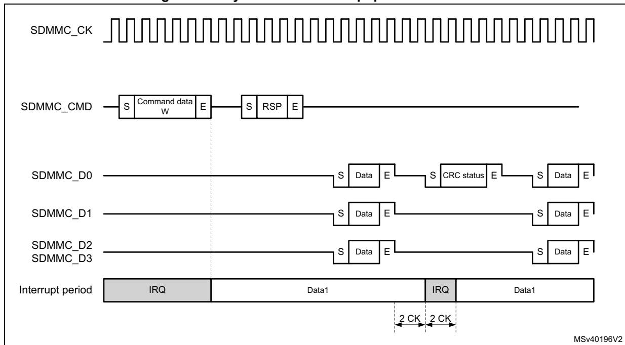
Figure 688. Synchronous interrupt period data write
