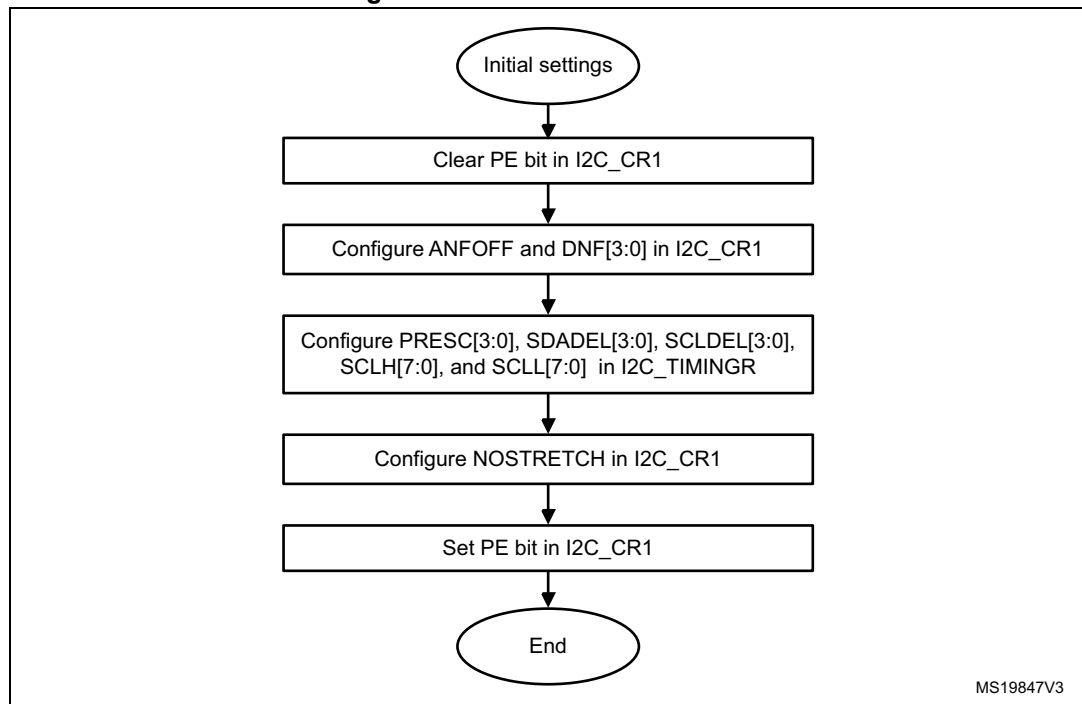
Figure 514. I2C initialization flow
