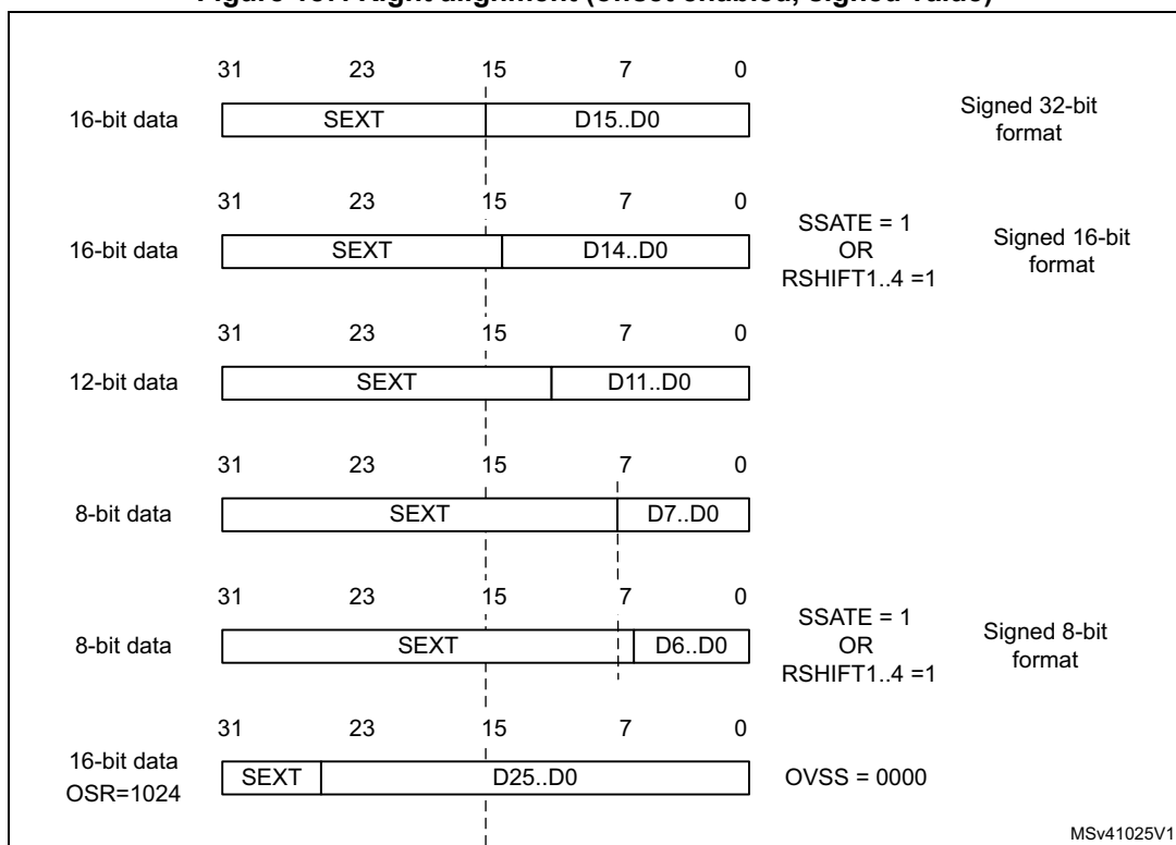
Figure 187. Right alignment (offset enabled, signed value)
