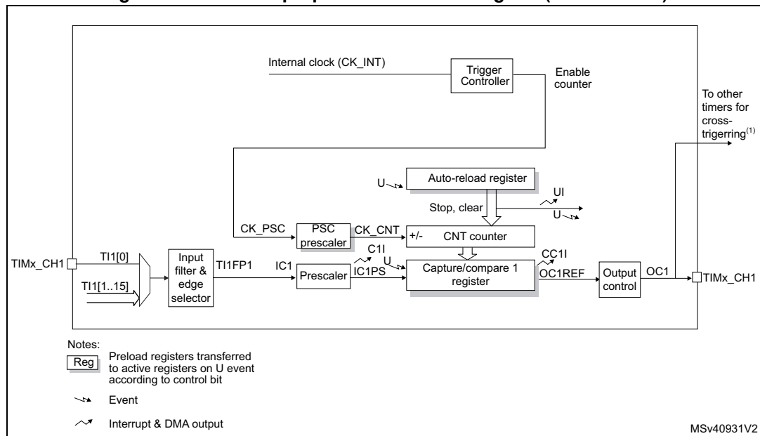
Figure 428. General-purpose timer block diagram (TIM13/TIM14)
