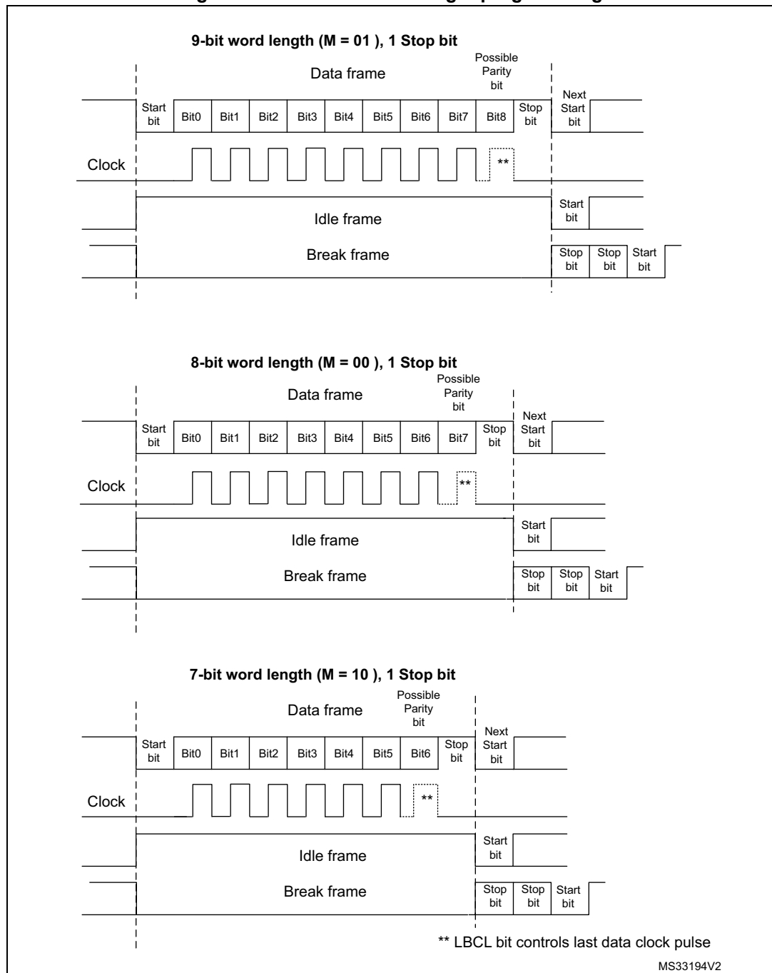
Figure 570. LPUART word length programming
