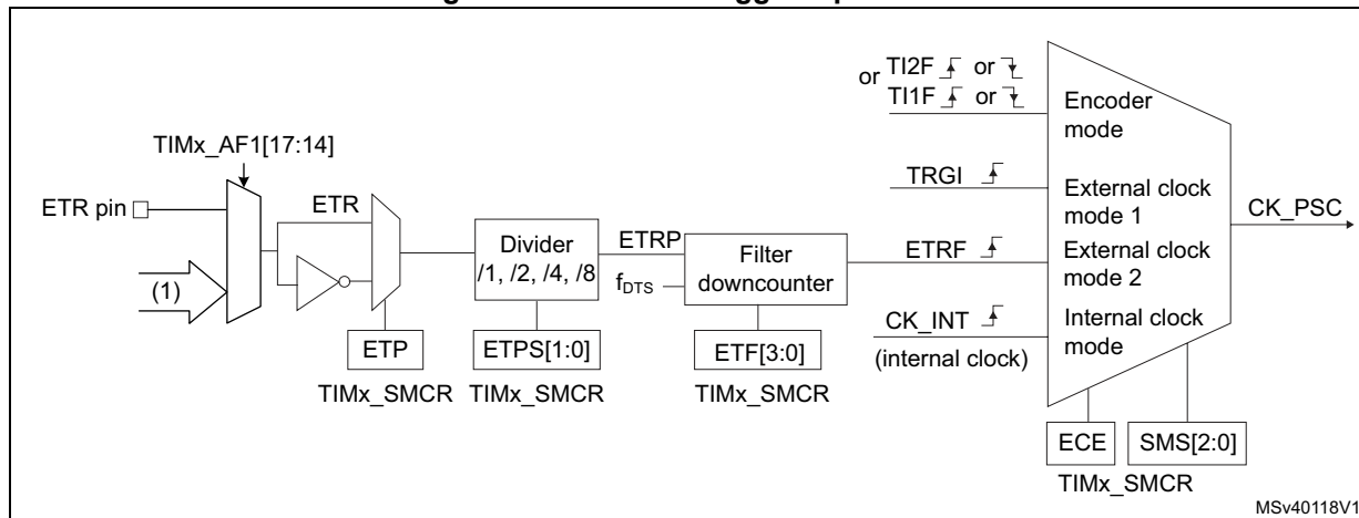
Figure 343. External trigger input block
