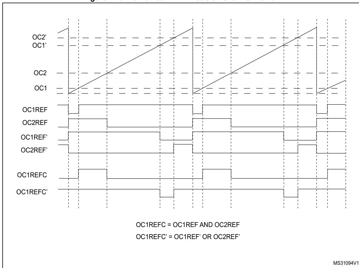
Figure 446. Combined PWM mode on channel 1 and 2
