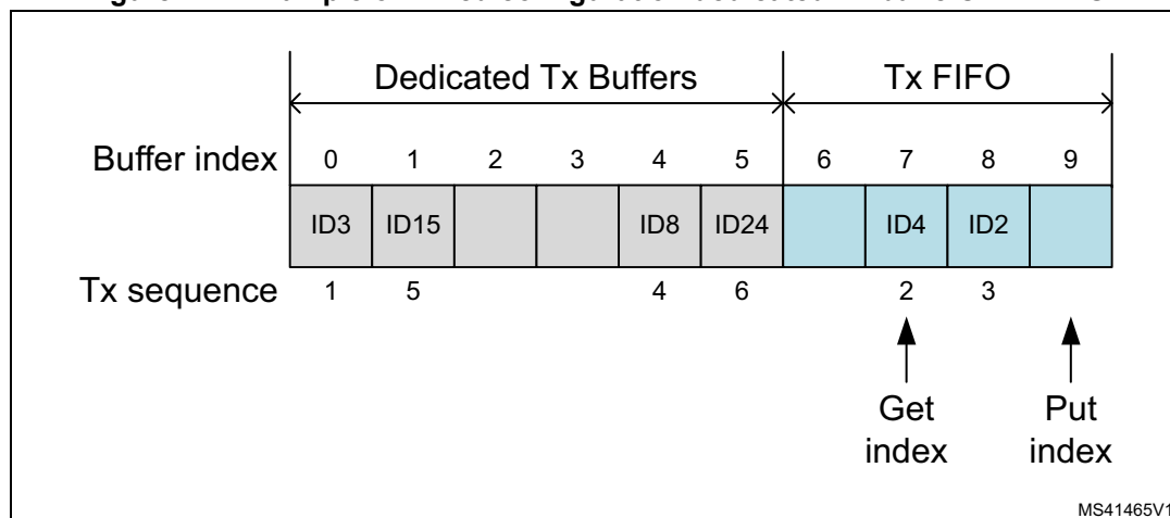
Figure 712. Example of mixed configuration dedicated Tx buffers / Tx FIFO
