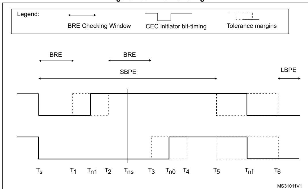
Figure 760. Error handling
