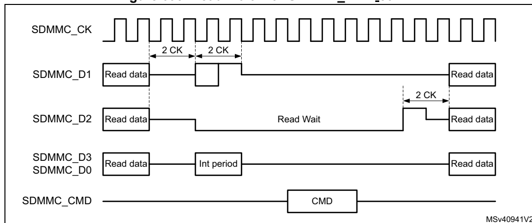
Figure 693. Read Wait with SDMMC_CLK < 50 MHz
