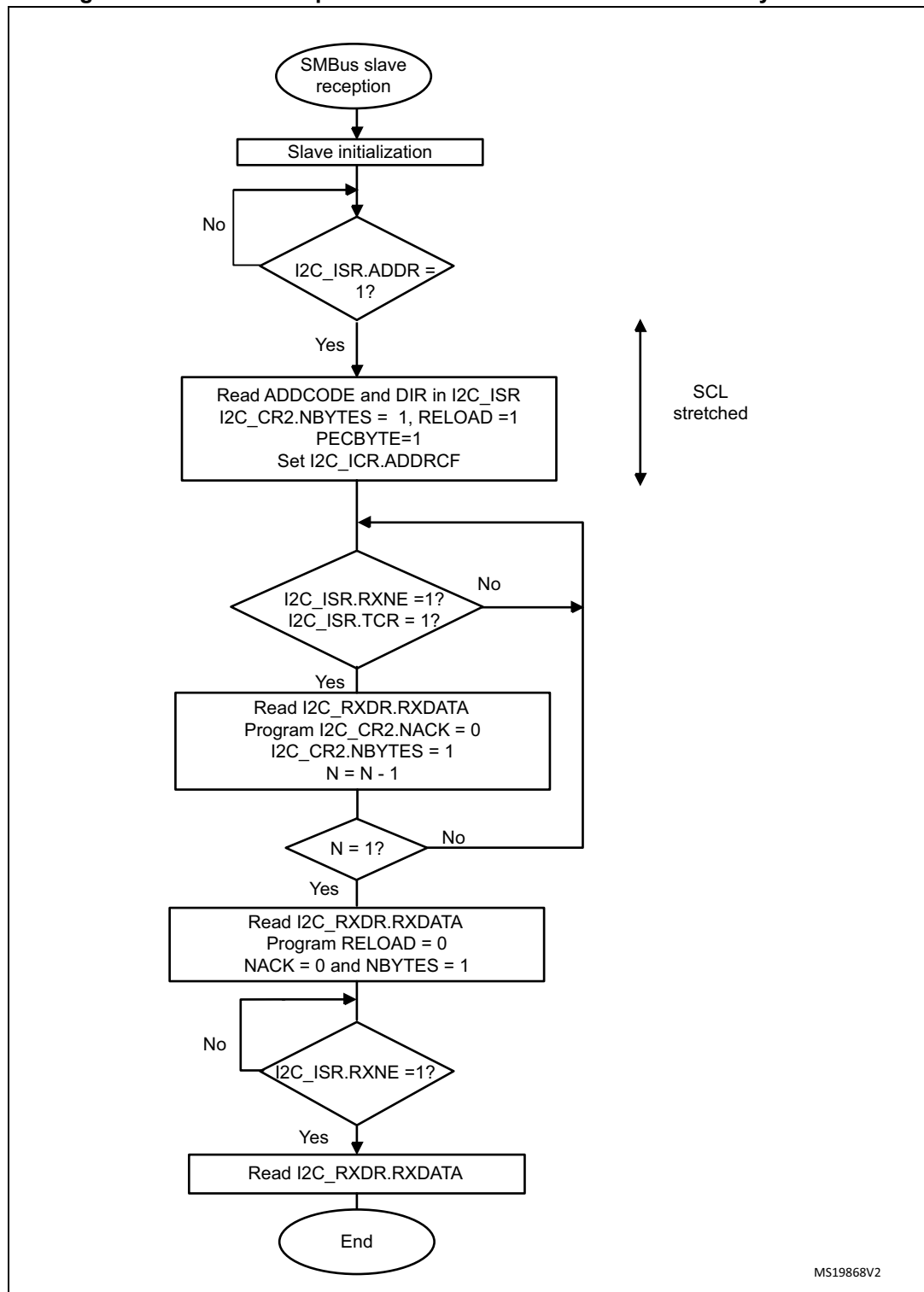
Figure 537. Transfer sequence flow for SMBus slave receiver N bytes + PEC
