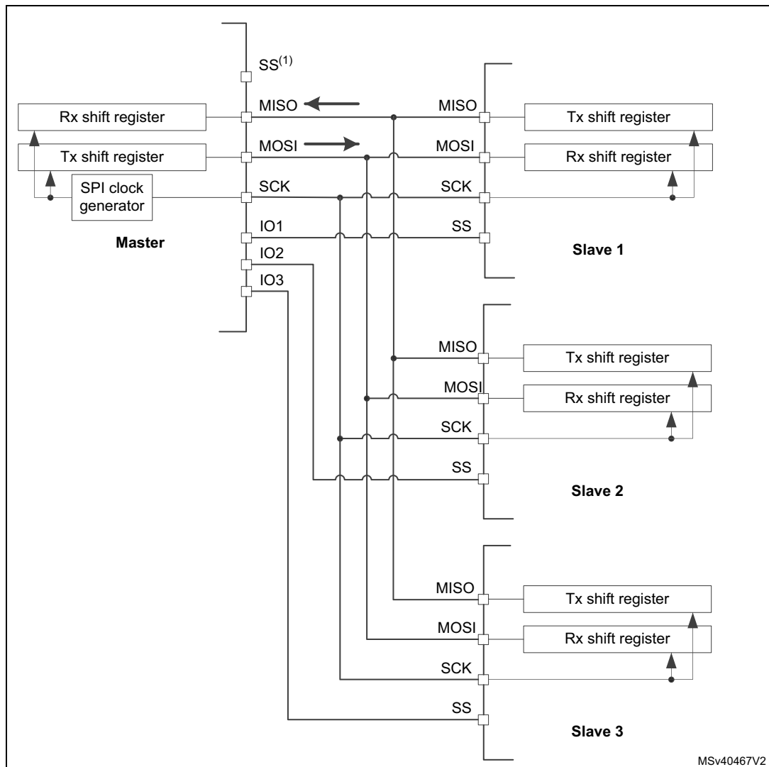
Figure 587. Master and three independent slaves at star topology
