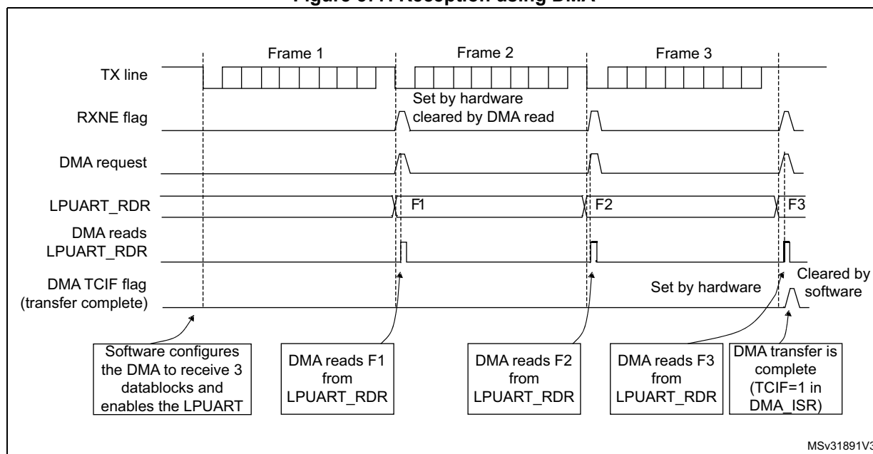
Figure 577. Reception using DMA
