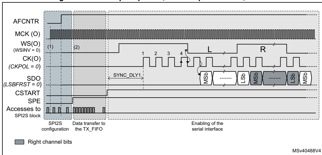
Figure 609. Startup sequence, I2S Philips standard, master
