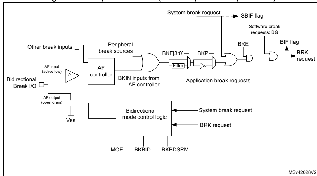
Figure 364. Output redirection (BRK2 request not represented)
