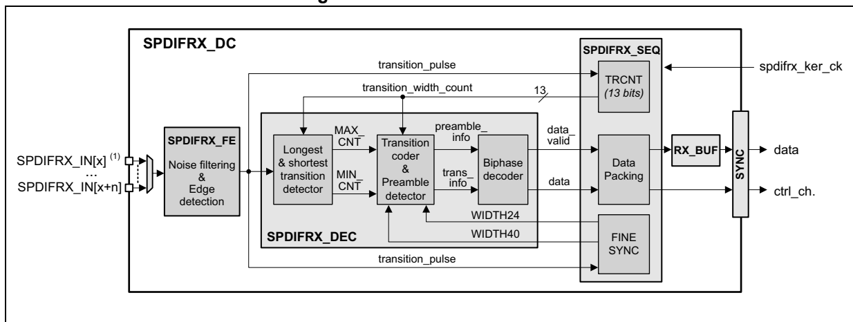
Figure 645. SPDIFRX decoder
