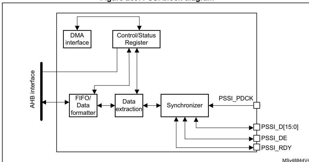
Figure 270. Top-level block diagram
