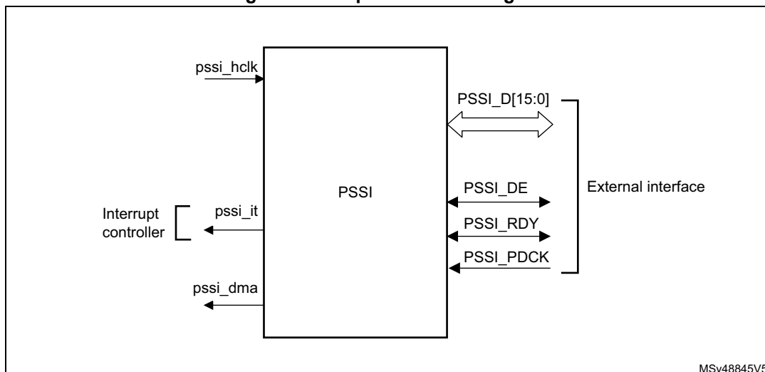
Figure 270. Top-level block diagram
