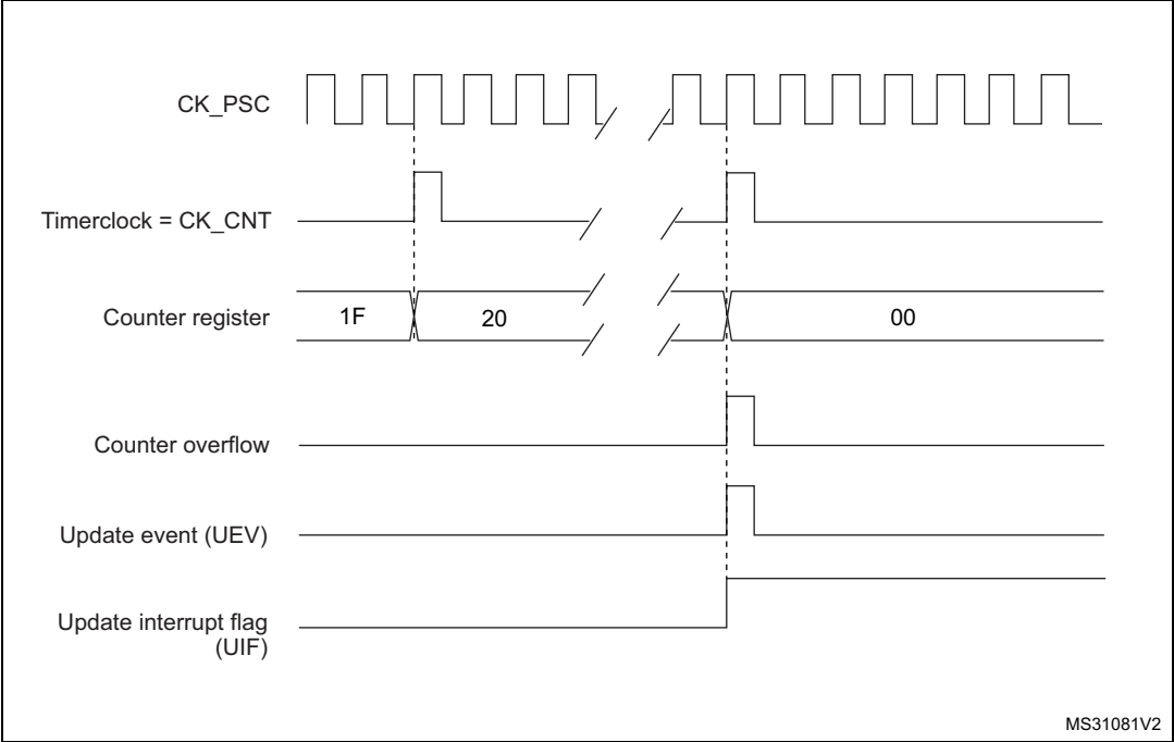
Figure 460. Counter timing diagram, internal clock divided by N
