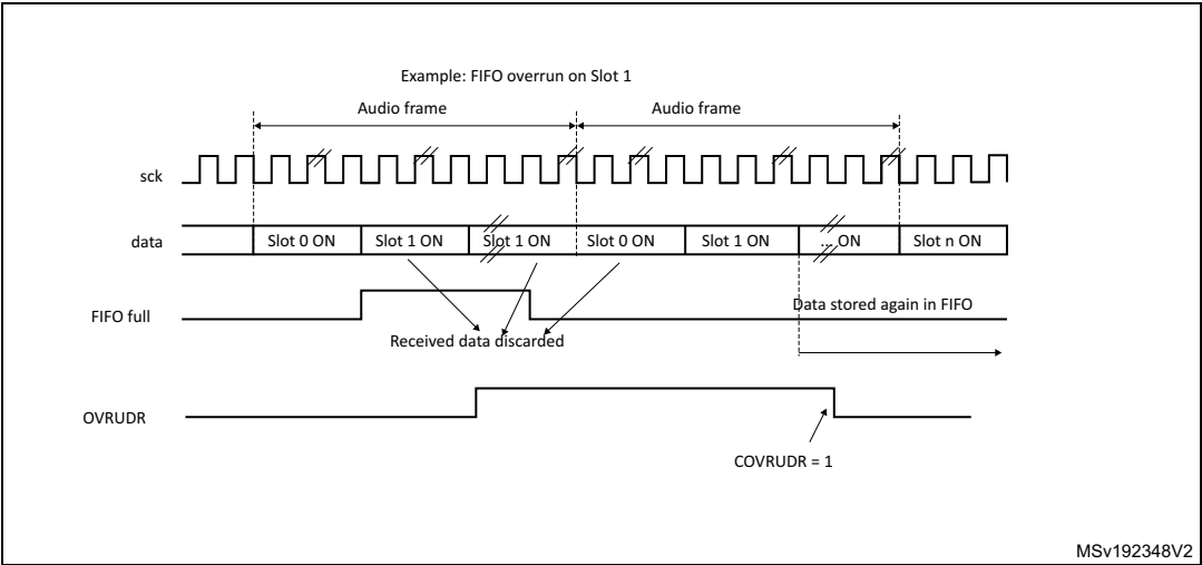
Figure 638. Overrun detection error
