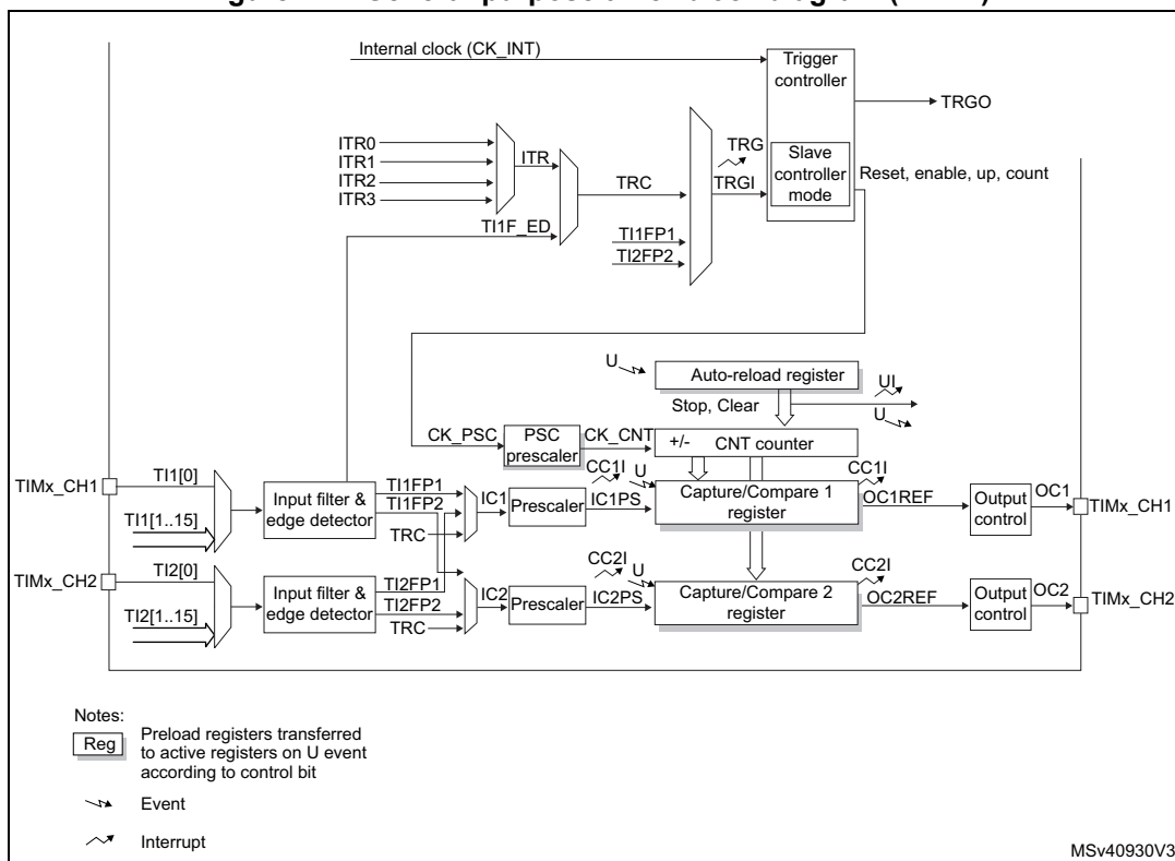
Figure 427. General-purpose timer block diagram (TIM12)
