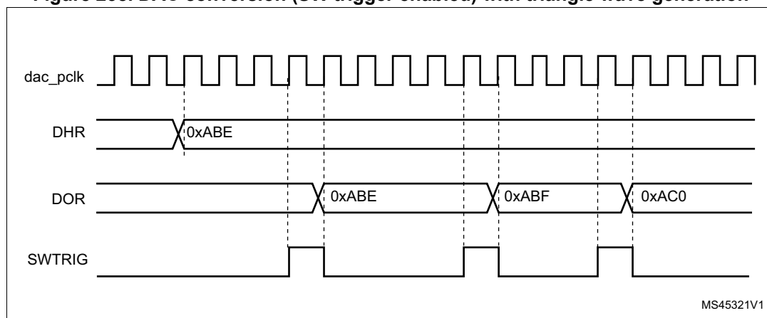
Figure 238. DAC conversion (SW trigger enabled) with triangle wave generation
