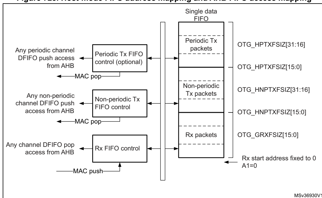
Figure 728. Host-mode FIFO address mapping and AHB FIFO access mapping
