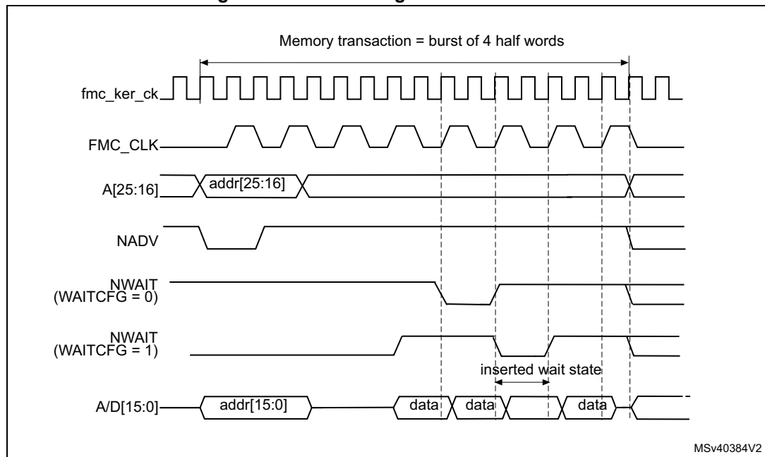
Figure 125. Synchronous multiplexed read mode waveforms - NOR, PSRAM (CRAM)
