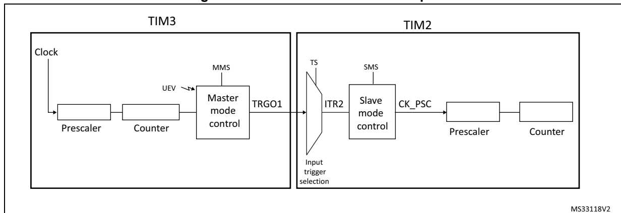
Figure 421. Master/slave connection example with 1 channel only timers
