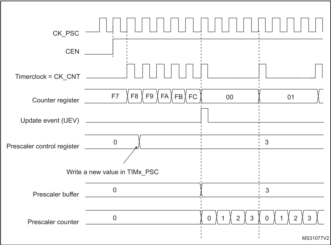
Figure 319. Counter timing diagram with prescaler division change from 1 to 4
