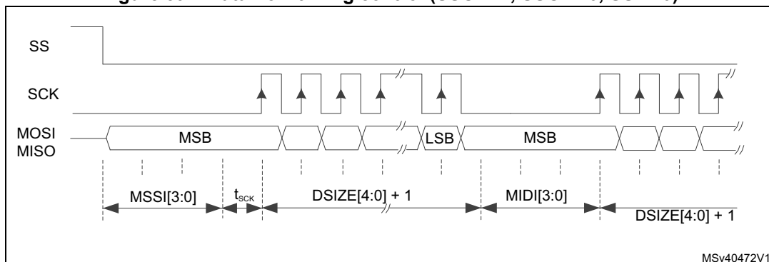
Figure 591. Data flow timing control (SSOE=1, SSOM=0, SSM=0)
