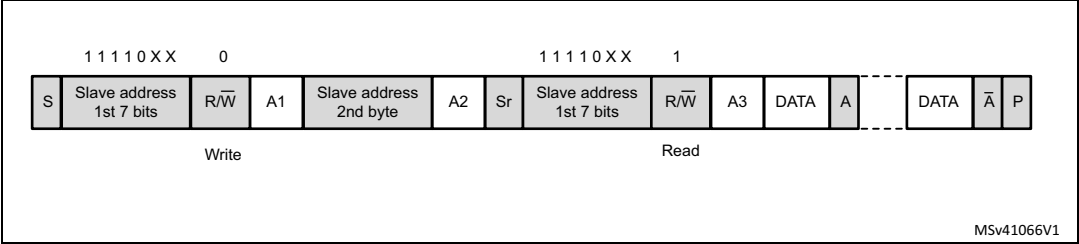
Figure 526. 10-bit address read access with HEAD10R = 0
