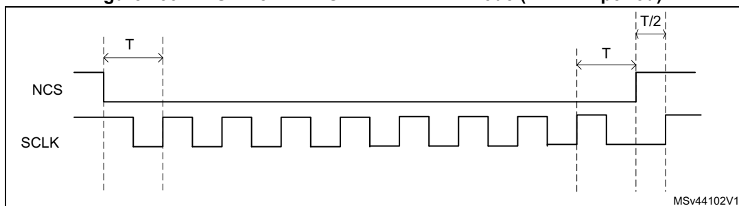
Figure 153. NCS when CKMODE = 1 in DTR mode ( T = \text{CLK period} )
