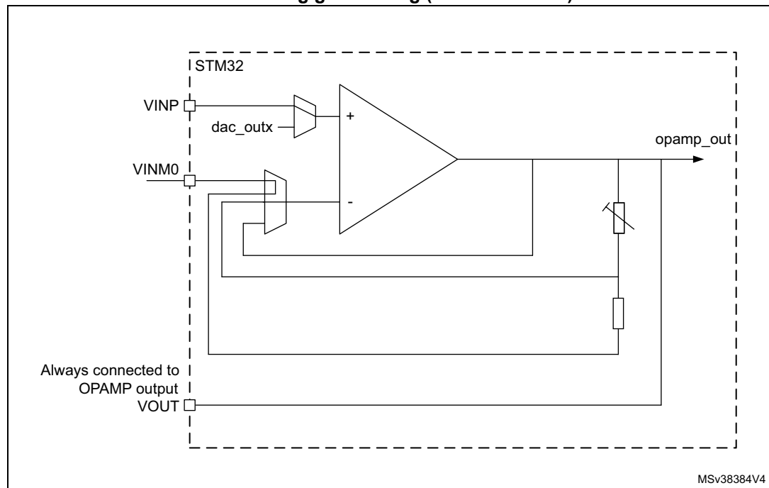
Figure 249. PGA mode, non-inverting gain setting (x2/x4/x8/x16) or inverting gain setting (x-1/x-3/x-7/x-15)
