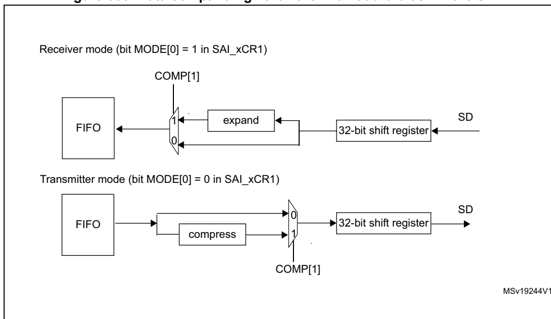
Figure 635. Data companding hardware in an audio block in the SAI
