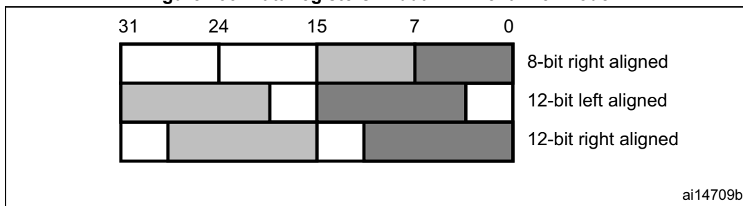
Figure 233. Data registers in dual DAC channel mode
