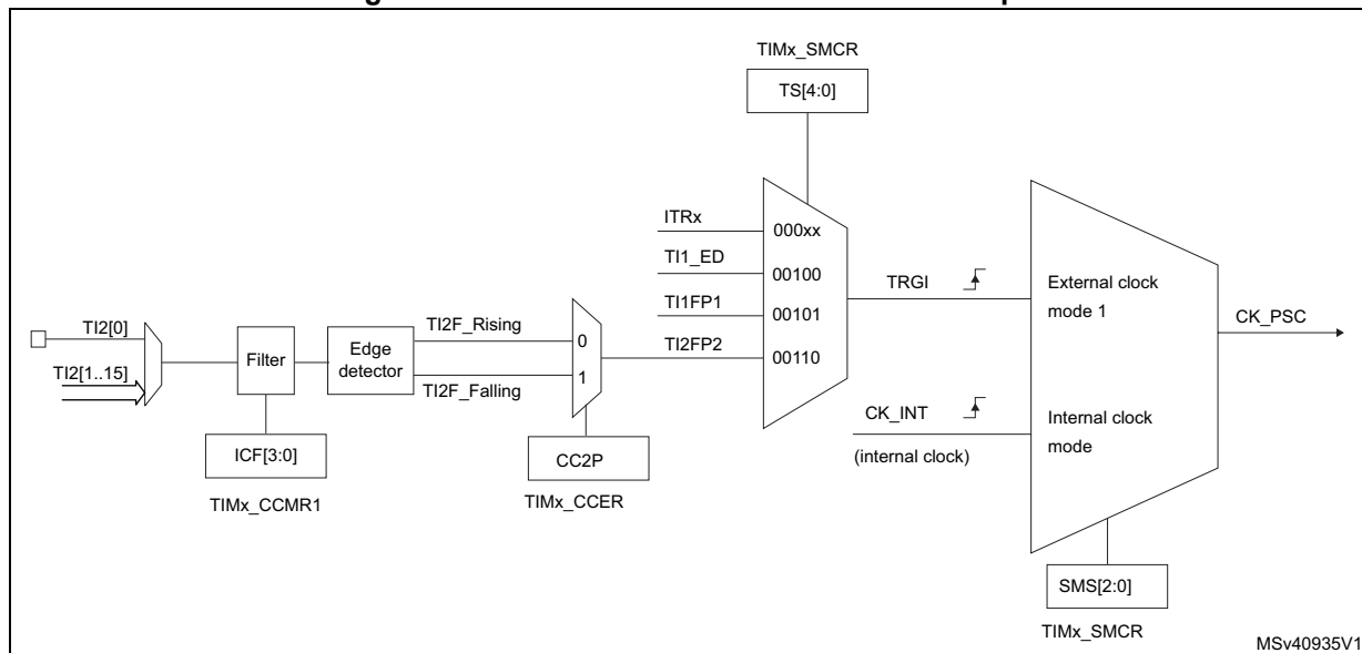
Figure 465. TI2 external clock connection example
