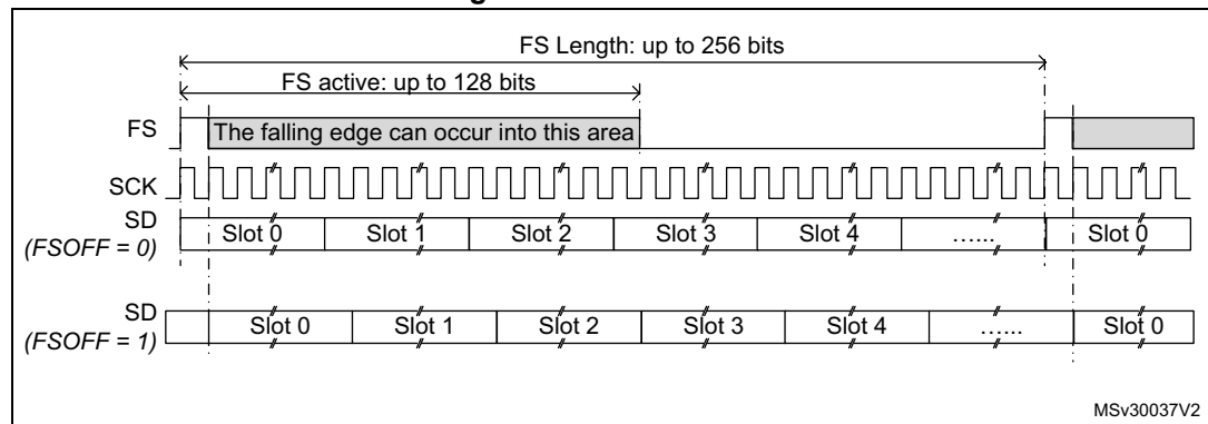
Figure 619. Audio frame
