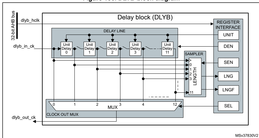
Figure 156. DLYB block diagram
