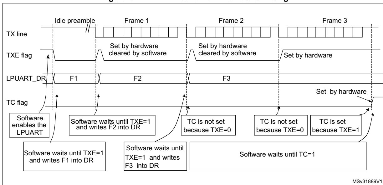
Figure 572. TC/TXE behavior when transmitting
