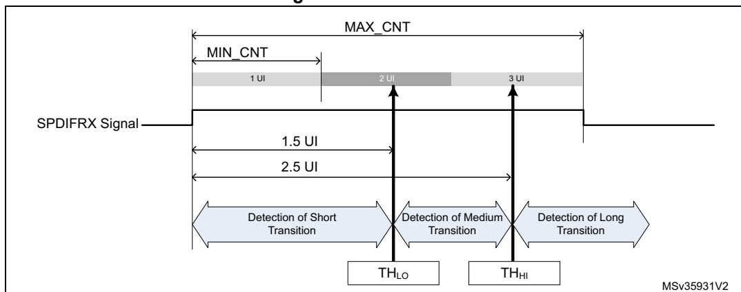
Figure 647. Thresholds
