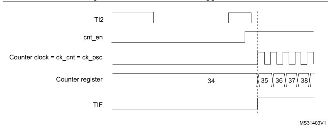
Figure 375. Control circuit in trigger mode
