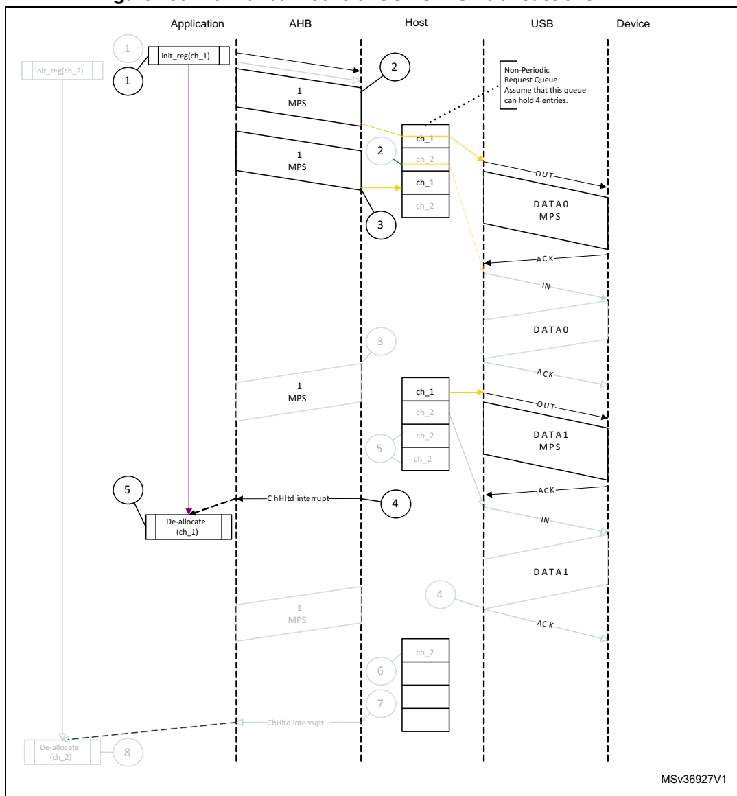
Figure 738. Normal bulk/control OUT/SETUP transactions - DMA
