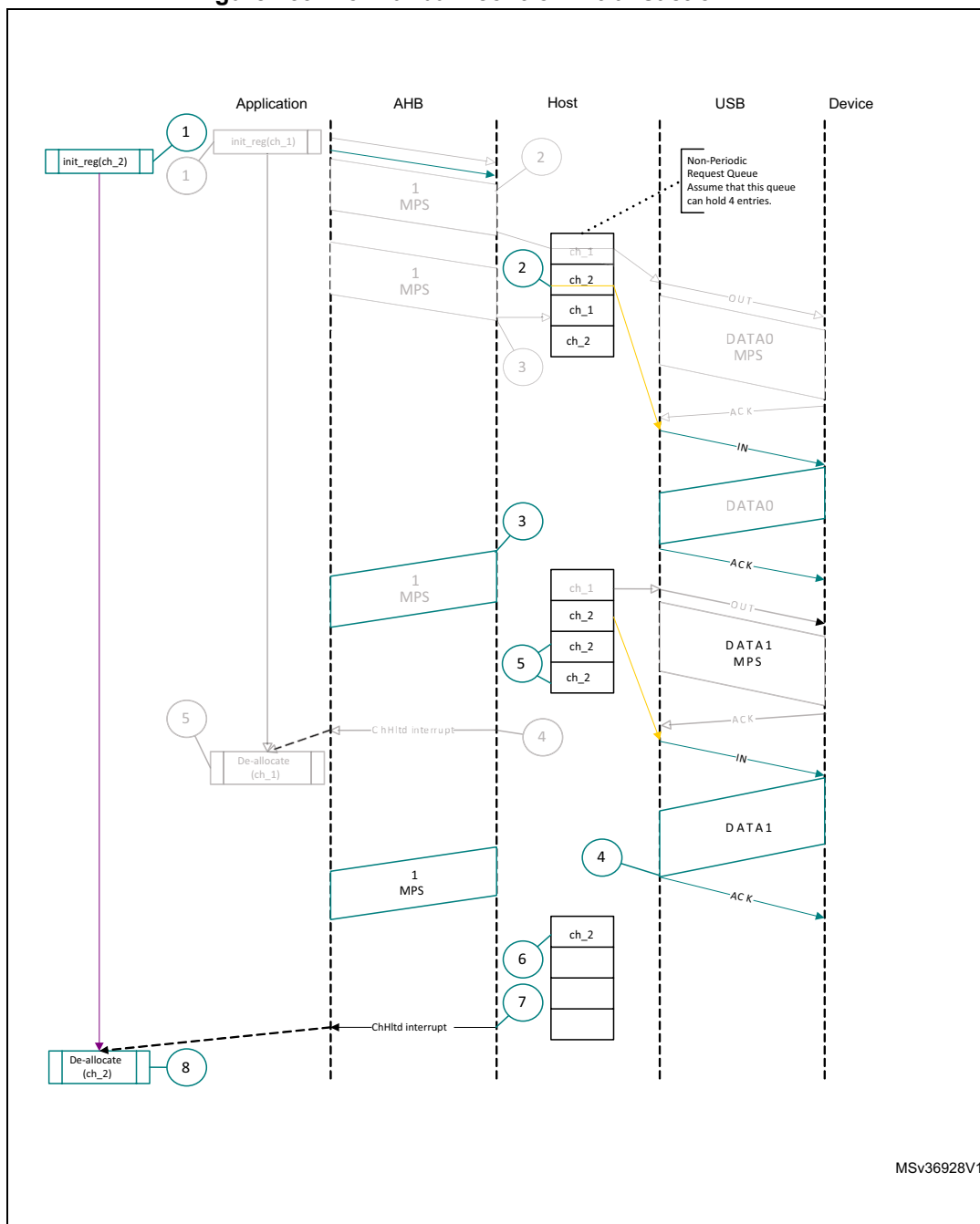
Figure 739. Normal bulk/control IN transaction - DMA
