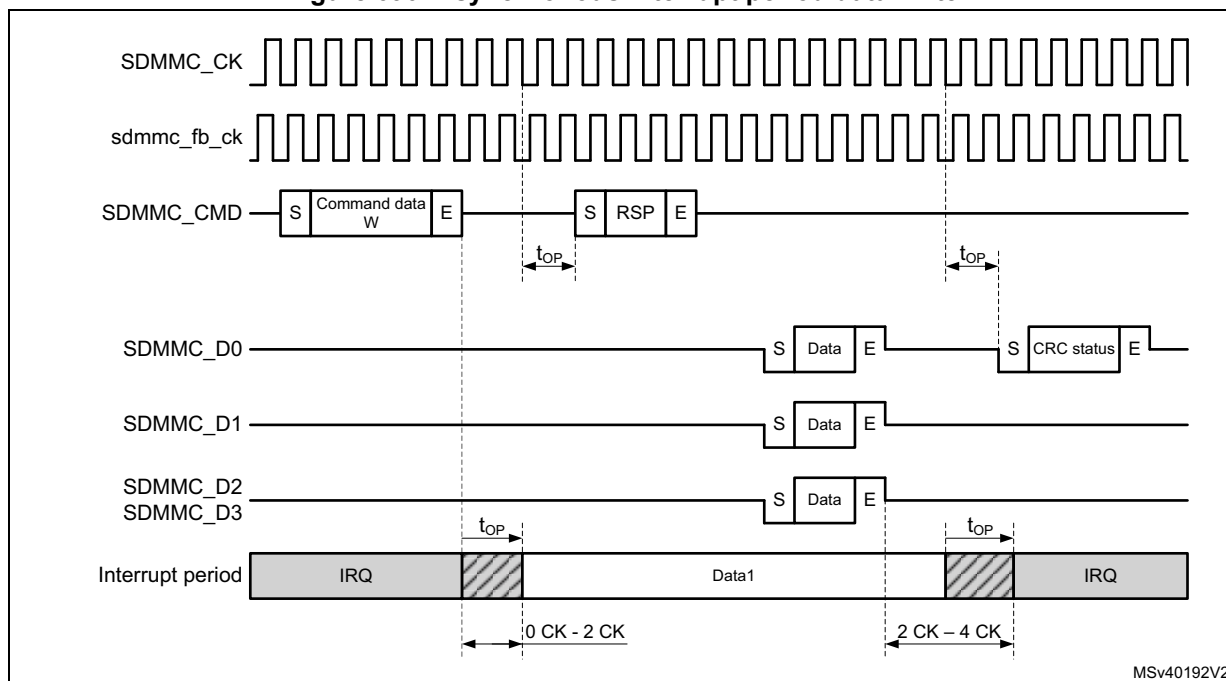
Figure 690. Asynchronous interrupt period data write
