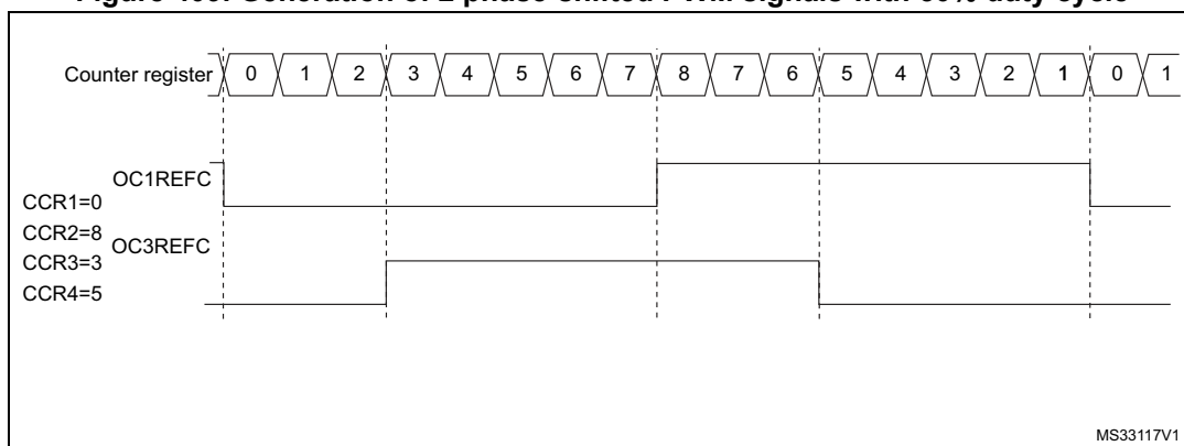
Figure 409. Generation of 2 phase-shifted PWM signals with 50% duty cycle
