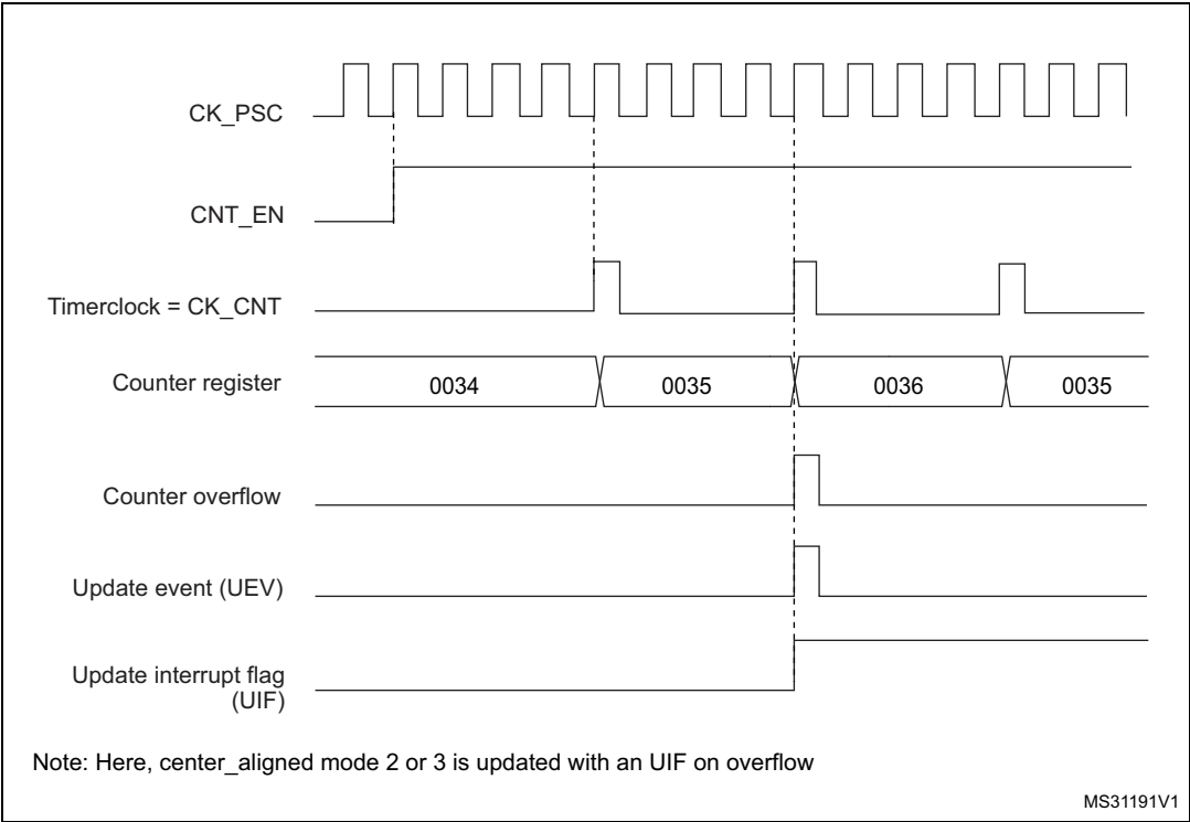
Figure 333. Counter timing diagram, internal clock divided by 4, TIMx_ARR=0x36
