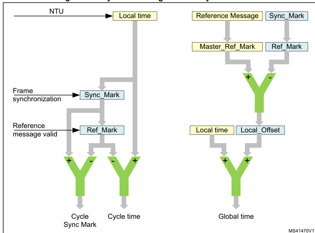
Figure 717. Cycle time and global time synchronization
