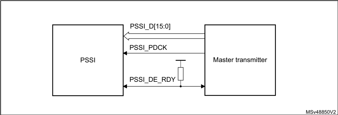
Figure 275. Bidirectional PSSI_DE/PSSI_RDY connection diagram
