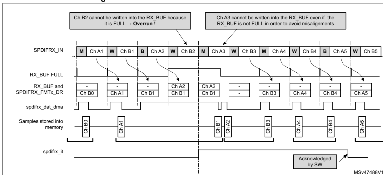
Figure 654. S/PDIF overrun error when RXSTEO = 1
