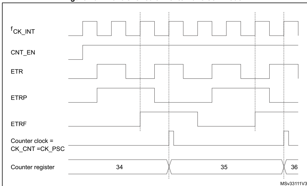
Figure 401. Control circuit in external clock mode 2
