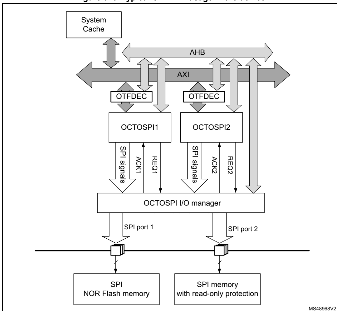
Figure 313. Typical OTFDEC usage in the device
