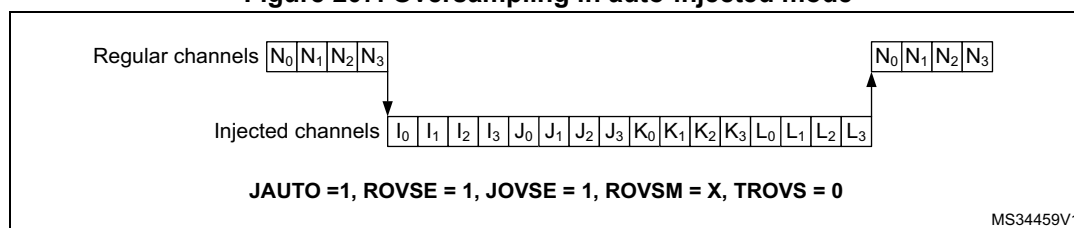
Figure 207. Oversampling in auto-injected mode
