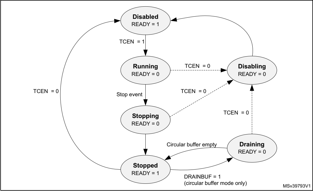
Figure 771. ETF state transition diagram
