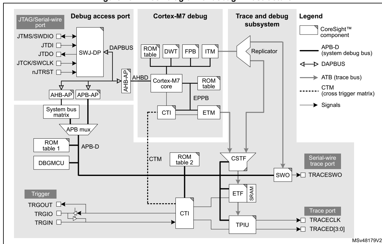
Figure 762. Block diagram of debug infrastructure
