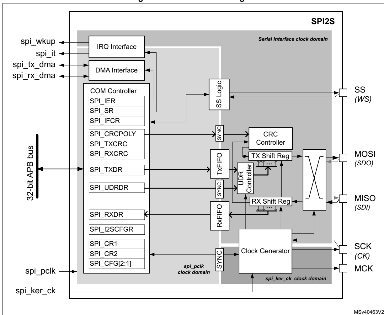
Figure 583. SPI2S block diagram
