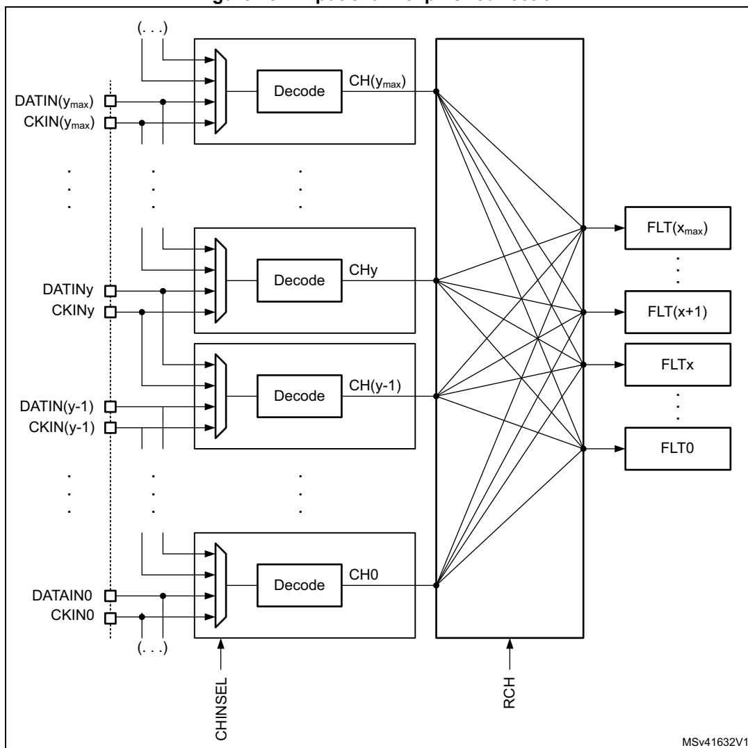
Figure 254. Input channel pins redirection
