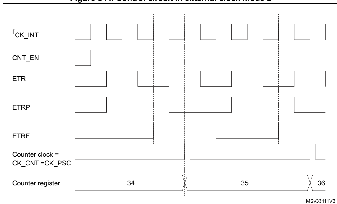
Figure 344. Control circuit in external clock mode 2
