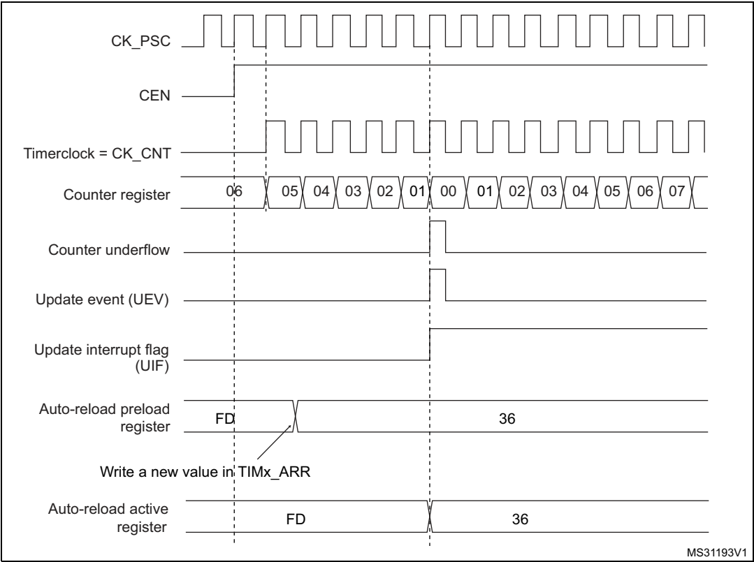
Figure 395. Counter timing diagram, Update event with ARPE=1 (counter underflow)
