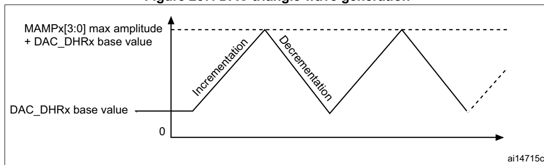
Figure 237. DAC triangle wave generation
