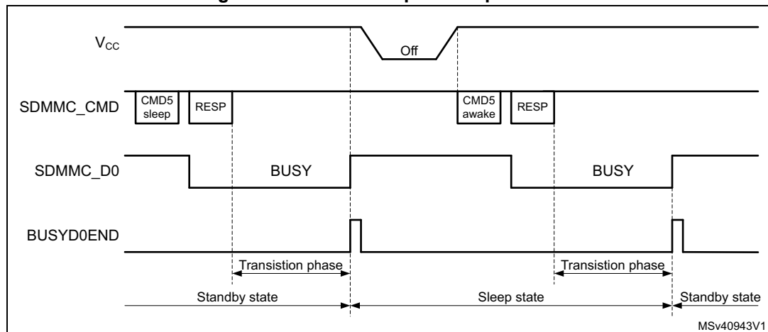
Figure 696. CMD5 Sleep Awake procedure
