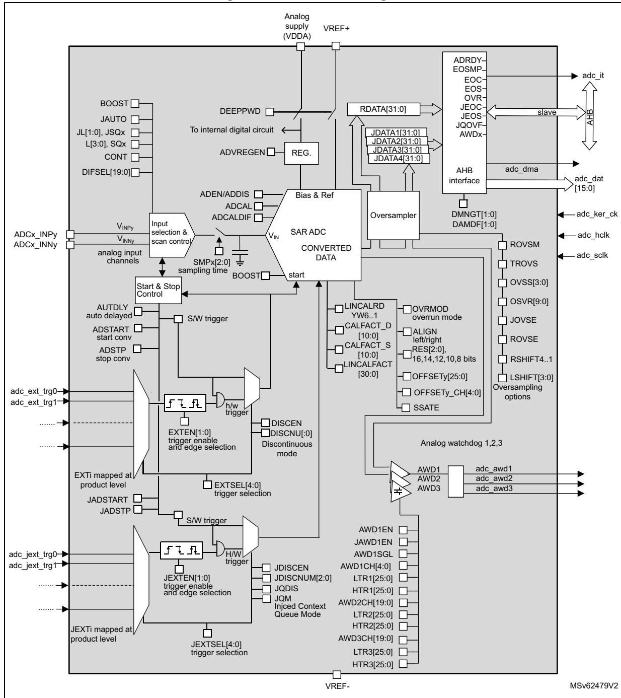
Figure 157. ADC block diagram
