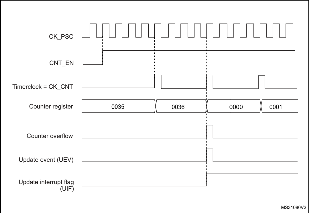
Figure 322. Counter timing diagram, internal clock divided by 4
