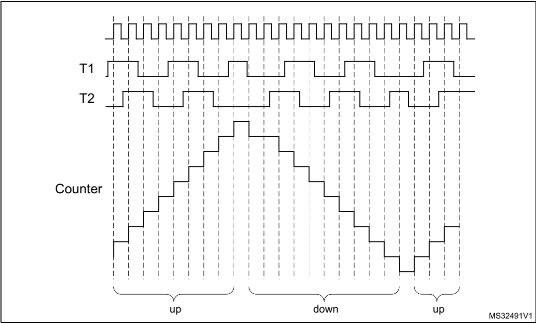
Figure 505. Encoder mode counting sequence
