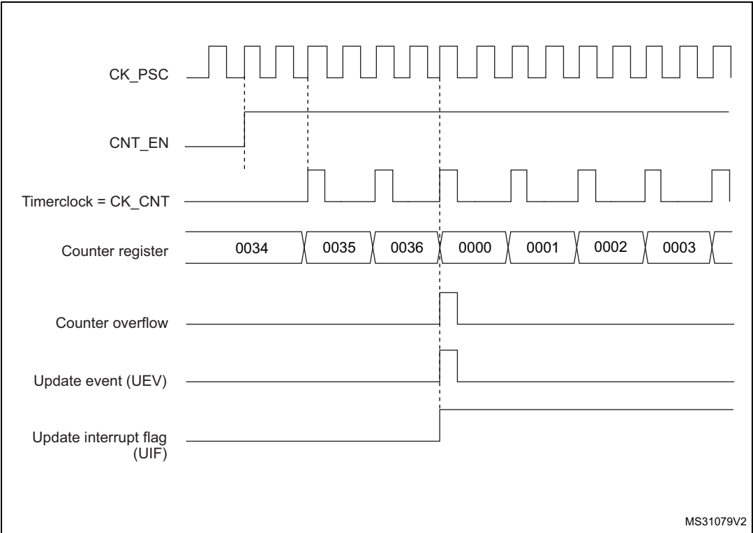
Figure 381. Counter timing diagram, internal clock divided by 2
