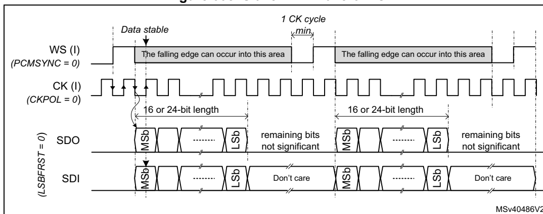
Figure 608. Slave PCM waveforms
