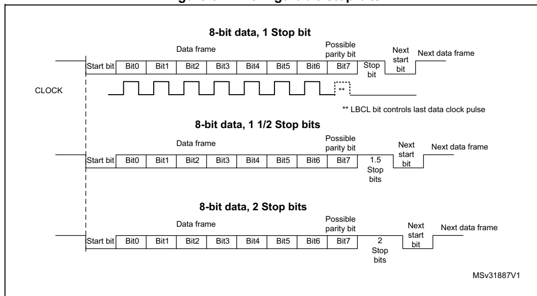
Figure 544. Configurable stop bits
