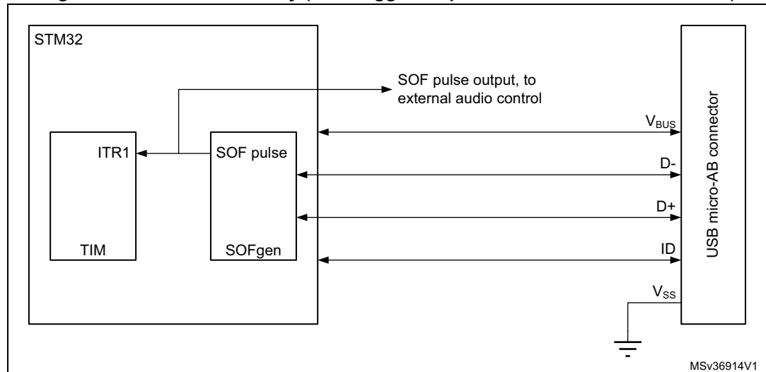
Figure 725. SOF connectivity (SOF trigger output to TIM and ITR1 connection)
