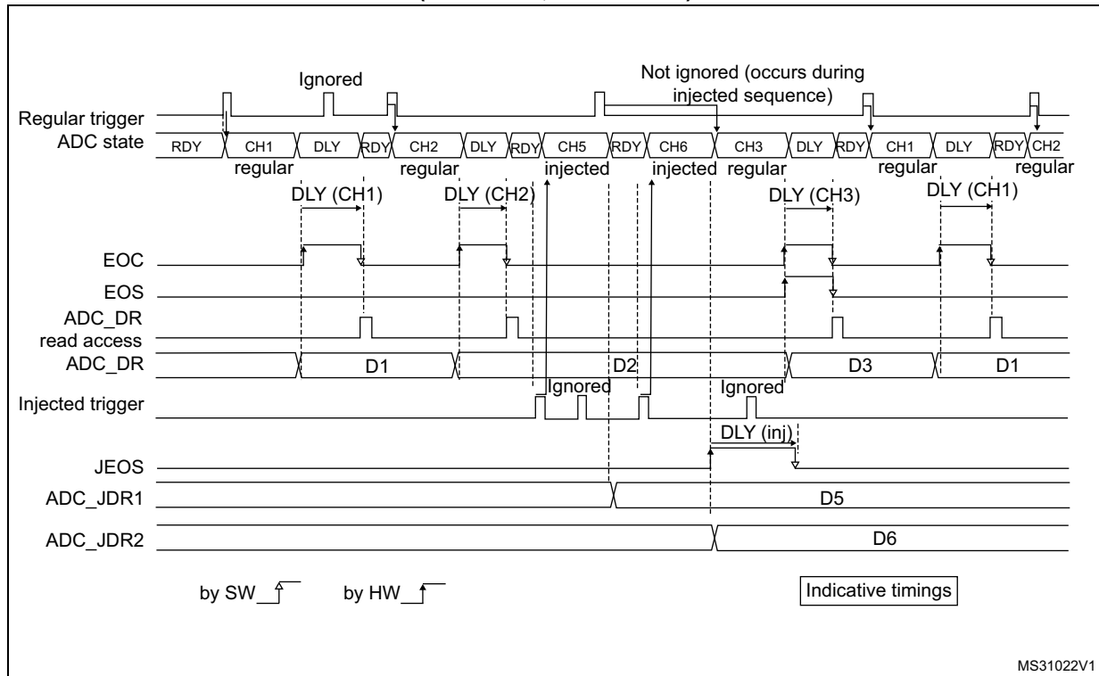
Figure 194. AUTDLY=1, regular HW conversions interrupted by injected conversions (DISCEN=1, JDISCEN=1)
