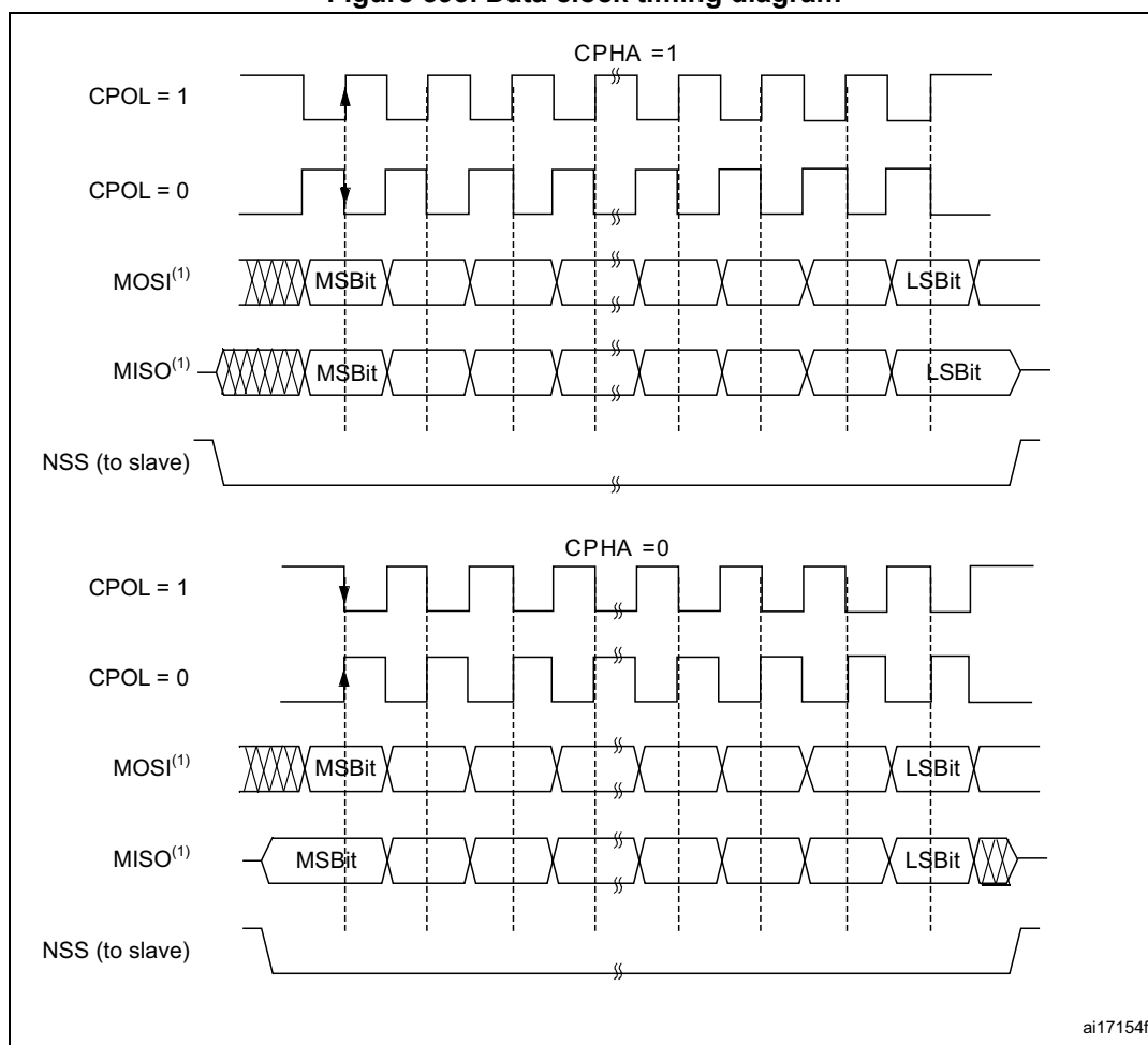
Figure 593. Data clock timing diagram
