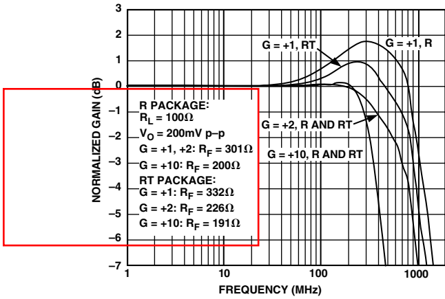
TPC 1. Frequency Response; G = +1, +2, +10 , R and RT Packages
