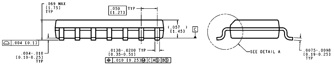
CONTROLLING DIMENSION IS INCH VALUES IN [ ] ARE MILLIMETERS
