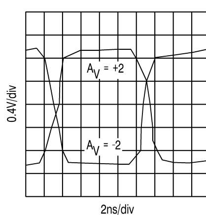
Pulse Response
