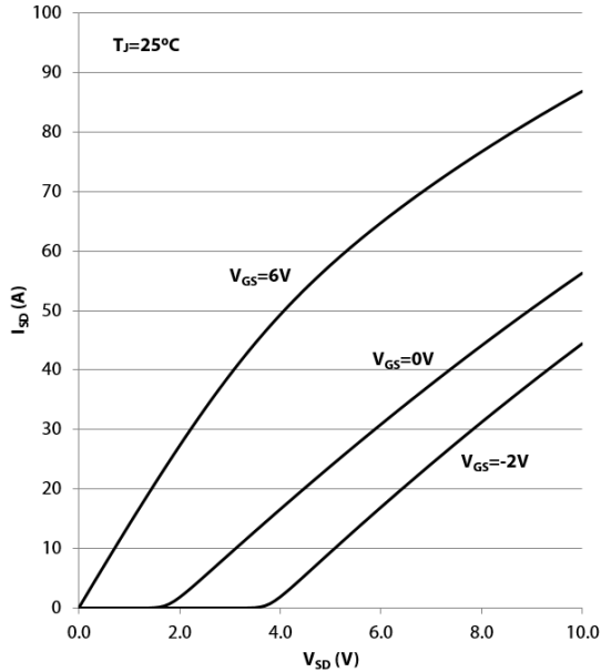
GS66506T Reverse Conduction Characteristics
