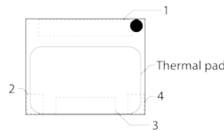
Package Outline
