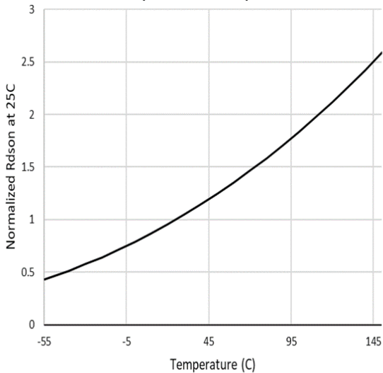
R_{DS(on)} Temperature Dependence
