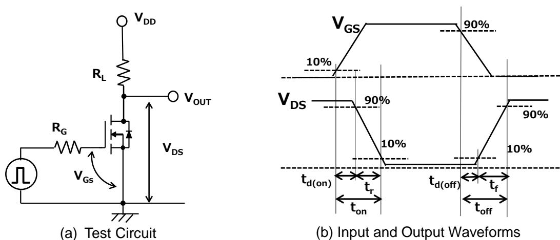
Figure 1.3 Switching Time Test Circuit and Input/Output Waveforms
