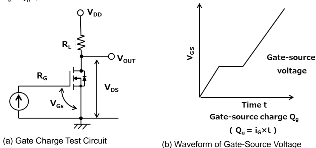
Figure 1.6 Gate Charge
