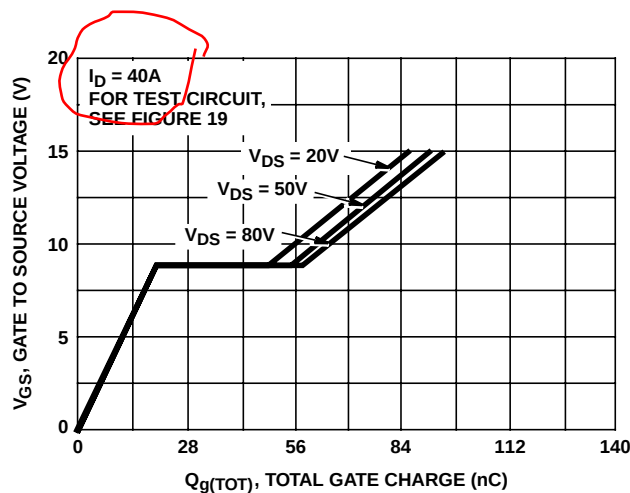
FIGURE 14. GATE TO SOURCE VOLTAGE vs GATE CHARGE
